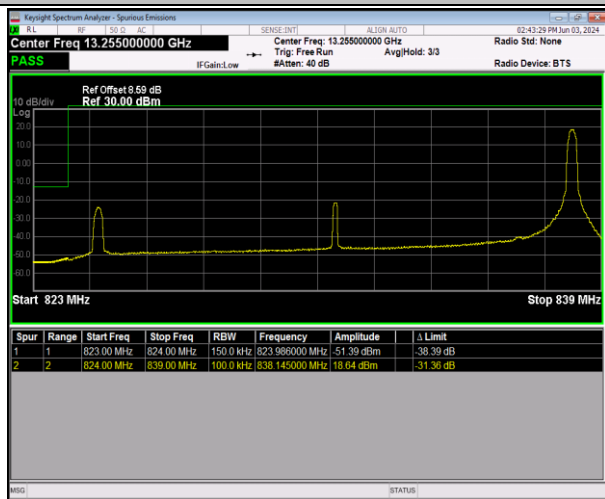
Band26_15MHz_QPSK_26865_1RB#74
