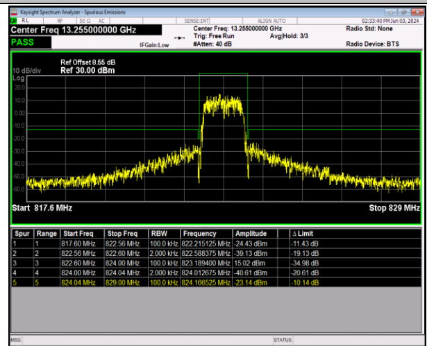
Band26_1.4MHz_64QAM_26783_6RB#0
