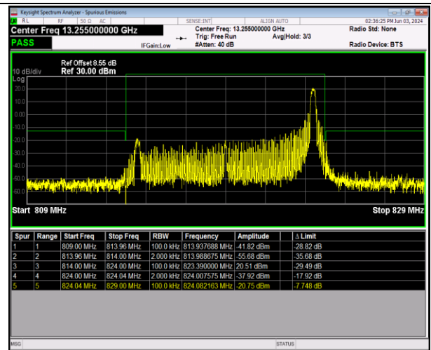
Band26_10MHz_QPSK_26740_1RB#49
