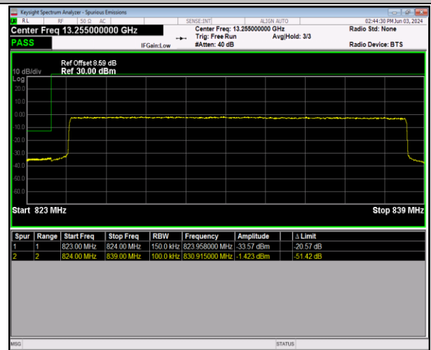
Band26_15MHz_QPSK_26865_75RB#0
