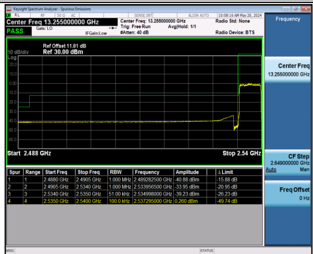
Band41_5MHz_64QAM_40065_25RB#0
