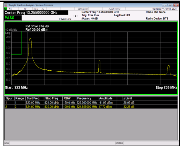
Band26_15MHz_64QAM_26865_1RB#0
