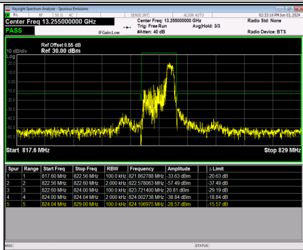
Band26_1.4MHz_64QAM_26783_1RB#5
