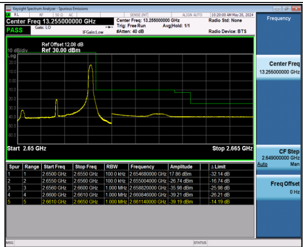
Band41_5MHz_16QAM_41215_1RB#24
