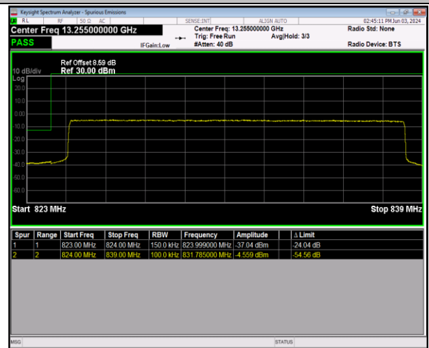
Band26_15MHz_64QAM_26865_75RB#0
