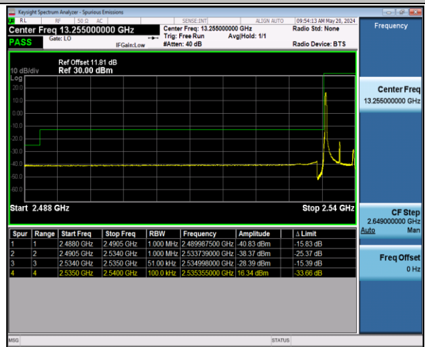
Band41_5MHz_64QAM_40065_1RB#0
