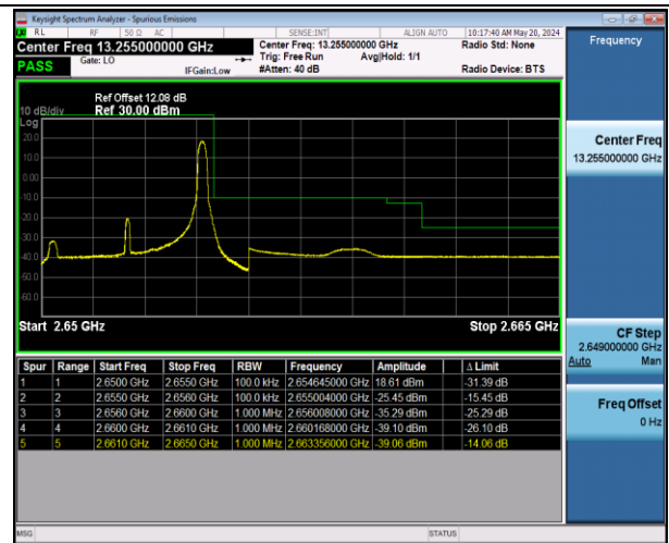
Band41_5MHz_QPSK_41215_1RB#24
