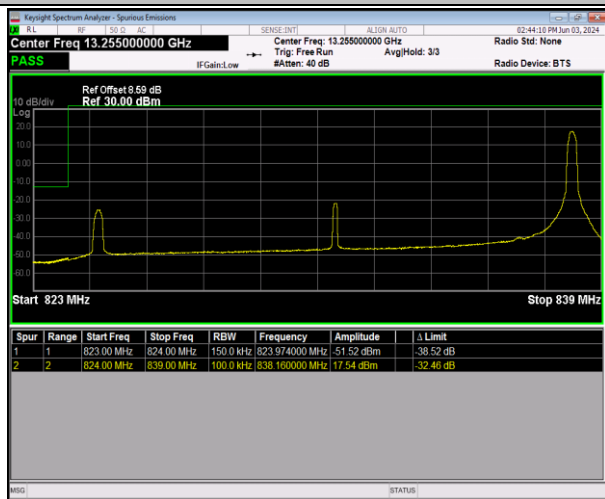
Band26_15MHz_64QAM_26865_1RB#74
