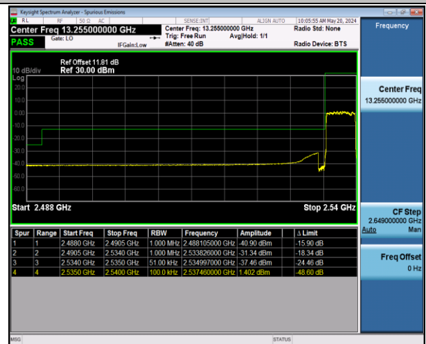
Band41_5MHz_16QAM_40065_25RB#0
