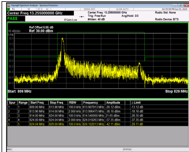
Band26_10MHz_QPSK_26740_1RB#0
