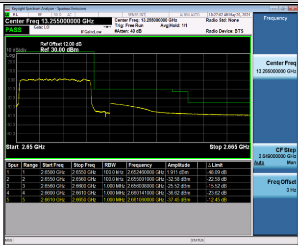
Band41_5MHz_16QAM_41215_25RB#0
