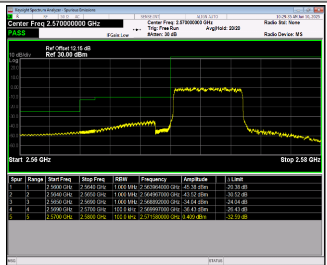
Band38-5MHz-16QAM-38225-1RB#24
