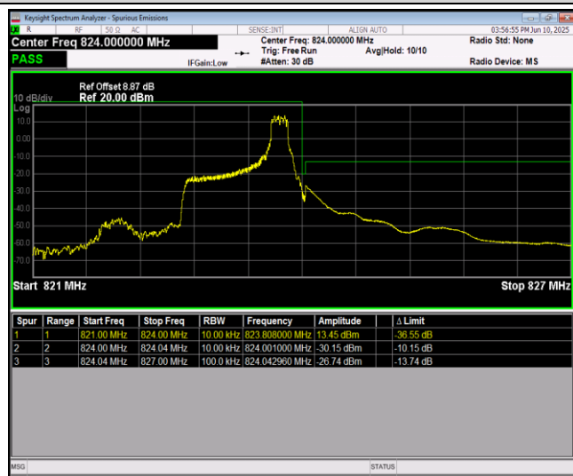
Band26-1.4MHz-64QAM-26797-1RB#0
