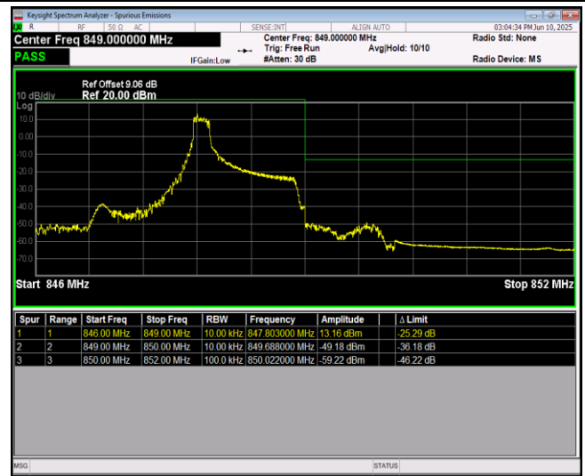
Band26-1.4MHz-64QAM-27033-6RB#0
