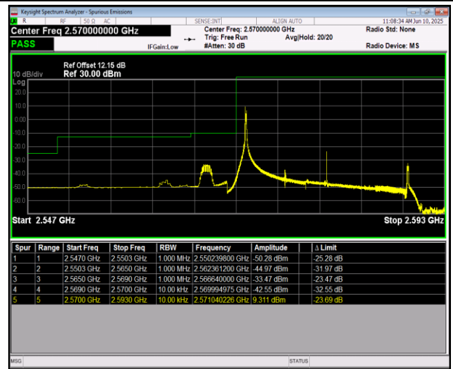
Band38-20MHz-QPSK-37850-100RB#0
