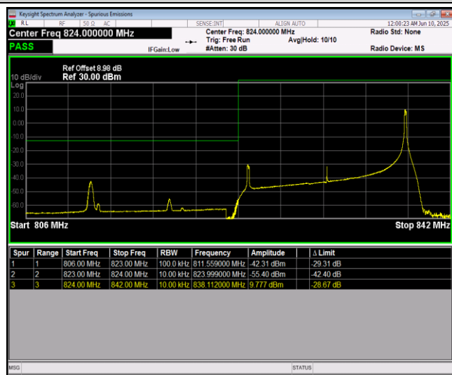
Band26-15MHz-64QAM-26965-1RB#0
