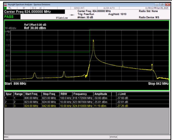
Band26-15MHz-16QAM-26865-75RB#0
