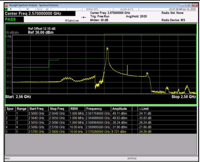
Band38-5MHz-QPSK-37775-25RB#0
