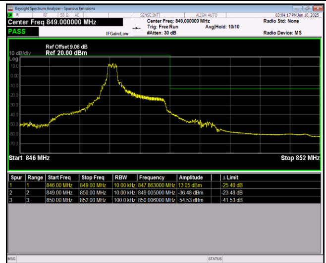
Band26-1.4MHz-16QAM-27033-6RB#0
