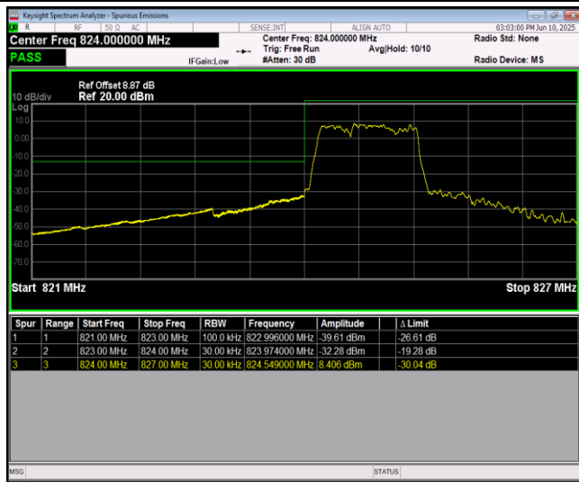
Band26-1.4MHz-64QAM-27033-1RB#5
