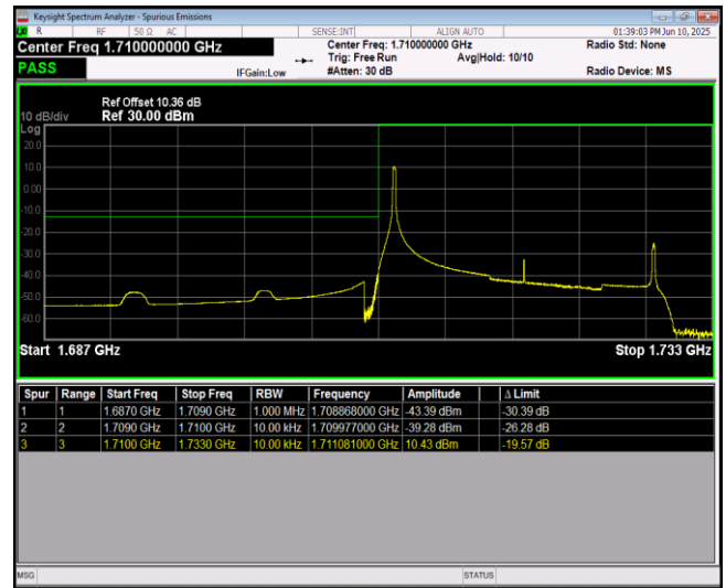
Band66-20MHz-QPSK-132072-100RB#0
