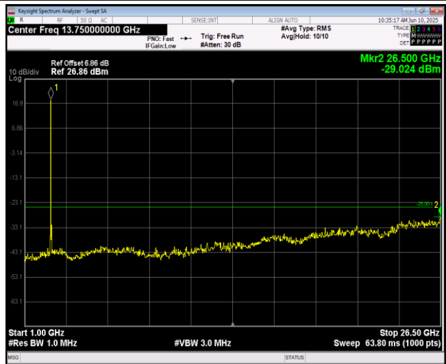
Band38-5MHz-16QAM-37775-1RB#0-Range2:1000~ 26500MHz
