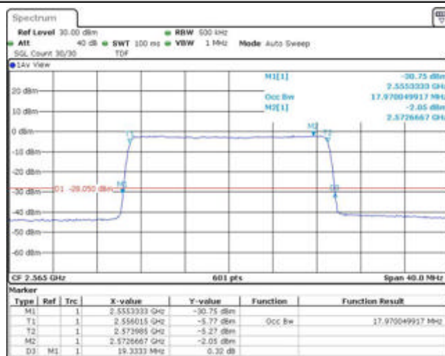
Band41-20MHz-16QAM-40590-100RB#0
