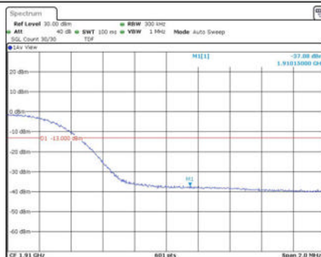
Band2-15MHz-16QAM-19125-75RB#0
