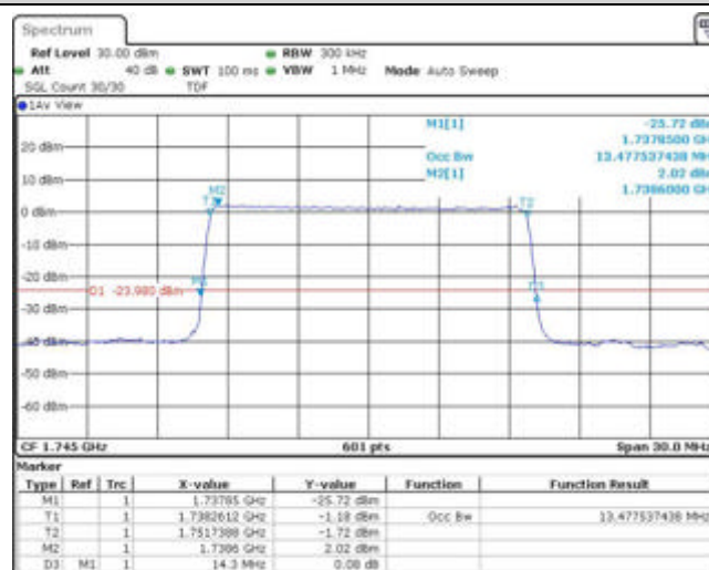
Band66-15MHz-16QAM-132322-75RB#0
