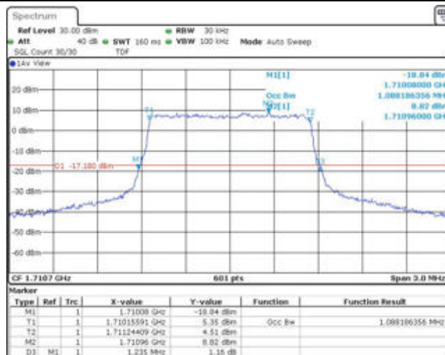
Band66-1.4MHz-QPSK-132322-6RB#0
