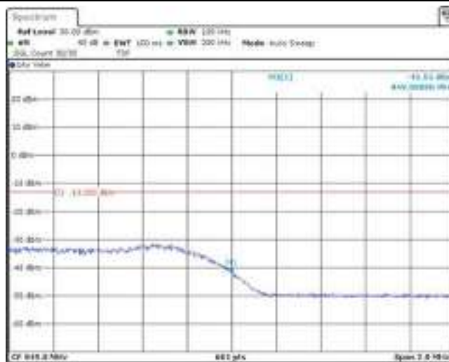
Band5-5MHz-QPSK-20625-1RB#24
