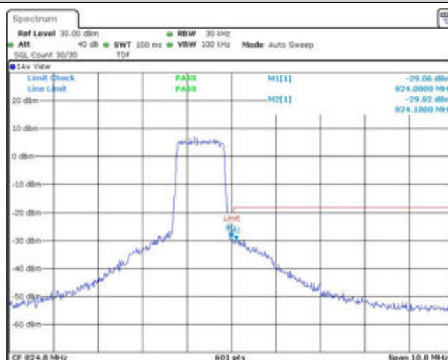
Band26-1.4MHz-16QAM-26797-1RB#0
