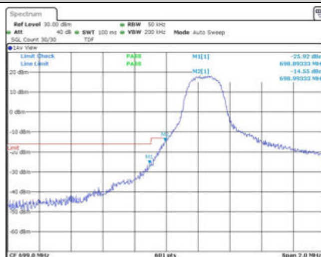
Band12-3MHz-QPSK-23025-1RB#14
