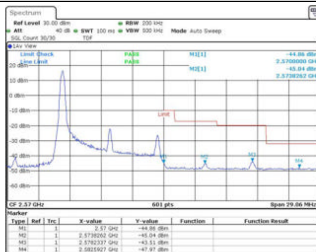
Band7-10MHz-16QAM-21400-1RB#49
