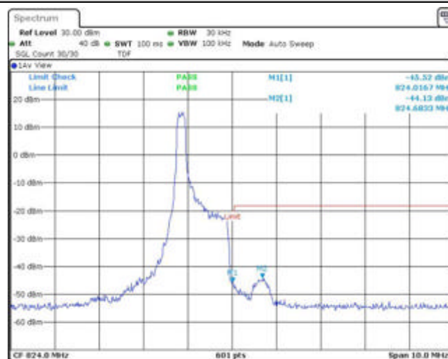
Band26-1.4MHz-QPSK-26783-1RB#5
