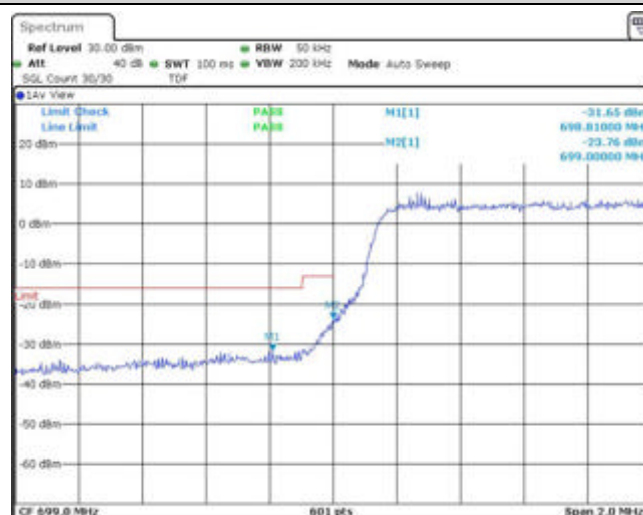
Band12-3MHz-QPSK-23025-15RB#0
