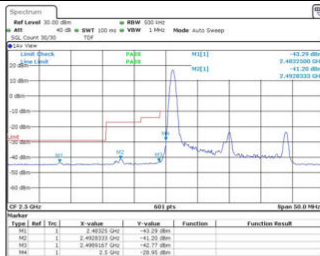
Band7-20MHz-16QAM-20850-1RB#99
