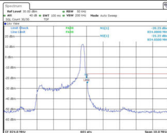
Band26-3MHz-QPSK-26775-15RB#0
