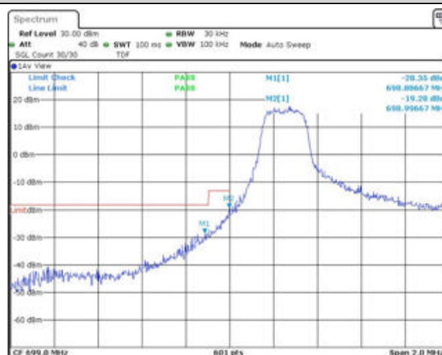
Band12-1.4MHz-16QAM-23017-1RB#5
