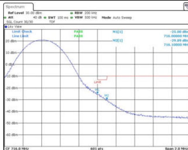
Band12-10MHz-QPSK-23130-50RB#0
