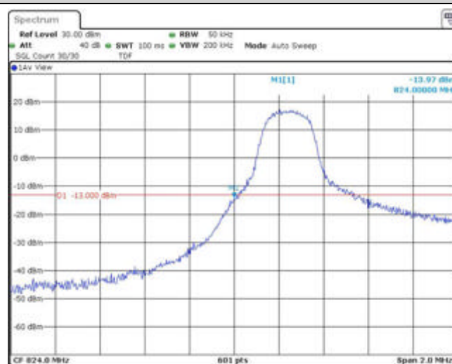
Band26-3MHz-QPSK-26805-1RB#14
