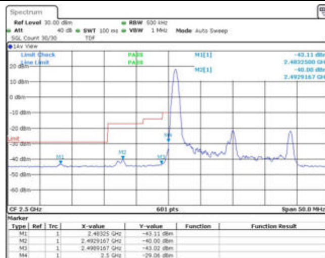
Band7-20MHz-QPSK-20850-1RB#99
