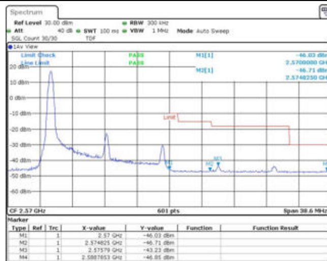
Band7-15MHz-16QAM-21375-1RB#74
