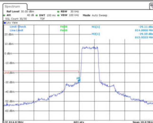
Band26-1.4MHz-QPSK-26697-6RB#0
