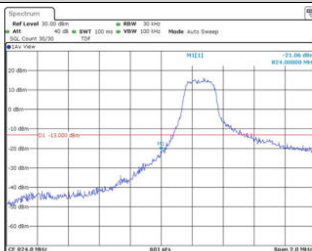
Band26-1.4MHz-16QAM-26797-1RB#5
