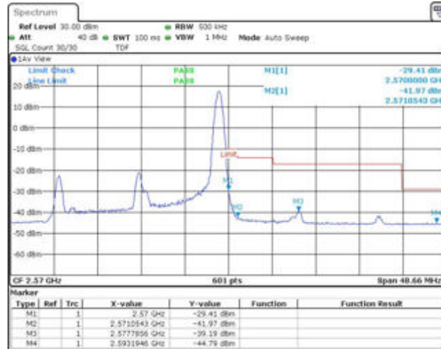
Band7-20MHz-16QAM-21350-100RB#0
