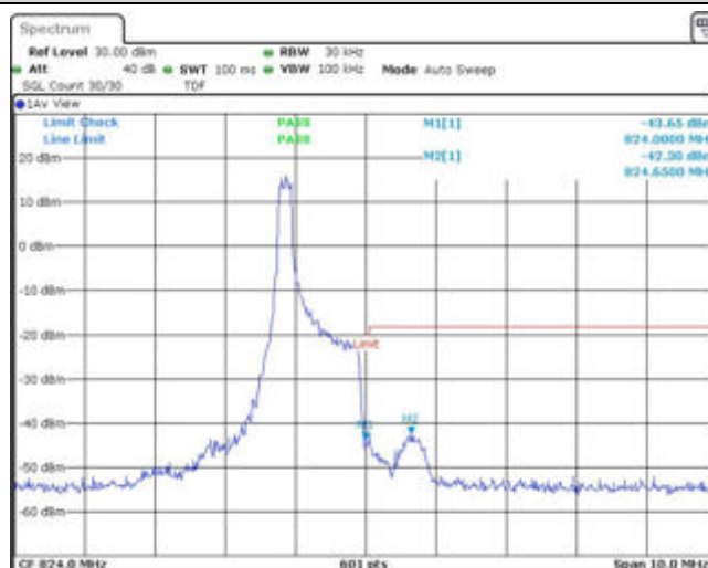
Band26-1.4MHz-16QAM-26783-1RB#5
