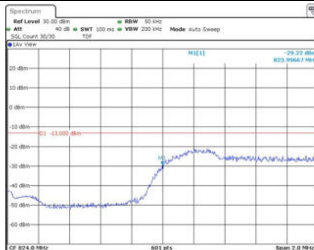
Band26-3MHz-QPSK-26805-15RB#0
