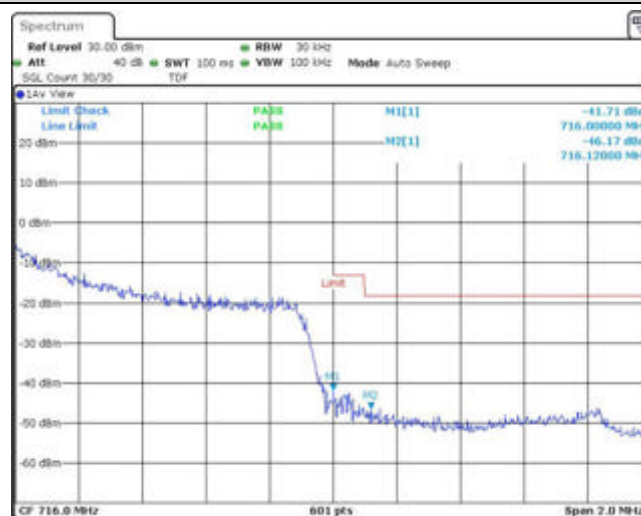
Band12-1.4MHz-QPSK-23173-1RB#5
