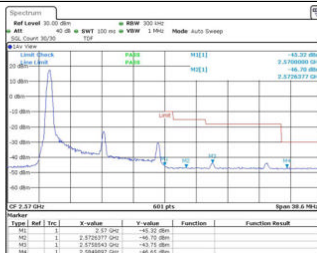
Band7-15MHz-QPSK-21375-1RB#74
