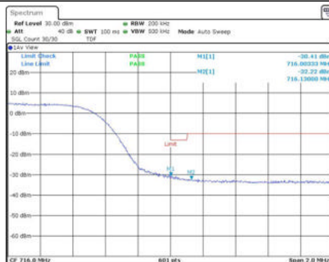
Band17-10MHz-16QAM-23780-1RB#0
