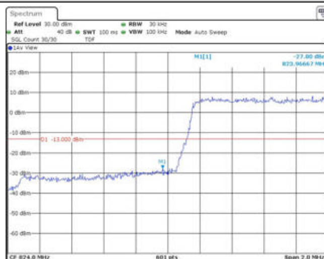
Band26-1.4MHz-QPSK-26797-6RB#0
