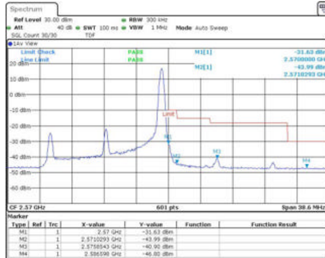
Band7-15MHz-16QAM-21375-75RB#0
