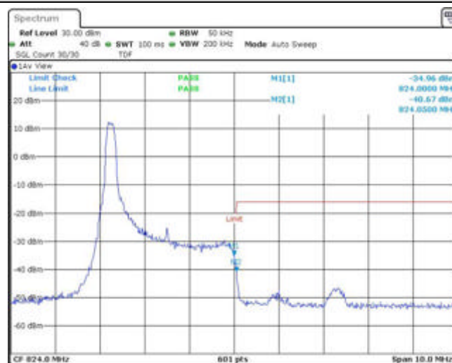
Band26-3MHz-QPSK-26775-1RB#14
