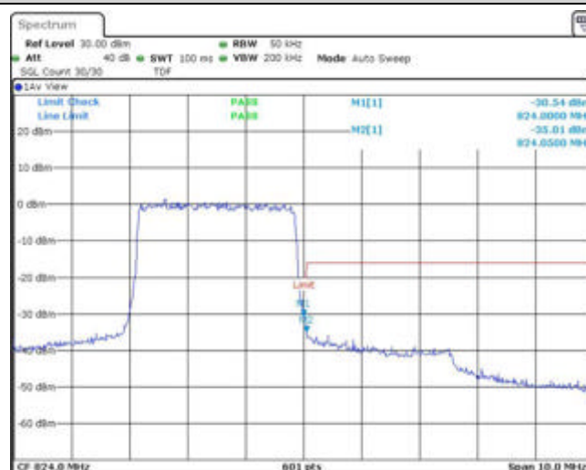
Band26-3MHz-QPSK-26775-15RB#0
