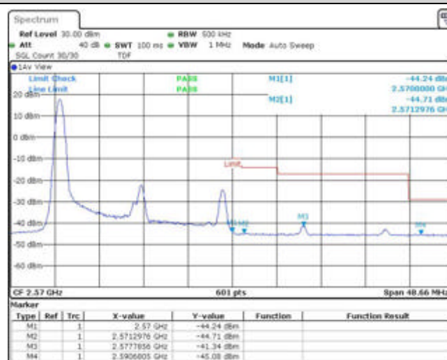
Band7-20MHz-QPSK-21350-1RB#99
