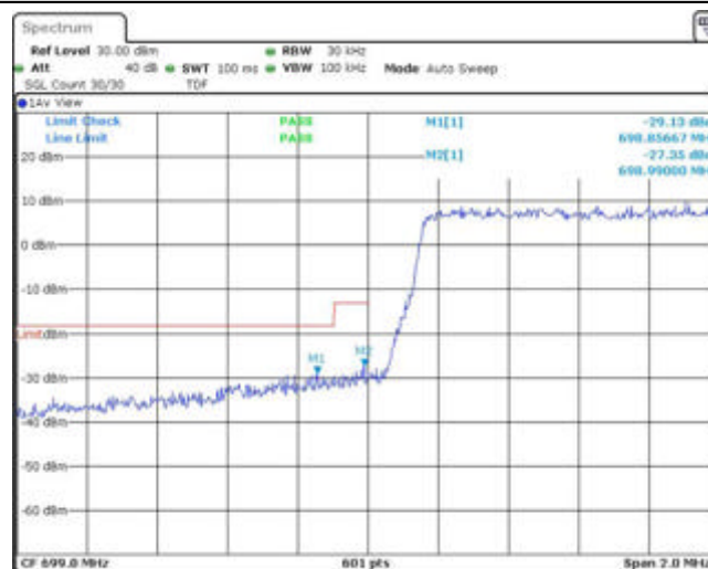
Band12-1.4MHz-QPSK-23173-1RB#0
