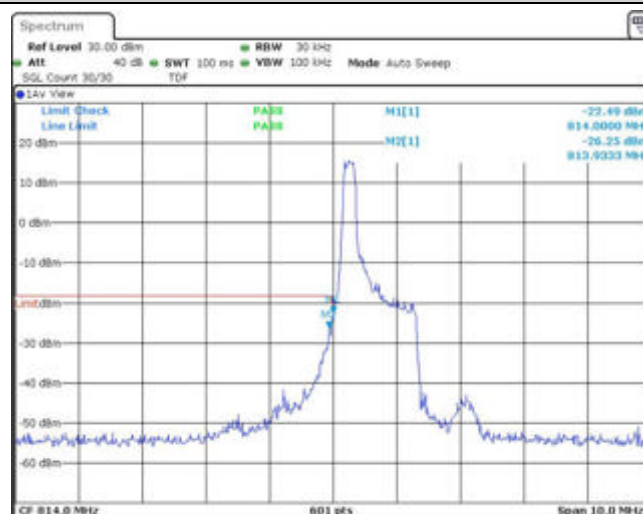
Band26-1.4MHz-QPSK-26697-1RB#5
