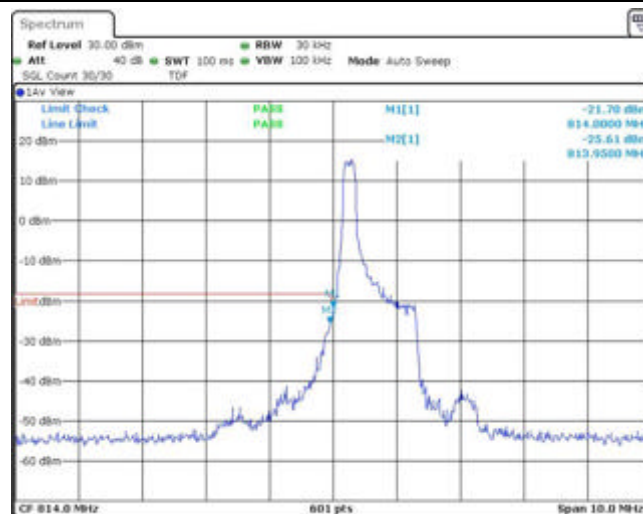
Band26-1.4MHz-16QAM-26697-1RB#5
