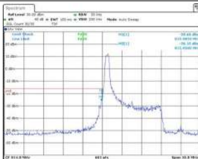
Band26-3MHz-16QAM-26705-1RB#14
