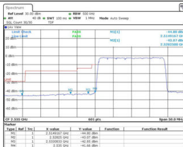
Band41-20MHz-16QAM-40140-100RB#0
