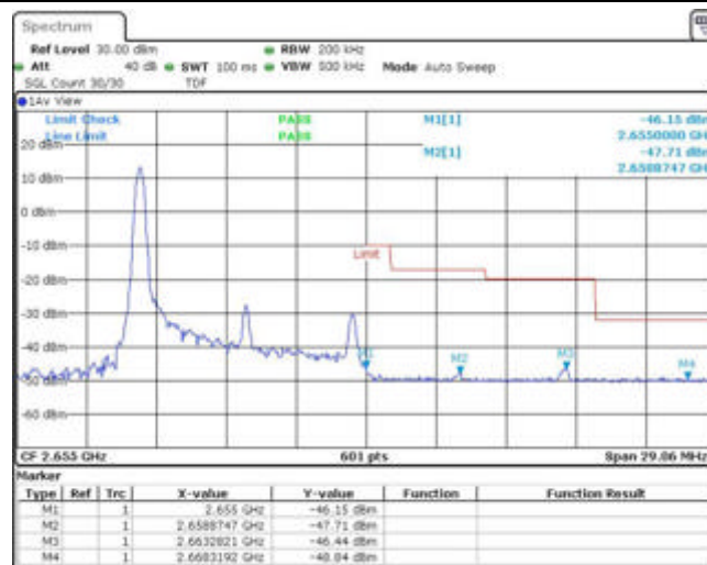
Band41-10MHz-QPSK-41190-1RB#49
