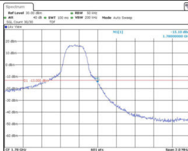
Band66-3MHz-QPSK-132657-15RB#0
