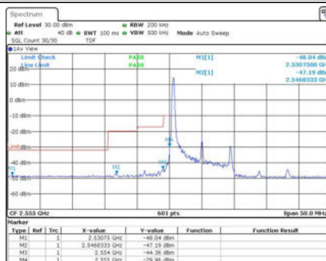
Band41-10MHz-16QAM-40290-1RB#49
