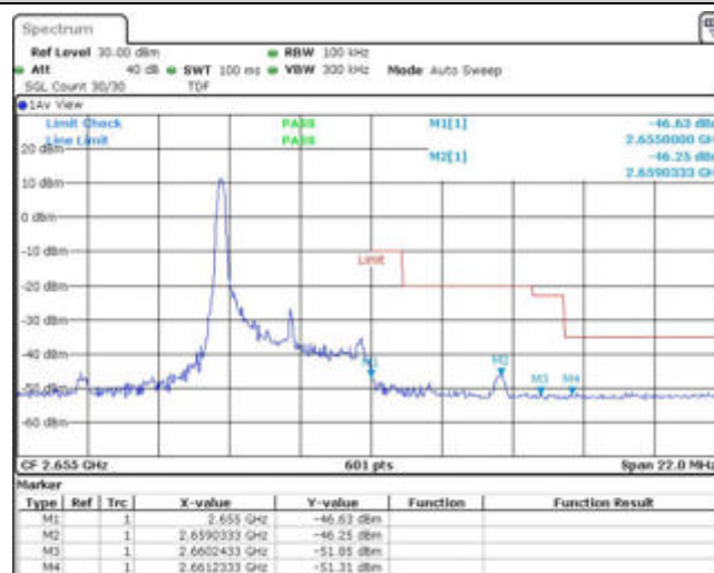
Band41-5MHz-16QAM-41215-1RB#24
