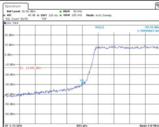
Band66-1.4MHz-QPSK-132665-1RB#0
