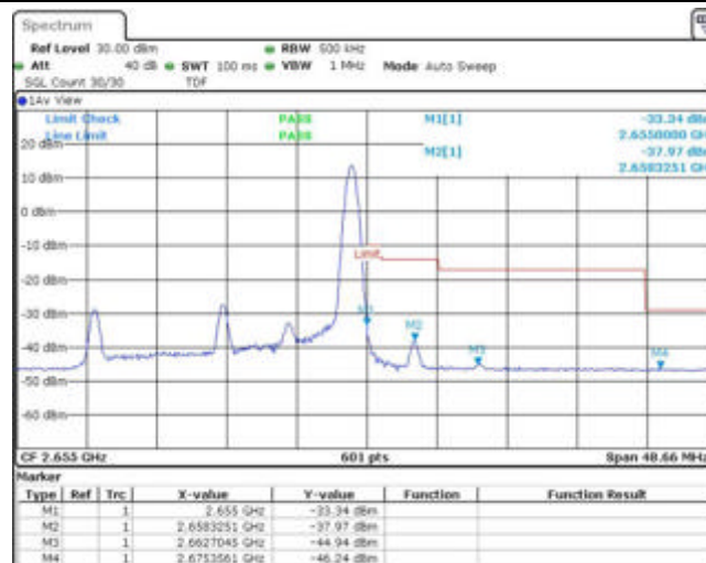
Band41-20MHz-QPSK-41140-100RB#0
