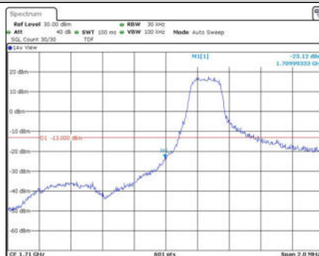
Band66-1.4MHz-QPSK-131979-1RB#5
