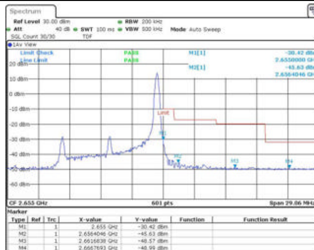
Band41-10MHz-16QAM-41190-50RB#0
