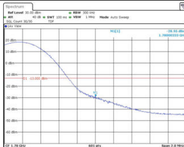
Band66-15MHz-QPSK-132597-75RB#0
