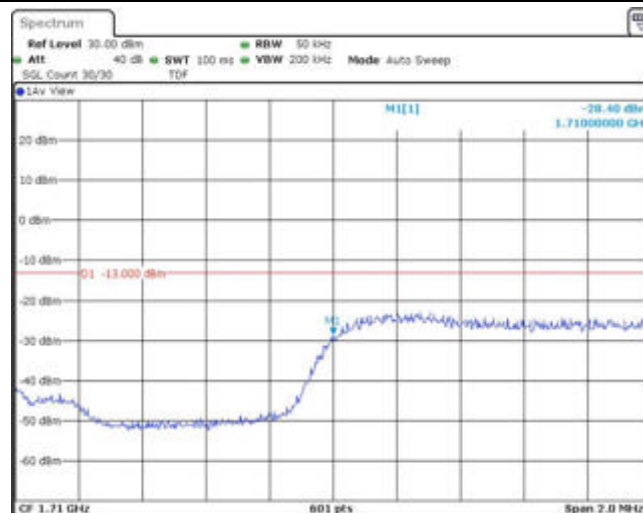
Band66-3MHz-QPSK-131987-15RB#0
