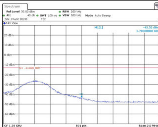
Band66-10MHz-16QAM-132622-1RB#49
