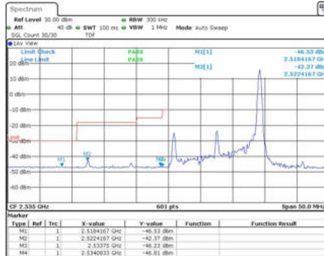
Band41-15MHz-16QAM-40115-75RB#0
