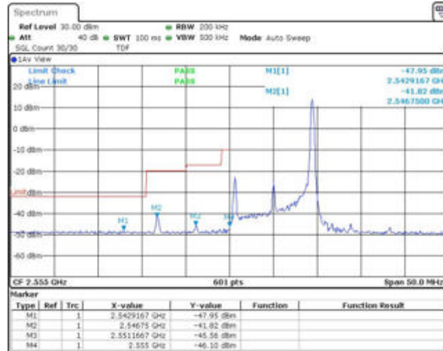
Band41-10MHz-16QAM-40290-50RB#0
