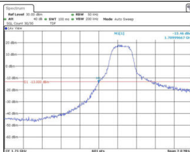
Band66-3MHz-16QAM-131987-1RB#14
