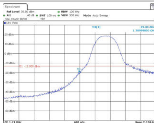
Band66-5MHz-QPSK-131997-1RB#24
