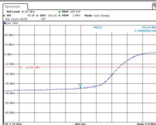
Band66-15MHz-QPSK-132047-75RB#0
