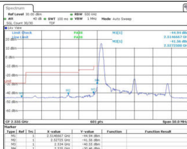
Band41-20MHz-16QAM-40140-1RB#99
