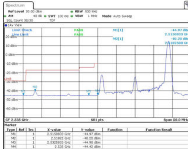
Band41-20MHz-QPSK-40140-100RB#0
