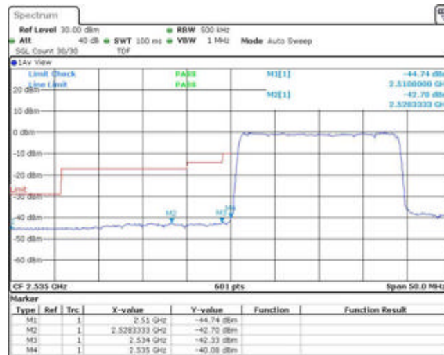
Band41-20MHz-QPSK-40340-1RB#0
