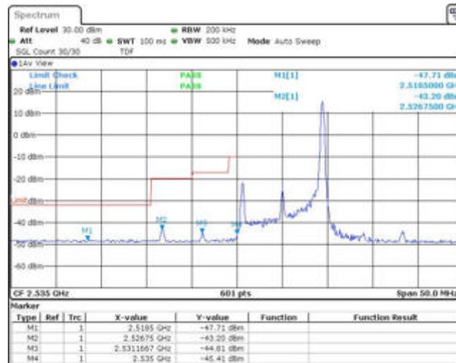
Band41-10MHz-QPSK-40090-50RB#0
