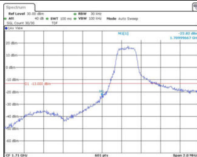
Band66-1.4MHz-16QAM-131979-1RB#5
