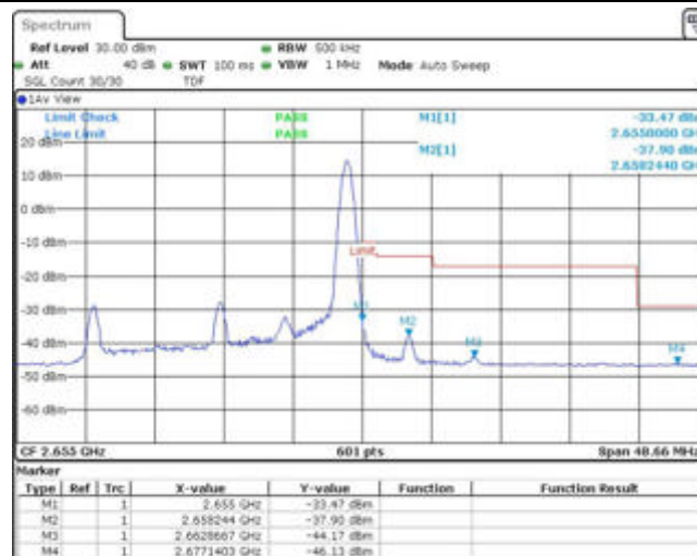
Band41-20MHz-16QAM-41140-100RB#0
