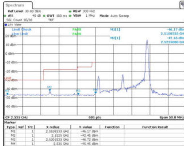
Band41-15MHz-QPSK-40115-75RB#0
