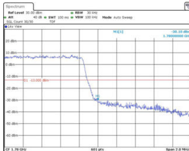
Band66-1.4MHz-16QAM-131979-1RB#0
