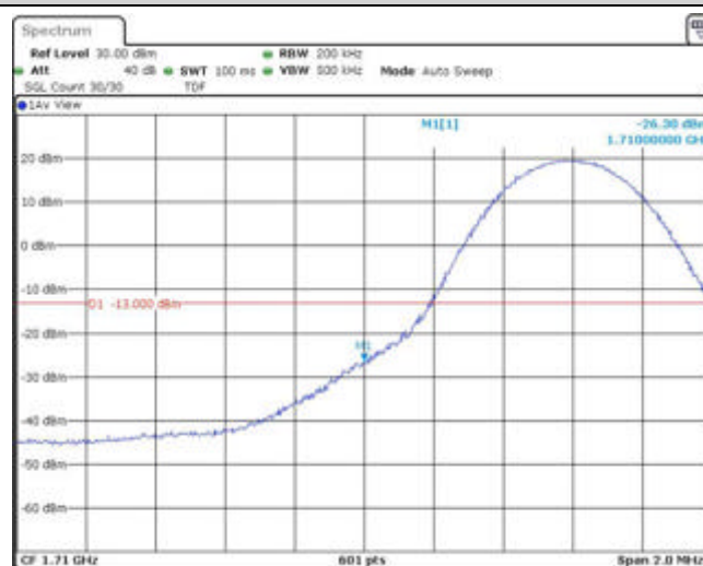
Band66-10MHz-QPSK-132022-1RB#49
