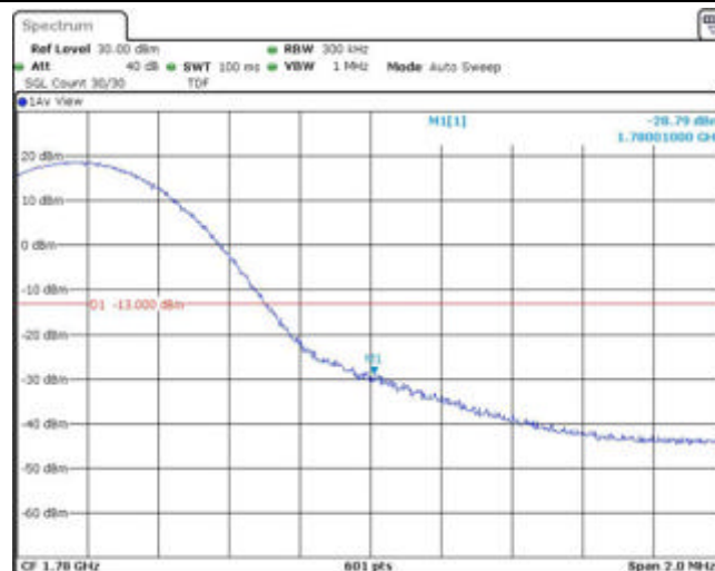
Band66-15MHz-16QAM-132597-75RB#0
