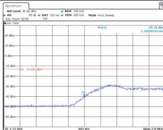
Band66-5MHz-16QAM-131997-25RB#0
