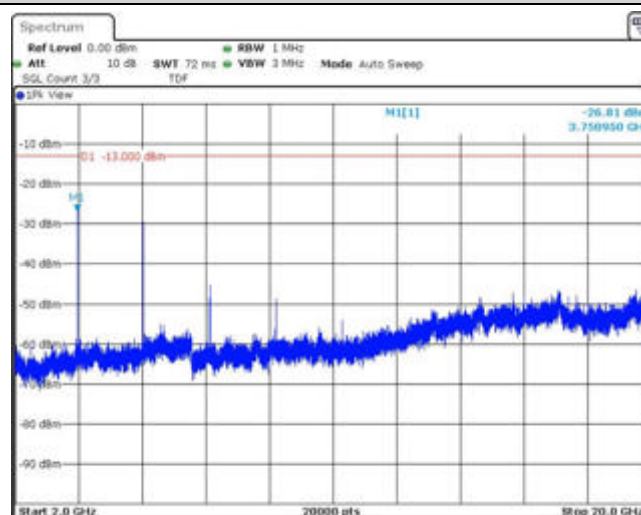
Band2-10MHz-QPSK-18900-1RB#0-Range3:2000~20000MHz
