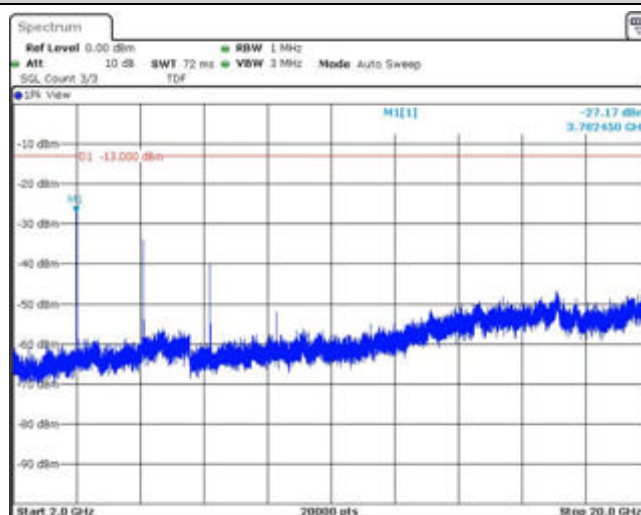
Band2-20MHz-16QAM-19100-1RB#0-Range3:2000~20000MHz
