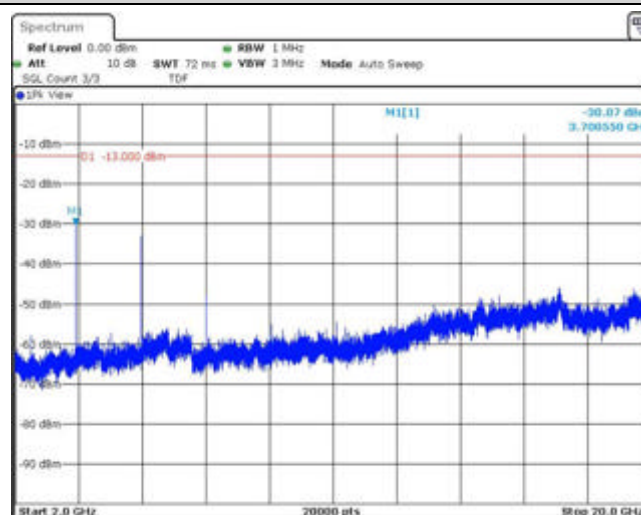
Band2-3MHz-16QAM-18615-1RB#0-Range3:2000~20000MHz
