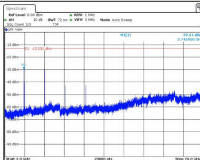
Band2-20MHz-16QAM-18900-1RB#0-Range3:2000~20000MHz
