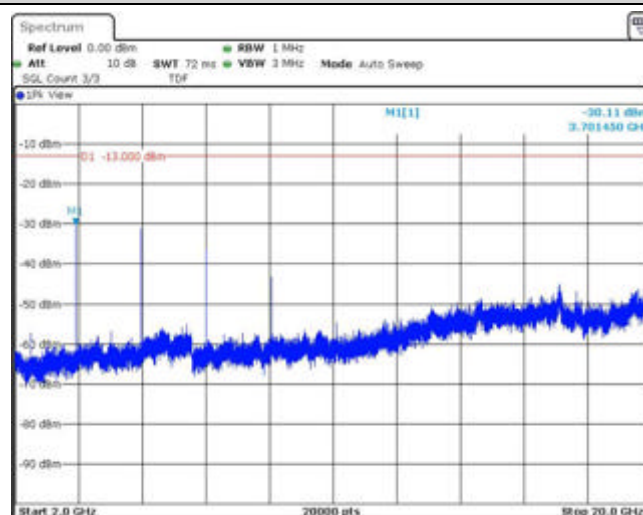
Band2-1.4MHz-16QAM-18607-1RB#0-Range3:2000~20000MHz
