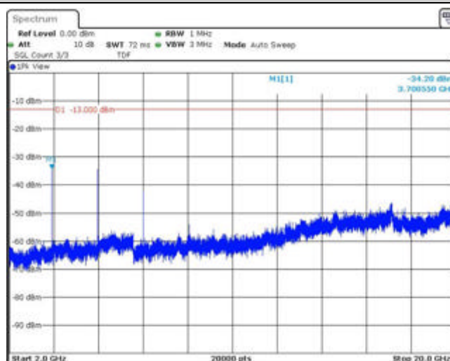
Band2-10MHz-QPSK-18650-1RB#0-Range3:2000~20000MHz
