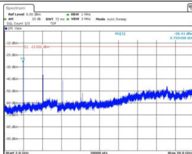
Band2-5MHz-QPSK-18900-1RB#0-Range3:2000~20000MHz
