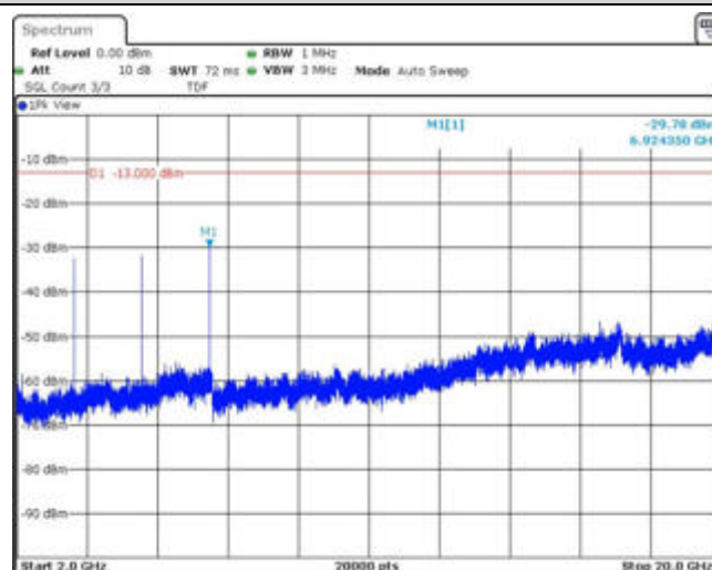
Band4-3MHz-16QAM-20175-1RB#0-Range3:2000~20000MHz
