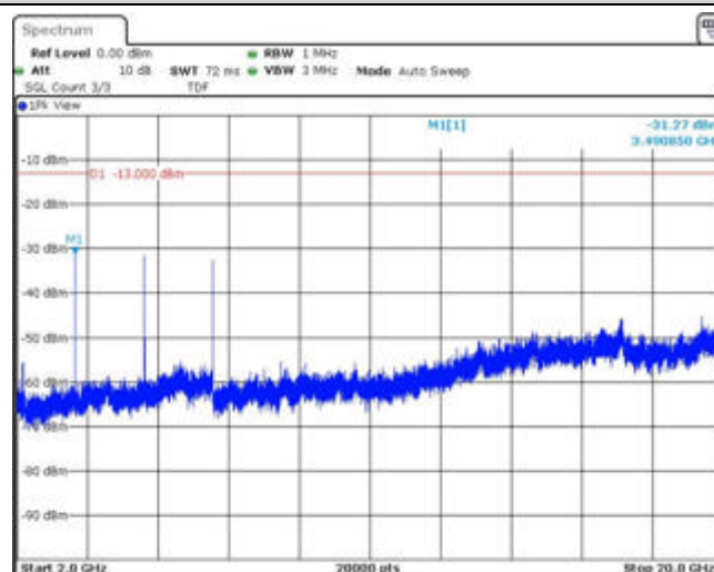
Band4-10MHz-16QAM-20350-1RB#0-Range3:2000~20000MHz
