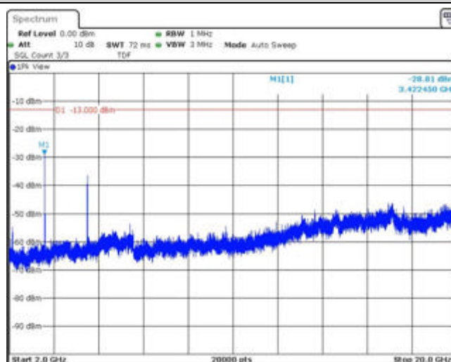
Band4-20MHz-16QAM-20050-1RB#0-Range3:2000~20000MHz
