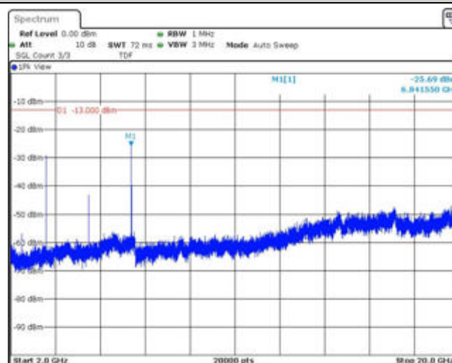
Band4-1.4MHz-16QAM-19957-1RB#0-Range3:2000~20000MHz
