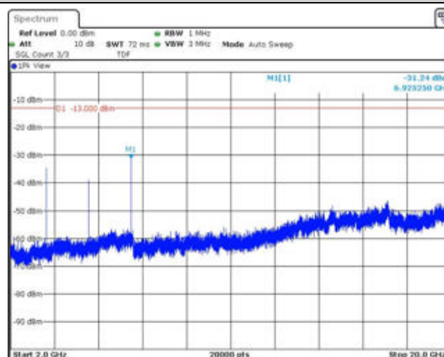
Band4-3MHz-QPSK-20175-1RB#0-Range3:2000~20000MHz
