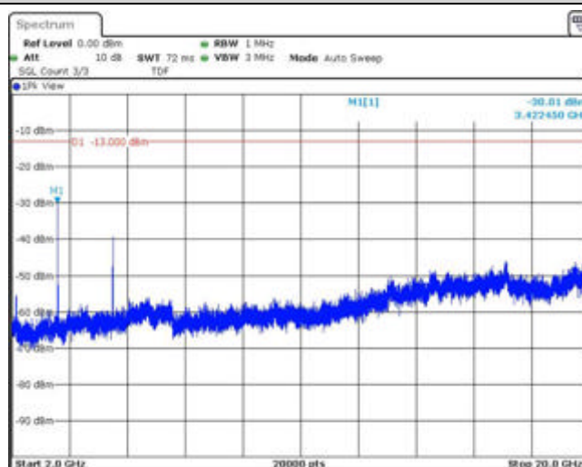
Band4-20MHz-QPSK-20050-1RB#0-Range3:2000~20000MHz
