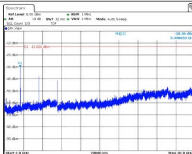
Band4-10MHz-QPSK-20350-1RB#0-Range3:2000~20000MHz
