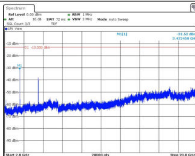
Band4-15MHz-16QAM-20025-1RB#0-Range3:2000~20000MHz
