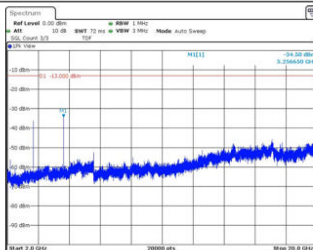
Band4-3MHz-QPSK-20385-1RB#0-Range3:2000~20000MHz
