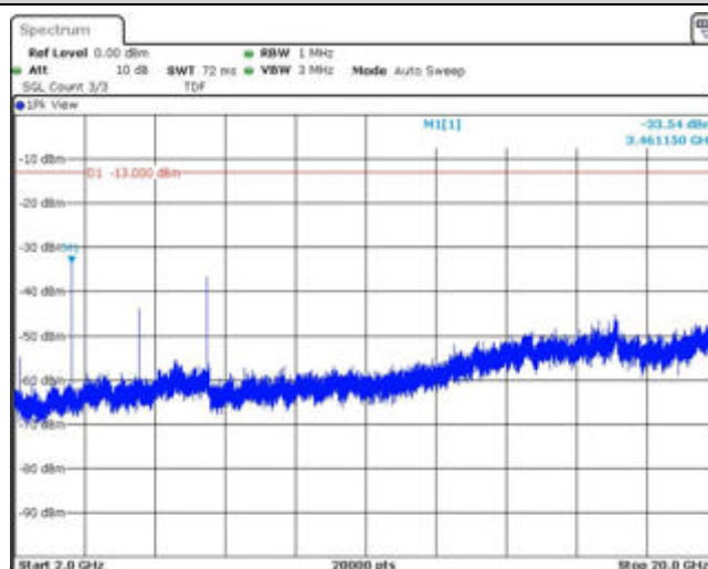
Band4-5MHz-QPSK-20175-1RB#0-Range3:2000~20000MHz
