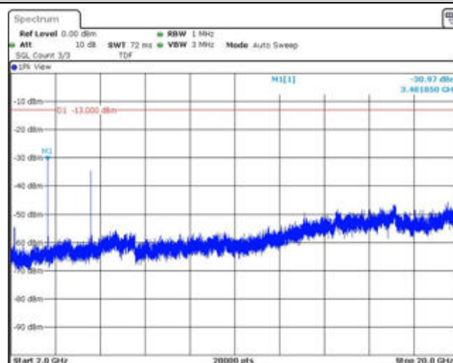
Band4-15MHz-16QAM-20325-1RB#0-Range3:2000~20000MHz
