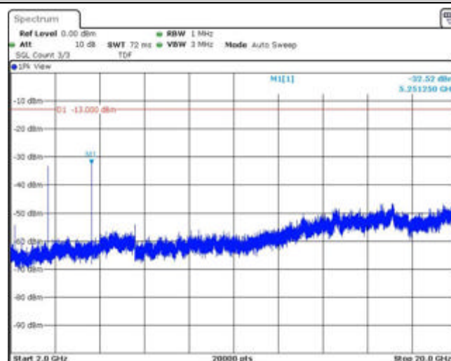
Band4-5MHz-16QAM-20375-1RB#0-Range3:2000~20000MHz
