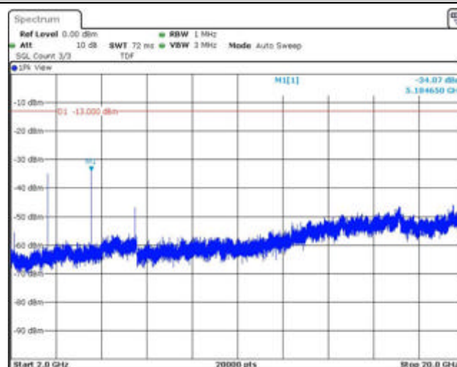
Band4-10MHz-QPSK-20175-1RB#0-Range3:2000~20000MHz
