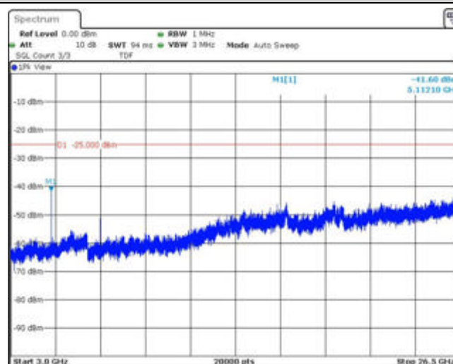
Band7-15MHz-16QAM-21375-1RB#0-Range3:3000~26500MHz
