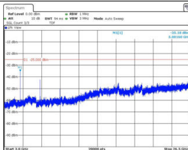
Band7-15MHz-QPSK-20825-1RB#0-Range3:3000~26500MHz
