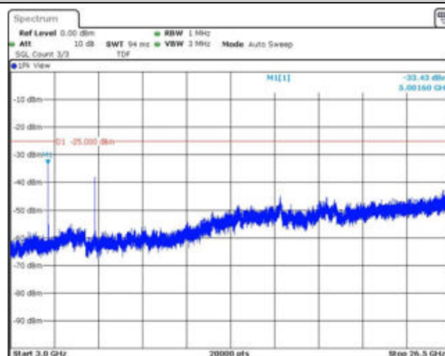
Band7-10MHz-16QAM-20800-1RB#0-Range3:3000~26500MHz
