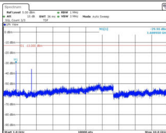
Band5-5MHz-16QAM-20625-1RB#0-Range2:1000~10000MHz
