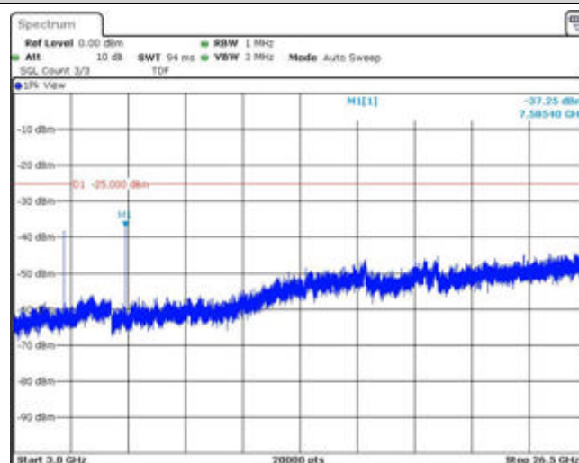
Band7-15MHz-16QAM-21375-1RB#0-Range1:30~1000MHz
