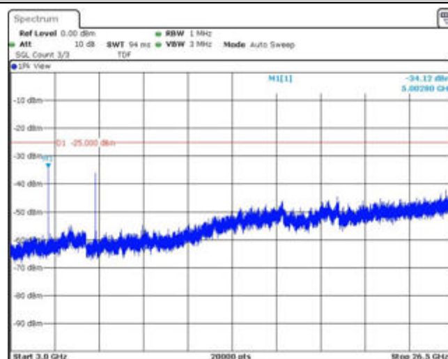
Band7-20MHz-16QAM-20850-1RB#0-Range3:3000~26500MHz
