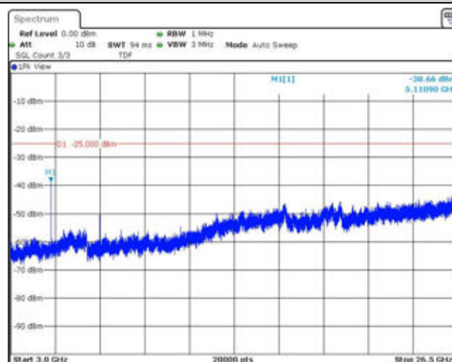
Band7-15MHz-QPSK-21375-1RB#0-Range3:3000~26500MHz
