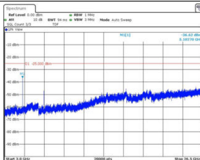
Band7-20MHz-16QAM-21350-1RB#0-Range3:3000~26500MHz
