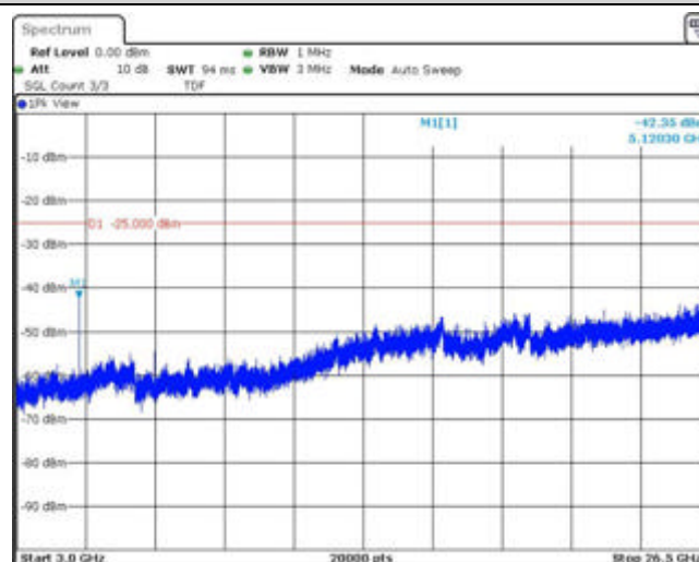
Band7-10MHz-16QAM-21400-1RB#0-Range3:3000~26500MHz
