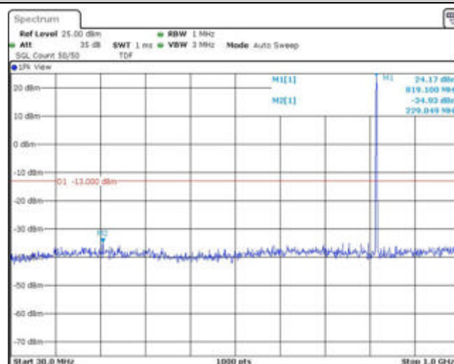
Band26-1.4MHz-QPSK-26740-1RB#0-Range1:30~1000MHz
