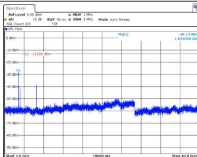
Band26-3MHz-QPSK-26775-1RB#0-Range2:1000~10000MHz
