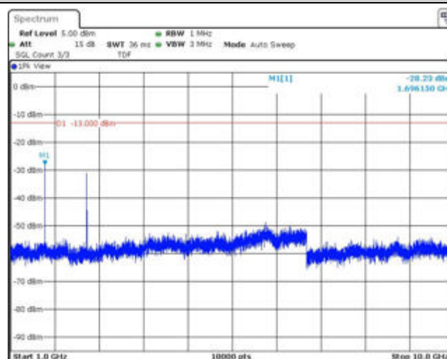
Band26-1.4MHz-QPSK-27033-1RB#0-Range2:1000~10000MHz
