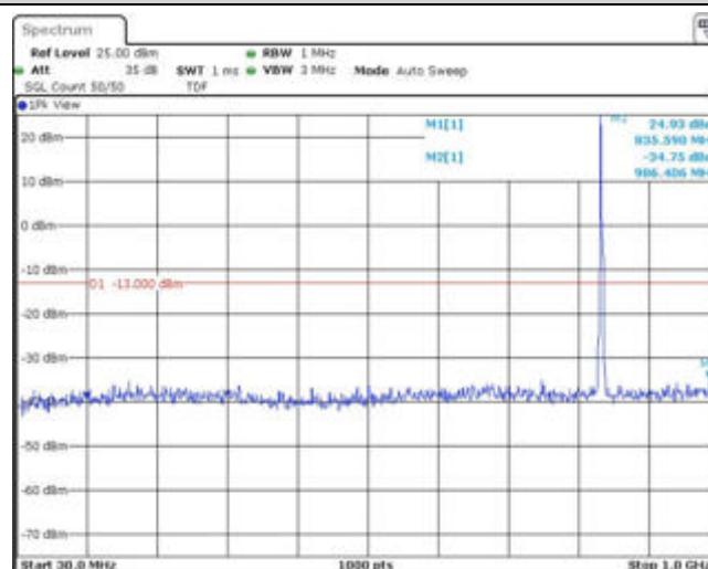
Band26-3MHz-QPSK-26915-1RB#0-Range1:30~1000MHz
