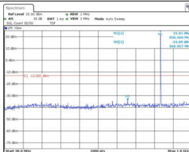
Band26-1.4MHz-QPSK-26915-1RB#0-Range1:30~1000MHz
