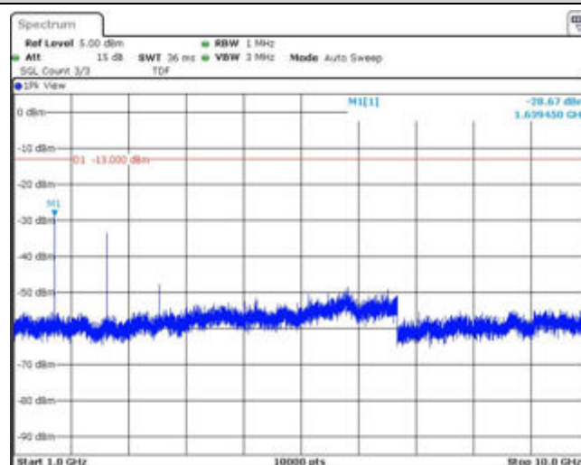
Band26-5MHz-16QAM-26765-1RB#0-Range2:1000~10000MHz
