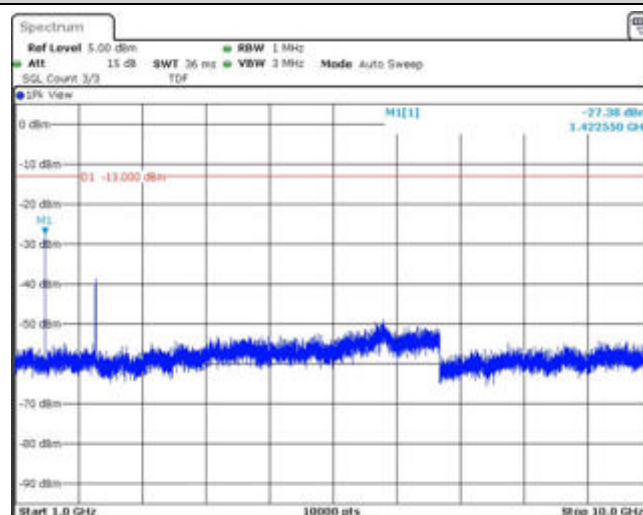
Band17-5MHz-QPSK-23825-1RB#0-Range2:1000~10000MHz
