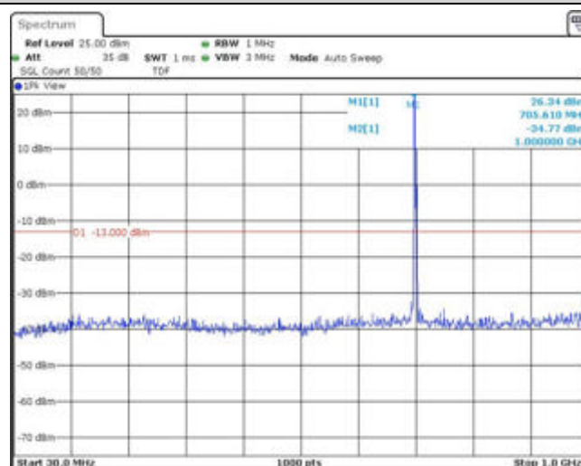
Band12-5MHz-16QAM-23095-1RB#0-Range1:30~1000MHz
