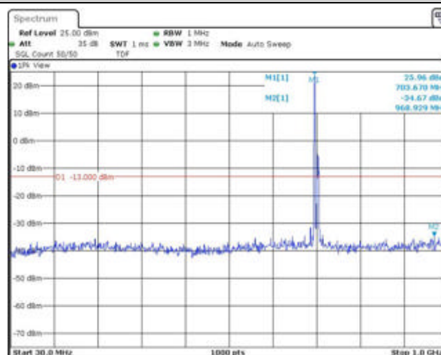
Band12-10MHz-QPSK-23095-1RB#0-Range1:30~1000MHz
