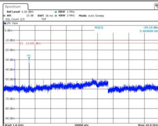
Band26-3MHz-16QAM-26775-1RB#0-Range2:1000~10000MHz
