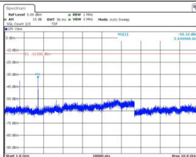
Band26-1.4MHz-16QAM-27033-1RB#0-Range2:1000~10000MHz
