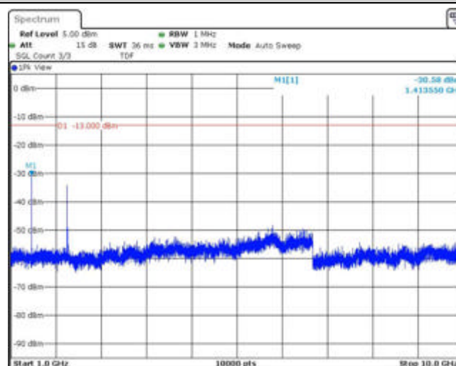
Band12-10MHz-QPSK-23130-1RB#0-Range2:1000~10000MHz
