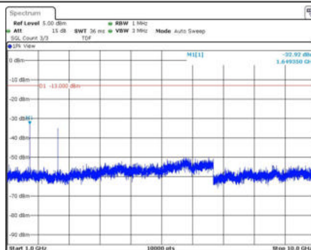
Band26-10MHz-16QAM-26840-1RB#0-Range2:1000~10000MHz
