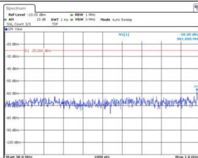
Band38-5MHz-16QAM-38000-1RB#0-Range1:30~1000MHz
