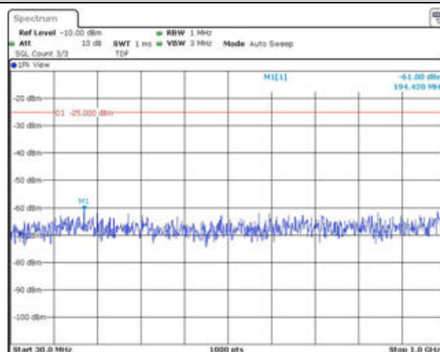
Band38-20MHz-16QAM-38150-1RB#0-Range1:30~1000MHz
