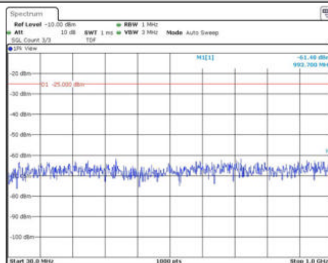
Band38-10MHz-QPSK-37800-1RB#0-Range1:30~1000MHz
