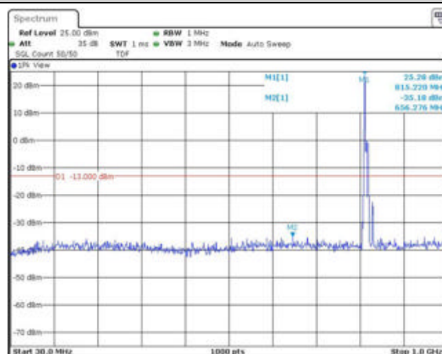
Band26-10MHz-16QAM-26740-1RB#0-Range1:30~1000MHz
