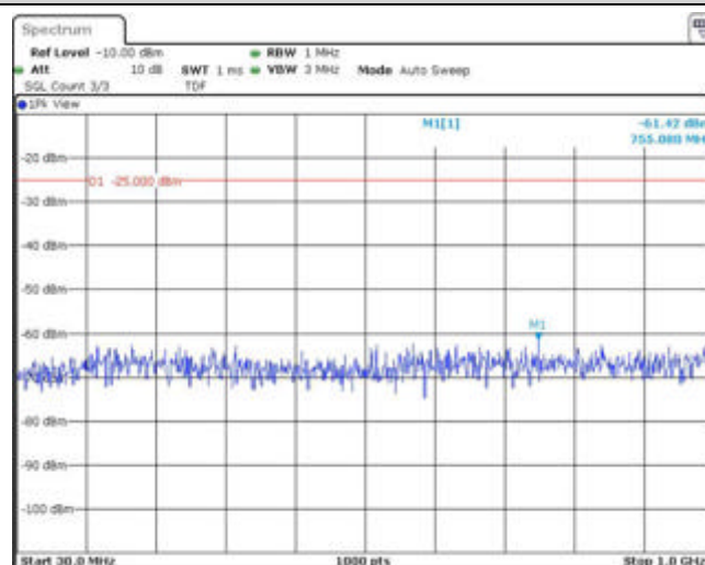
Band38-10MHz-16QAM-37800-1RB#0-Range1:30~1000MHz
