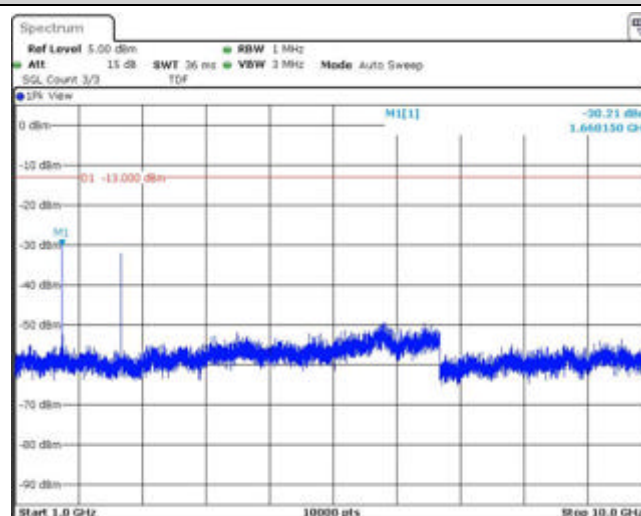
Band26-15MHz-QPSK-26915-1RB#0-Range2:1000~10000MHz
