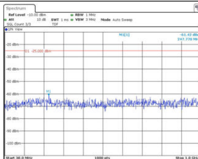
Band38-20MHz-QPSK-37850-1RB#0-Range1:30~1000MHz
