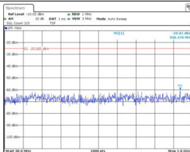
Band38-5MHz-16QAM-37775-1RB#0-Range1:30~1000MHz
