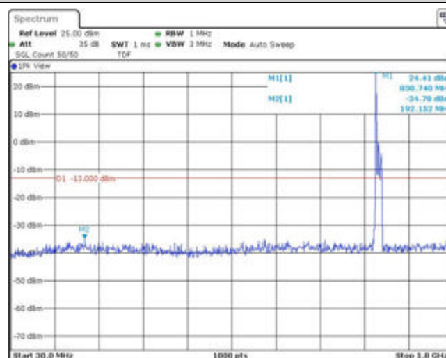
Band26-15MHz-QPSK-26915-1RB#0-Range1:30~1000MHz
