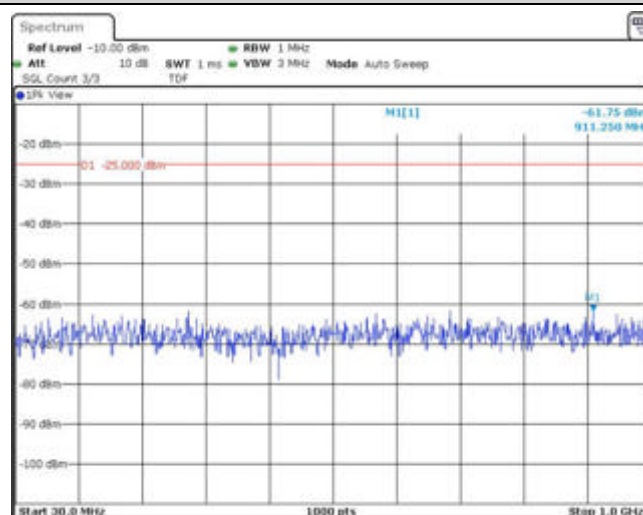
Band41-5MHz-QPSK-40690-1RB#0-Range1:30~1000MHz
