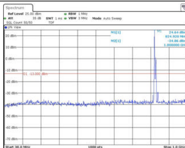
Band26-10MHz-QPSK-26840-1RB#0-Range1:30~1000MHz
