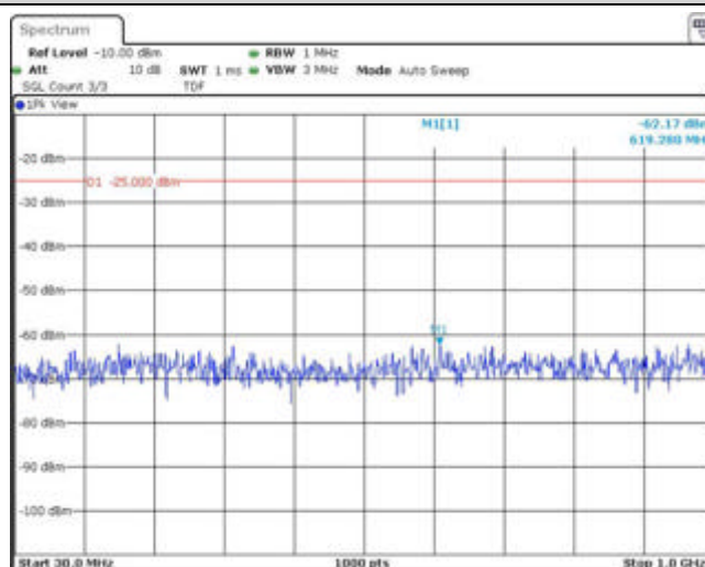
Band38-5MHz-16QAM-38225-1RB#0-Range1:30~1000MHz
