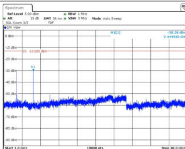
Band26-15MHz-QPSK-26765-1RB#0-Range2:1000~10000MHz
