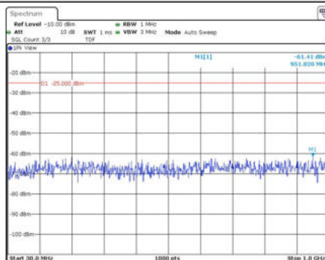
Band38-15MHz-16QAM-38175-1RB#0-Range1:30~1000MHz
