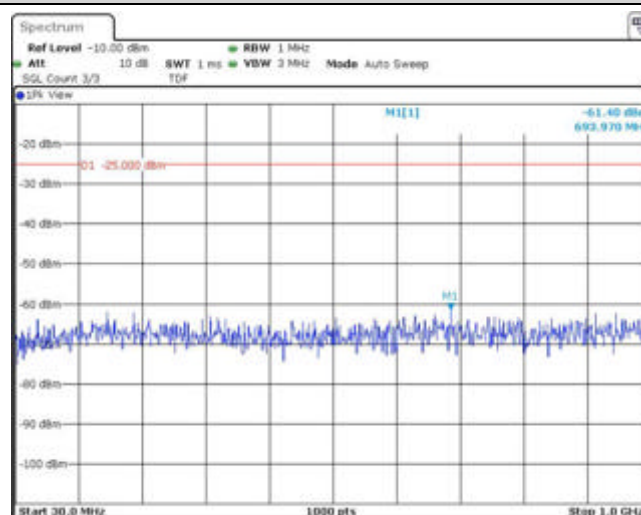
Band38-5MHz-QPSK-37775-1RB#0-Range1:30~1000MHz
