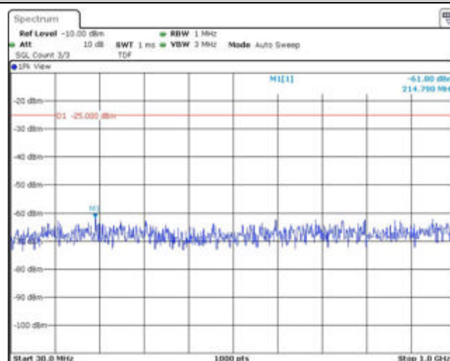
Band38-20MHz-QPSK-38000-1RB#0-Range1:30~1000MHz
