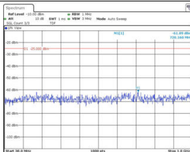
Band38-5MHz-QPSK-38225-1RB#0-Range1:30~1000MHz
