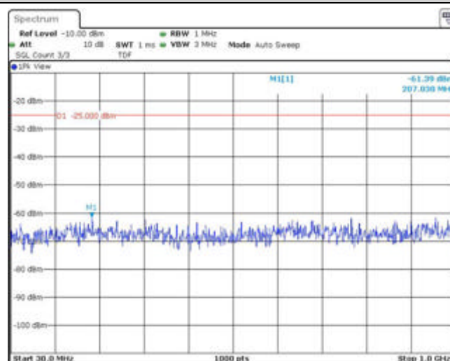
Band38-20MHz-QPSK-38150-1RB#0-Range1:30~1000MHz
