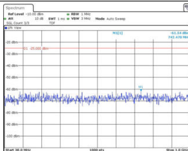
Band41-15MHz-QPSK-40690-1RB#0-Range1:30~1000MHz
