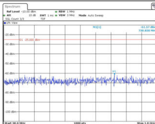
Band41-20MHz-QPSK-40690-1RB#0-Range1:30~1000MHz
