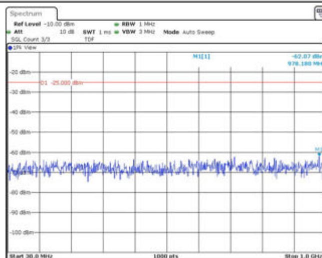
Band41-20MHz-QPSK-40340-1RB#0-Range1:30~1000MHz
