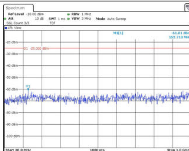
Band41-15MHz-16QAM-40590-1RB#0-Range1:30~1000MHz
