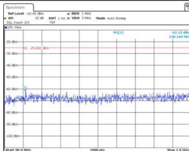
Band41-5MHz-16QAM-40065-1RB#0-Range1:30~1000MHz
