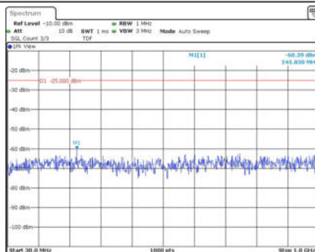
Band41-10MHz-16QAM-40590-1RB#0-Range1:30~1000MHz
