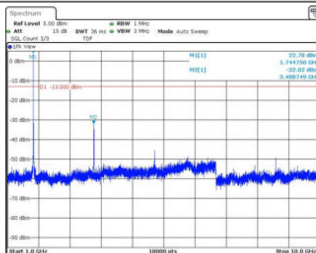
Band66-1.4MHz-QPSK-132322-1RB#0-Range2:1000~10000MHz
