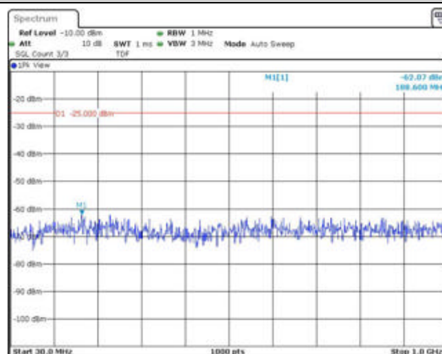
Band41-20MHz-16QAM-41140-1RB#0-Range2:1000~3000MHz
