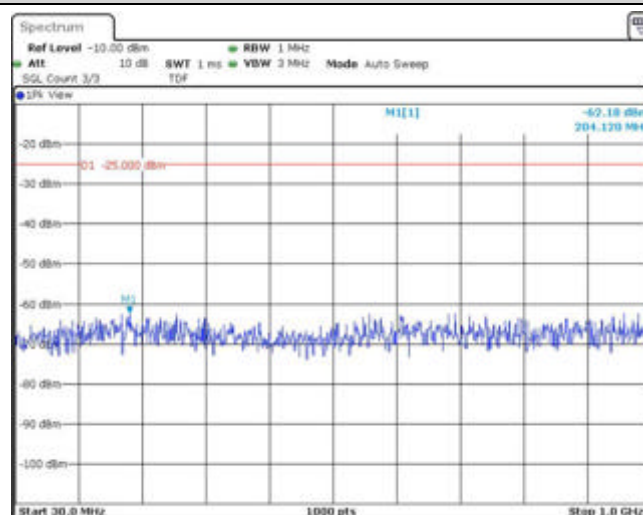
Band41-5MHz-16QAM-40590-1RB#0-Range1:30~1000MHz
