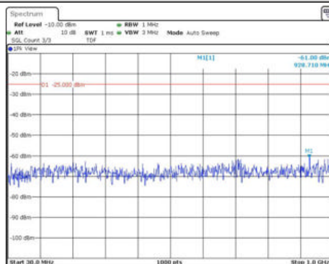
Band41-10MHz-QPSK-40090-1RB#0-Range1:30~1000MHz
