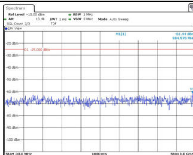
Band41-5MHz-16QAM-40690-1RB#0-Range1:30~1000MHz
