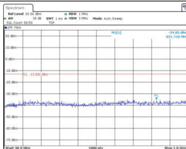
Band66-1.4MHz-16QAM-131979-1RB#0-Range1:30~1000MHz
