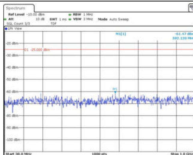
Band41-10MHz-QPSK-40590-1RB#0-Range1:30~1000MHz
