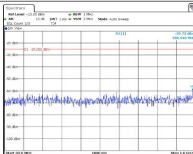
Band41-10MHz-16QAM-40690-1RB#0-Range1:30~1000MHz
