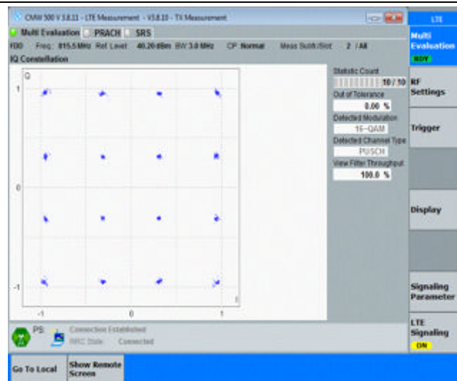
Band26-3MHz-16QAM-26740-15RB#0
