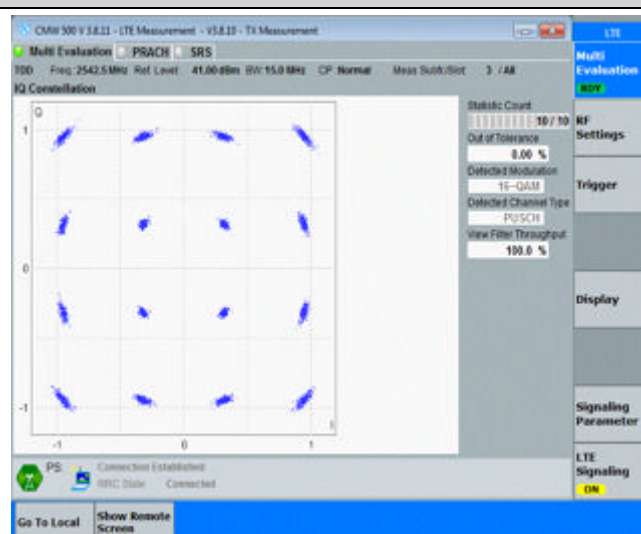
Band41-15MHz-16QAM-40315-75RB#0
