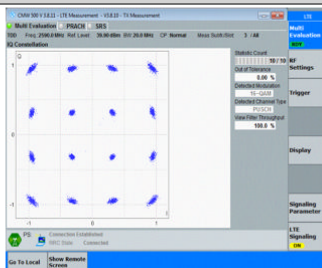
Band41-20MHz-16QAM-40690-100RB#0
