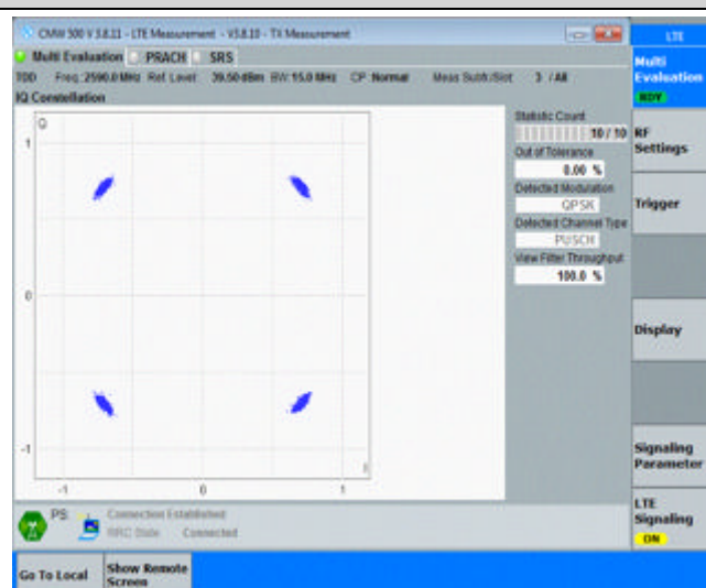
Band41-15MHz-QPSK-40690-75RB#0
