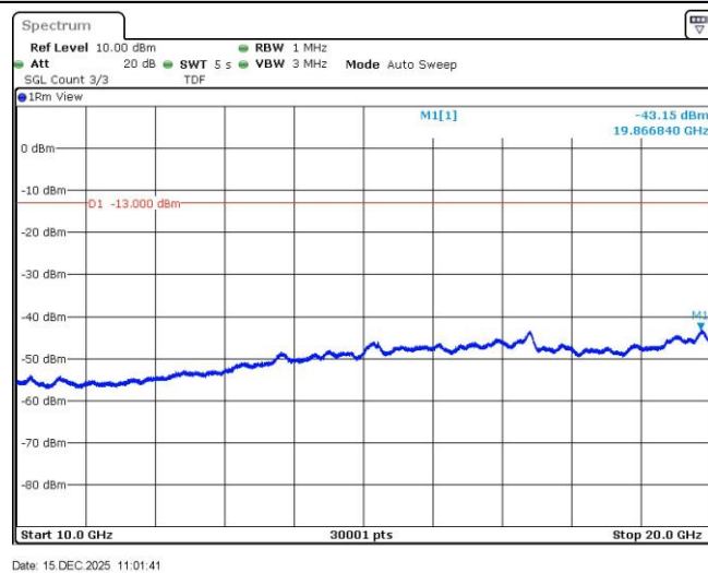
Band2-9400-3-10000~20000MHz
