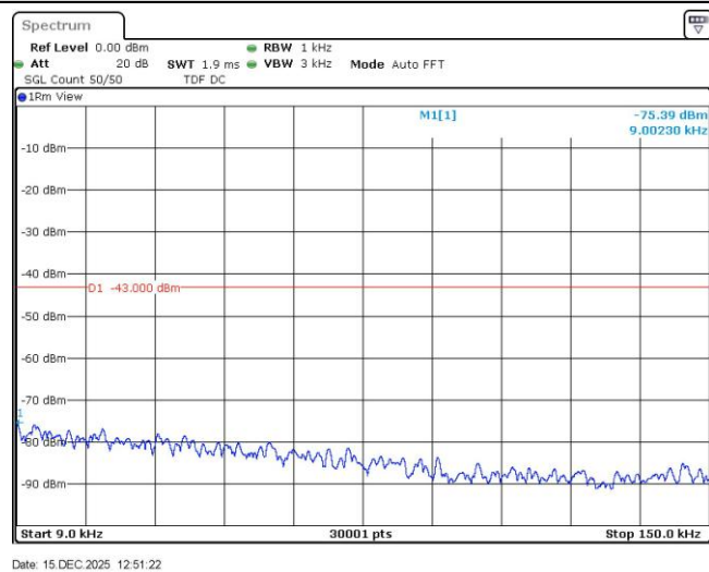
Band4-1413-3-0.009~0.15MHz
