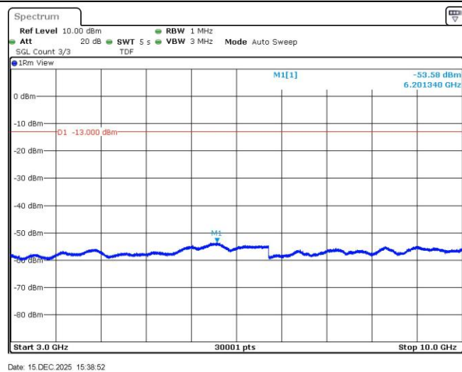
Band5-4132-4-3000~10000MHz
