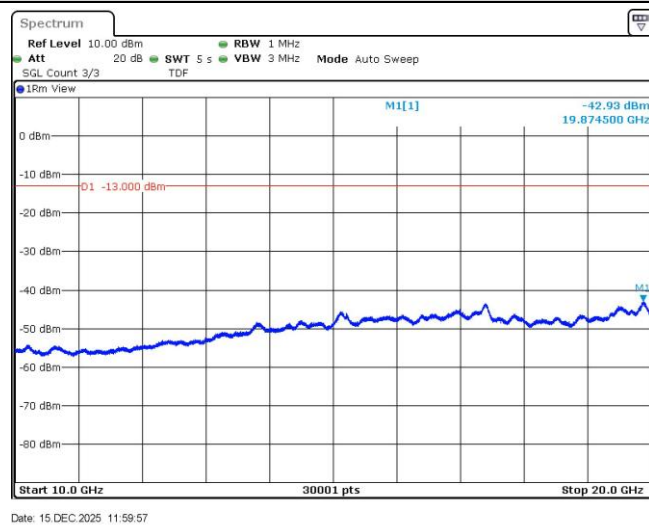
Band2-9538-5-10000~20000MHz
