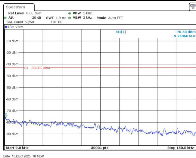
Band5-4132-2-0.009~0.15MHz
