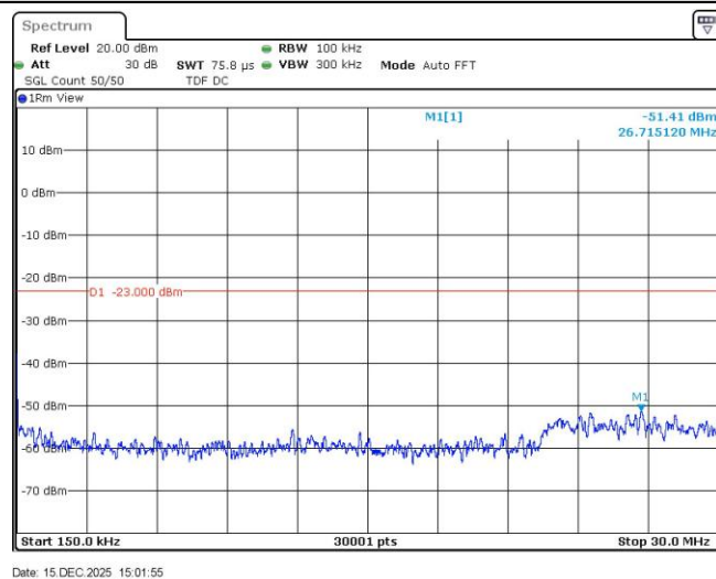
Band5-4132-1-0.15~30MHz
