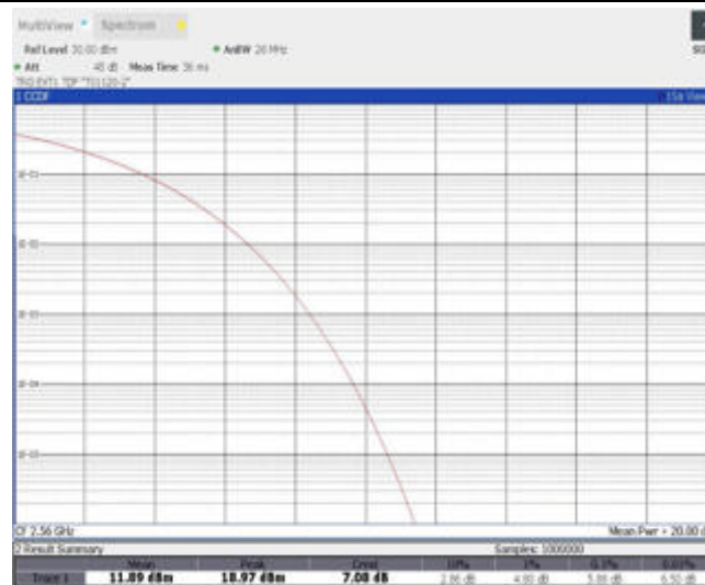
Band41-10MHz-16QAM-40590-1RB#0
