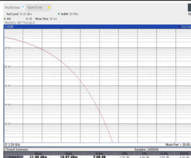
Band41-10MHz-QPSK-40690-1RB#0
