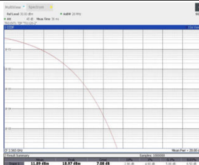
Band41-20MHz-16QAM-40340-100RB#0
