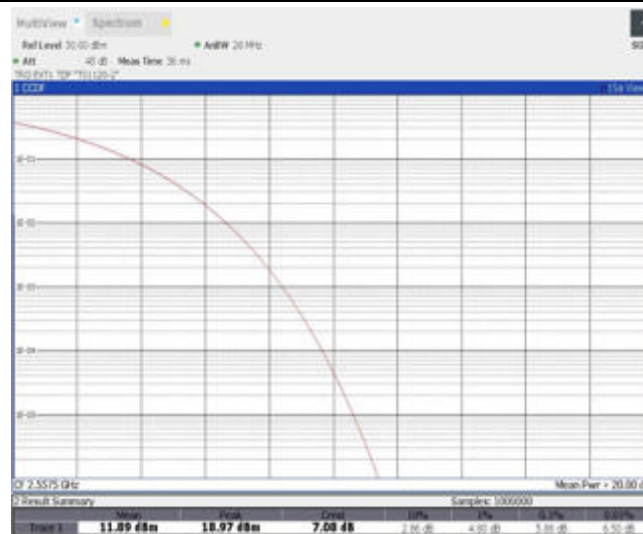
Band41-5MHz-16QAM-40265-25RB#0
