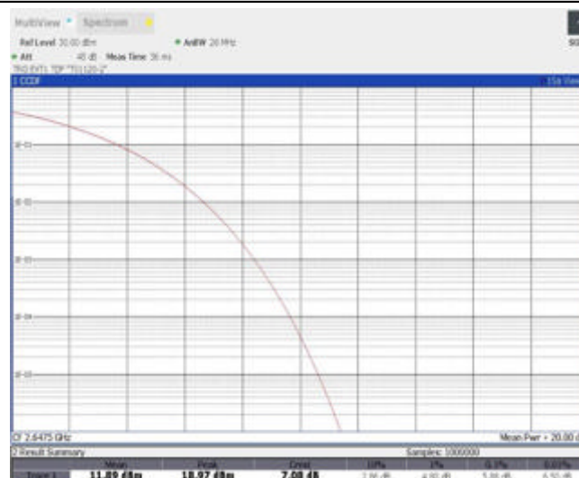
Band41-15MHz-16QAM-40115-1RB#0
