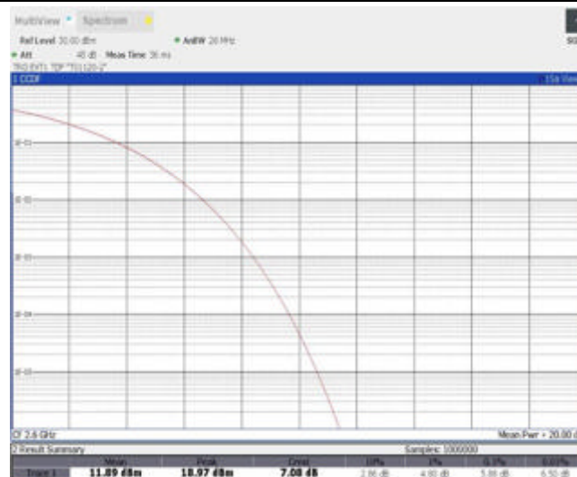
Band41-5MHz-QPSK-40690-25RB#0
