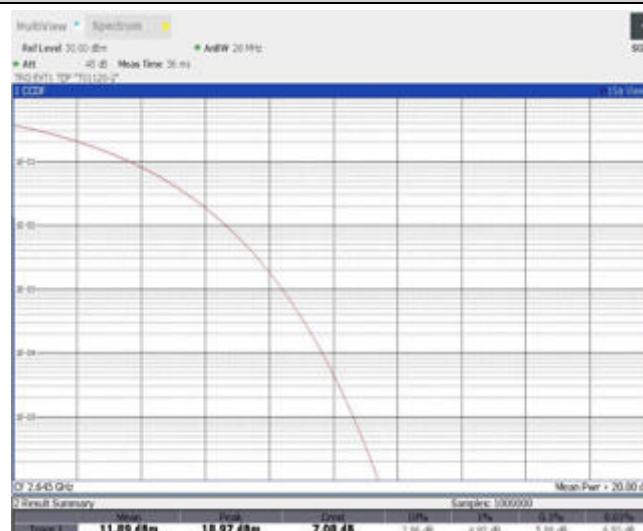
Band41-20MHz-QPSK-41140-100RB#0
