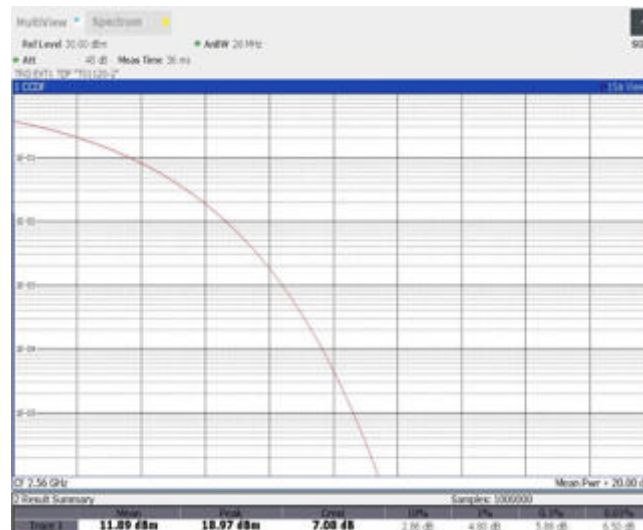
Band41-10MHz-QPSK-40290-50RB#0
