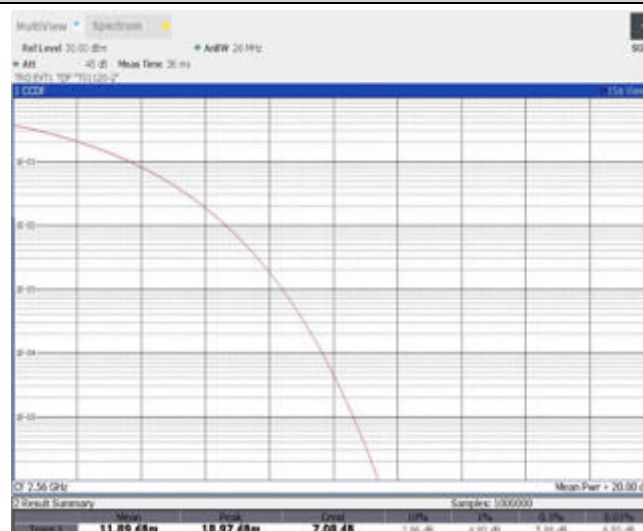
Band41-10MHz-QPSK-40590-1RB#0
