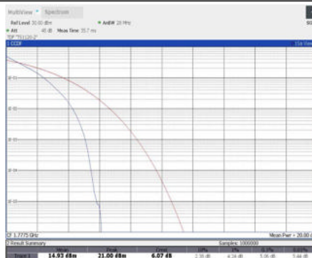
Band66-5MHz-16QAM-131997-1RB#0
