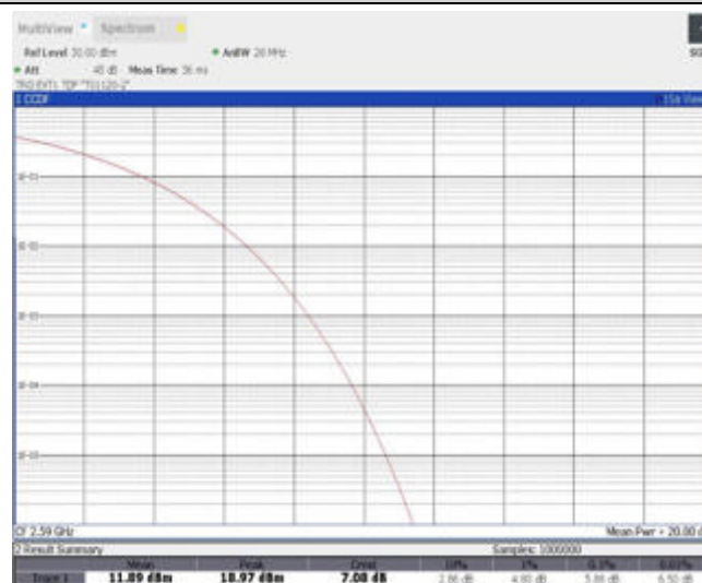
Band41-10MHz-16QAM-40690-1RB#0
