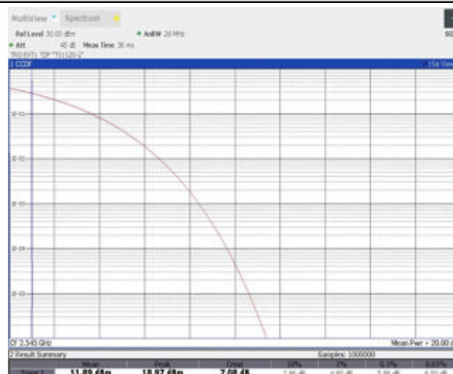
Band41-20MHz-16QAM-40340-1RB#0
