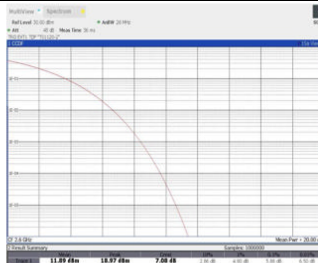
Band41-10MHz-QPSK-41190-1RB#0
