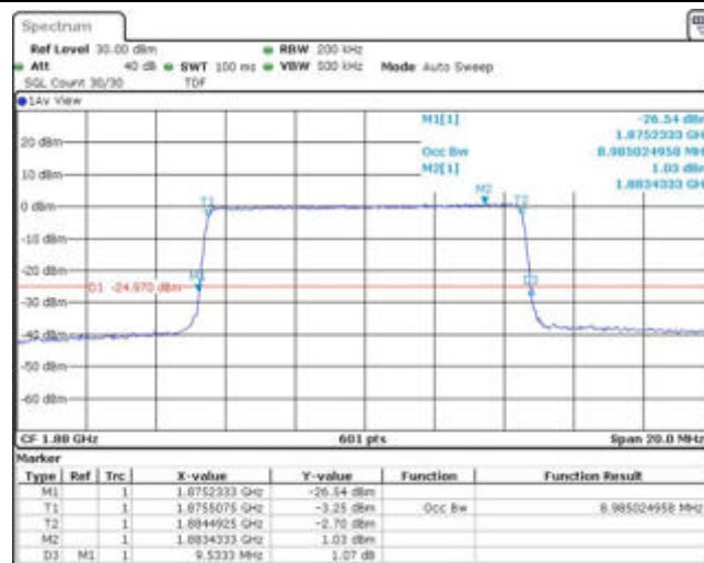
Band2-10MHz-16QAM-19150-50RB#0
