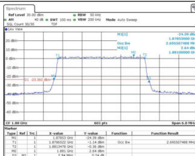
Band2-3MHz-16QAM-19185-15RB#0
