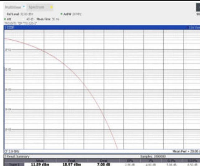
Band41-20MHz-QPSK-40690-100RB#0
