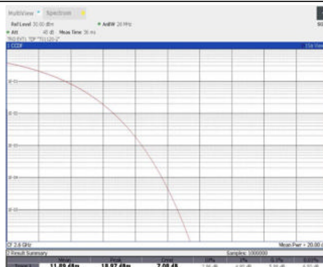
Band41-20MHz-16QAM-41140-1RB#0
