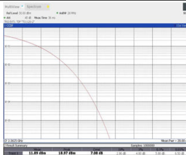
Band41-15MHz-QPSK-40315-75RB#0
