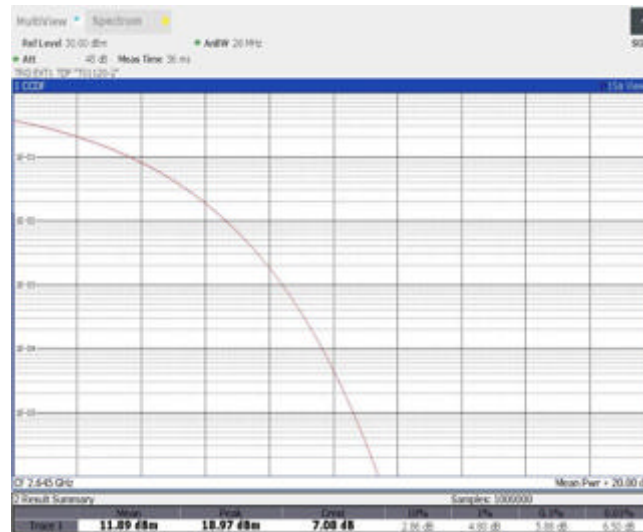
Band41-20MHz-16QAM-40140-1RB#0
