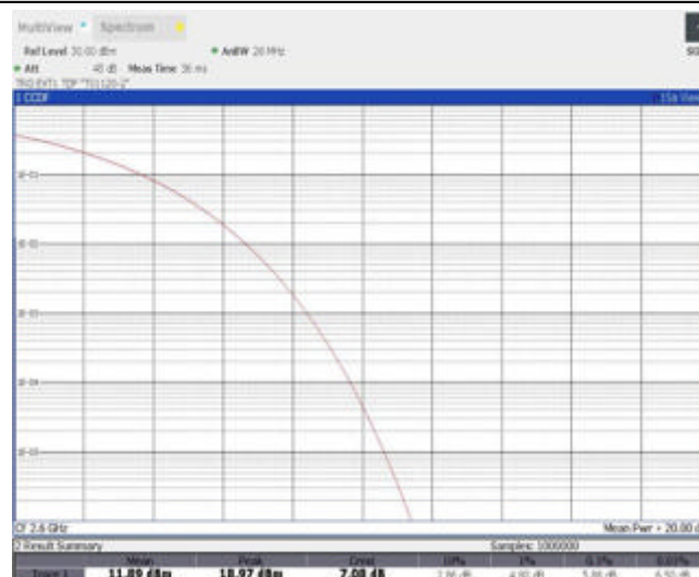
Band41-15MHz-QPSK-40690-75RB#0
