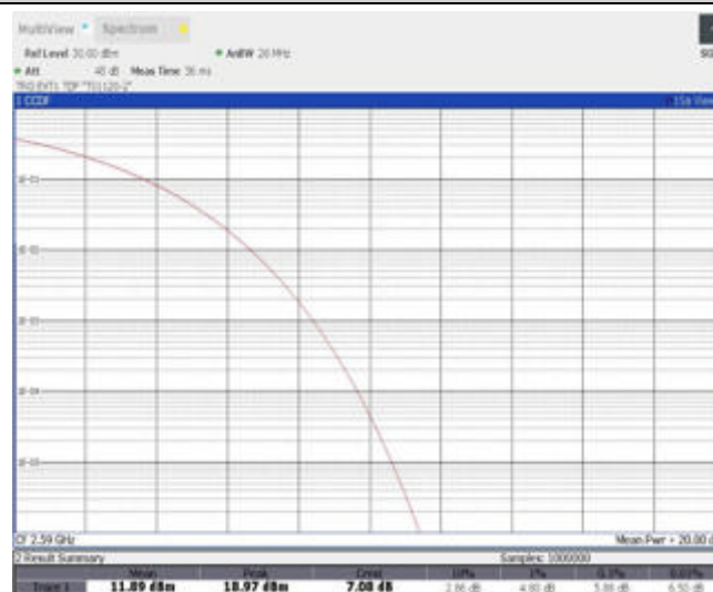
Band41-5MHz-16QAM-40590-25RB#0
