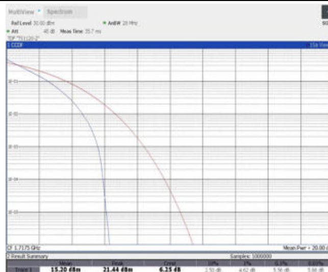
Band66-15MHz-QPSK-132322-1RB#0
