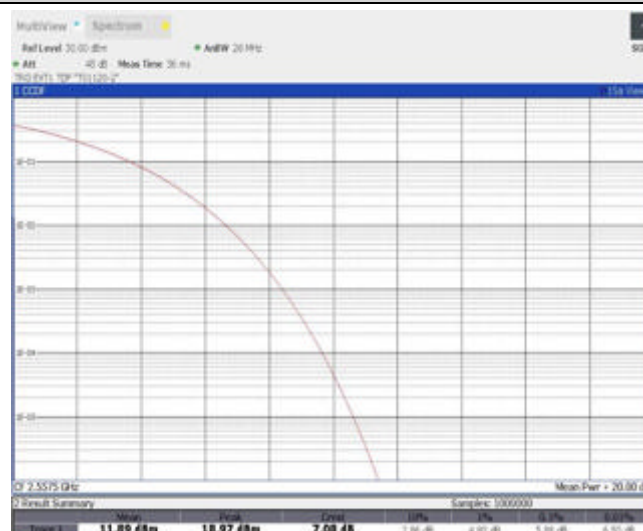
Band41-5MHz-QPSK-40265-25RB#0
