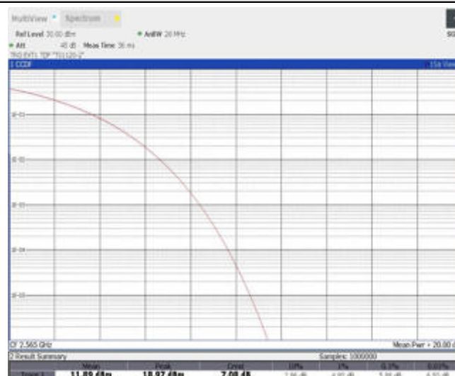
Band41-20MHz-QPSK-40340-100RB#0
