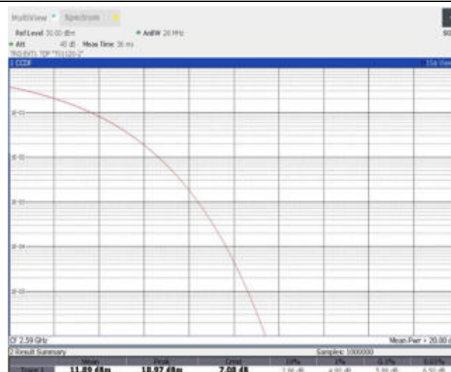
Band41-5MHz-QPSK-40590-25RB#0
