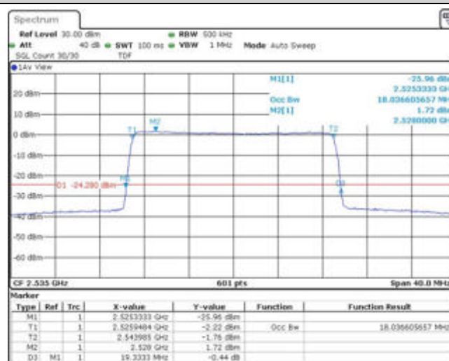
Band7-20MHz-16QAM-21350-100RB#0
