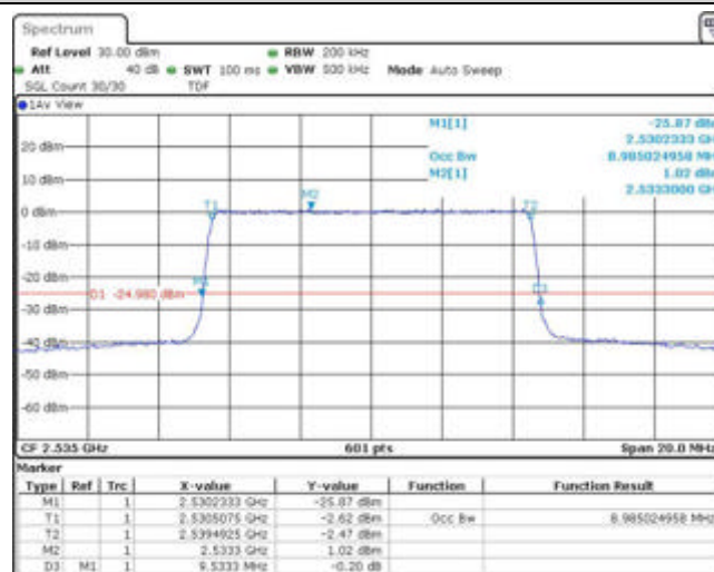
Band7-10MHz-16QAM-21400-50RB#0
