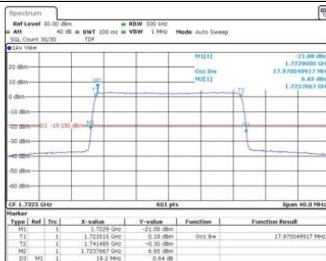
Band4-20MHz-16QAM-20300-100RB#0
