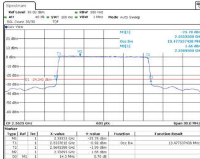
Band7-15MHz-16QAM-20825-75RB#0
