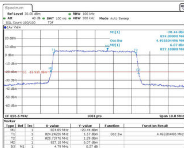
Band5-5MHz-QPSK-20525-25RB#0
