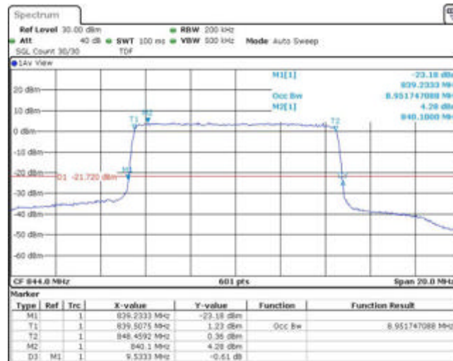
Band5-10MHz-16QAM-20450-50RB#0
