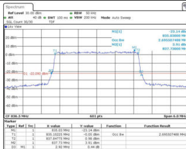
Band5-3MHz-16QAM-20635-15RB#0
