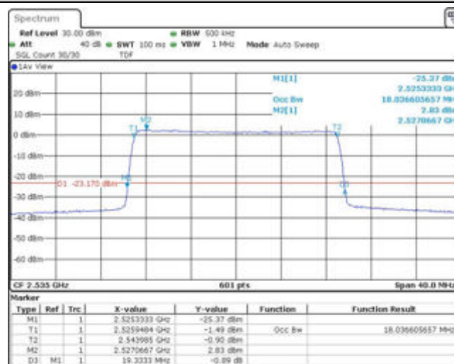
Band7-20MHz-QPSK-21350-100RB#0
