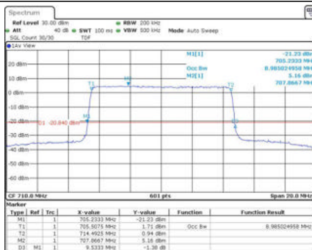
Band17-10MHz-16QAM-23800-50RB#0
