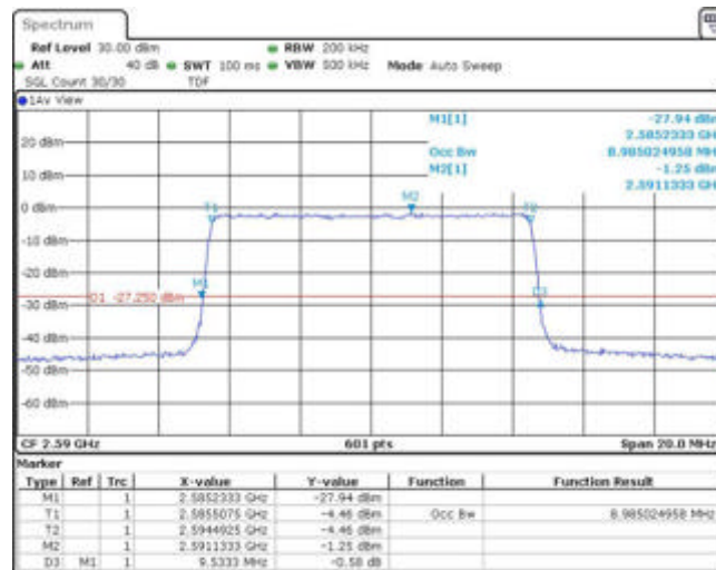
Band41-10MHz-16QAM-40690-50RB#0
