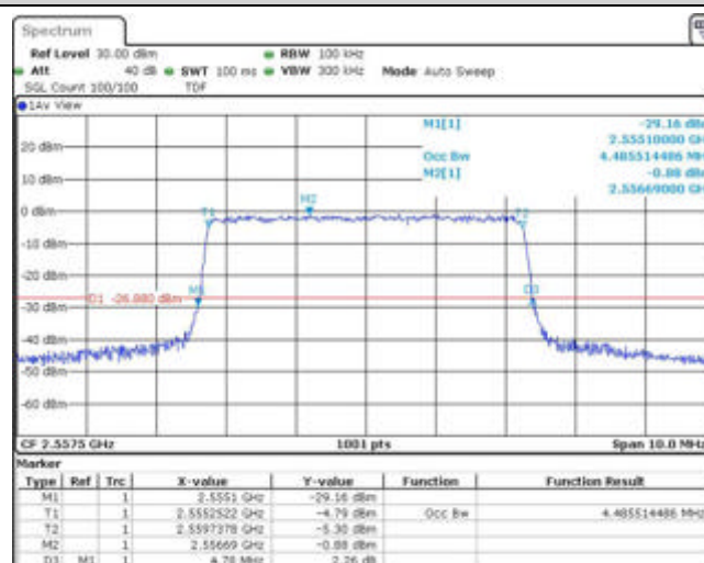
Band41-5MHz-16QAM-40590-25RB#0
