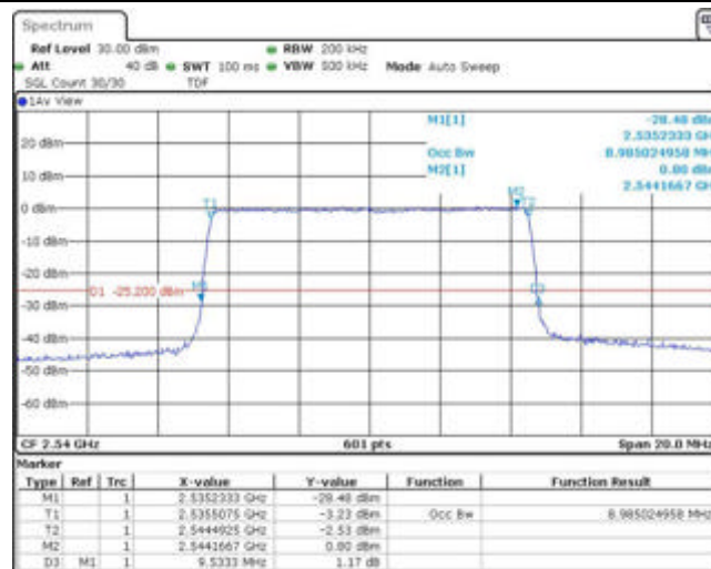
Band41-10MHz-QPSK-40290-50RB#0
