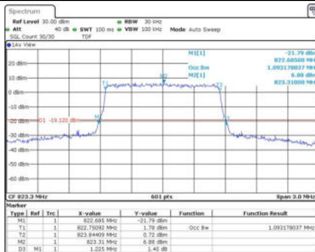
Band26-1.4MHz-16QAM-26797-6RB#0
