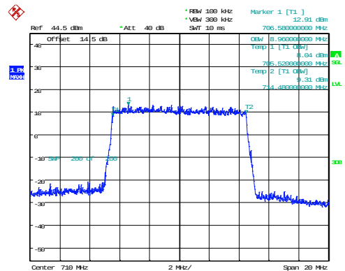
Occupied Bandwidth
