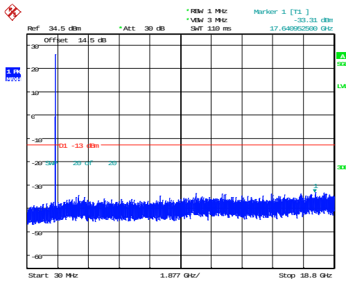
1.4MHz_Middle_QPSK_1@0(30MHz~18.8GHz)
