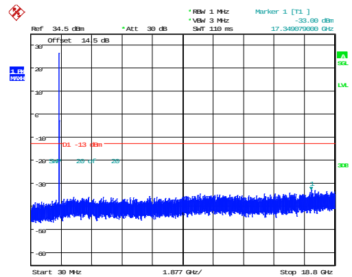
10MHz_High_QPSK_1@0(30MHz~18.8GHz)
