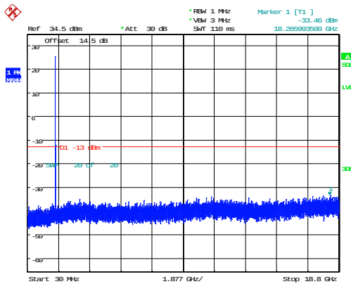
3MHz_Low_QPSK_1@0(30MHz~18.8GHz)
