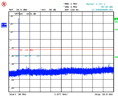
1.4MHz_High_QPSK_1@0(30MHz~18.8GHz)
