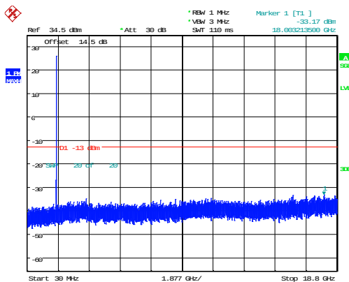
3MHz_High_QPSK_1@0(30MHz~18.8GHz)
