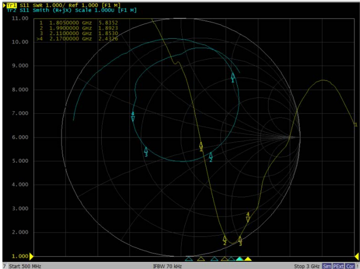
Three-in-one antenna
