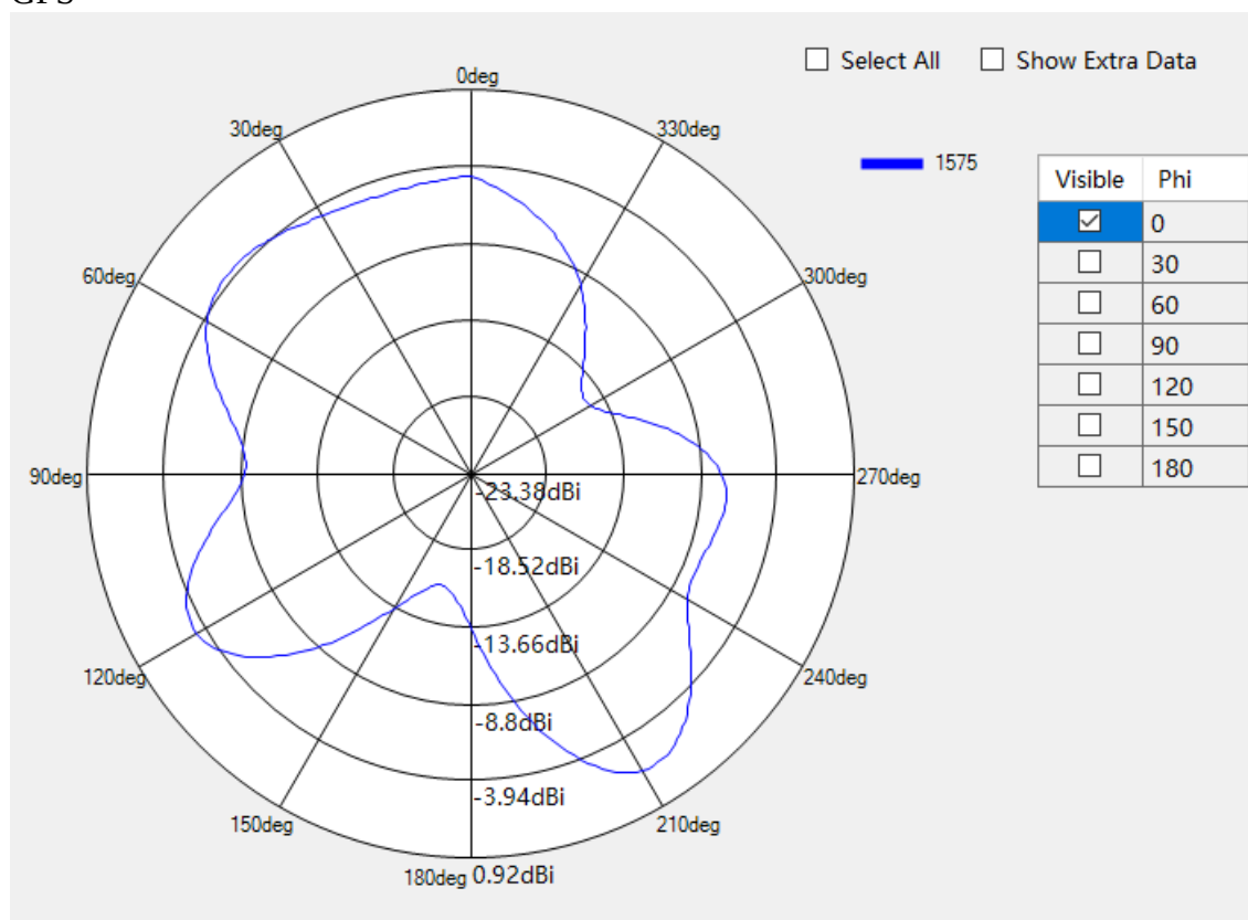
Three-in-one antenna GPS
