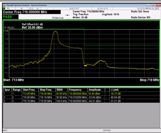
Band12-1.4MHz-64QAM-23173-6RB#0
