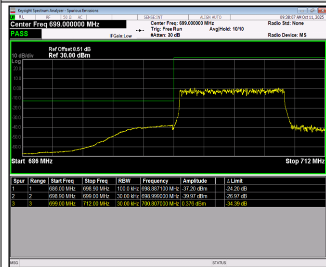
Band12-10MHz-64QAM-23130-1RB#49
