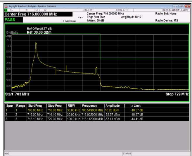
Band12-10MHz-16QAM-23130-50RB#0
