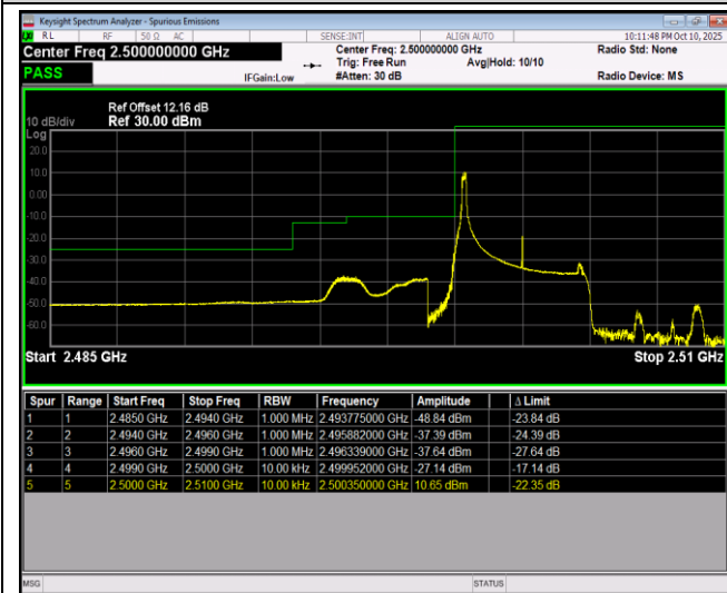
Band7-5MHz-16QAM-20775-25RB#0
