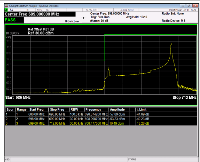
Band12-10MHz-64QAM-23130-1RB#0
