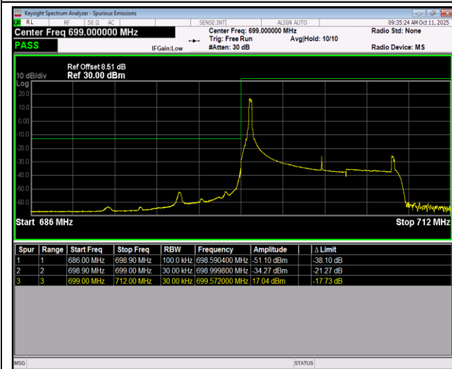
Band12-10MHz-64QAM-23060-50RB#0
