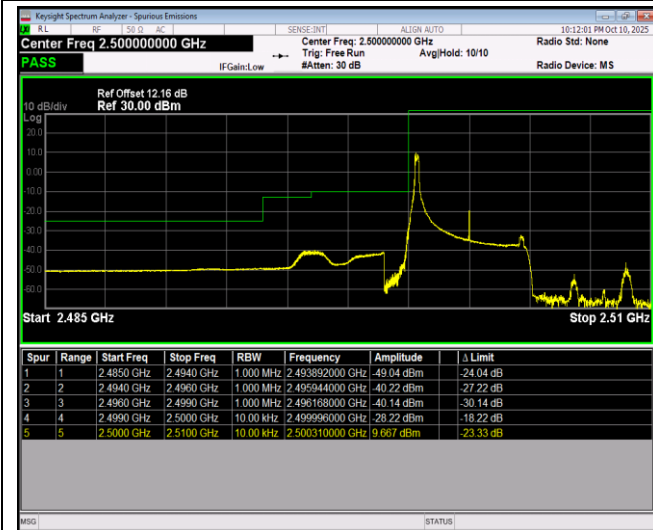
Band7-5MHz-64QAM-20775-25RB#0
