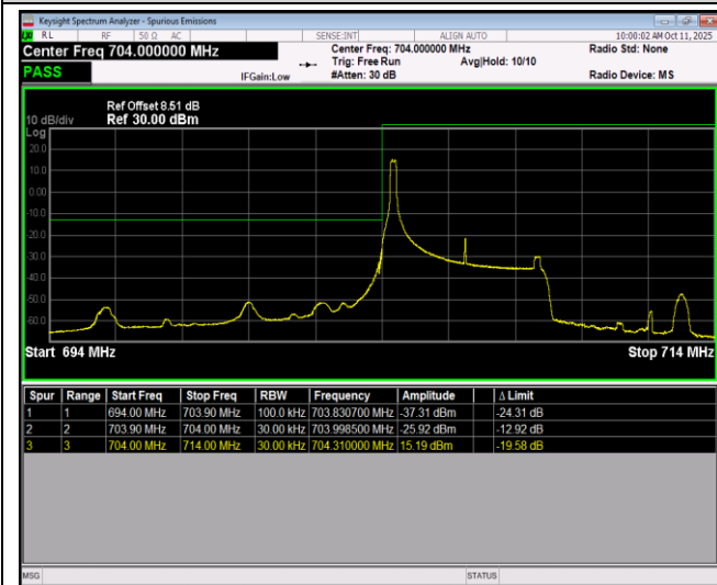
Band17-5MHz-QPSK-23755-25RB#0
