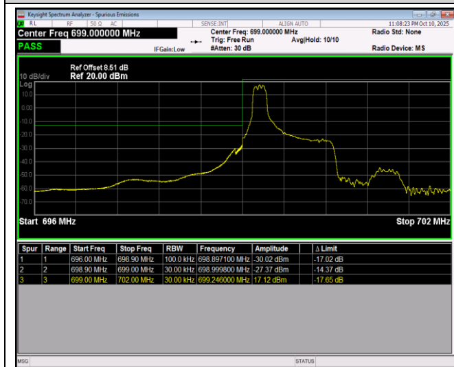
Band12-1.4MHz-64QAM-23017-6RB#0
