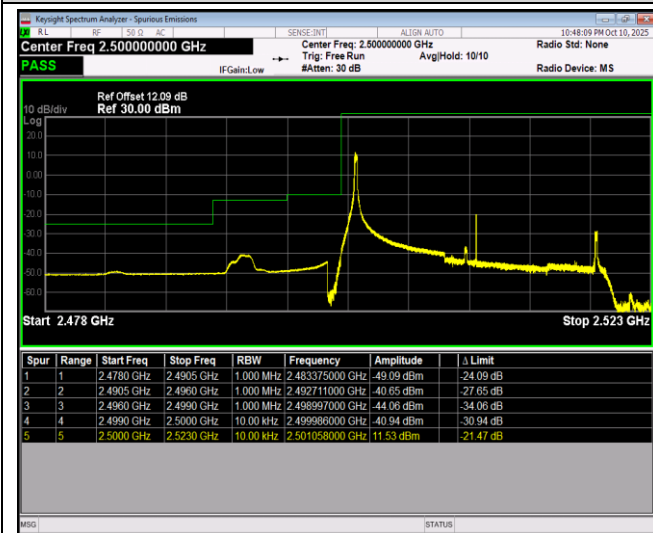
Band7-20MHz-64QAM-20850-100RB#0
