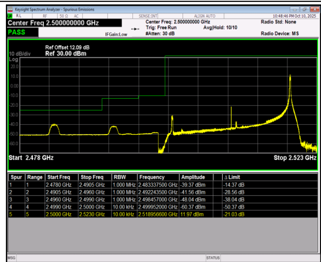
Band7-20MHz-64QAM-21350-1RB#0
