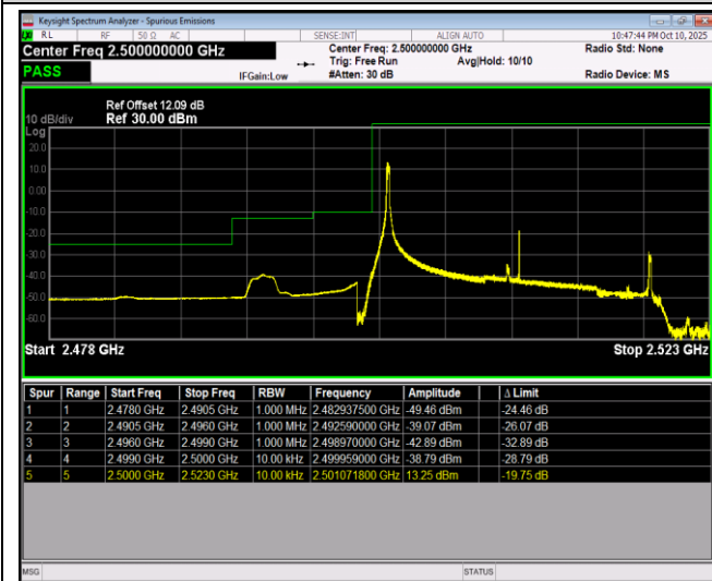
Band7-20MHz-QPSK-20850-100RB#0
