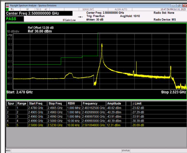
Band7-20MHz-16QAM-20850-100RB#0
