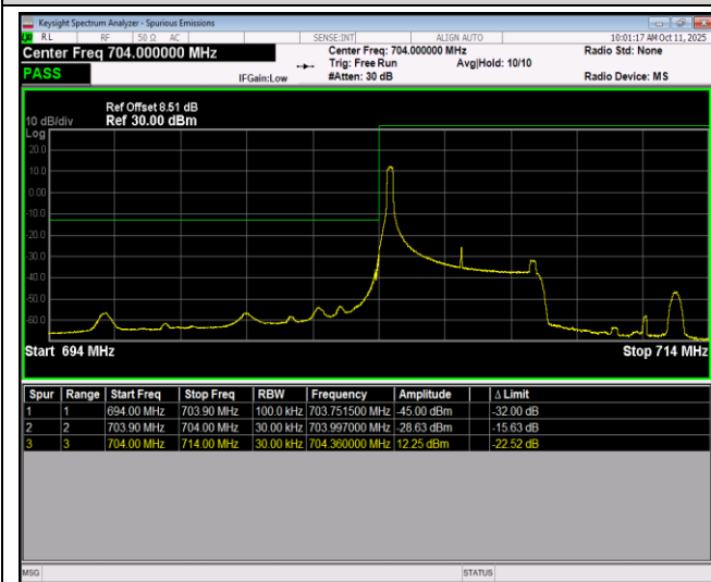
Band17-5MHz-64QAM-23755-25RB#0
