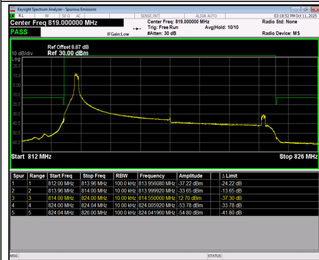
Band26-10MHz-QPSK-26740-50RB#0
