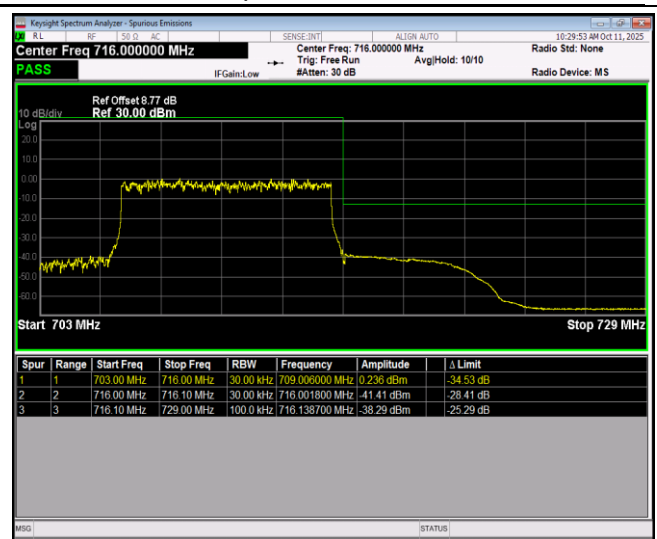
Band17-10MHz-64QAM-23780-1RB#49
