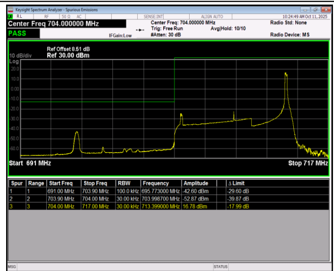
Band17-10MHz-64QAM-23800-1RB#0
