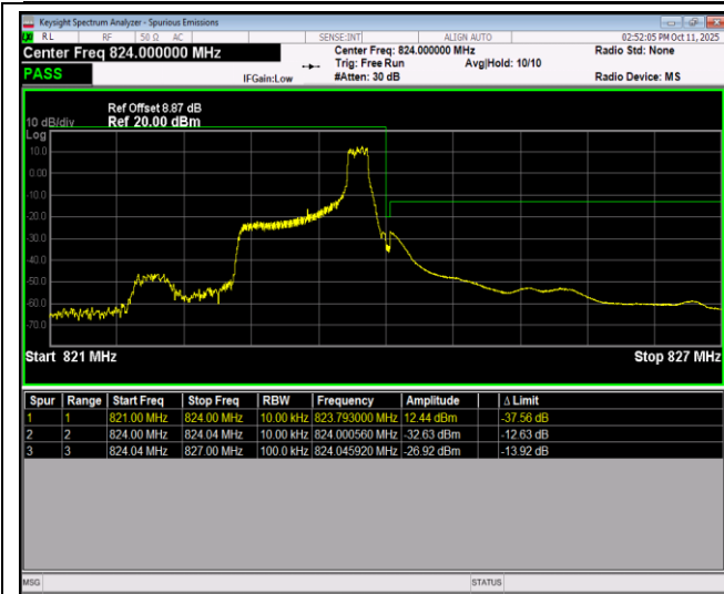
Band26-1.4MHz-64QAM-26797-1RB#0
