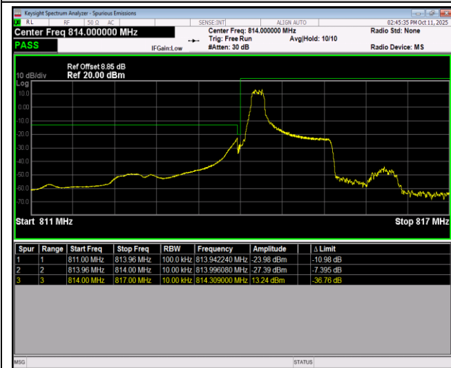
Band26-1.4MHz-QPSK-26697-6RB#0
