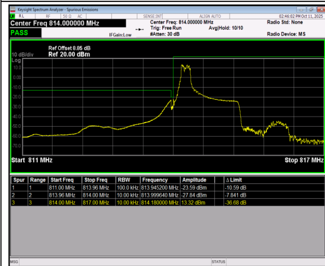
Band26-1.4MHz-16QAM-26697-6RB#0
