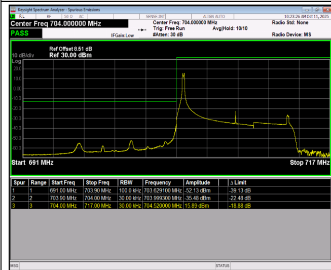
Band17-10MHz-64QAM-23780-50RB#0
