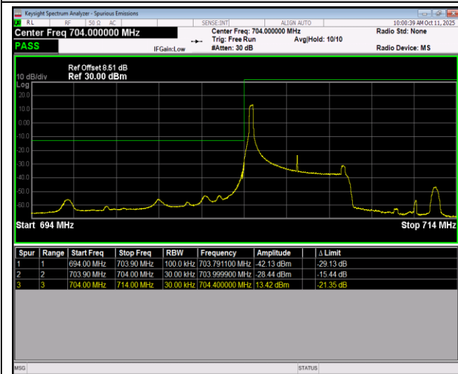
Band17-5MHz-16QAM-23755-25RB#0
