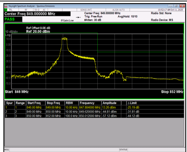
Band26-1.4MHz-16QAM-27033-6RB#0
