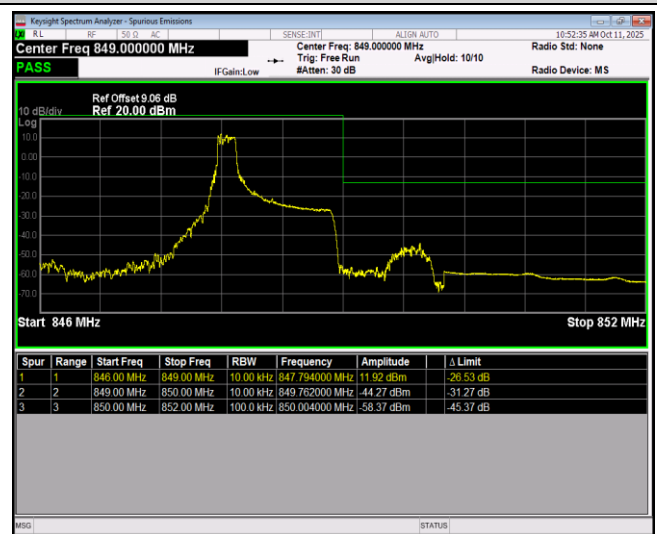
Band26-1.4MHz-64QAM-27033-6RB#0
