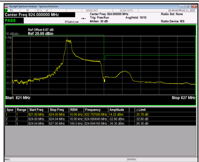
Band26-1.4MHz-QPSK-26783-6RB#0
