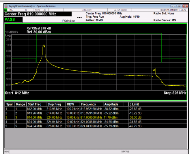
Band26-10MHz-16QAM-26740-50RB#0
