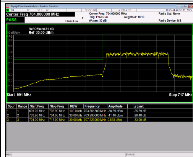
Band17-10MHz-16QAM-23800-1RB#49
