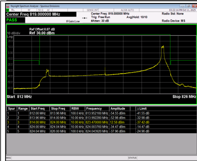
Band26-10MHz-64QAM-26740-1RB#0
