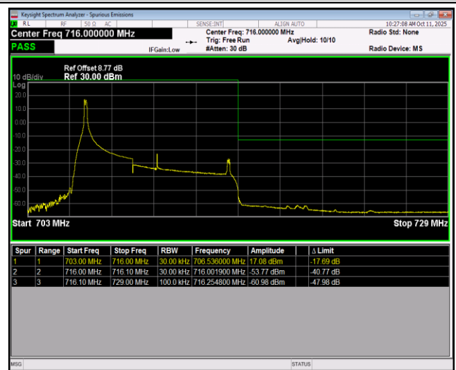
Band17-10MHz-16QAM-23800-50RB#0
