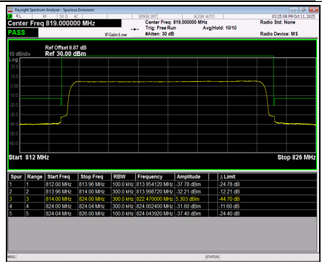
Band26-10MHz-64QAM-26740-1RB#49
