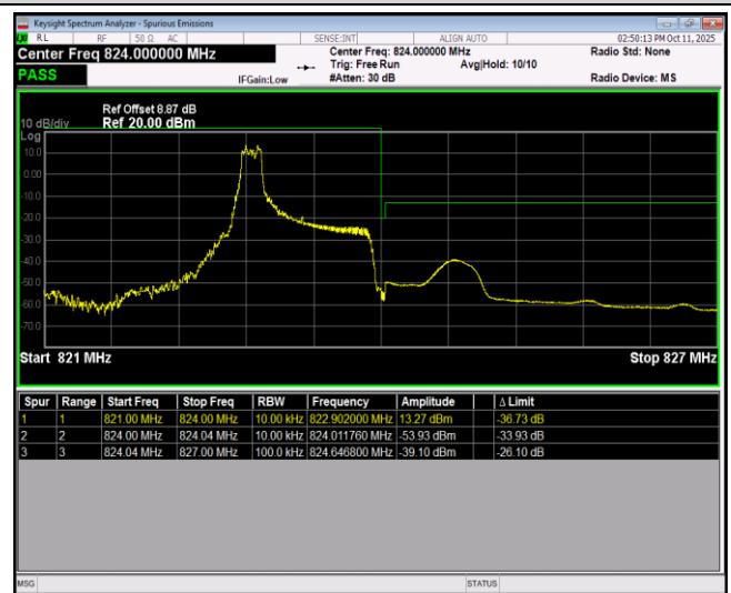
Band26-1.4MHz-16QAM-26783-6RB#0
