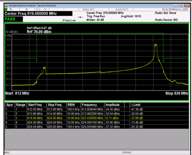
Band26-10MHz-16QAM-26740-1RB#0
