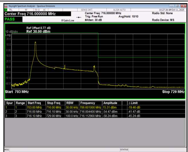
Band17-10MHz-64QAM-23800-50RB#0
