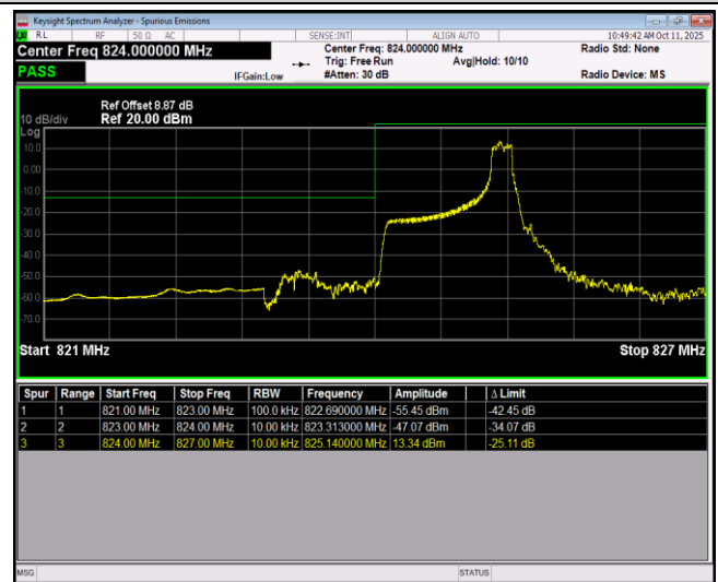
Band26-1.4MHz-QPSK-27033-1RB#0
