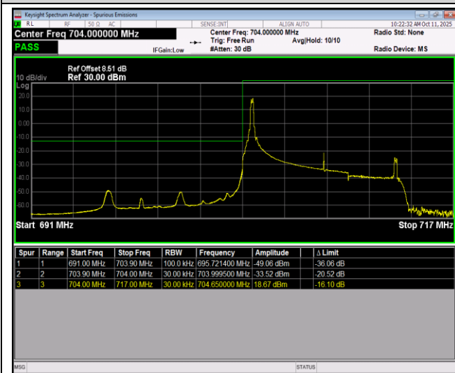
Band17-10MHz-QPSK-23780-50RB#0
