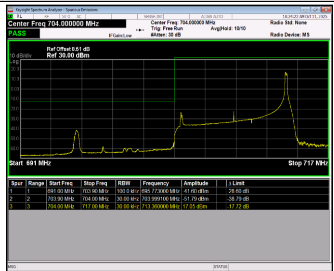
Band17-10MHz-16QAM-23800-1RB#0
