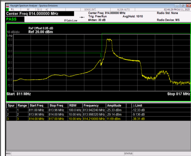
Band26-1.4MHz-64QAM-26697-6RB#0
