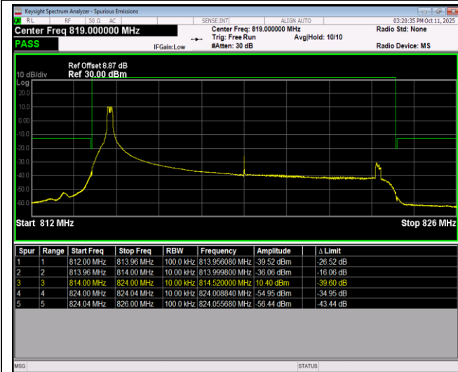
Band26-10MHz-64QAM-26740-50RB#0
