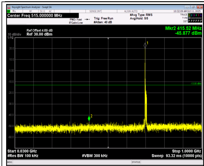
Band17-10MHz-64QAM-23800-1RB#0-Range1:30~1000MHz
