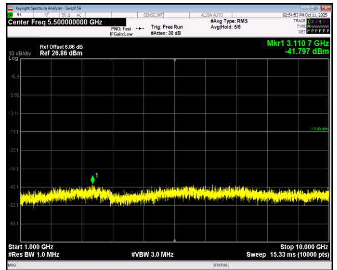
Band26-1.4MHz-QPSK-26783-1RB#0-Range2:1000~10000MHz
