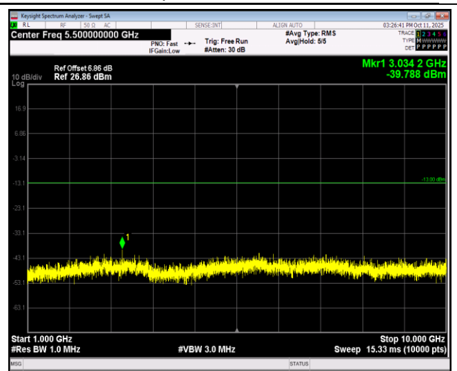
Band26-10MHz-16QAM-26740-1RB#0-Range2:1000~10000MHz
