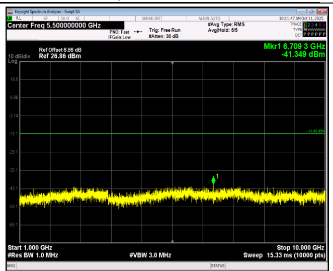
Band17-5MHz-64QAM-23790-1RB#0-Range2:1000~10000MHz
