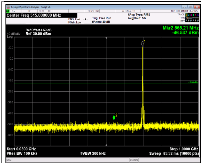
Band17-5MHz-64QAM-23790-1RB#0-Range1:30~1000MHz
