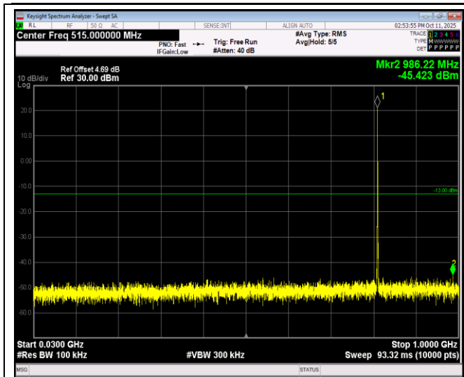
Band26-1.4MHz-QPSK-26740-1RB#0-Range1:30~1000MHz
