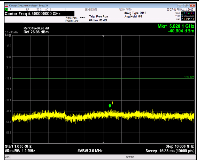
Band26-10MHz-64QAM-26740-1RB#0-Range2:1000~10000MHz
