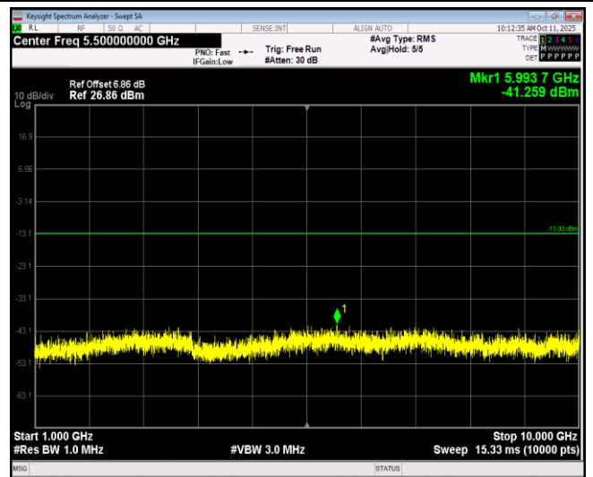
Band17-5MHz-64QAM-23825-1RB#0-Range2:1000~10000MHz
