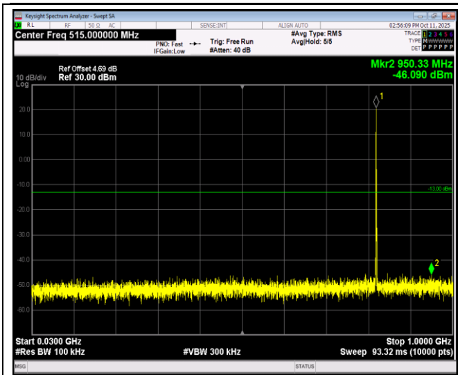
Band26-1.4MHz-64QAM-26797-1RB#0-Range1:30~1000MHz
