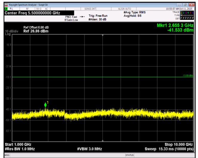
Band26-1.4MHz-64QAM-26915-1RB#0-Range2:1000~10000MHz
