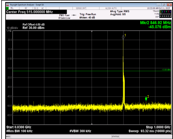
Band26-1.4MHz-QPSK-26697-1RB#0-Range1:30~1000MHz
