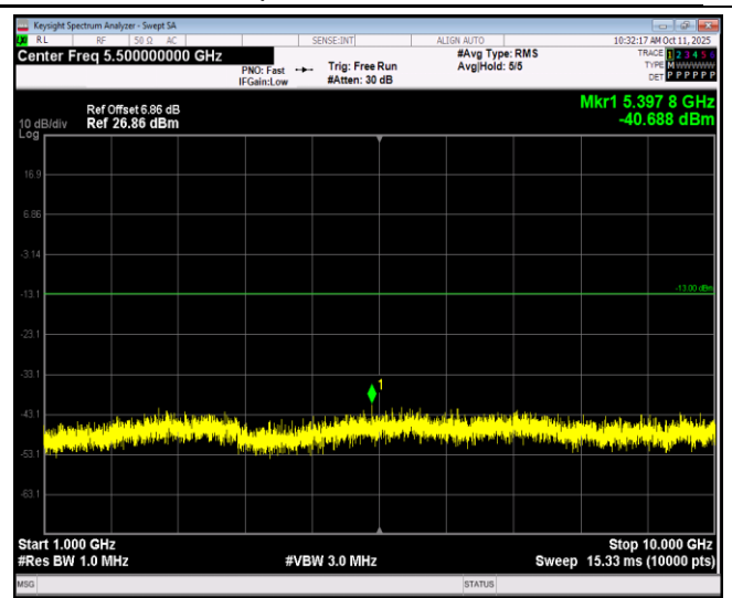
Band17-10MHz-64QAM-23800-1RB#0-Range2:1000~10000MHz
