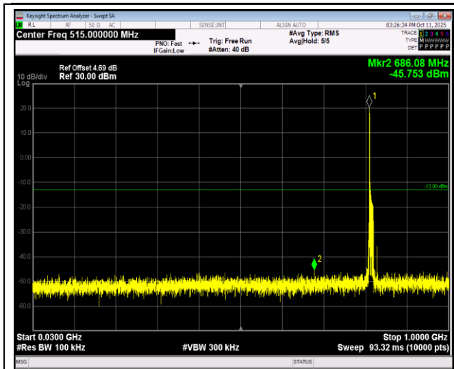
Band26-10MHz-16QAM-26740-1RB#0-Range1:30~1000MHz
