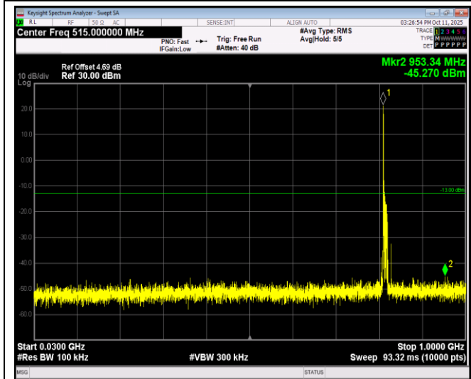
Band26-10MHz-64QAM-26740-1RB#0-Range1:30~1000MHz
