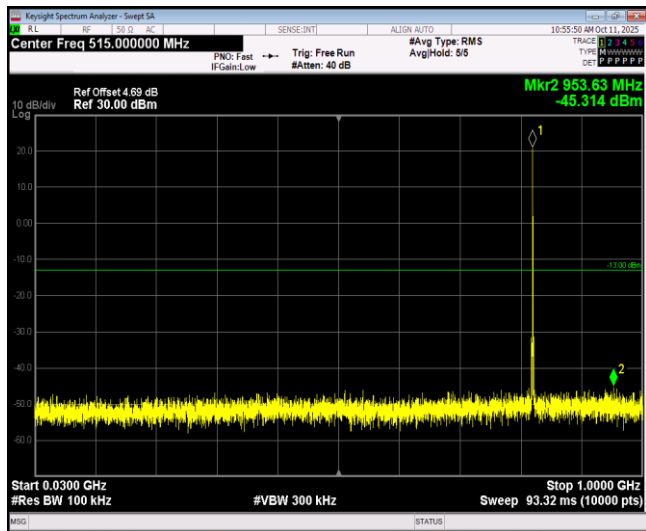
Band26-1.4MHz-64QAM-26915-1RB#0-Range1:30~1000MHz
