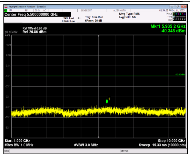
Band26-1.4MHz-QPSK-26740-1RB#0-Range2:1000~10000MHz
