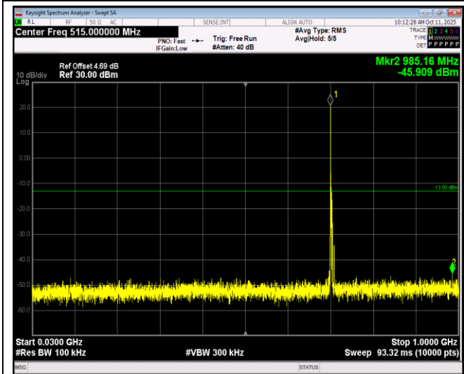
Band17-5MHz-64QAM-23825-1RB#0-Range1:30~1000MHz
