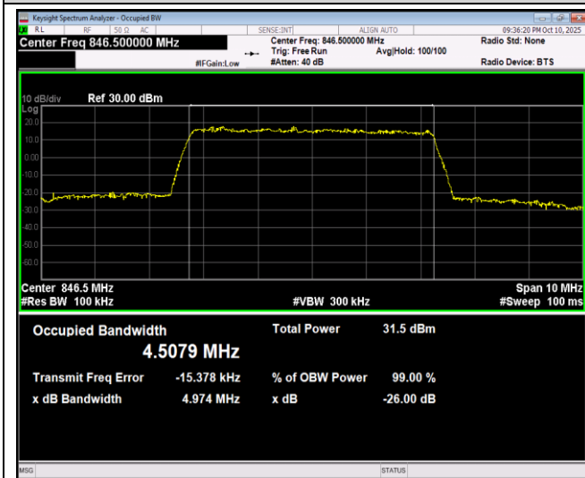
Band5-5MHz-16QAM-20525-25RB#0
