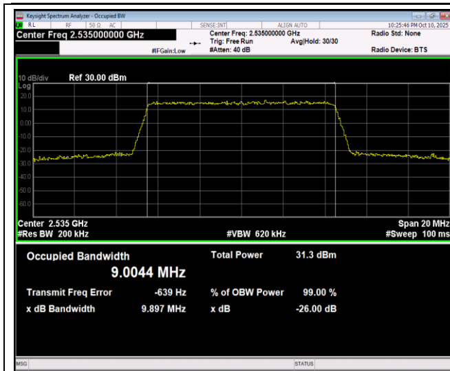
Band7-10MHz-16QAM-20800-50RB#0
