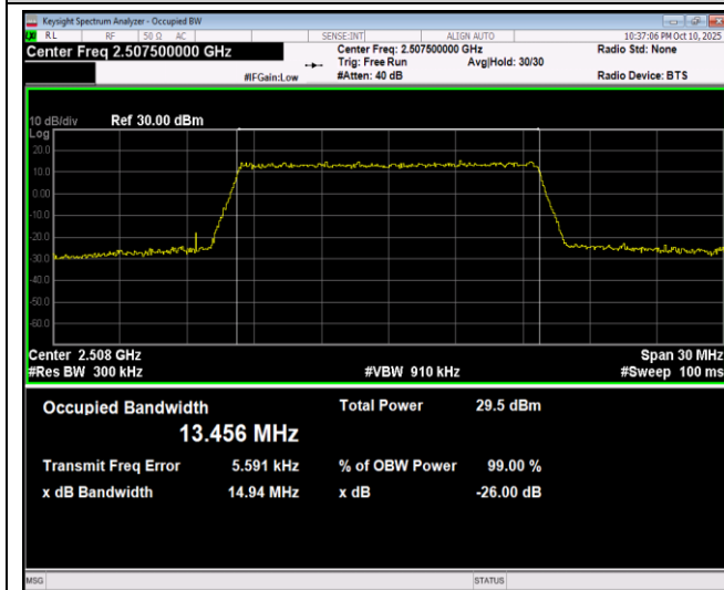
Band7-15MHz-64QAM-21375-75RB#0
