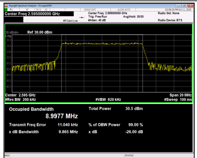
Band38-10MHz-16QAM-37800-50RB#0
