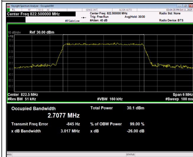
Band26-3MHz-16QAM-26915-15RB#0
