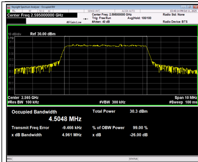
Band38-5MHz-16QAM-37775-25RB#0
