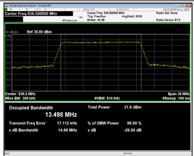
Band26-15MHz-16QAM-26865-75RB#0
