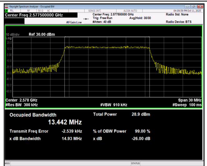
Band38-15MHz-64QAM-38175-75RB#0
