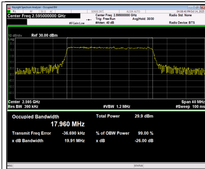
Band41-20MHz-64QAM-40140-100RB#0
