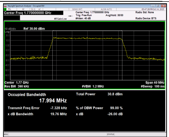
Band66-20MHz-64QAM-132322-100RB#0
