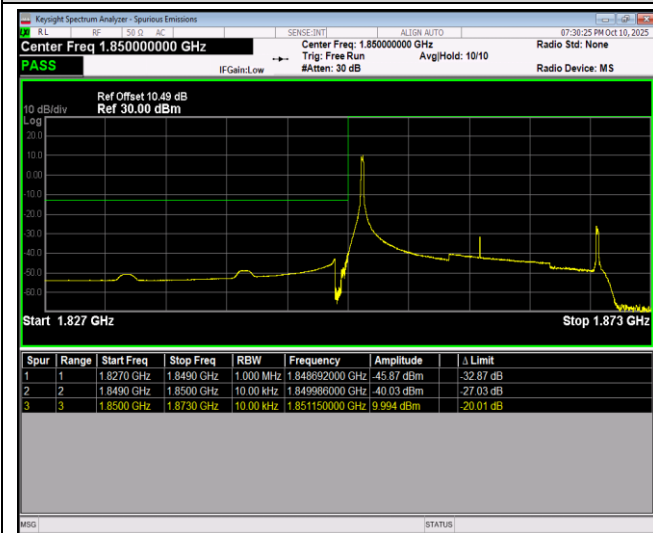
Band2-20MHz-64QAM-18700-100RB#0
