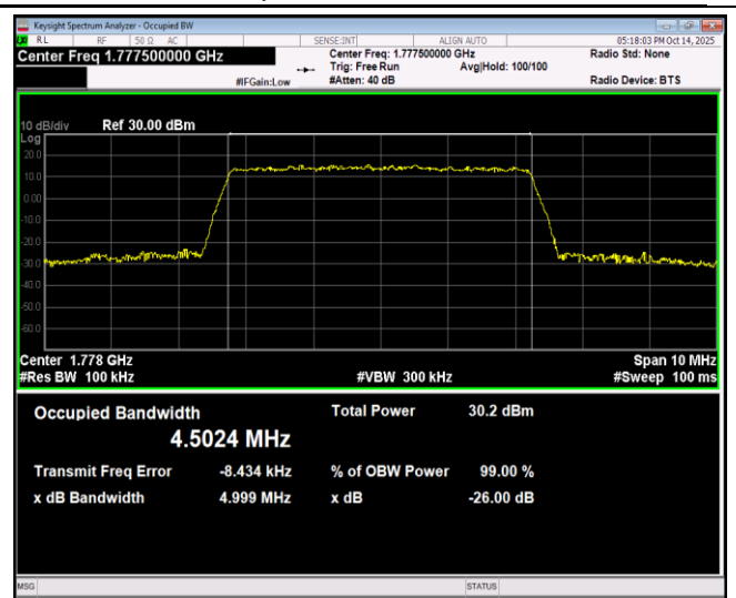
Band66-10MHz-QPSK-132322-50RB#0
