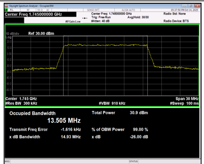
Band66-15MHz-64QAM-132047-75RB#0
