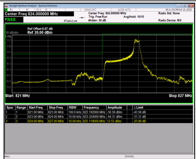
Band5-1.4MHz-64QAM-20643-1RB#0
