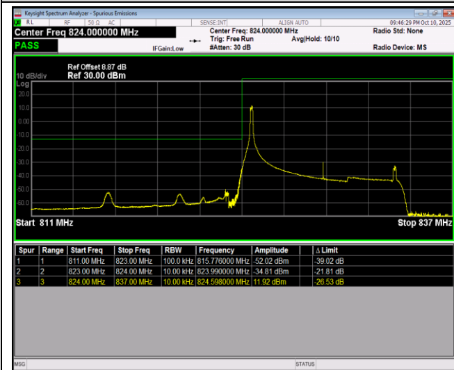
Band5-10MHz-16QAM-20450-50RB#0
