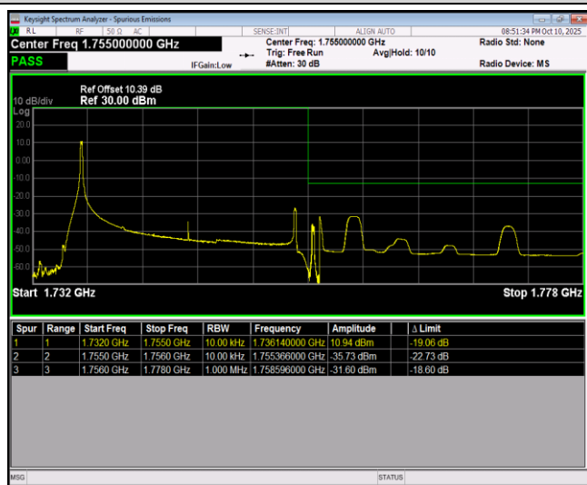
Band4-20MHz-QPSK-20300-100RB#0
