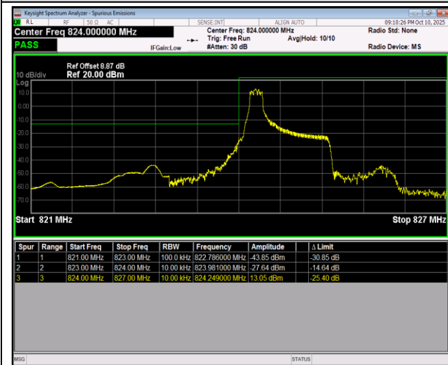
Band5-1.4MHz-QPSK-20407-6RB#0
