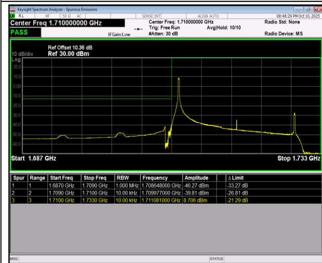
Band4-20MHz-64QAM-20050-100RB#0
