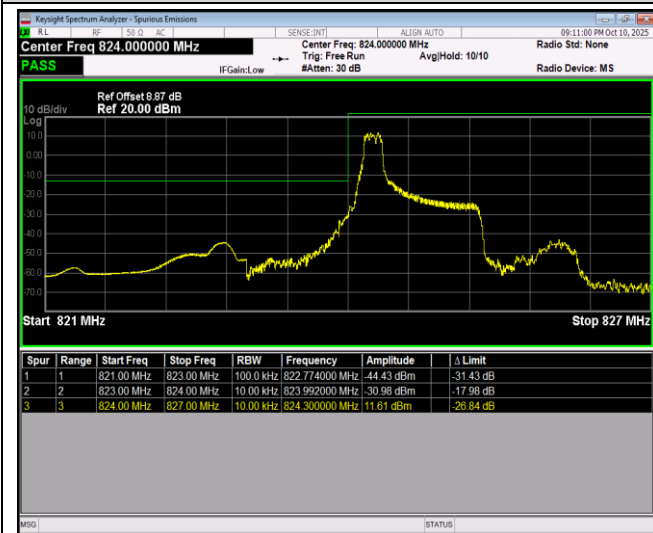
Band5-1.4MHz-64QAM-20407-6RB#0
