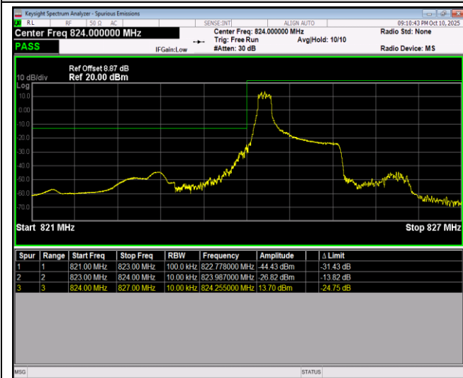
Band5-1.4MHz-16QAM-20407-6RB#0
