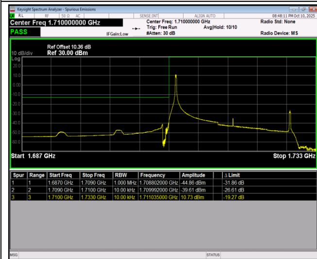
Band4-20MHz-16QAM-20050-100RB#0
