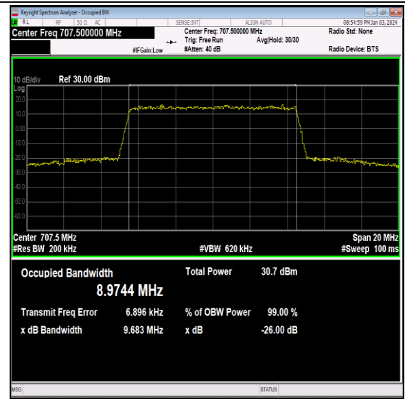
Band12-10MHz-16QAM-23095-50RB#0-PASS
