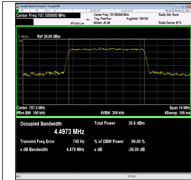
Band12-5MHz-16QAM-23095-25RB#0-PASS
