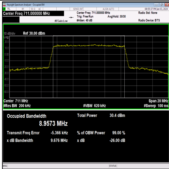
Band12-10MHz-16QAM-23130-50RB#0-PASS
