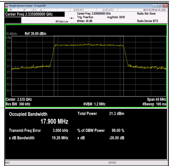
Band7-20MHz-16QAM-21100-100RB#0-PASS
