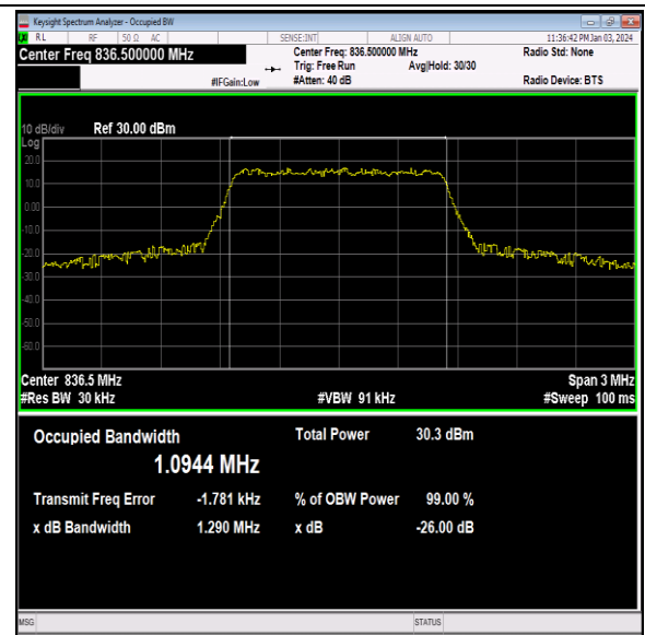
26(824-849)-1.4MHz-QPSK-26915-6RB#0-PASS
