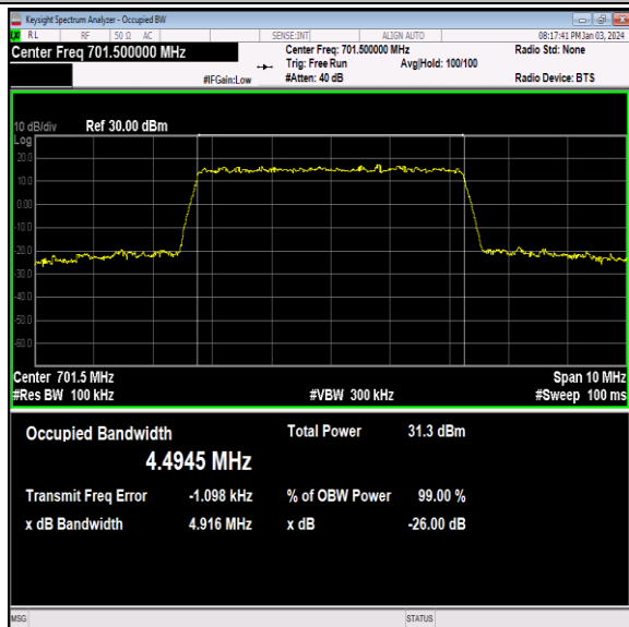
Band12-5MHz-64QAM-23035-25RB#0-PASS
