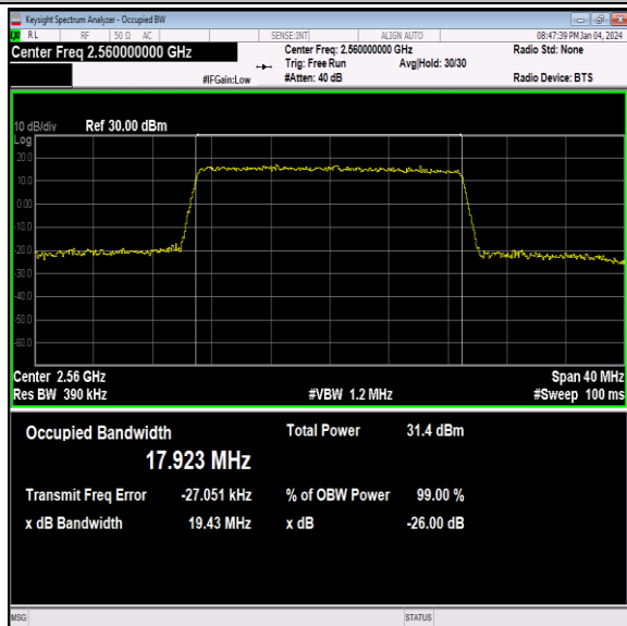
Band7-20MHz-16QAM-21350-100RB#0-PASS
