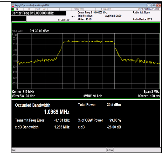
26(814-824)-1.4MHz-64QAM-26740-6RB#0-PASS
