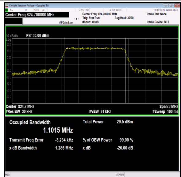
26(824-849)-1.4MHz-16QAM-26797-6RB#0-PASS
