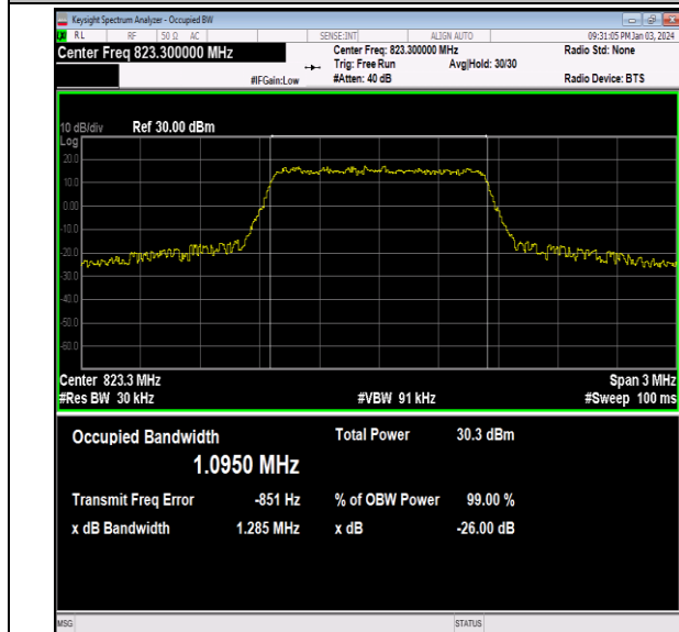
26(814-824)-1.4MHz-64QAM-26783-6RB#0-PASS
