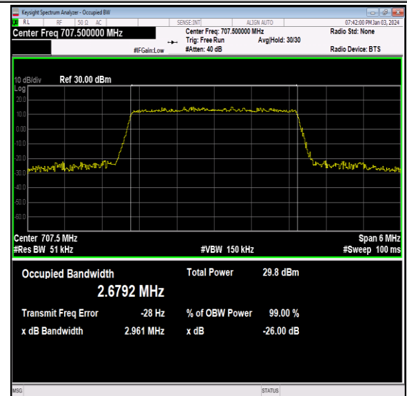
Band12-3MHz-16QAM-23095-15RB#0-PASS
