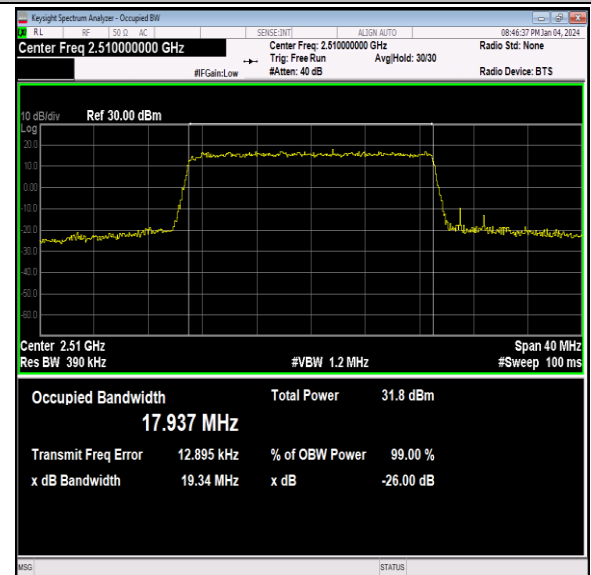
Band7-20MHz-64QAM-20850-100RB#0-PASS
