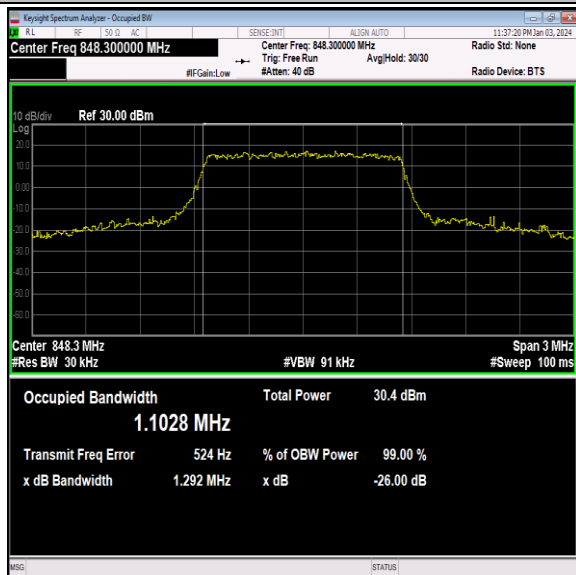
26(824-849)-1.4MHz-QPSK-27033-6RB#0-PASS
