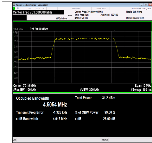
Band12-5MHz-QPSK-23035-25RB#0-PASS
