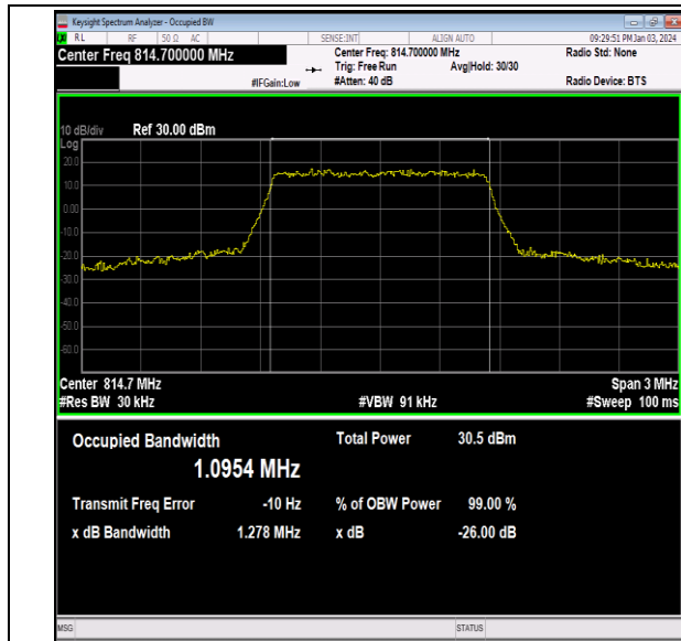
26(814-824)-1.4MHz-64QAM-26697-6RB#0-PASS
