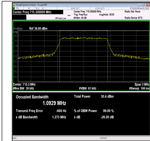
Band12-1.4MHz-QPSK-23173-6RB#0-PASS
