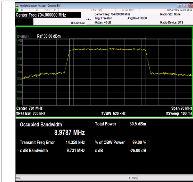
Band12-10MHz-16QAM-23060-50RB#0-PASS
