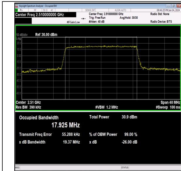
Band7-20MHz-16QAM-20850-100RB#0-PASS
