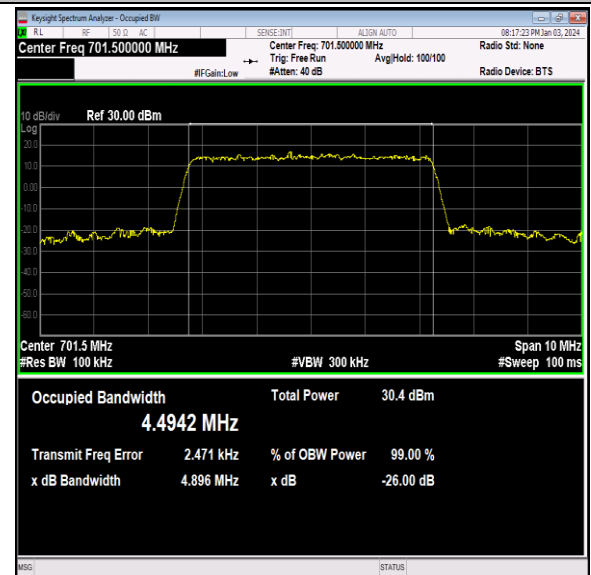
Band12-5MHz-16QAM-23035-25RB#0-PASS
