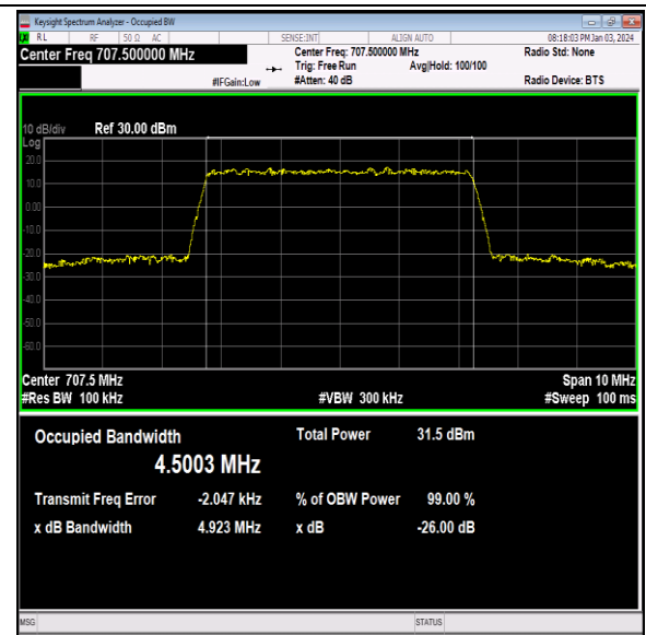
Band12-5MHz-QPSK-23095-25RB#0-PASS
