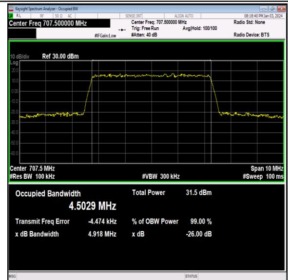
Band12-5MHz-64QAM-23095-25RB#0-PASS
