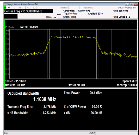
Band12-1.4MHz-16QAM-23173-6RB#0-PASS
