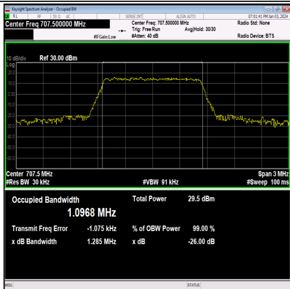
Band12-1.4MHz-16QAM-23095-6RB#0-PASS
