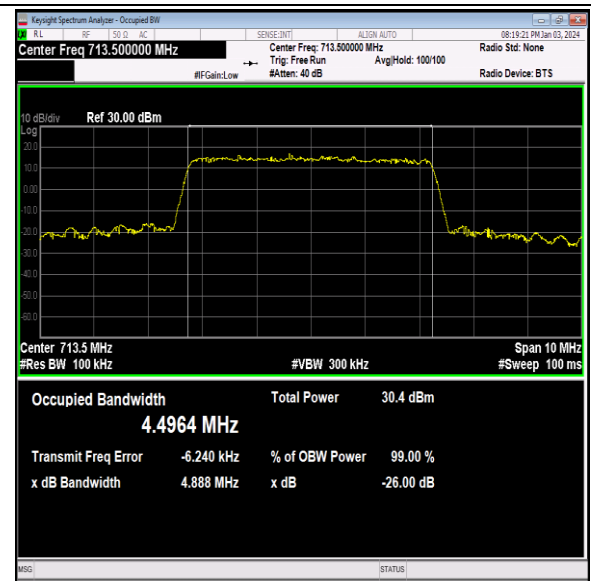
Band12-5MHz-16QAM-23155-25RB#0-PASS
