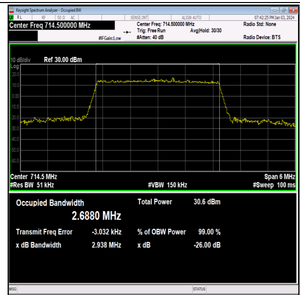
Band12-3MHz-QPSK-23165-15RB#0-PASS
