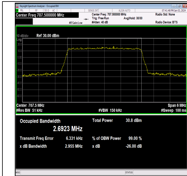
Band12-3MHz-QPSK-23095-15RB#0-PASS
