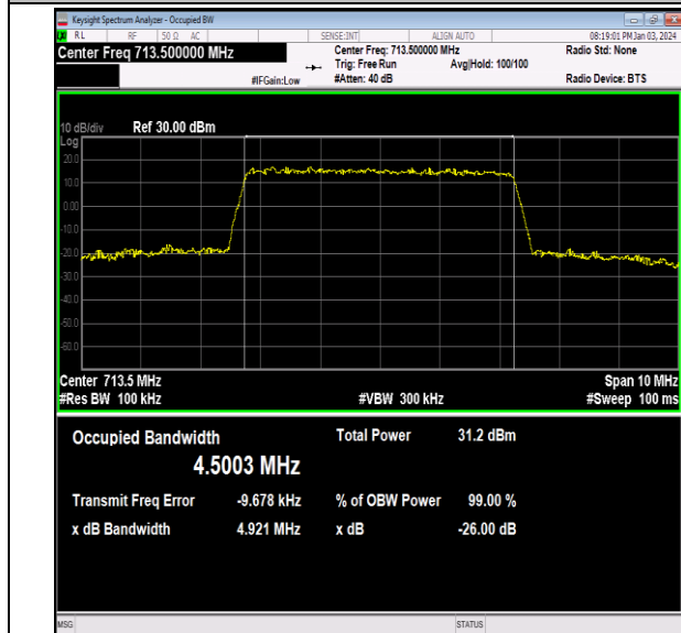
Band12-5MHz-QPSK-23155-25RB#0-PASS
