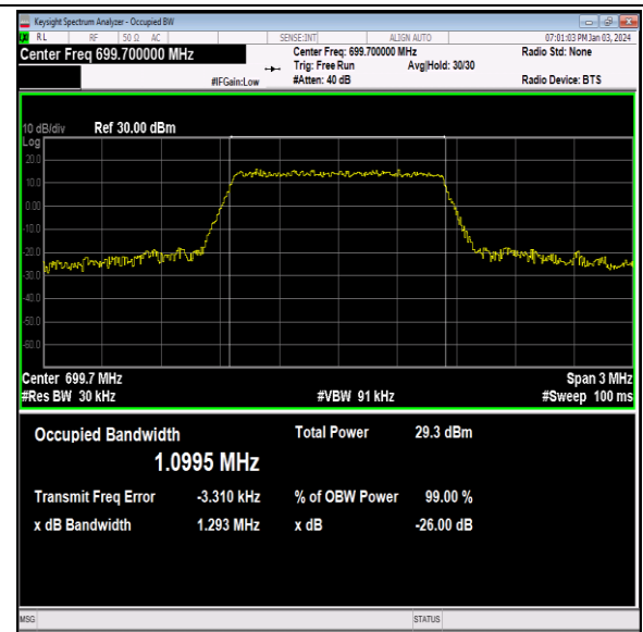
Band12-1.4MHz-16QAM-23017-6RB#0-PASS
