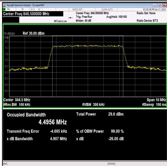
26(824-849)-5MHz-64QAM-27015-25RB#0-PASS
