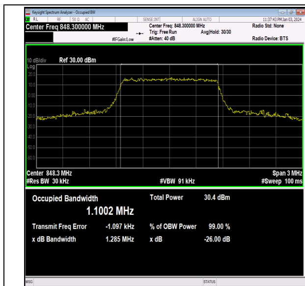
26(824-849)-1.4MHz-64QAM-27033-6RB#0-PASS
