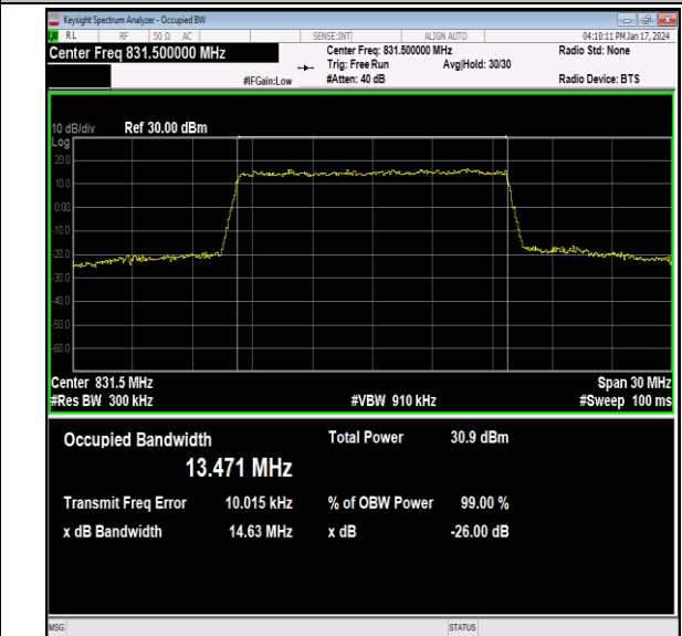
26(824-849)-15MHz-16QAM-26865-75RB#0-PASS
