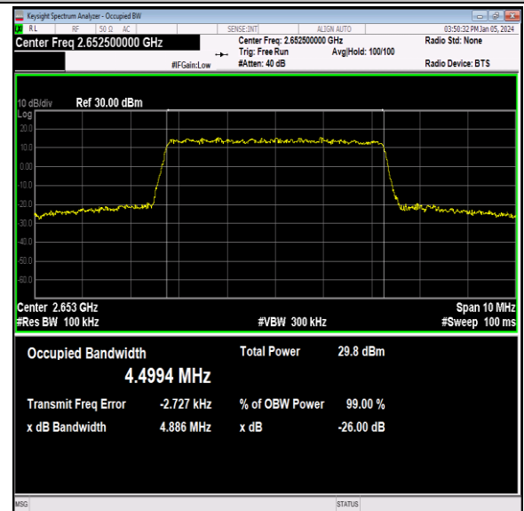
41(2535-2655)-5MHz-64QAM-41215-25RB#0-PASS
