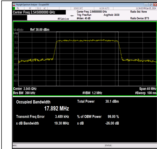
41(2535-2655)-20MHz-64QAM-40140-100RB#0-PASS
