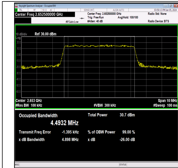
41(2535-2655)-5MHz-16QAM-41215-25RB#0-PASS
