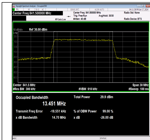
26(824-849)-15MHz-64QAM-26965-75RB#0-PASS
