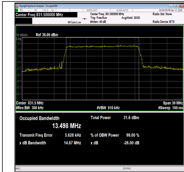
26(824-849)-15MHz-QPSK-26865-75RB#0-PASS
