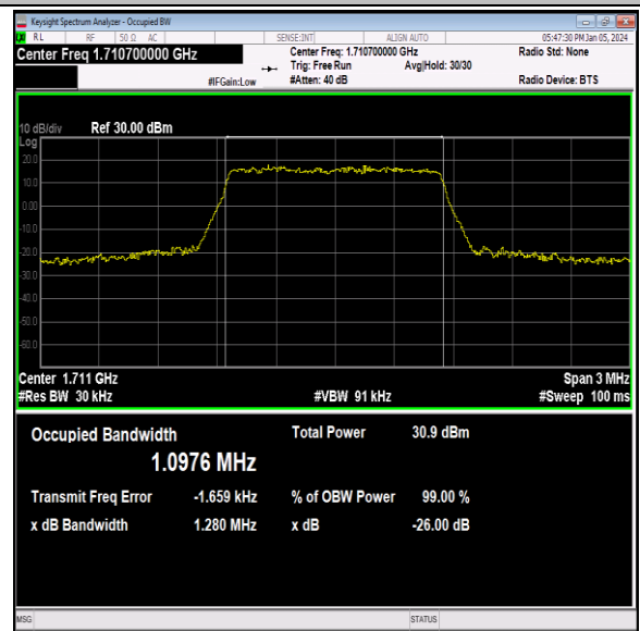
Band66-1.4MHz-QPSK-131979-6RB#0-PASS
