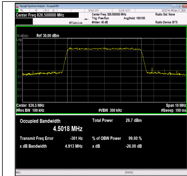
26(824-849)-5MHz-64QAM-26815-25RB#0-PASS
