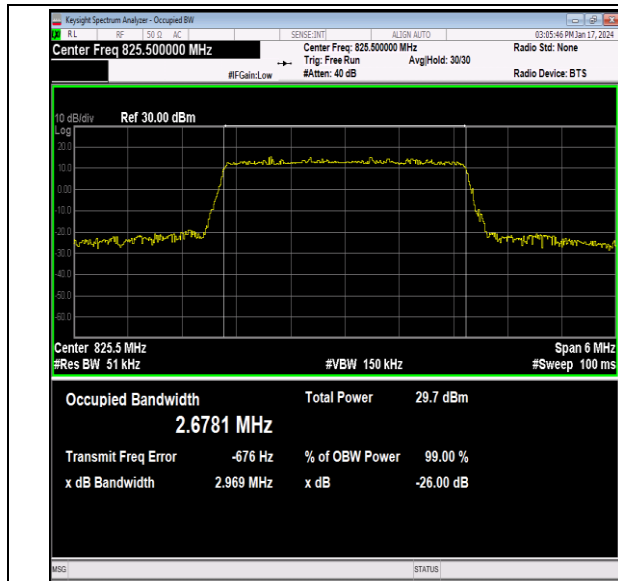
26(824-849)-3MHz-16QAM-26805-15RB#0-PASS
