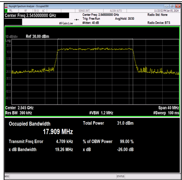
41(2535-2655)-20MHz-16QAM-40140-100RB#0-PASS
