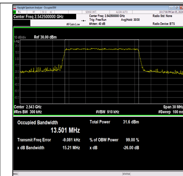
41(2535-2655)-15MHz-QPSK-40115-75RB#0-PASS
