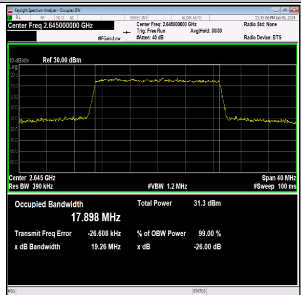
41(2535-2655)-20MHz-16QAM-41140-100RB#0-PASS
