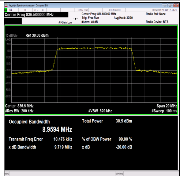
26(824-849)-10MHz-16QAM-26915-50RB#0-PASS
