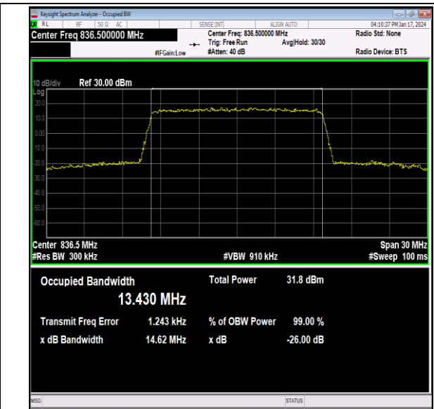
26(824-849)-15MHz-QPSK-26915-75RB#0-PASS
