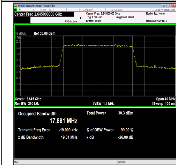
41(2535-2655)-20MHz-64QAM-41140-100RB#0-PASS
