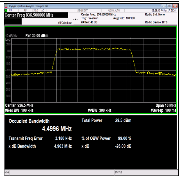
26(824-849)-5MHz-64QAM-26915-25RB#0-PASS
