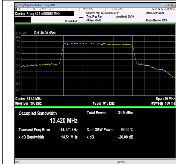
26(824-849)-15MHz-QPSK-26965-75RB#0-PASS
