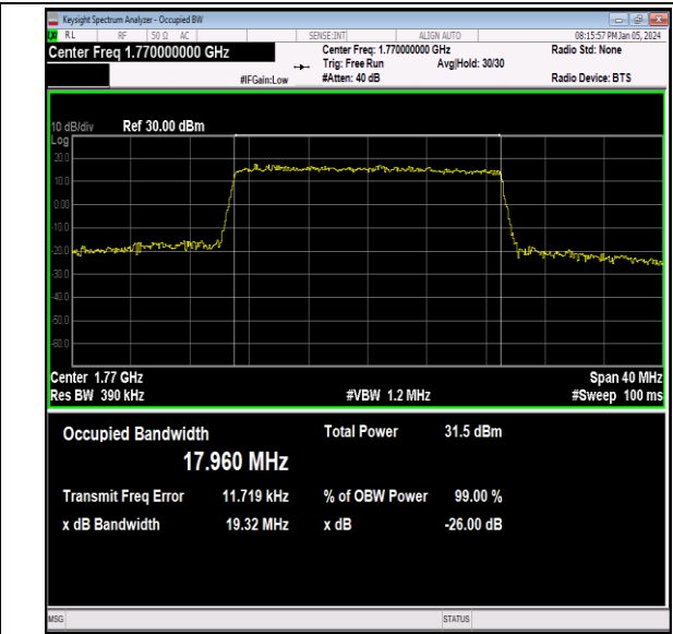
Band66-20MHz-16QAM-132572-100RB#0-PASS
