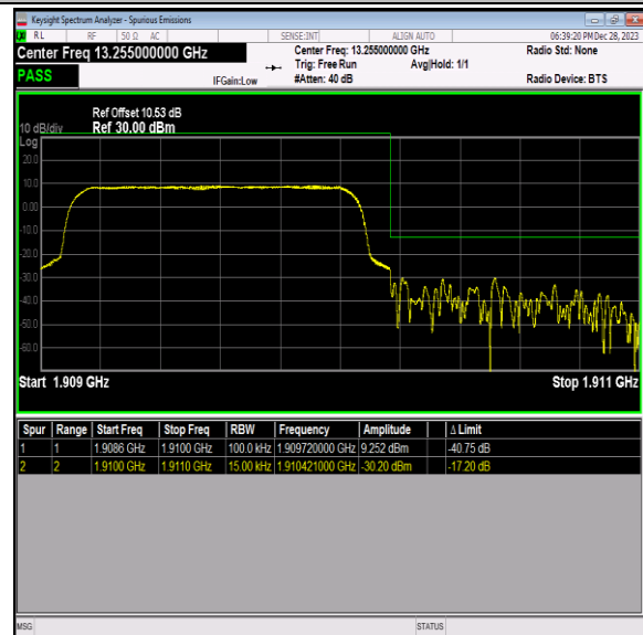
Band2_1.4MHz_16QAM_19193_6RB#0
