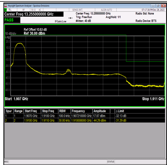
Band2_3MHz_64QAM_19185_1RB#0
