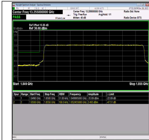
Band2_5MHz_16QAM_18625_25RB#0
