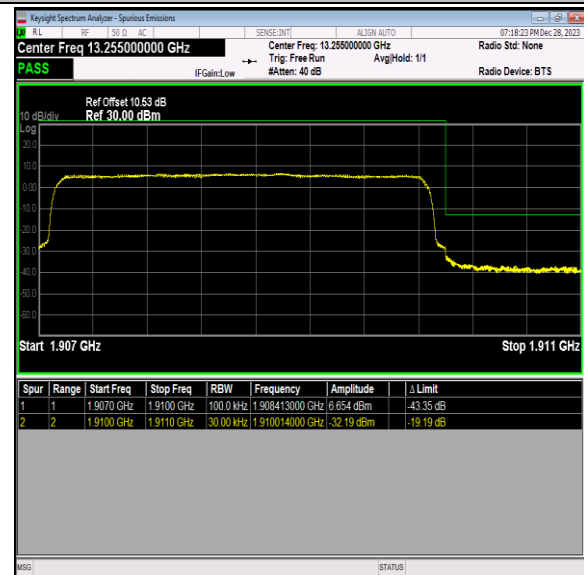
Band2_3MHz_QPSK_19185_15RB#0
