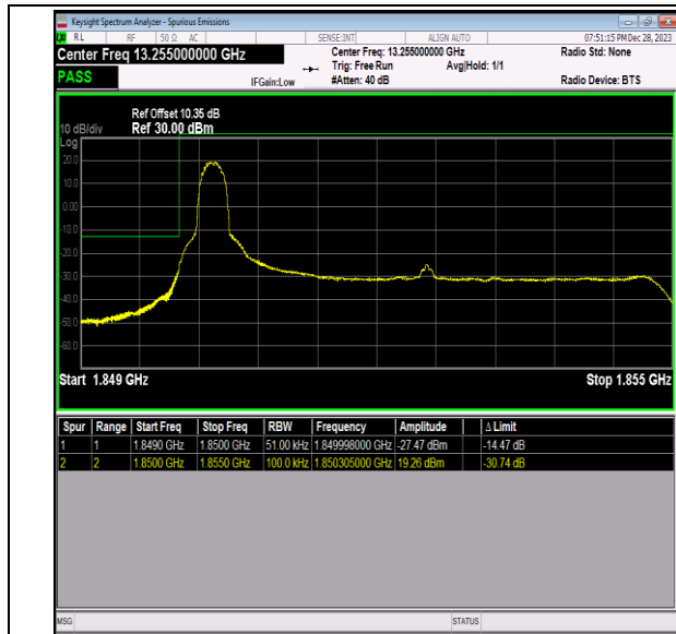
Band2_5MHz_QPSK_18625_1RB#0
