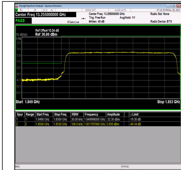
Band2_3MHz_QPSK_18615_15RB#0
