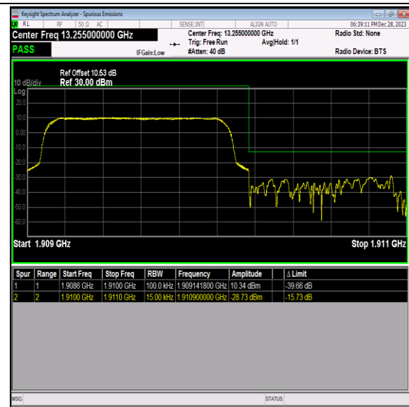
Band2_1.4MHz_QPSK_19193_6RB#0
