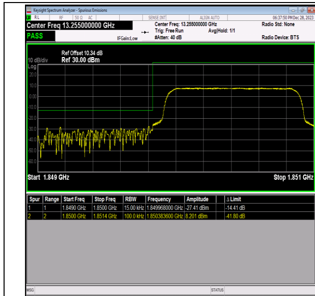
Band2_1.4MHz_16QAM_18607_6RB#0
