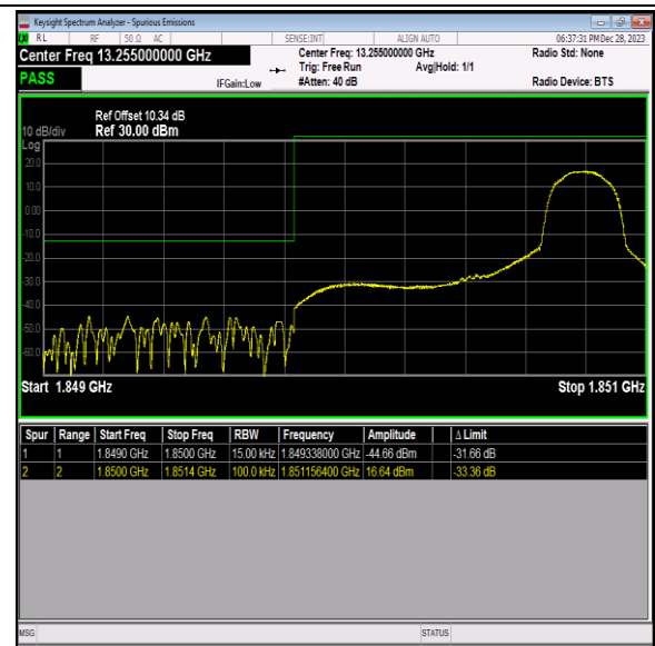
Band2_1.4MHz_64QAM_18607_1RB#5
