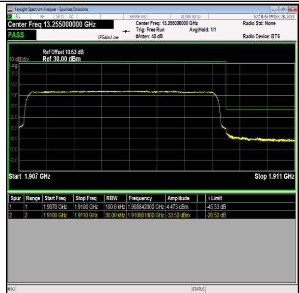
Band2_3MHz_64QAM_19185_15RB#0
