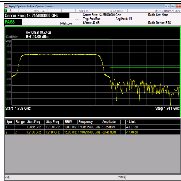
Band2_1.4MHz_64QAM_19193_6RB#0
