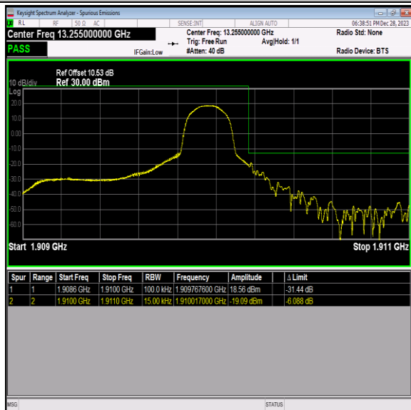
Band2_1.4MHz_16QAM_19193_1RB#5
