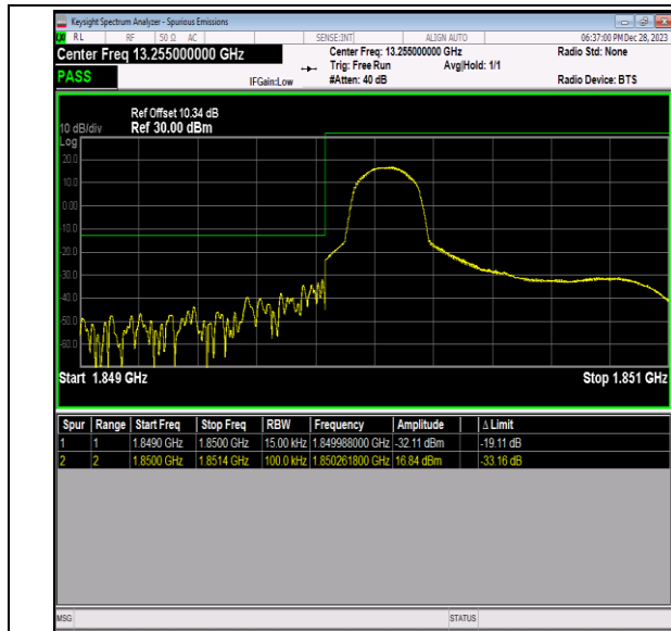
Band2_1.4MHz_64QAM_18607_1RB#0
