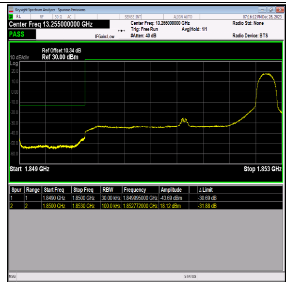
Band2_3MHz_16QAM_18615_1RB#14
