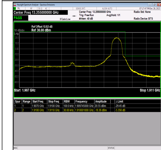
Band2_3MHz_QPSK_19185_1RB#14
