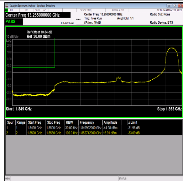
Band2_3MHz_64QAM_18615_1RB#14
