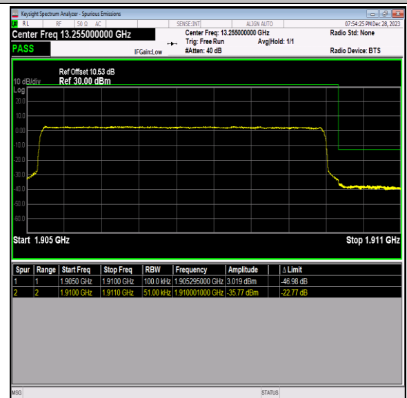
Band2_5MHz_16QAM_19175_25RB#0
