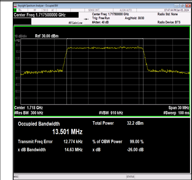
Band66-15MHz-QPSK-132047-75RB#0-PASS
