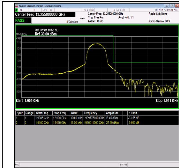
Band2_1.4MHz_64QAM_19193_1RB#5
