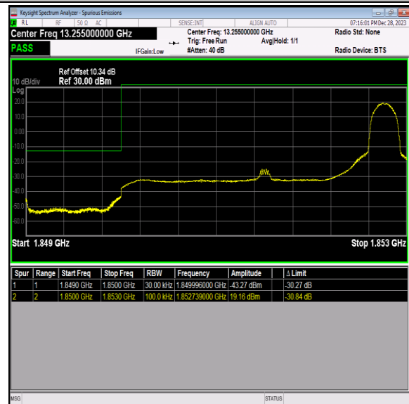
Band2_3MHz_QPSK_18615_1RB#14
