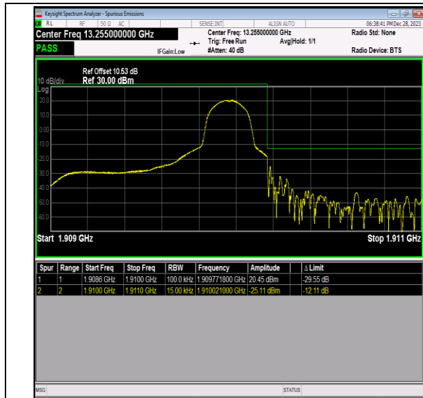
Band2_1.4MHz_QPSK_19193_1RB#5
