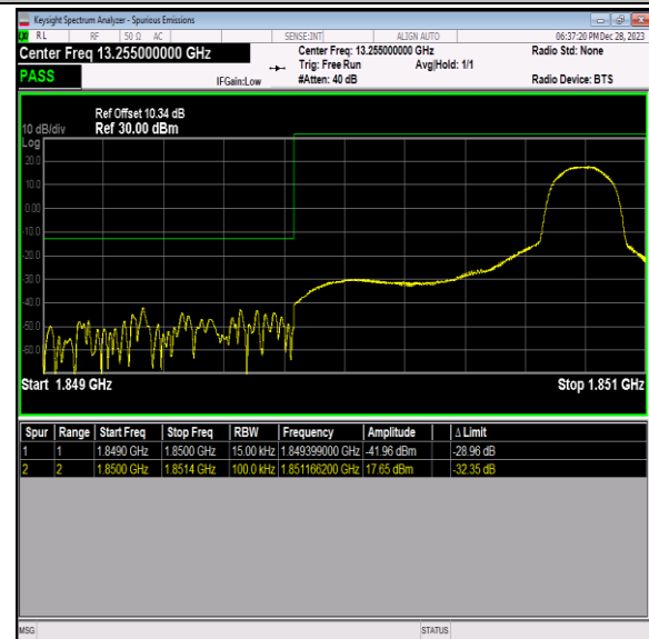
Band2_1.4MHz_16QAM_18607_1RB#5
