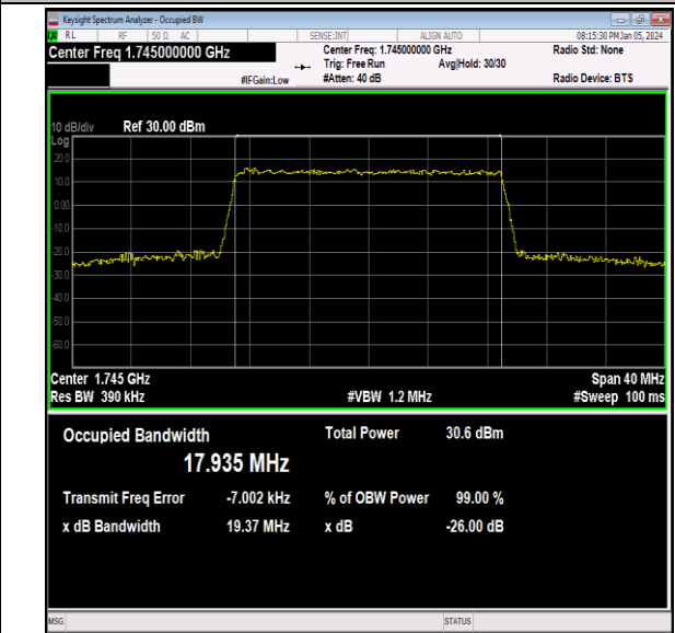
Band66-20MHz-64QAM-132322-100RB#0-PASS
