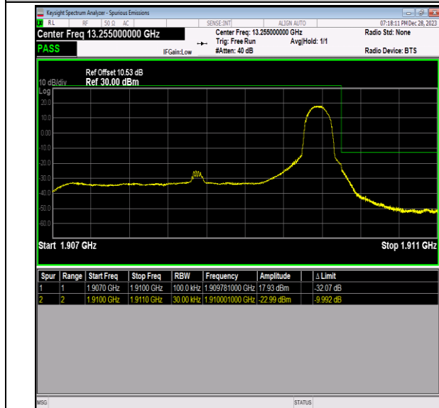
Band2_3MHz_64QAM_19185_1RB#14
