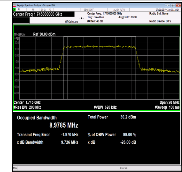
Band66-10MHz-64QAM-132322-50RB#0-PASS
