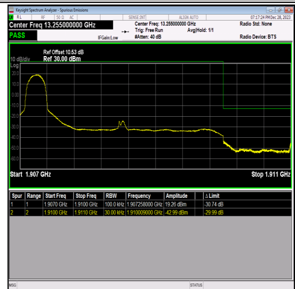
Band2_3MHz_16QAM_19185_1RB#0
