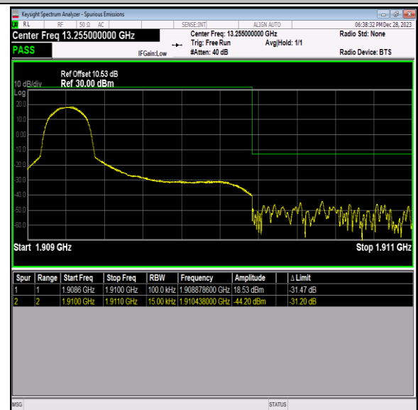
Band2_1.4MHz_64QAM_19193_1RB#0
