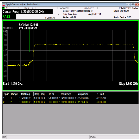
Band2_5MHz_QPSK_18625_25RB#0
