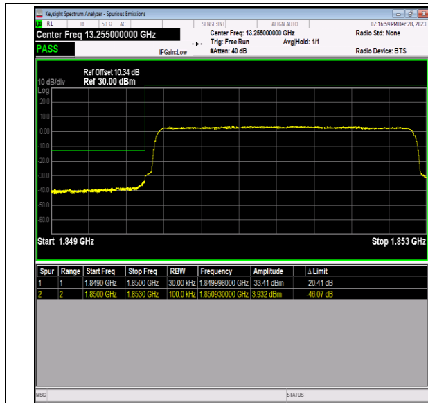
Band2_3MHz_64QAM_18615_15RB#0
