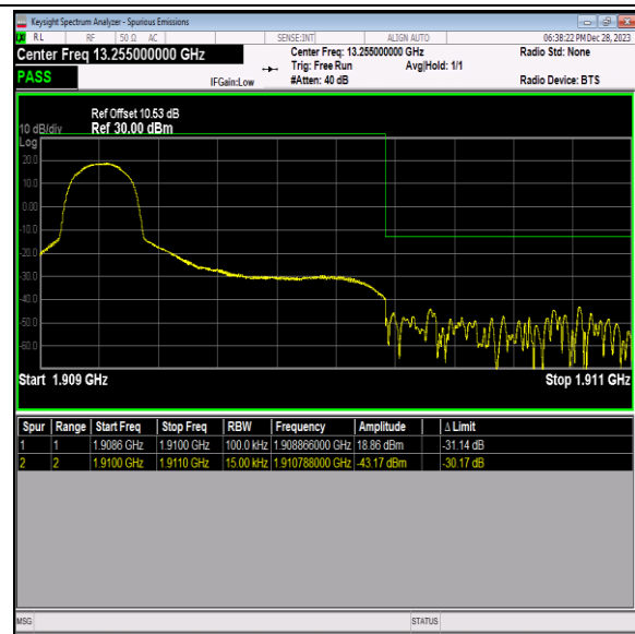
Band2_1.4MHz_16QAM_19193_1RB#0
