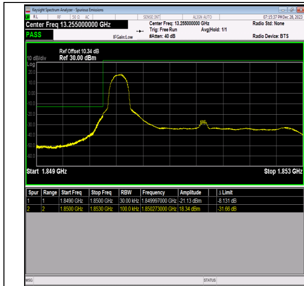
Band2_3MHz_16QAM_18615_1RB#0
