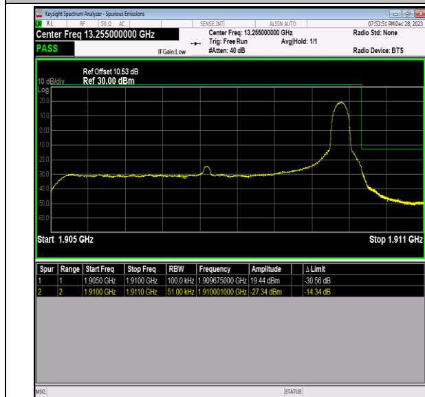
Band2_5MHz_16QAM_19175_1RB#24
