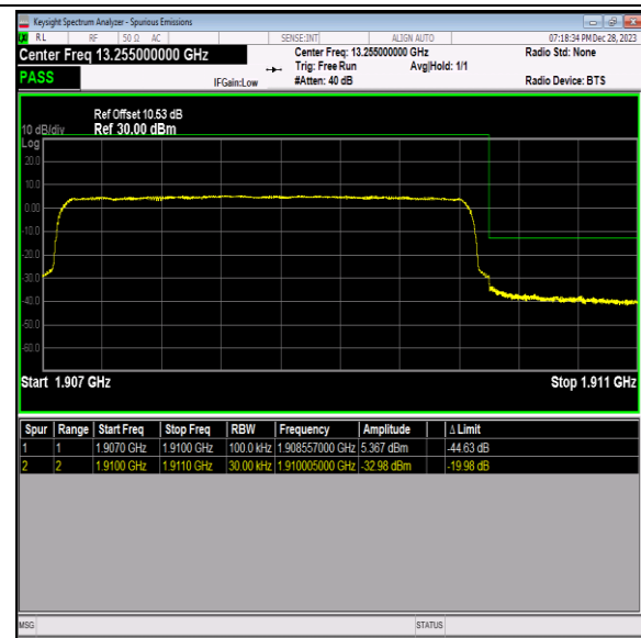
Band2_3MHz_16QAM_19185_15RB#0
