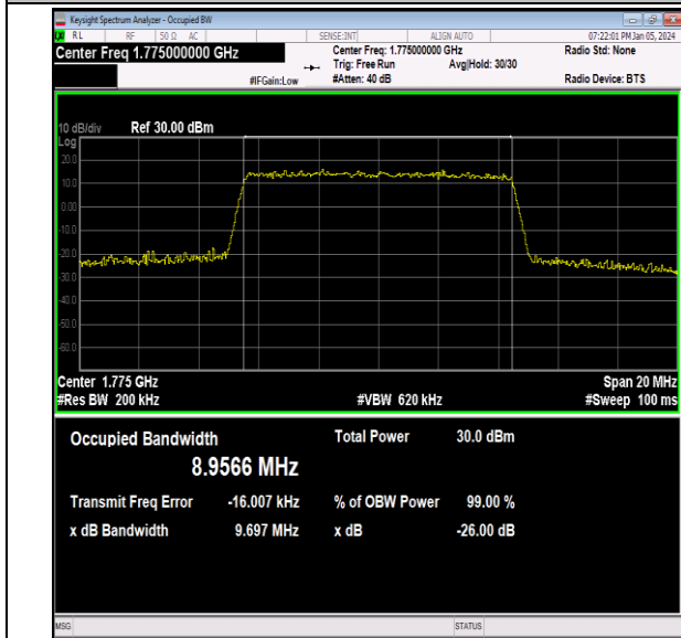
Band66-10MHz-64QAM-132622-50RB#0-PASS
