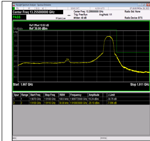
Band2_3MHz_16QAM_19185_1RB#14
