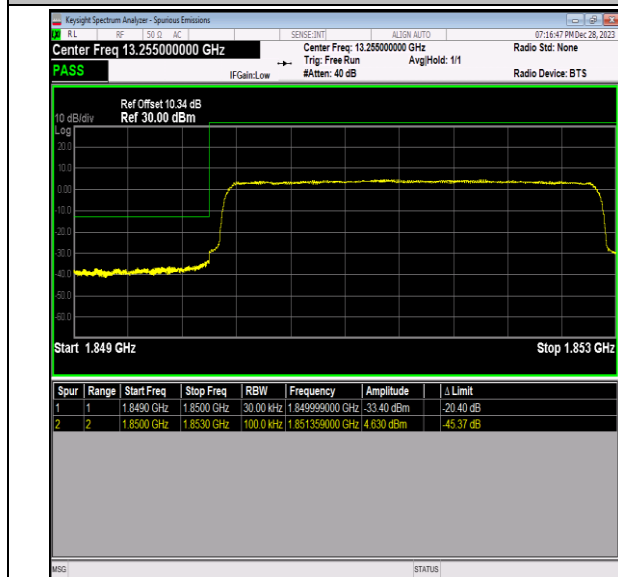
Band2_3MHz_16QAM_18615_15RB#0
