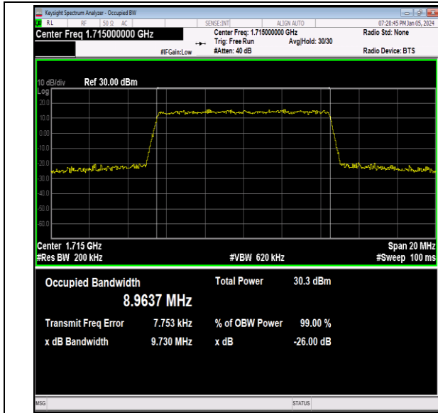
Band66-10MHz-64QAM-132022-50RB#0-PASS
