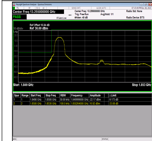
Band2_3MHz_64QAM_18615_1RB#0
