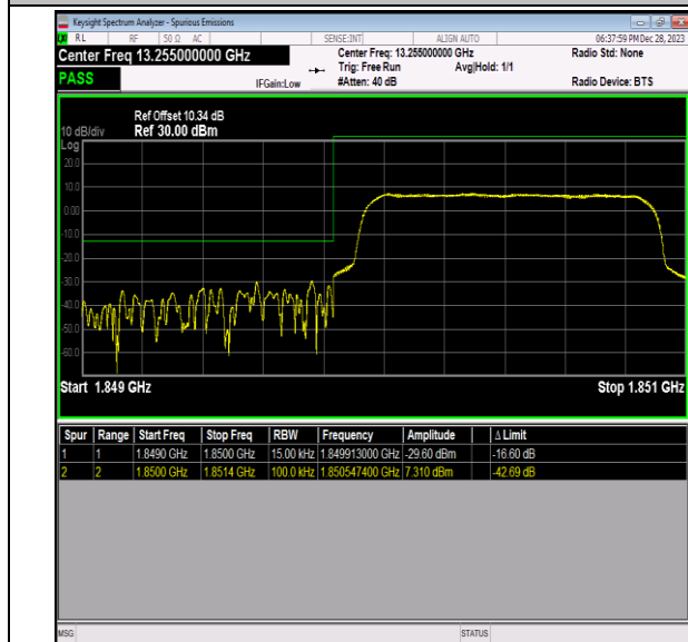
Band2_1.4MHz_64QAM_18607_6RB#0
