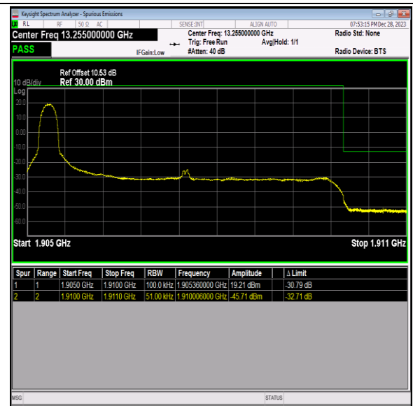
Band2_5MHz_16QAM_19175_1RB#0
