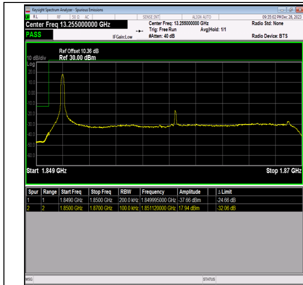
Band2_20MHz_16QAM_18700_1RB#0
