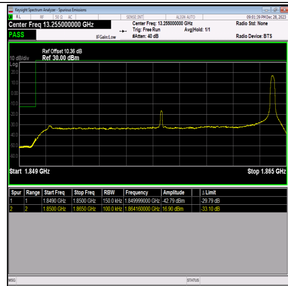
Band2_15MHz_64QAM_18675_1RB#74
