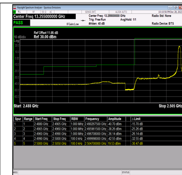
Band7_5MHz_QPSK_20775_1RB#24
