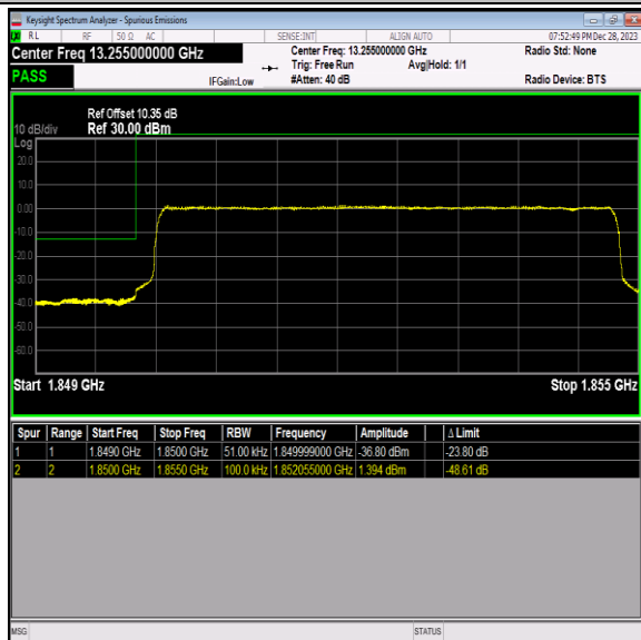
Band2_5MHz_64QAM_18625_25RB#0
