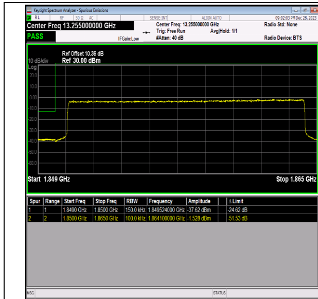
Band2_15MHz_16QAM_18675_75RB#0
