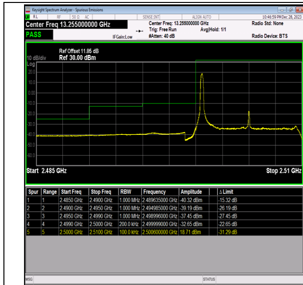
Band7_10MHz_16QAM_20800_1RB#0
