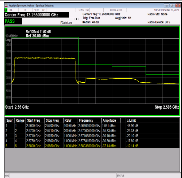
Band7_10MHz_QPSK_21400_50RB#0
