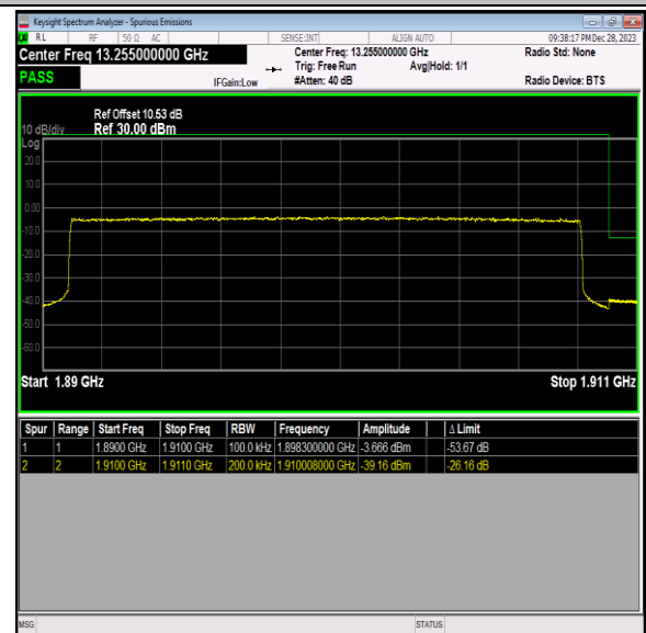
Band2_20MHz_64QAM_19100_100RB#0
