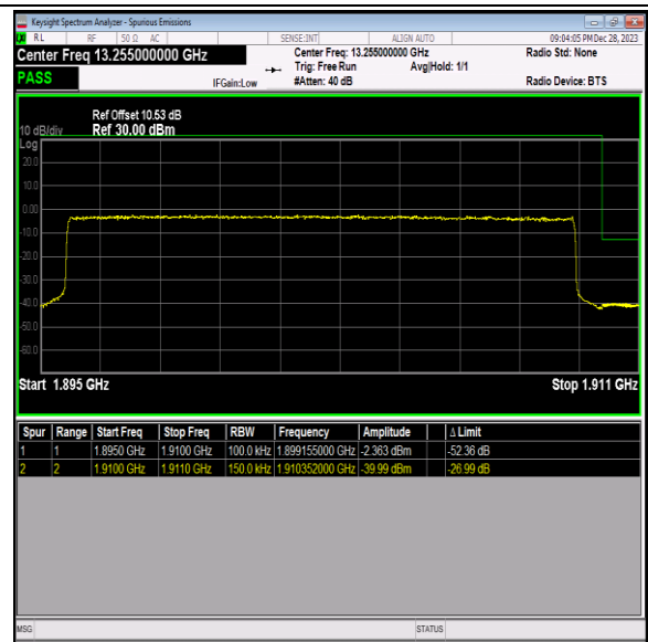
Band2_15MHz_64QAM_19125_75RB#0
