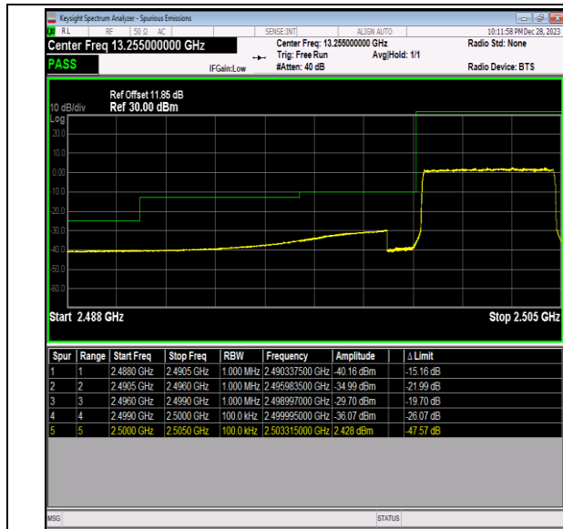
Band7_5MHz_16QAM_20775_25RB#0
