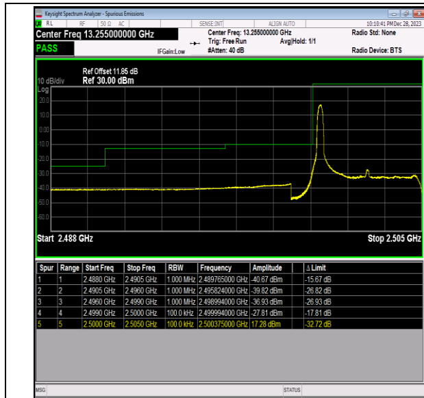
Band7_5MHz_64QAM_20775_1RB#0
