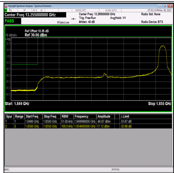
Band2_5MHz_64QAM_18625_1RB#24
