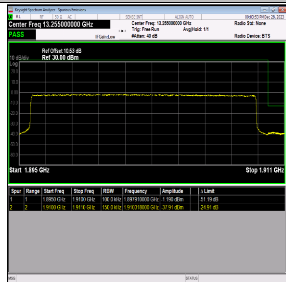
Band2_15MHz_16QAM_19125_75RB#0
