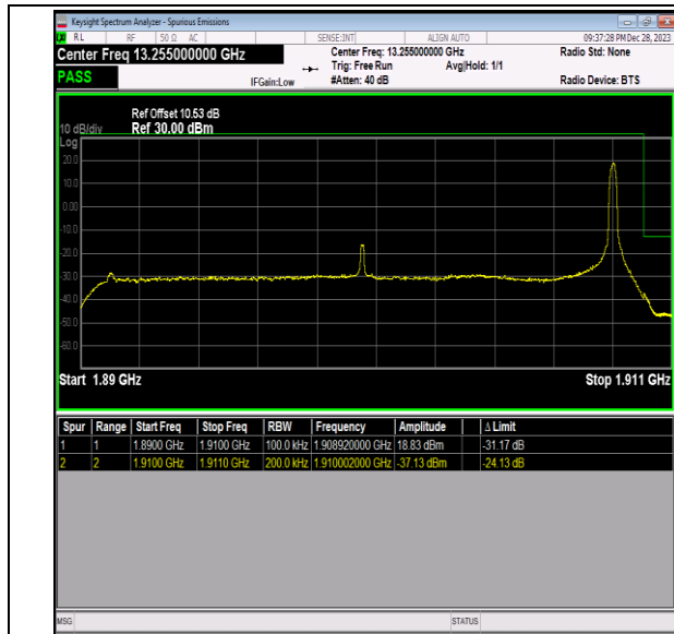
Band2_20MHz_16QAM_19100_1RB#99
