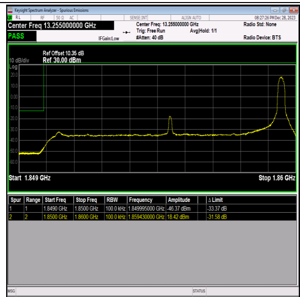
Band2_10MHz_16QAM_18650_1RB#49
