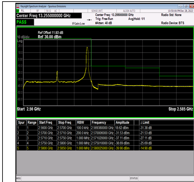
Band7_10MHz_16QAM_21400_1RB#49
