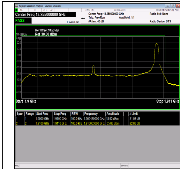
Band2_10MHz_16QAM_19150_1RB#49
