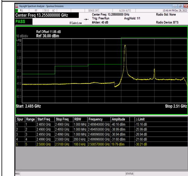
Band7_10MHz_QPSK_20800_1RB#0
