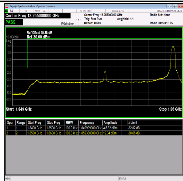
Band2_10MHz_QPSK_18650_1RB#49
