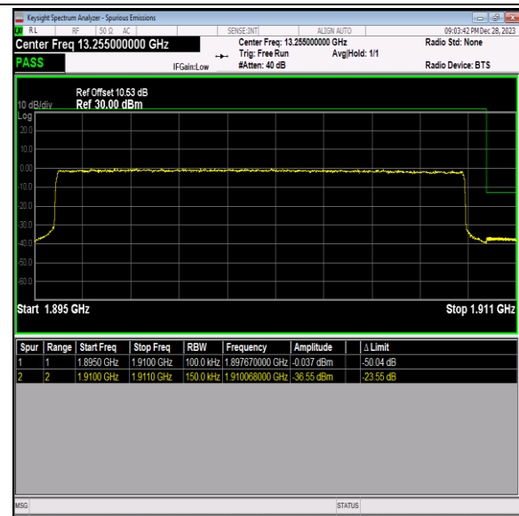
Band2_15MHz_QPSK_19125_75RB#0
