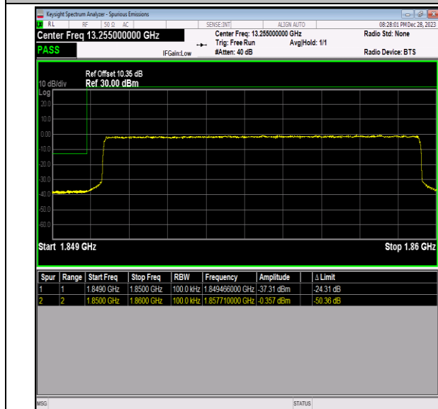
Band2_10MHz_16QAM_18650_50RB#0
