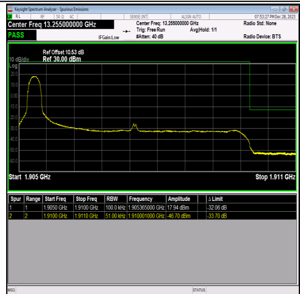
Band2_5MHz_64QAM_19175_1RB#0
