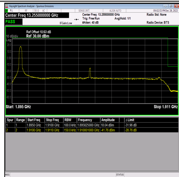
Band2_15MHz_64QAM_19125_1RB#0
