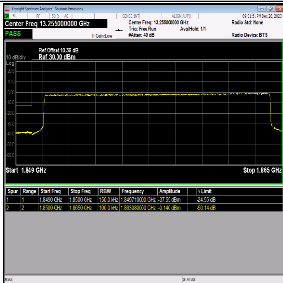
Band2_15MHz_QPSK_18675_75RB#0
