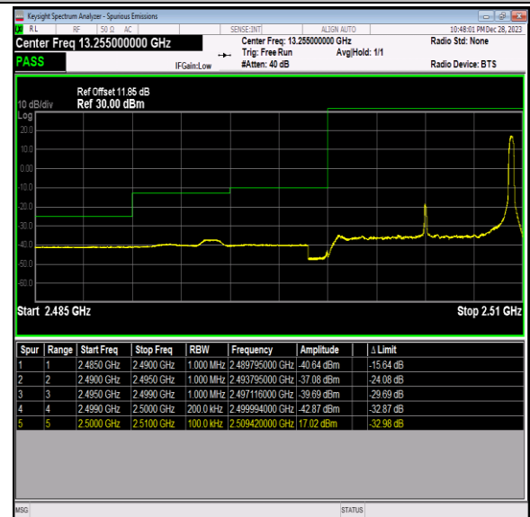
Band7_10MHz_64QAM_20800_1RB#49
