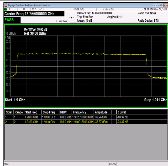
Band2_10MHz_QPSK_19150_50RB#0
