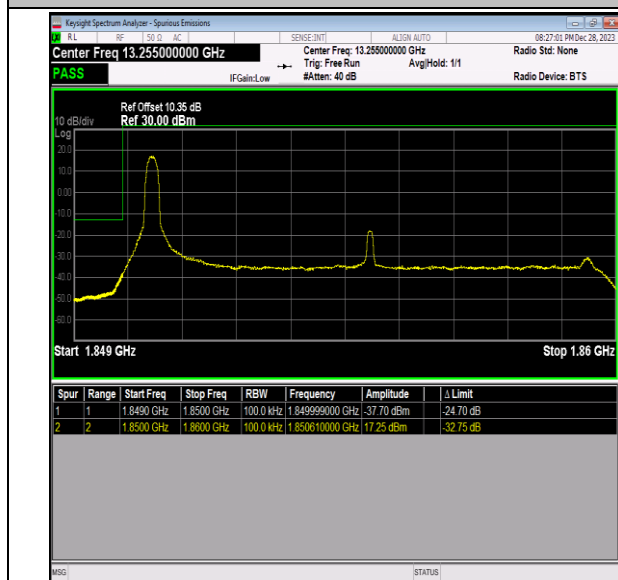
Band2_10MHz_64QAM_18650_1RB#0
