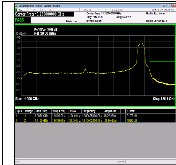
Band2_5MHz_64QAM_19175_1RB#24
