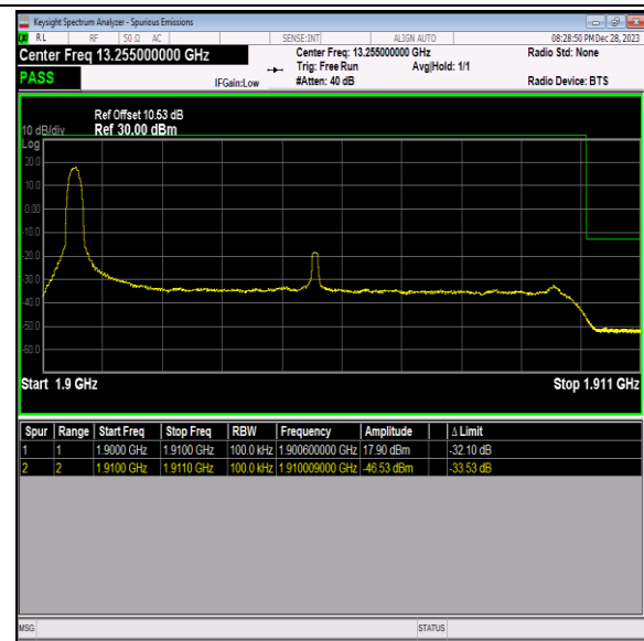
Band2_10MHz_64QAM_19150_1RB#0
