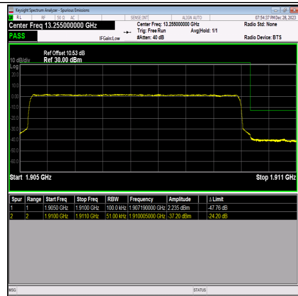
Band2_5MHz_64QAM_19175_25RB#0
