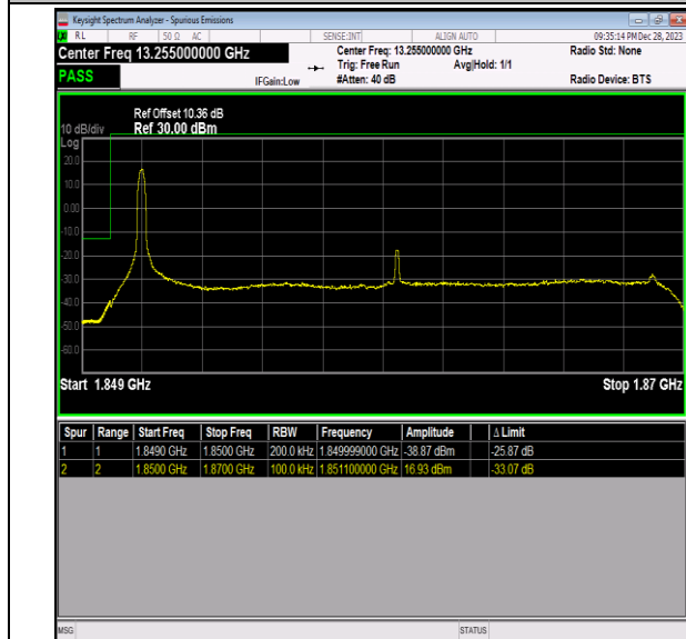
Band2_20MHz_64QAM_18700_1RB#0
