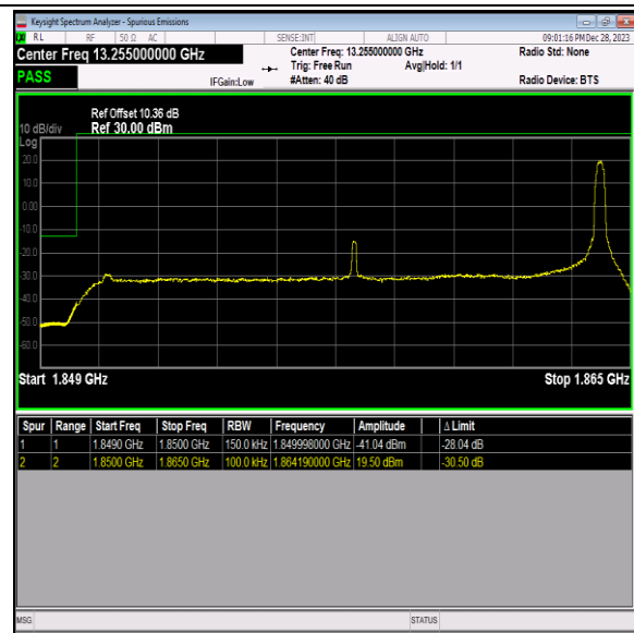
Band2_15MHz_QPSK_18675_1RB#74
