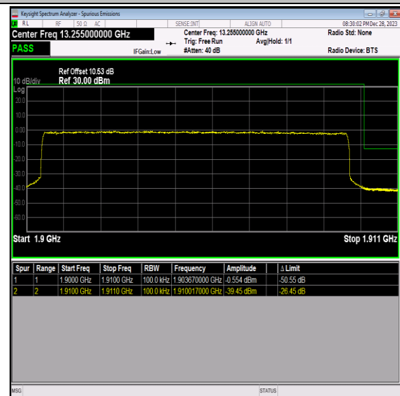
Band2_10MHz_64QAM_19150_50RB#0
