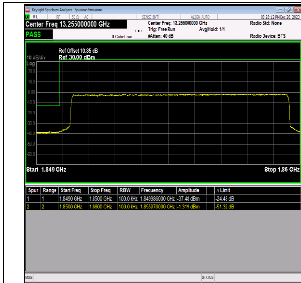
Band2_10MHz_64QAM_18650_50RB#0
