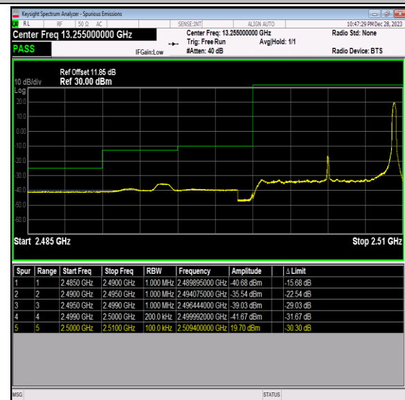
Band7_10MHz_QPSK_20800_1RB#49
