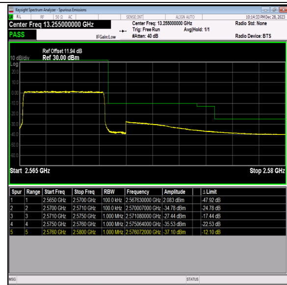
Band7_5MHz_64QAM_21425_25RB#0
