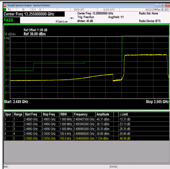
Band7_5MHz_64QAM_20775_25RB#0
