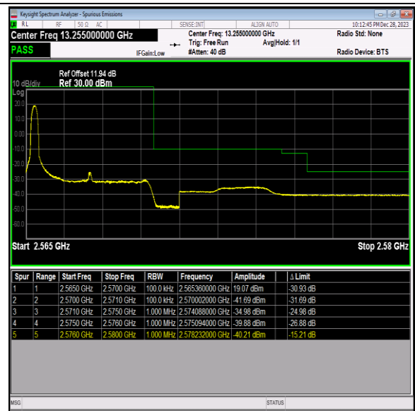
Band7_5MHz_16QAM_21425_1RB#0
