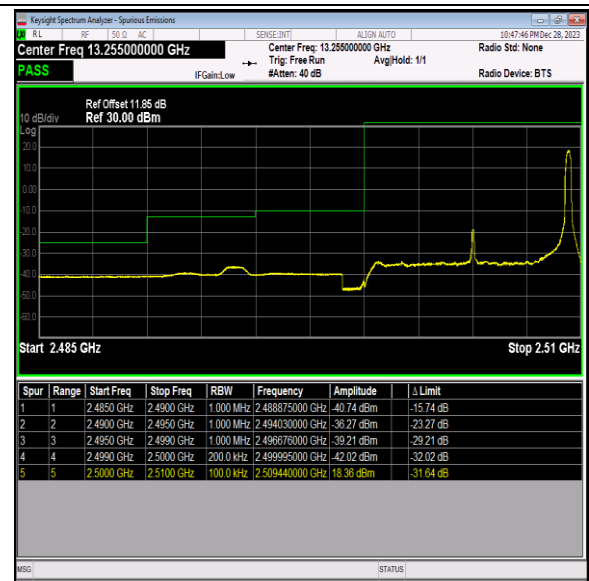
Band7_10MHz_16QAM_20800_1RB#49
