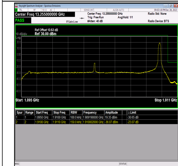
Band2_15MHz_16QAM_19125_1RB#74
