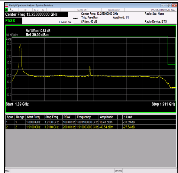
Band2_20MHz_16QAM_19100_1RB#0
