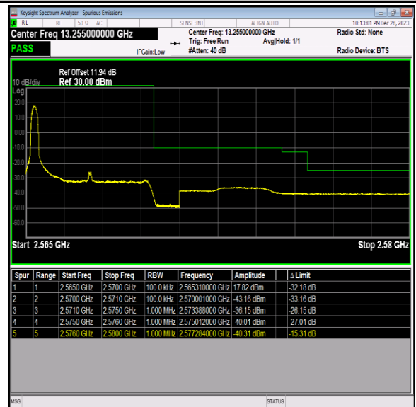
Band7_5MHz_64QAM_21425_1RB#0
