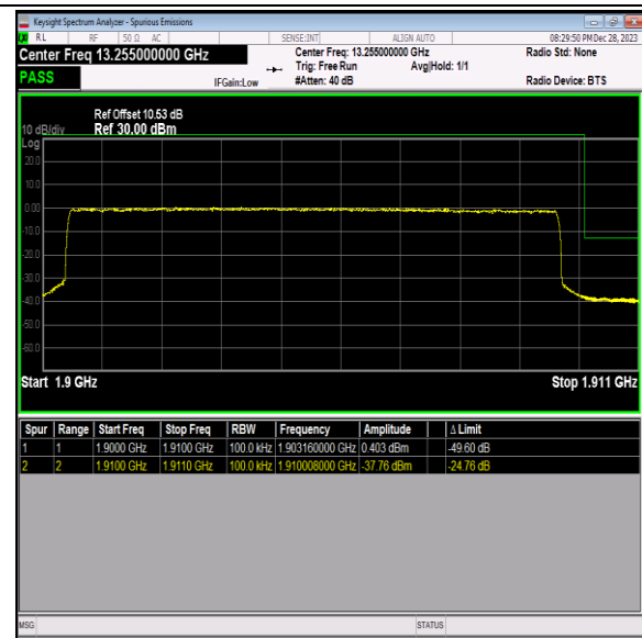
Band2_10MHz_16QAM_19150_50RB#0
