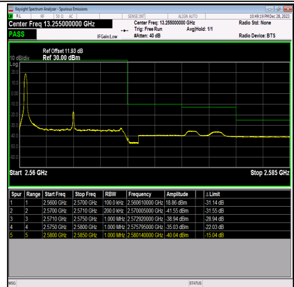
Band7_10MHz_16QAM_21400_1RB#0
