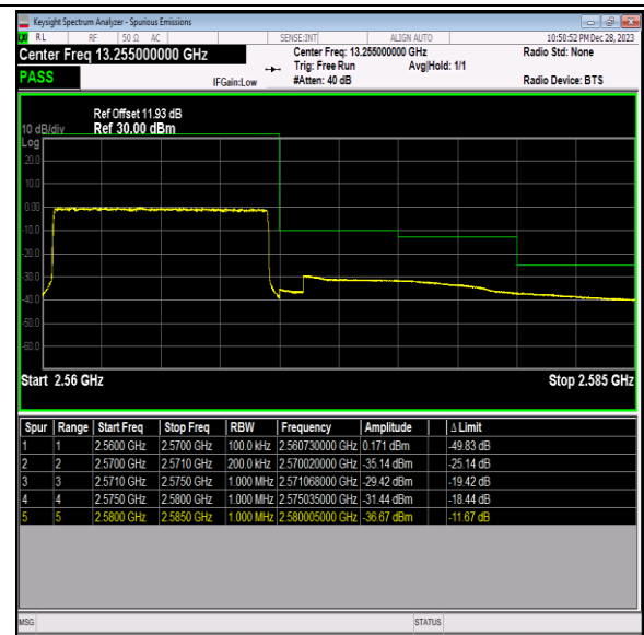
Band7_10MHz_16QAM_21400_50RB#0
