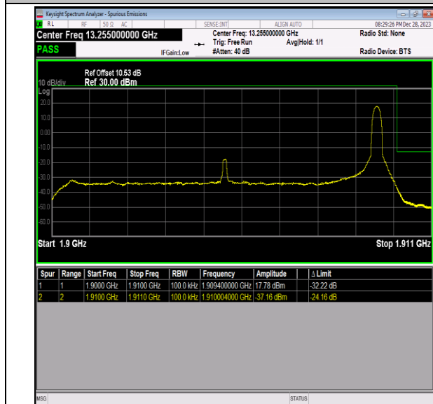
Band2_10MHz_64QAM_19150_1RB#49
