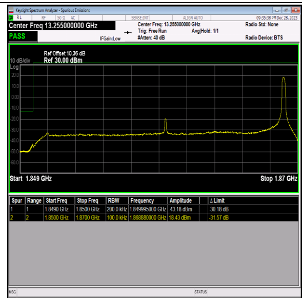
Band2_20MHz_16QAM_18700_1RB#99
