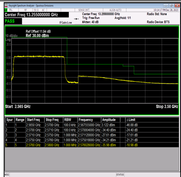
Band7_5MHz_16QAM_21425_25RB#0
