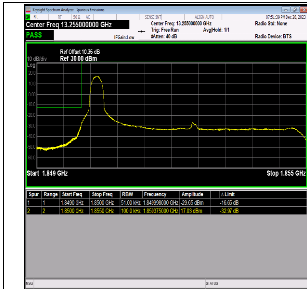
Band2_5MHz_64QAM_18625_1RB#0
