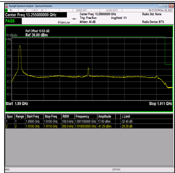
Band2_20MHz_64QAM_19100_1RB#0
