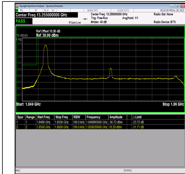
Band2_10MHz_16QAM_18650_1RB#0
