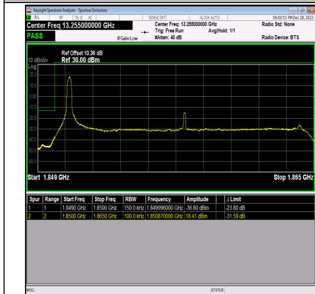
Band2_15MHz_16QAM_18675_1RB#0
