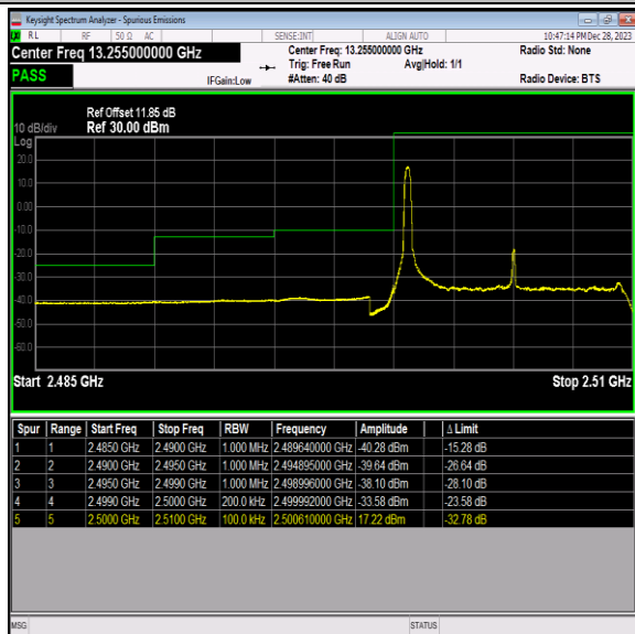
Band7_10MHz_64QAM_20800_1RB#0
