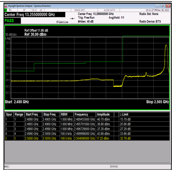
Band7_5MHz_64QAM_20775_1RB#24
