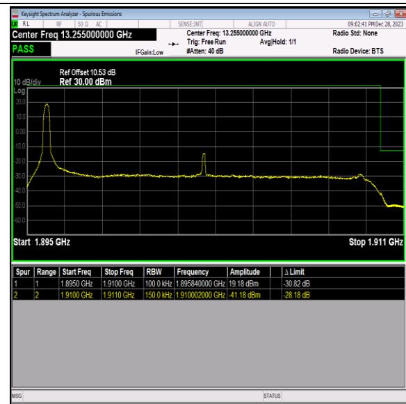
Band2_15MHz_16QAM_19125_1RB#0
