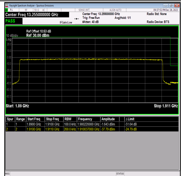
Band2_20MHz_QPSK_19100_100RB#0
