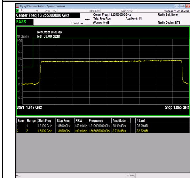
Band2_15MHz_64QAM_18675_75RB#0
