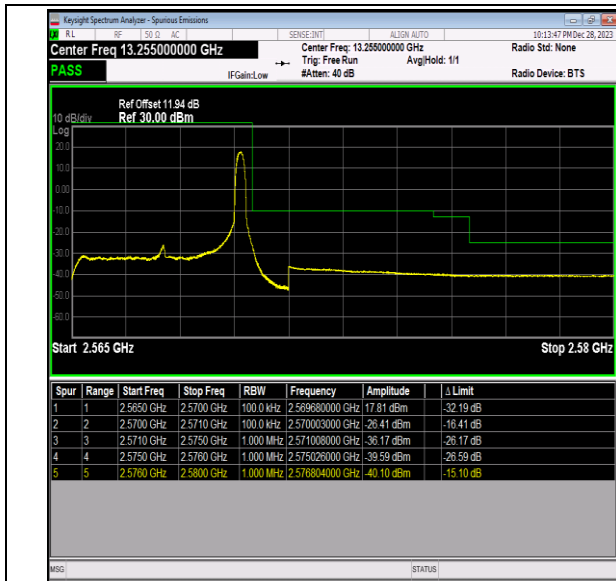
Band7_5MHz_64QAM_21425_1RB#24
