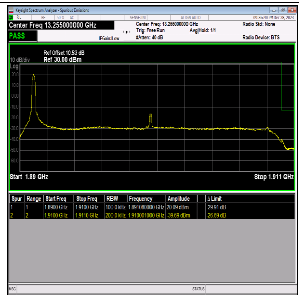
Band2_20MHz_QPSK_19100_1RB#0
