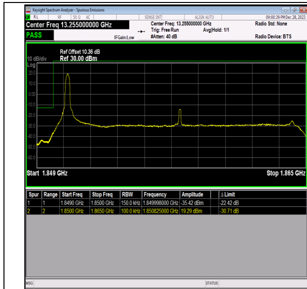
Band2_15MHz_QPSK_18675_1RB#0
