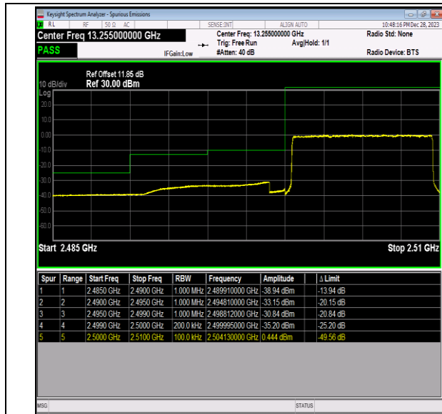
Band7_10MHz_QPSK_20800_50RB#0
