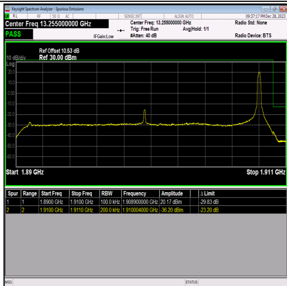
Band2_20MHz_QPSK_19100_1RB#99
