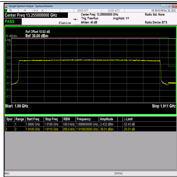
Band2_20MHz_16QAM_19100_100RB#0
