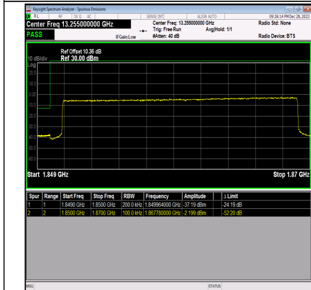
Band2_20MHz_16QAM_18700_100RB#0
