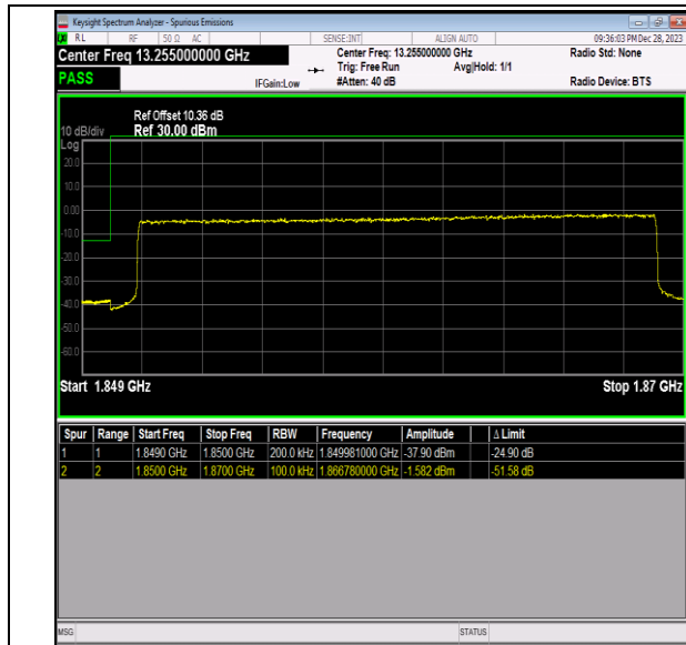
Band2_20MHz_QPSK_18700_100RB#0
