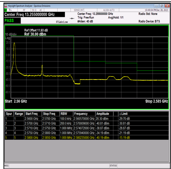
Band7_10MHz_QPSK_21400_1RB#0
