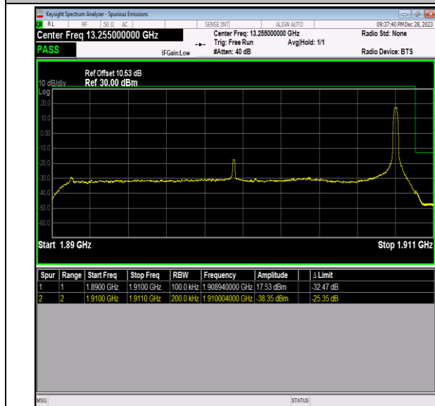
Band2_20MHz_64QAM_19100_1RB#99
