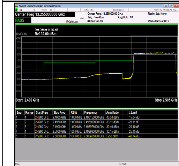
Band7_5MHz_QPSK_20775_25RB#0
