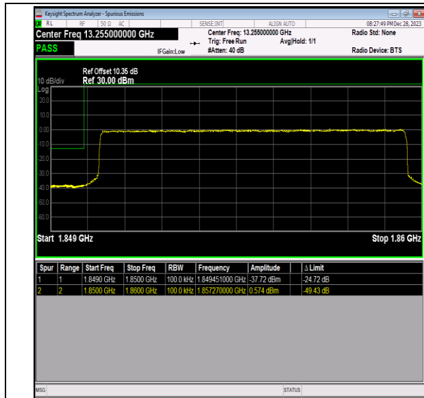
Band2_10MHz_QPSK_18650_50RB#0
