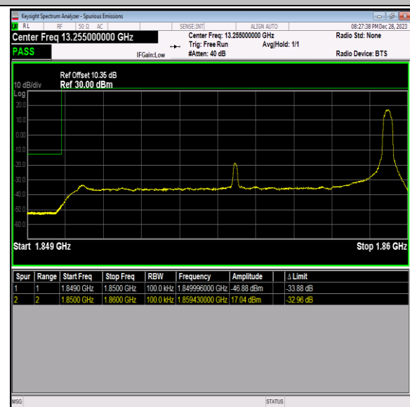
Band2_10MHz_64QAM_18650_1RB#49
