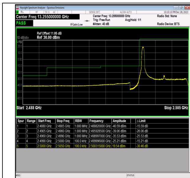
Band7_5MHz_QPSK_20775_1RB#0
