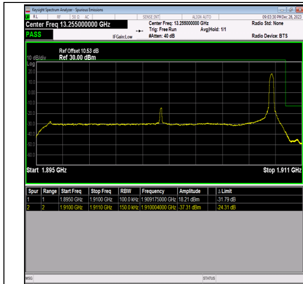
Band2_15MHz_64QAM_19125_1RB#74
