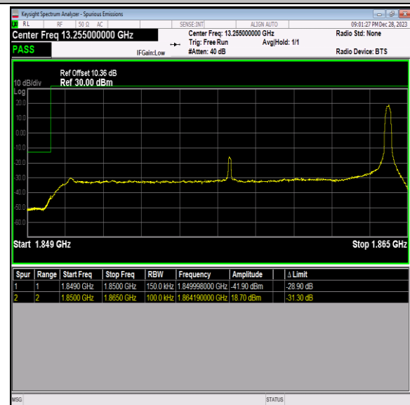
Band2_15MHz_16QAM_18675_1RB#74
