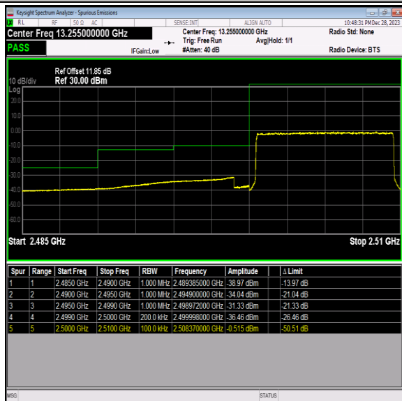
Band7_10MHz_16QAM_20800_50RB#0
