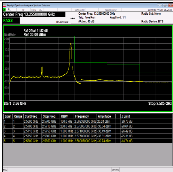
Band7_10MHz_QPSK_21400_1RB#49
