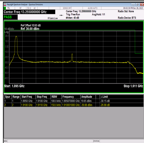
Band2_15MHz_QPSK_19125_1RB#0
