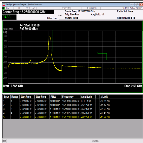
Band7_5MHz_16QAM_21425_1RB#24
