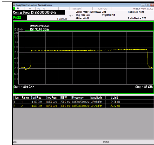
Band2_20MHz_64QAM_18700_100RB#0
