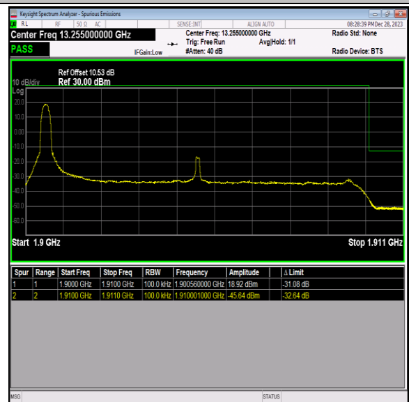
Band2_10MHz_16QAM_19150_1RB#0
