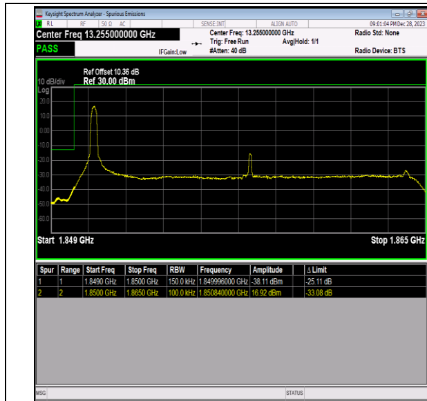
Band2_15MHz_64QAM_18675_1RB#0
