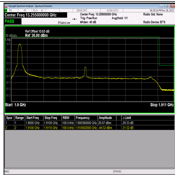
Band2_10MHz_QPSK_19150_1RB#0
