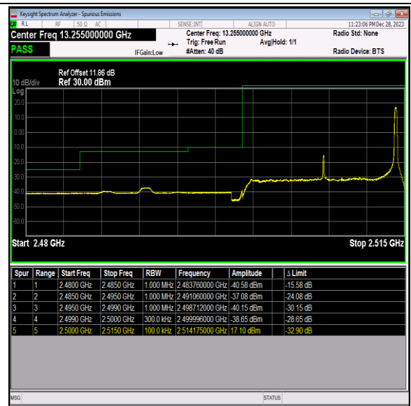
Band7_15MHz_64QAM_20825_1RB#74
