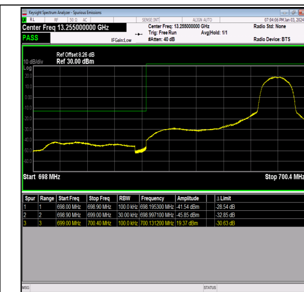
Band12_1.4MHz_64QAM_23017_1RB#5
