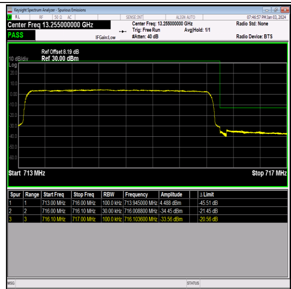
Band12_3MHz_16QAM_23165_15RB#0
