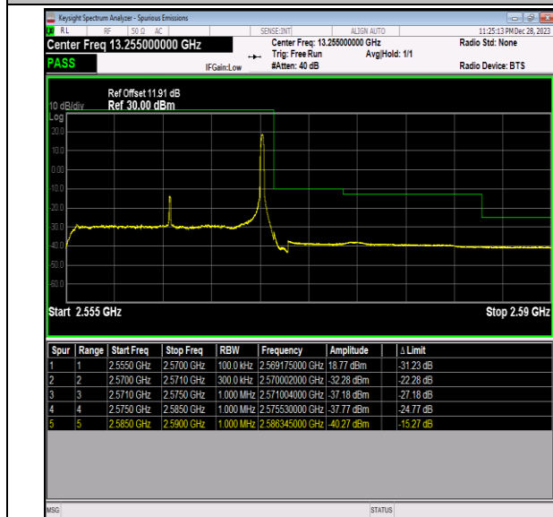
Band7_15MHz_16QAM_21375_1RB#74
