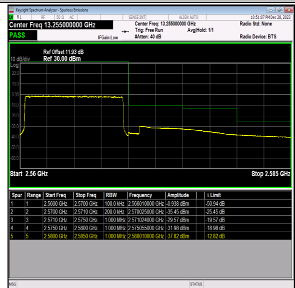
Band7_10MHz_64QAM_21400_50RB#0
