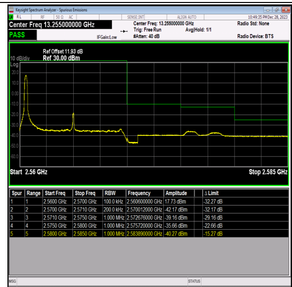
Band7_10MHz_64QAM_21400_1RB#0
