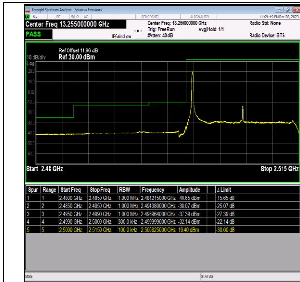
Band7_15MHz_QPSK_20825_1RB#0
