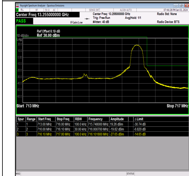
Band12_3MHz_64QAM_23165_1RB#14
