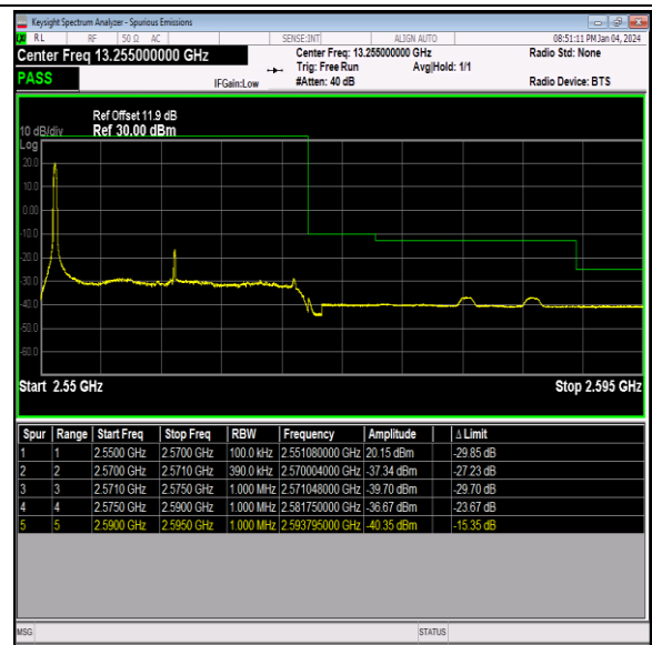
Band7_20MHz_64QAM_21350_1RB#0
