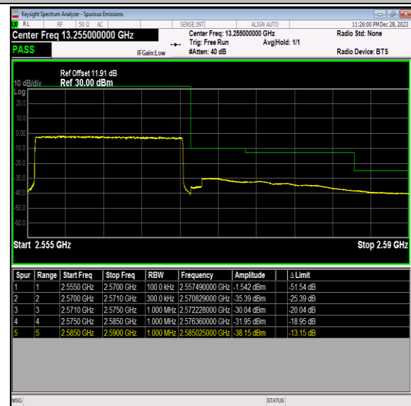
Band7_15MHz_16QAM_21375_75RB#0
