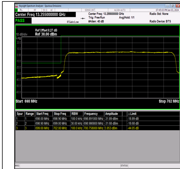
Band12_3MHz_64QAM_23025_15RB#0
