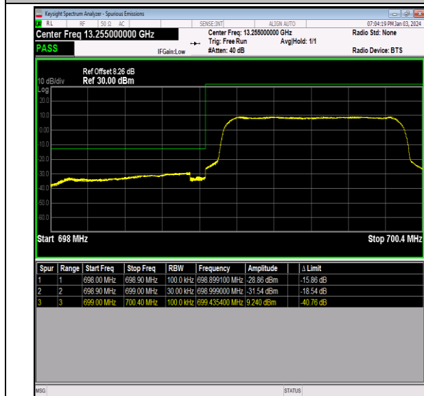
Band12_1.4MHz_QPSK_23017_6RB#0
