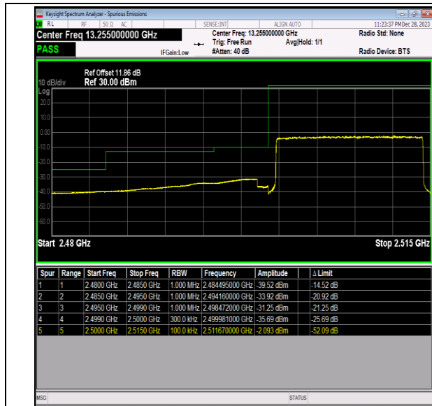
Band7_15MHz_16QAM_20825_75RB#0
