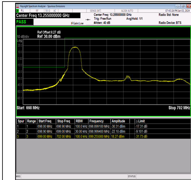
Band12_3MHz_16QAM_23025_1RB#0
