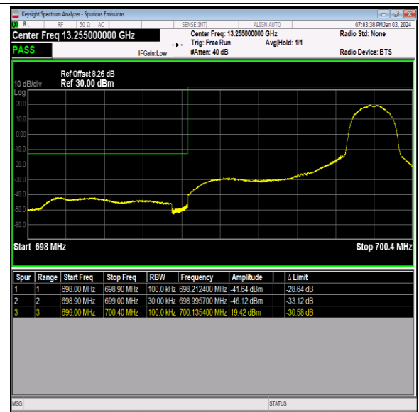
Band12_1.4MHz_QPSK_23017_1RB#5
