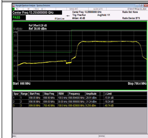
Band12_1.4MHz_64QAM_23017_6RB#0
