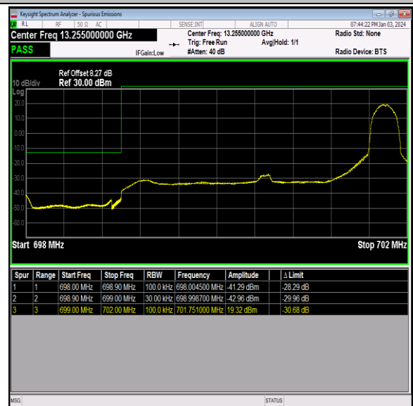
Band12_3MHz_64QAM_23025_1RB#14
