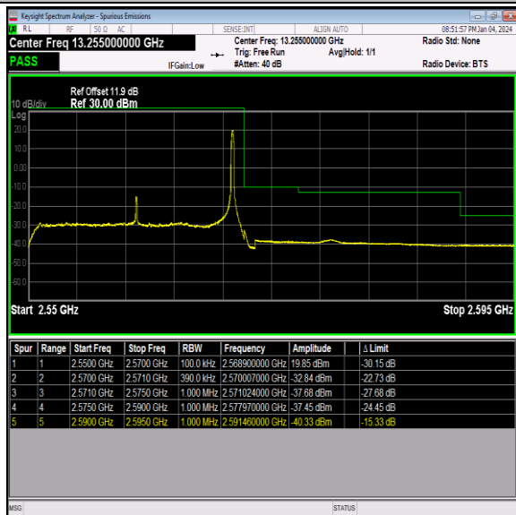
Band7_20MHz_64QAM_21350_1RB#99
