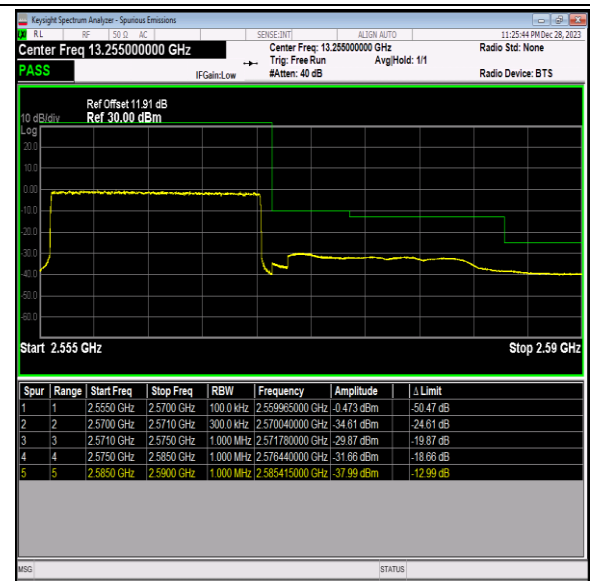
Band7_15MHz_QPSK_21375_75RB#0
