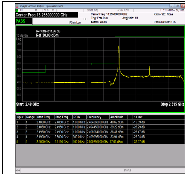
Band7_15MHz_64QAM_20825_1RB#0
