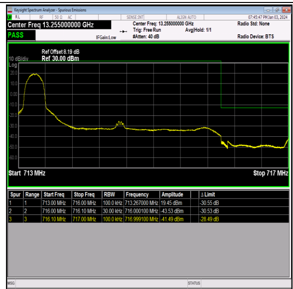
Band12_3MHz_64QAM_23165_1RB#0
