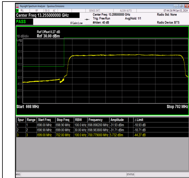
Band12_3MHz_QPSK_23025_15RB#0
