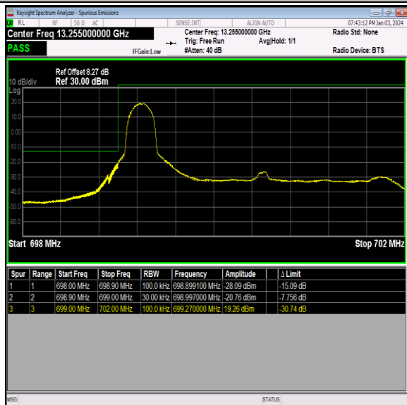
Band12_3MHz_QPSK_23025_1RB#0
