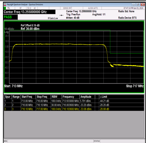
Band12_3MHz_64QAM_23165_15RB#0
