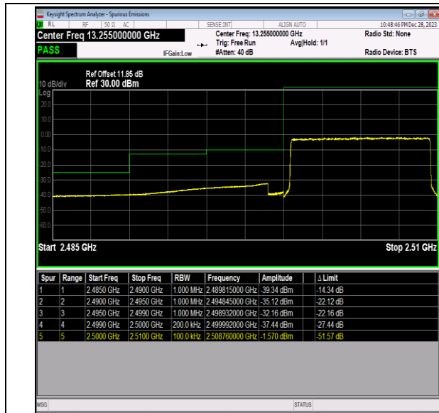
Band7_10MHz_64QAM_20800_50RB#0
