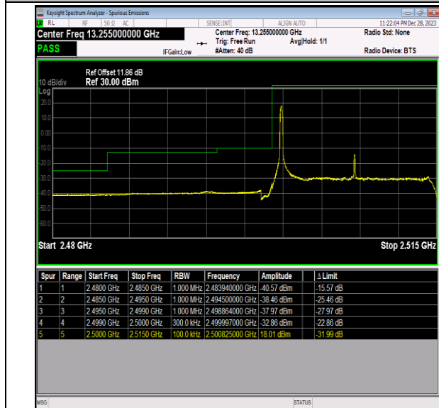
Band7_15MHz_16QAM_20825_1RB#0
