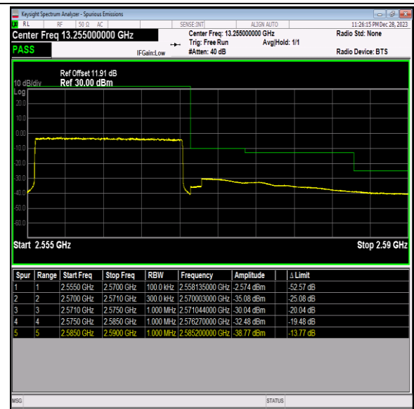
Band7_15MHz_64QAM_21375_75RB#0
