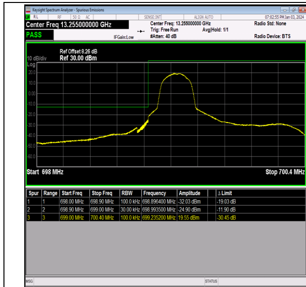
Band12_1.4MHz_QPSK_23017_1RB#0
