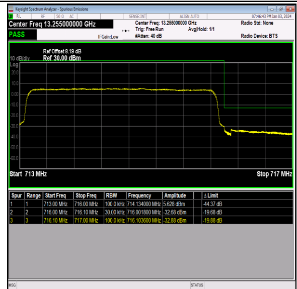
Band12_3MHz_QPSK_23165_15RB#0
