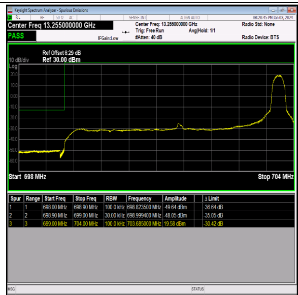
Band12_5MHz_QPSK_23035_1RB#24
