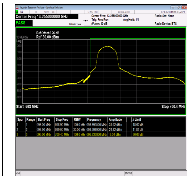
Band12_1.4MHz_64QAM_23017_1RB#0
