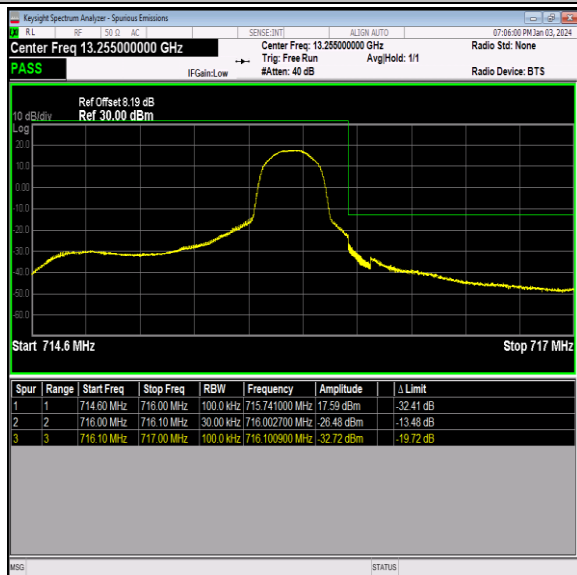
Band12_1.4MHz_16QAM_23173_1RB#5
