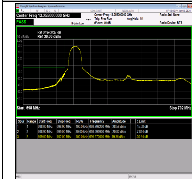
Band12_3MHz_64QAM_23025_1RB#0
