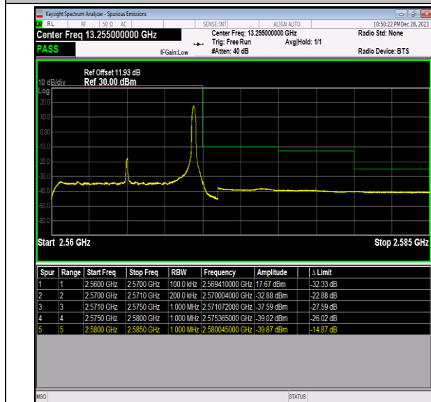
Band7_10MHz_64QAM_21400_1RB#49
