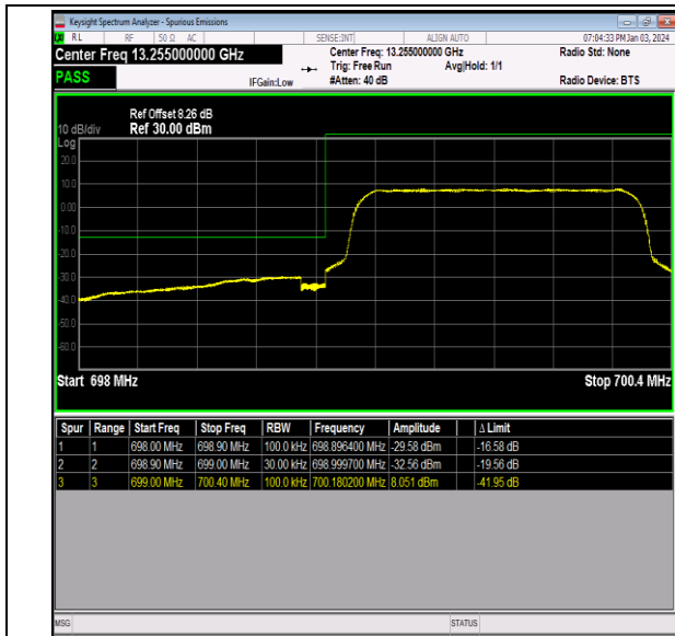
Band12_1.4MHz_16QAM_23017_6RB#0
