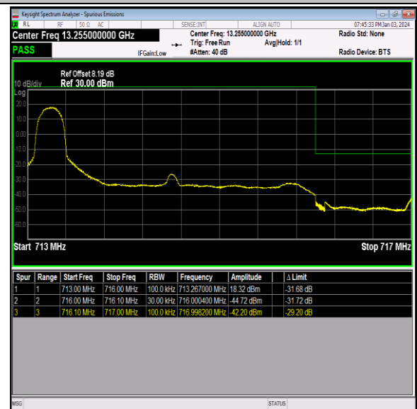
Band12_3MHz_16QAM_23165_1RB#0
