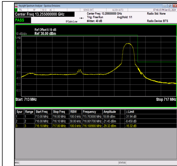
Band12_3MHz_16QAM_23165_1RB#14
