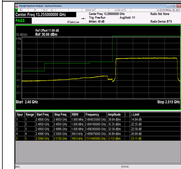
Band7_15MHz_64QAM_20825_75RB#0
