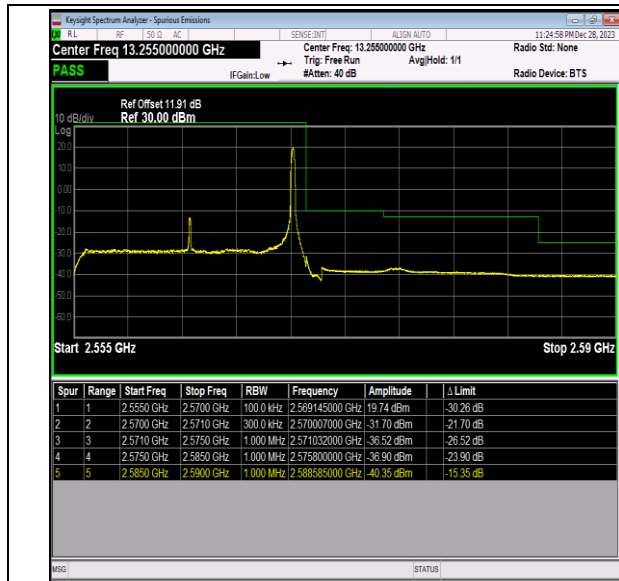
Band7_15MHz_QPSK_21375_1RB#74
