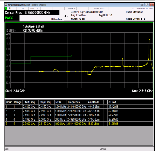
Band7_15MHz_16QAM_20825_1RB#74
