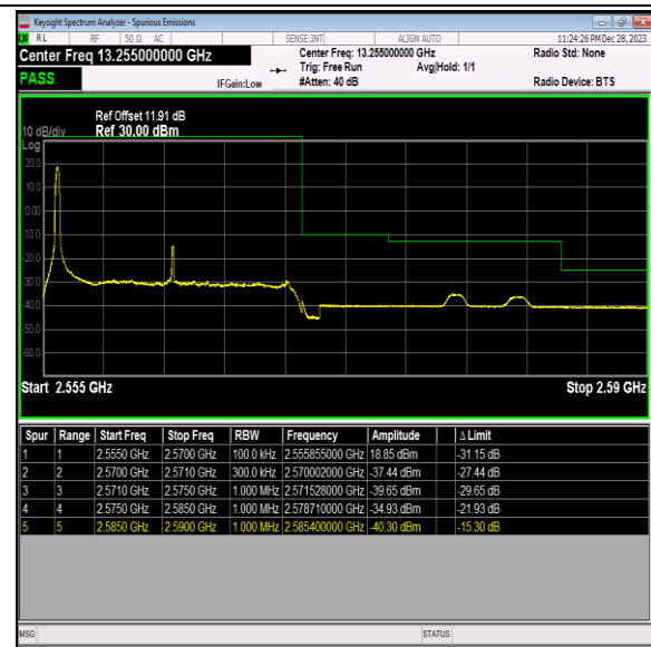
Band7_15MHz_16QAM_21375_1RB#0
