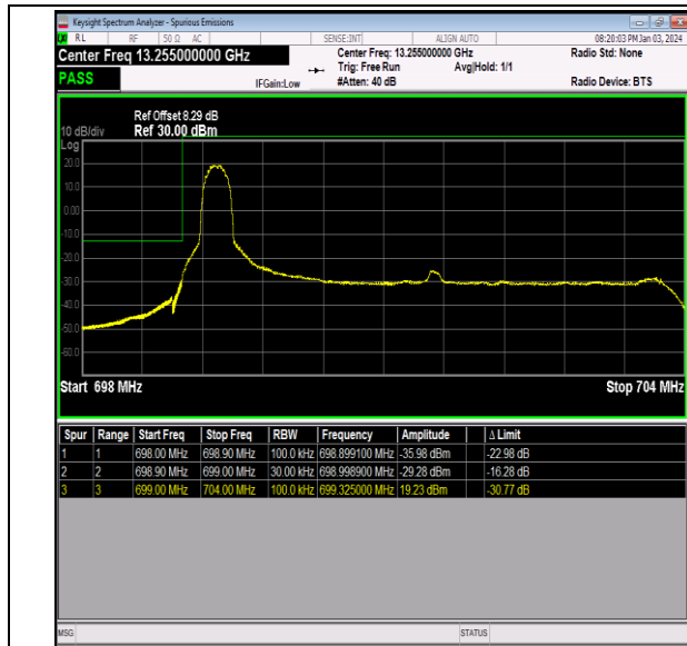
Band12_5MHz_QPSK_23035_1RB#0
