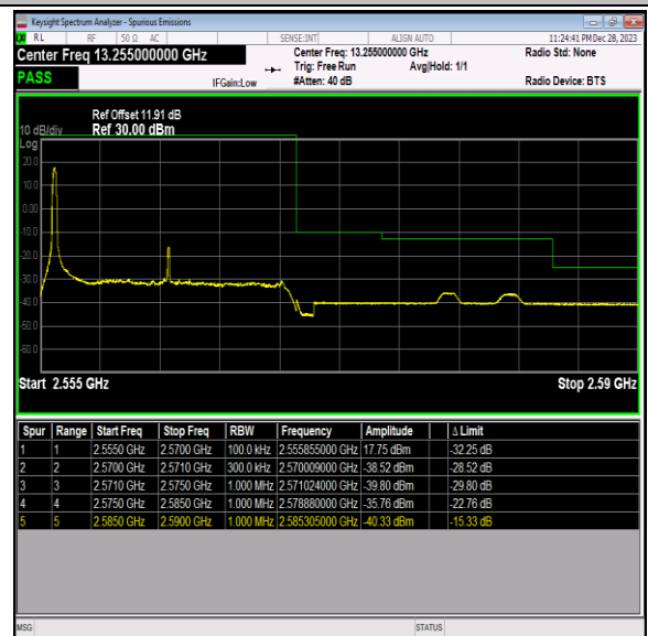
Band7_15MHz_64QAM_21375_1RB#0
