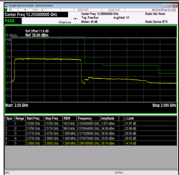
Band7_20MHz_64QAM_21350_100RB#0
