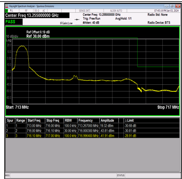
Band12_3MHz_QPSK_23165_1RB#0
