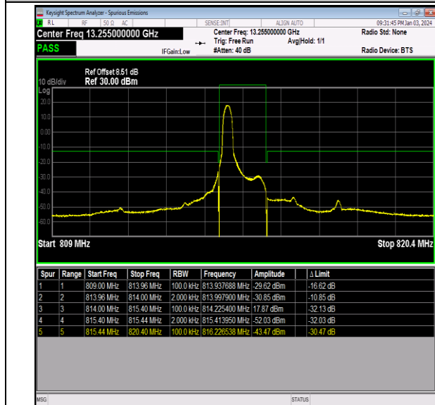
Band26_1.4MHz_16QAM_26697_1RB#0
