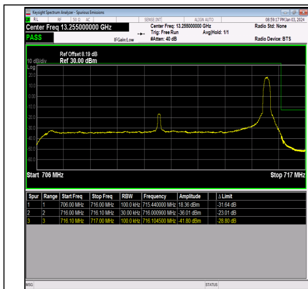
Band12_10MHz_16QAM_23130_1RB#49
