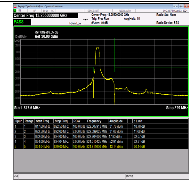
Band26_1.4MHz_16QAM_26783_1RB#0
