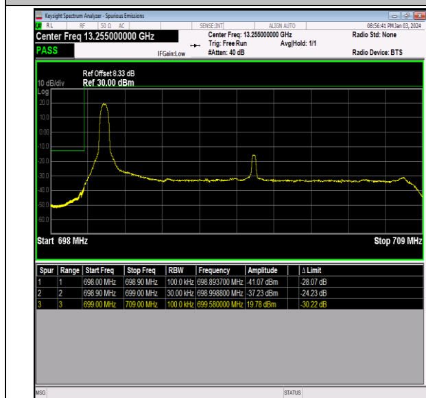
Band12_10MHz_64QAM_23060_1RB#0
