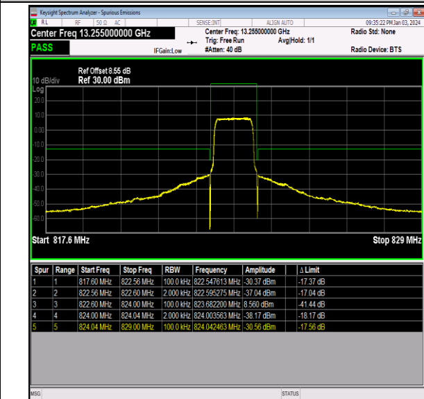
Band26_1.4MHz_16QAM_26783_6RB#0
