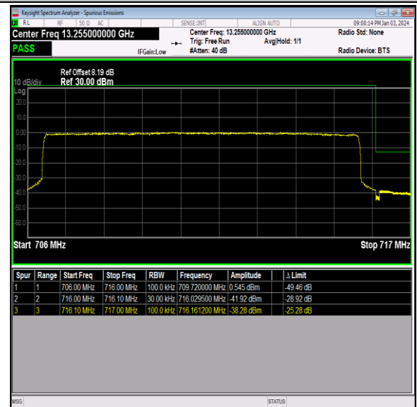
Band12_10MHz_64QAM_23130_50RB#0
