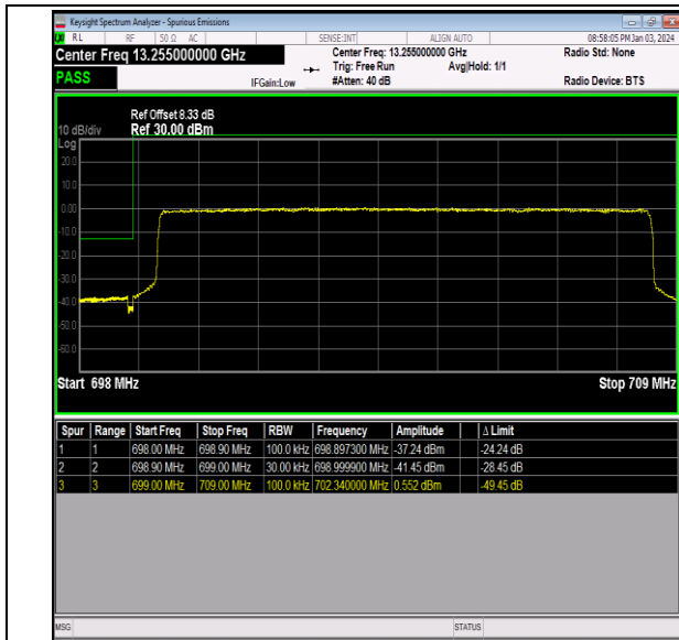
Band12_10MHz_64QAM_23060_50RB#0
