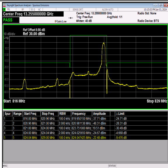
Band26_3MHz_64QAM_26775_1RB#14
