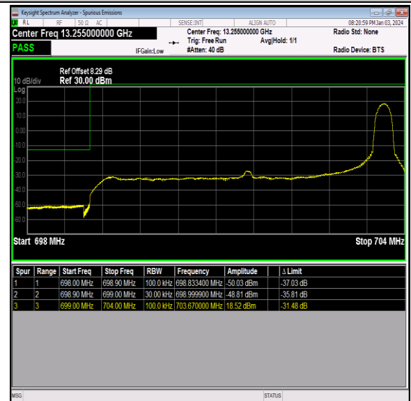
Band12_5MHz_16QAM_23035_1RB#24
