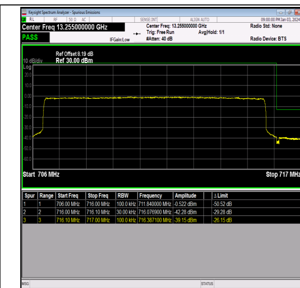
Band12_10MHz_16QAM_23130_50RB#0
