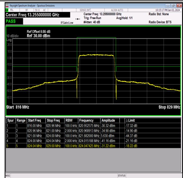
Band26_3MHz_QPSK_26775_15RB#0
