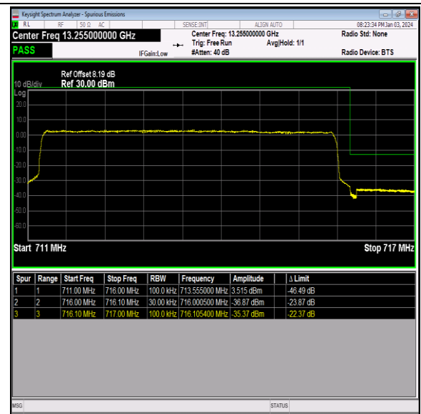
Band12_5MHz_QPSK_23155_25RB#0
