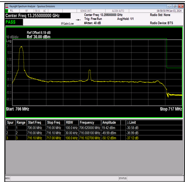
Band12_10MHz_64QAM_23130_1RB#0
