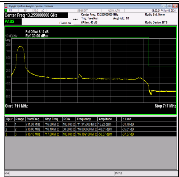
Band12_5MHz_16QAM_23155_1RB#0
