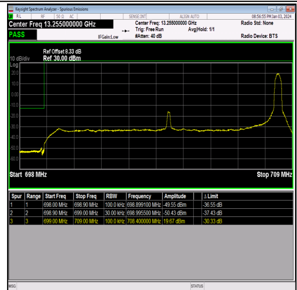
Band12_10MHz_QPSK_23060_1RB#49
