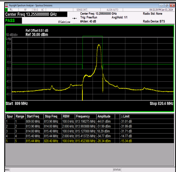
Band26_1.4MHz_16QAM_26697_1RB#5
