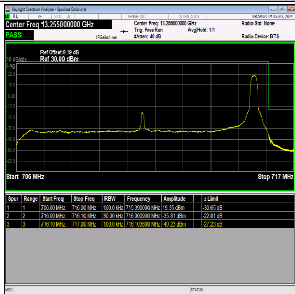
Band12_10MHz_QPSK_23130_1RB#49
