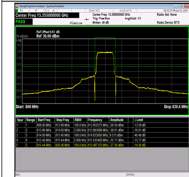
Band26_1.4MHz_QPSK_26697_6RB#0
