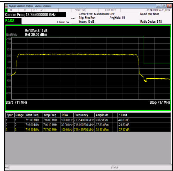
Band12_5MHz_64QAM_23155_25RB#0
