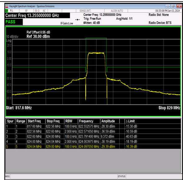
Band26_1.4MHz_QPSK_26783_6RB#0
