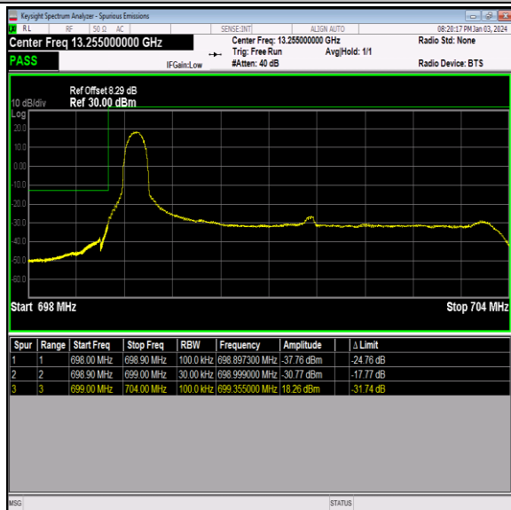
Band12_5MHz_16QAM_23035_1RB#0
