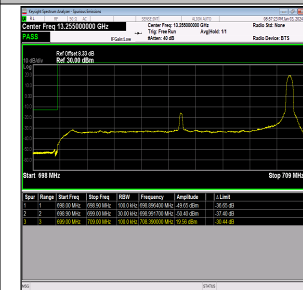
Band12_10MHz_64QAM_23060_1RB#49
