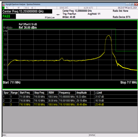
Band12_5MHz_16QAM_23155_1RB#24
