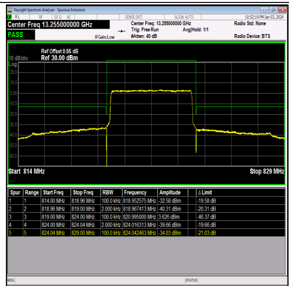
Band26_5MHz_QPSK_26765_25RB#0
