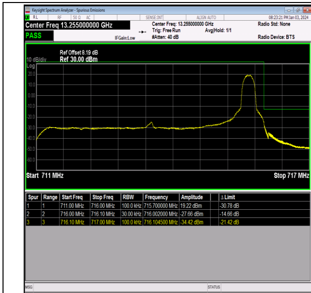
Band12_5MHz_64QAM_23155_1RB#24
