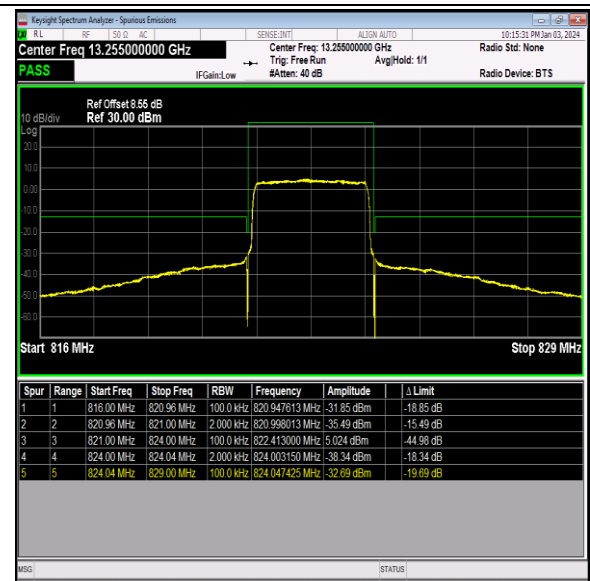
Band26_3MHz_16QAM_26775_15RB#0
