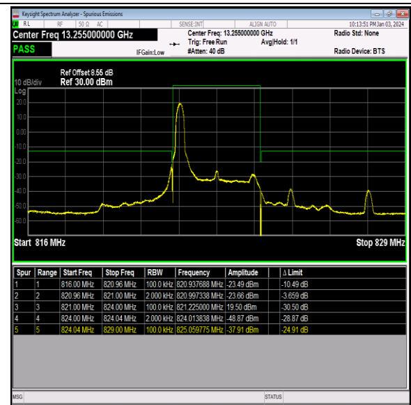
Band26_3MHz_QPSK_26775_1RB#0
