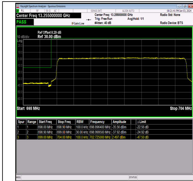
Band12_5MHz_16QAM_23035_25RB#0
