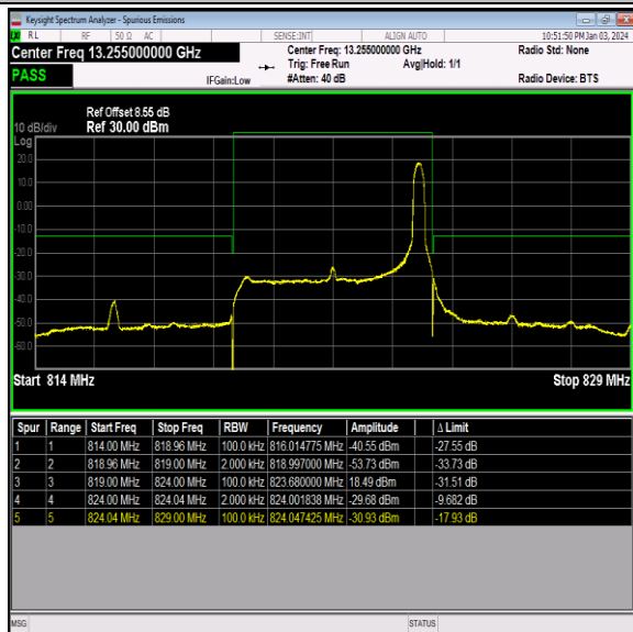
Band26_5MHz_16QAM_26765_1RB#24
