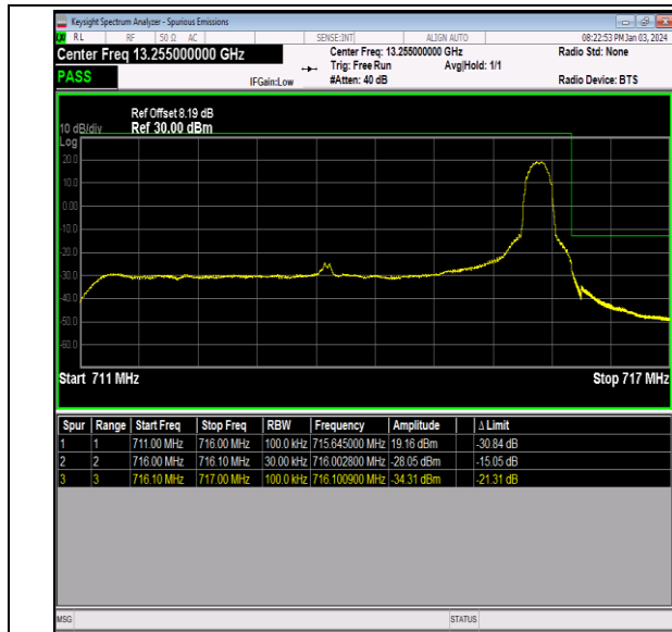
Band12_5MHz_QPSK_23155_1RB#24
