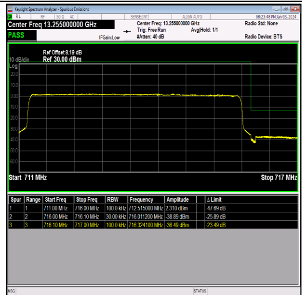
Band12_5MHz_16QAM_23155_25RB#0
