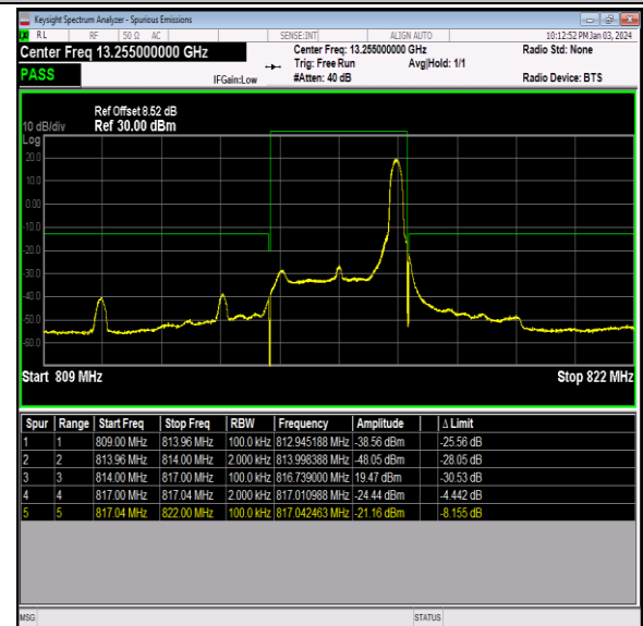
Band26_3MHz_64QAM_26705_1RB#14
