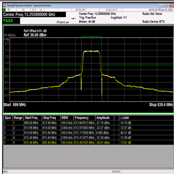
Band26_1.4MHz_64QAM_26697_6RB#0
