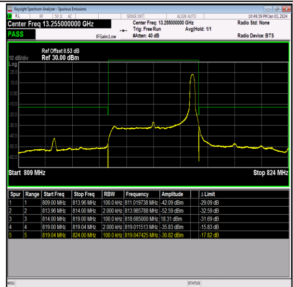
Band26_5MHz_16QAM_26715_1RB#24
