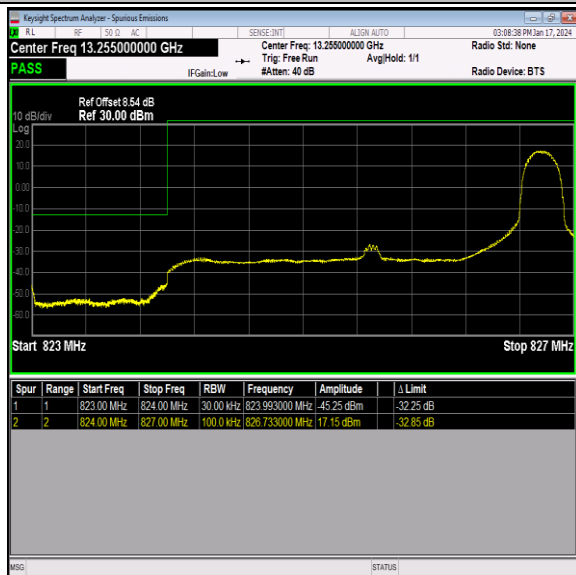
Band26_3MHz_64QAM_26805_1RB#14
