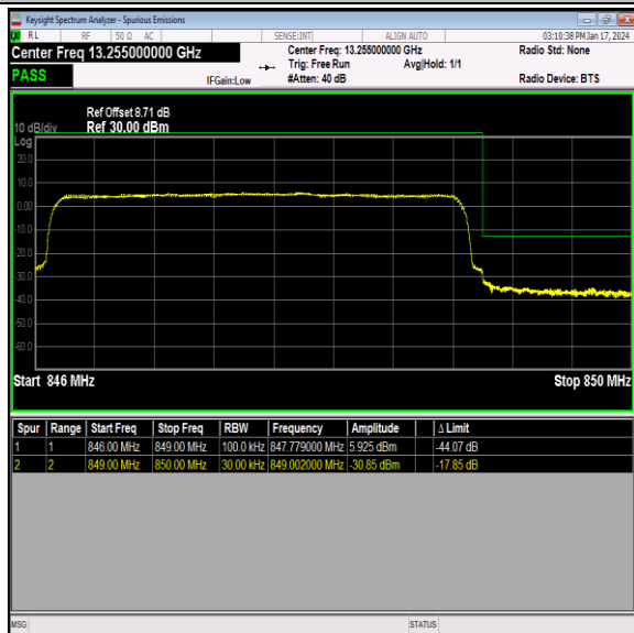
Band26_3MHz_QPSK_27025_15RB#0
