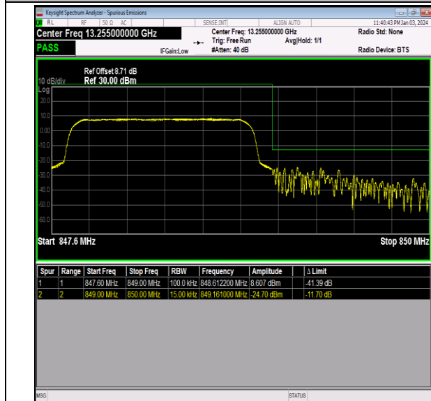
Band26_1.4MHz_16QAM_27033_6RB#0
