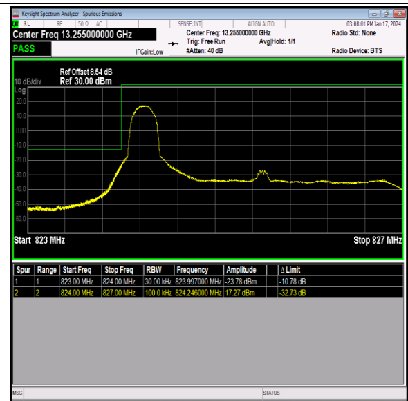
Band26_3MHz_64QAM_26805_1RB#0
