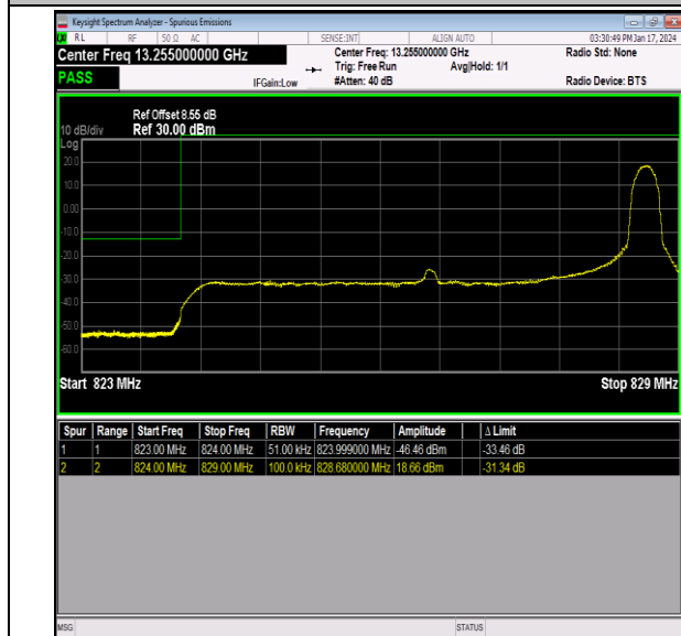
Band26_5MHz_16QAM_26815_1RB#24
