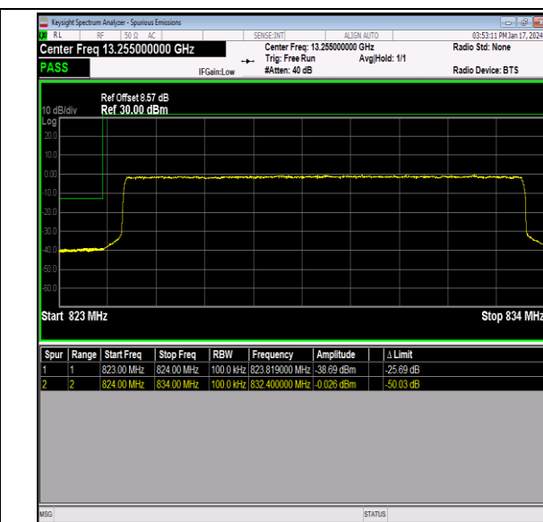
Band26_10MHz_16QAM_26840_50RB#0
