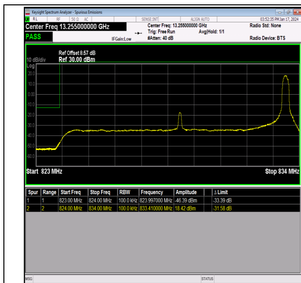
Band26_10MHz_16QAM_26840_1RB#49
