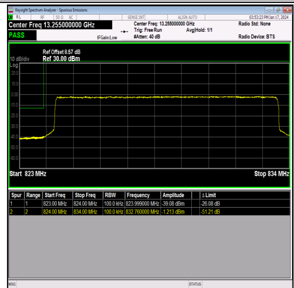
Band26_10MHz_64QAM_26840_50RB#0
