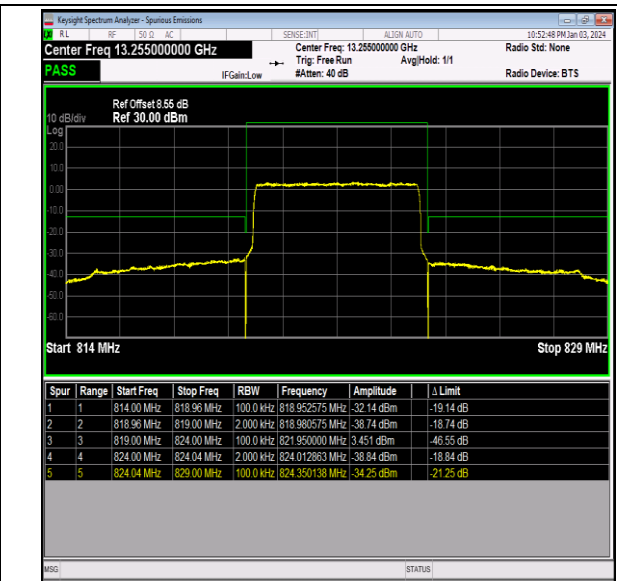
Band26_5MHz_64QAM_26765_25RB#0
