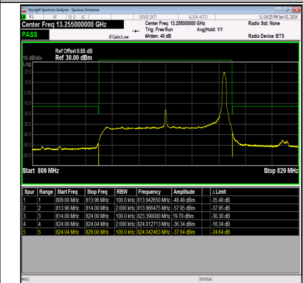
Band26_10MHz_QPSK_26740_1RB#49
