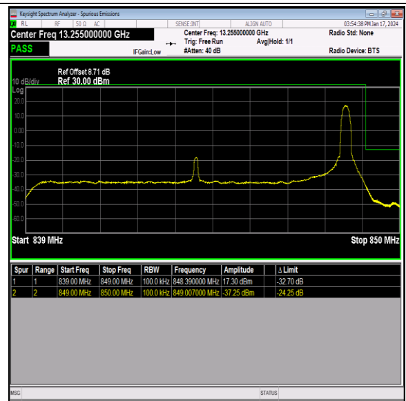
Band26_10MHz_64QAM_26990_1RB#49
