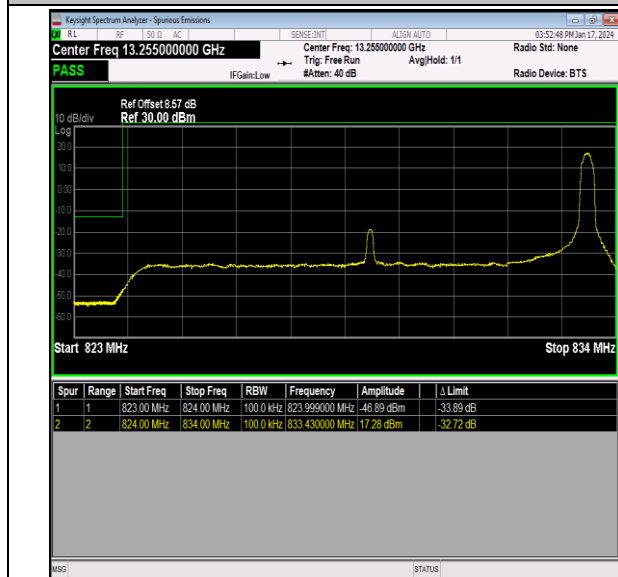
Band26_10MHz_64QAM_26840_1RB#49
