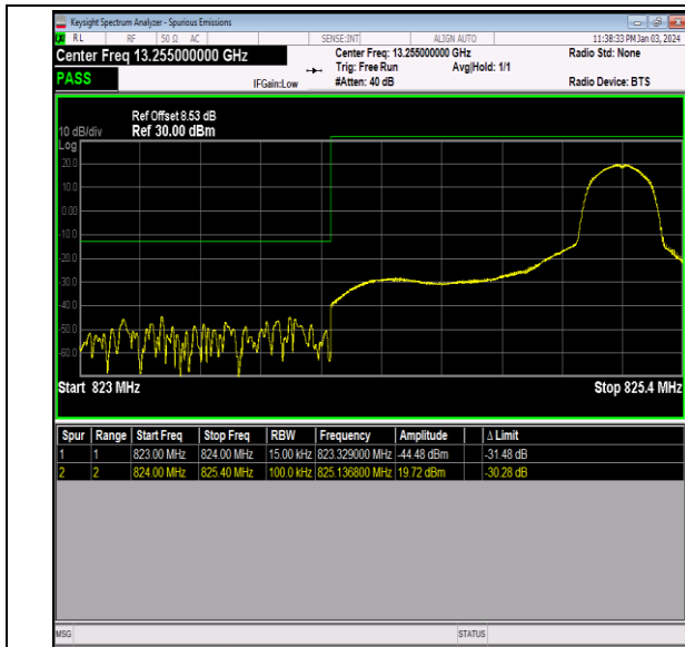
Band26_1.4MHz_QPSK_26797_1RB#5
