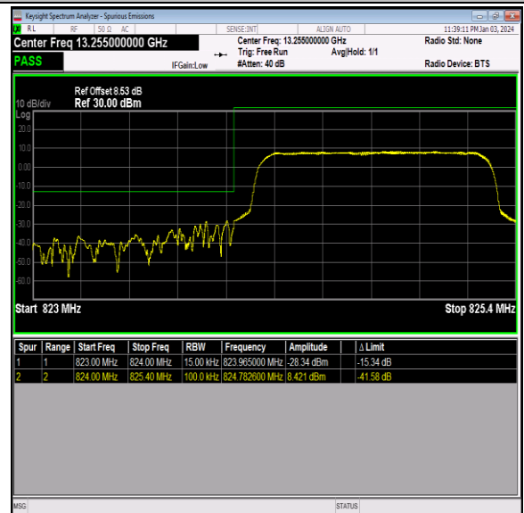
Band26_1.4MHz_16QAM_26797_6RB#0
