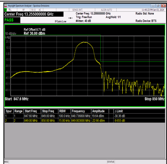
Band26_1.4MHz_64QAM_27033_1RB#5
