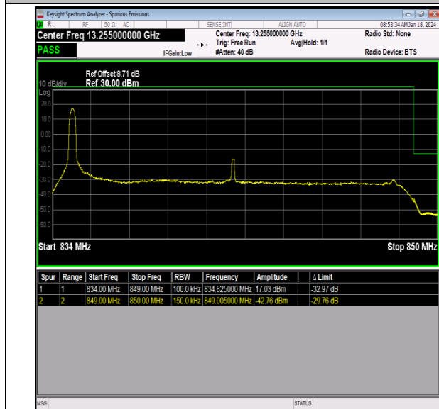
Band26_15MHz_64QAM_26965_1RB#0
