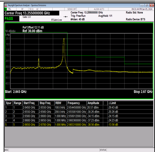
Band41_10MHz_QPSK_41190_1RB#49
