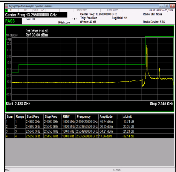
Band41_10MHz_64QAM_40090_1RB#0
