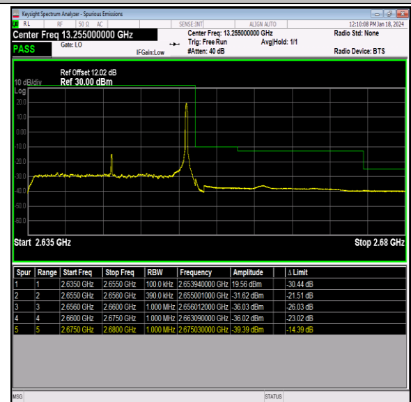
Band41_20MHz_QPSK_41140_1RB#99
