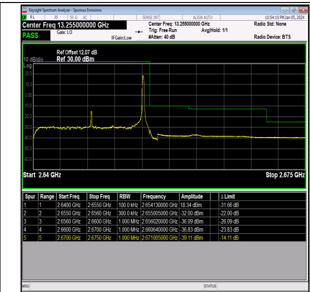
Band41_15MHz_64QAM_41165_1RB#74
