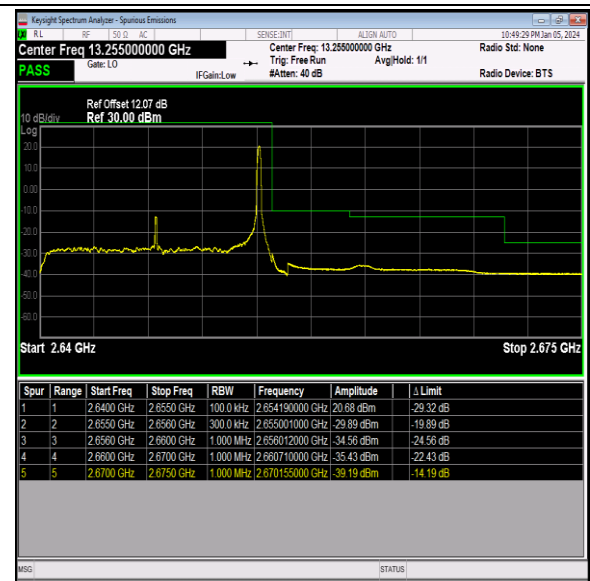
Band41_15MHz_QPSK_41165_1RB#74
