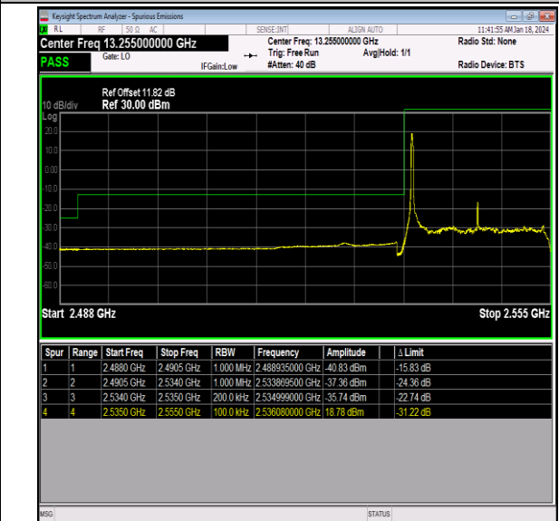
Band41_20MHz_QPSK_40140_1RB#0
