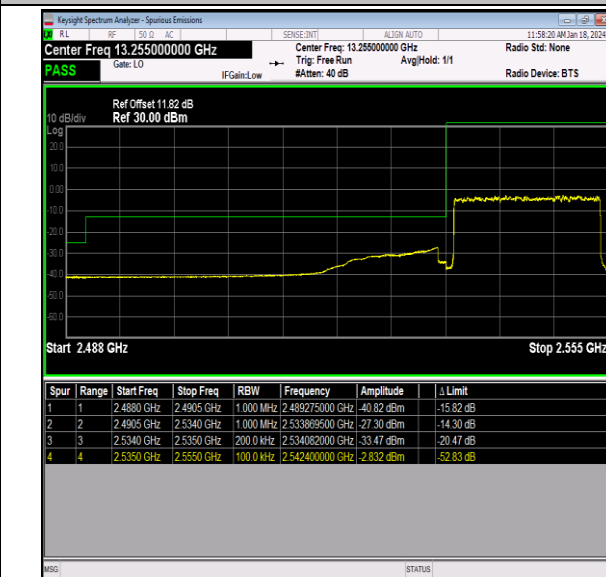
Band41_20MHz_16QAM_40140_100RB#0
