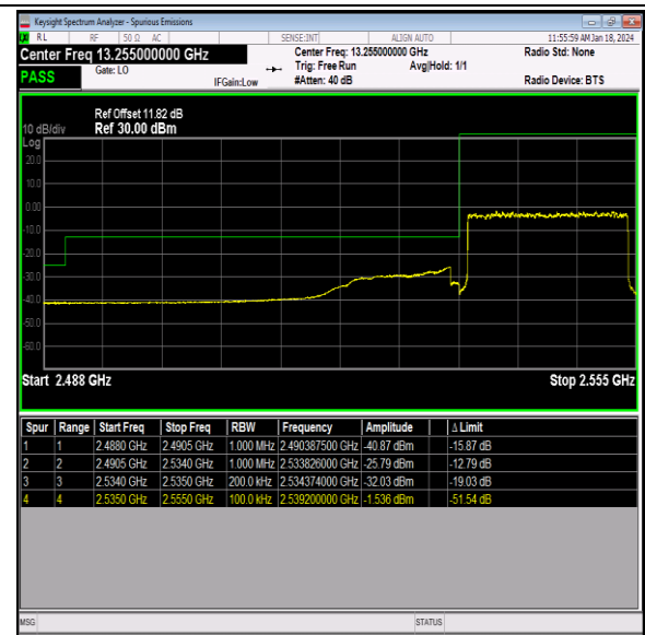
Band41_20MHz_QPSK_40140_100RB#0
