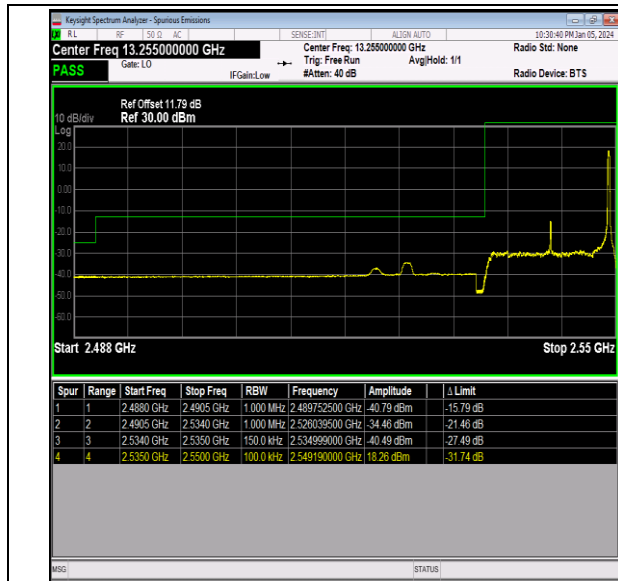
Band41_15MHz_16QAM_40115_1RB#74
