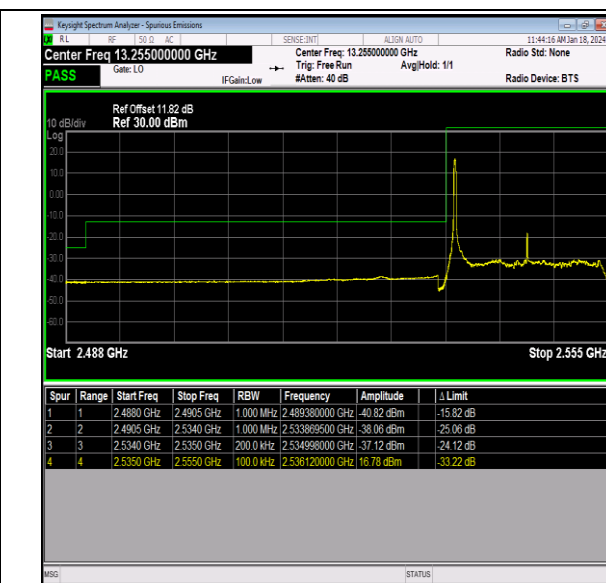
Band41_20MHz_16QAM_40140_1RB#0
