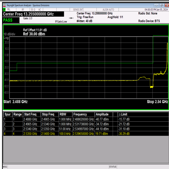
Band41_5MHz_QPSK_40065_1RB#24
