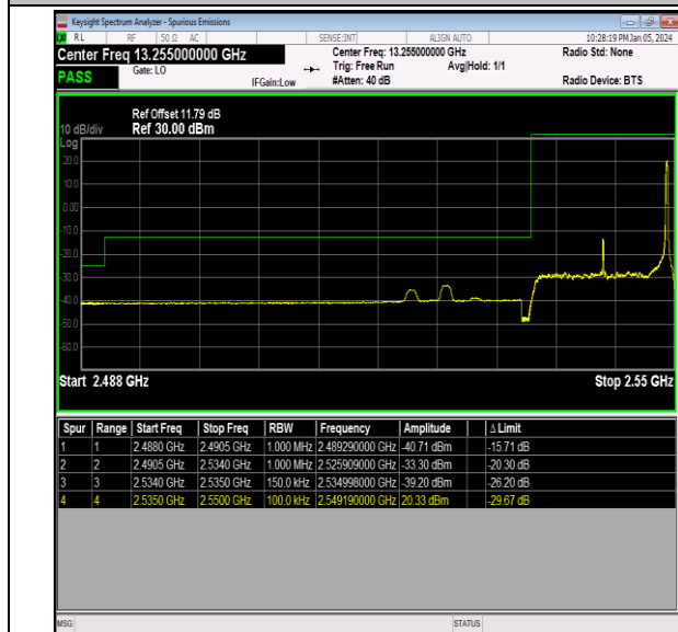
Band41_15MHz_QPSK_40115_1RB#74
