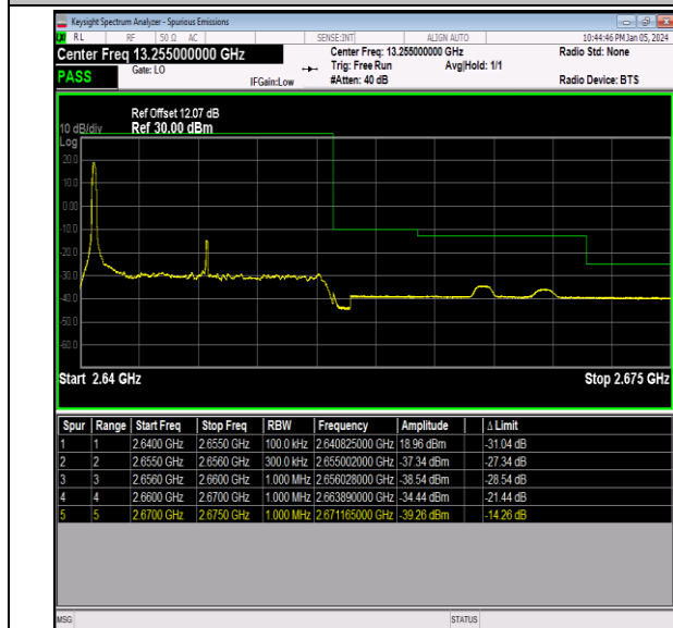
Band41_15MHz_16QAM_41165_1RB#0
