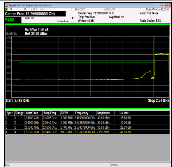
Band41_5MHz_64QAM_40065_25RB#0
