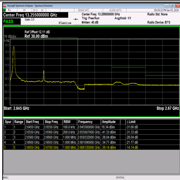
Band41_10MHz_64QAM_41190_1RB#0
