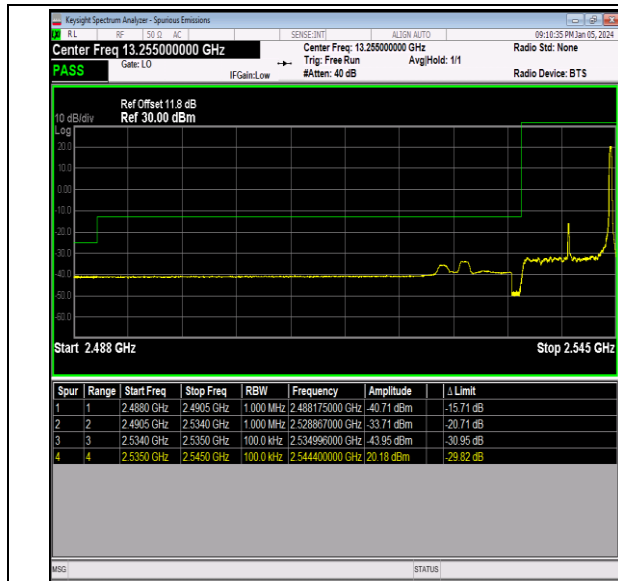
Band41_10MHz_QPSK_40090_1RB#49
