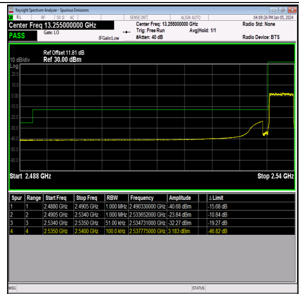
Band41_5MHz_16QAM_40065_25RB#0
