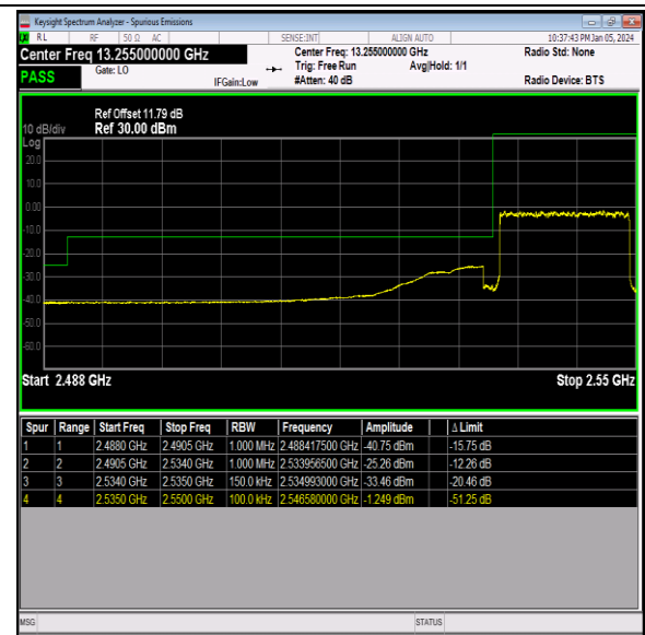
Band41_15MHz_16QAM_40115_75RB#0
