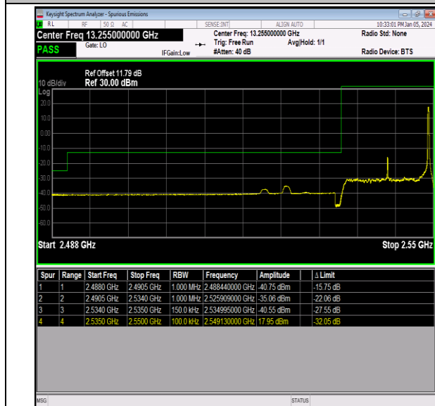
Band41_15MHz_64QAM_40115_1RB#74
