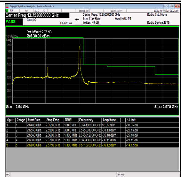
Band41_15MHz_16QAM_41165_1RB#74
