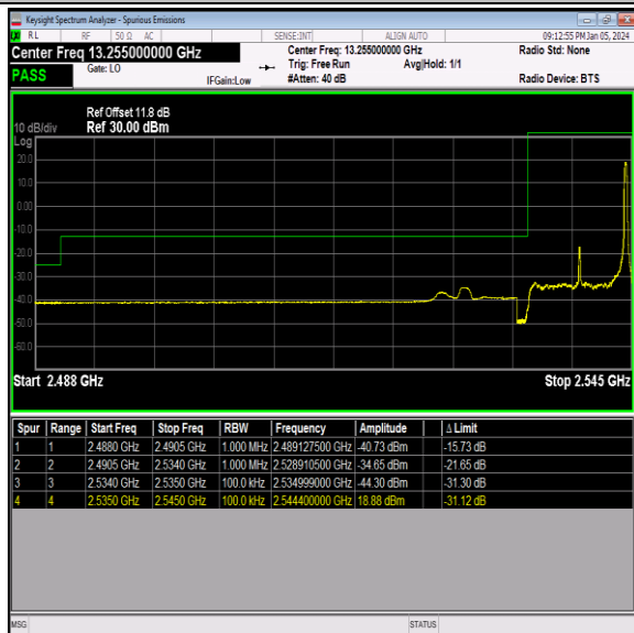
Band41_10MHz_16QAM_40090_1RB#49
