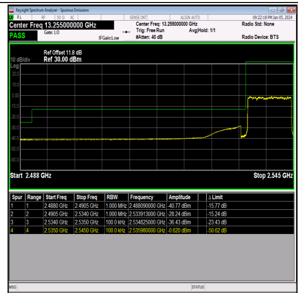
Band41_10MHz_64QAM_40090_50RB#0
