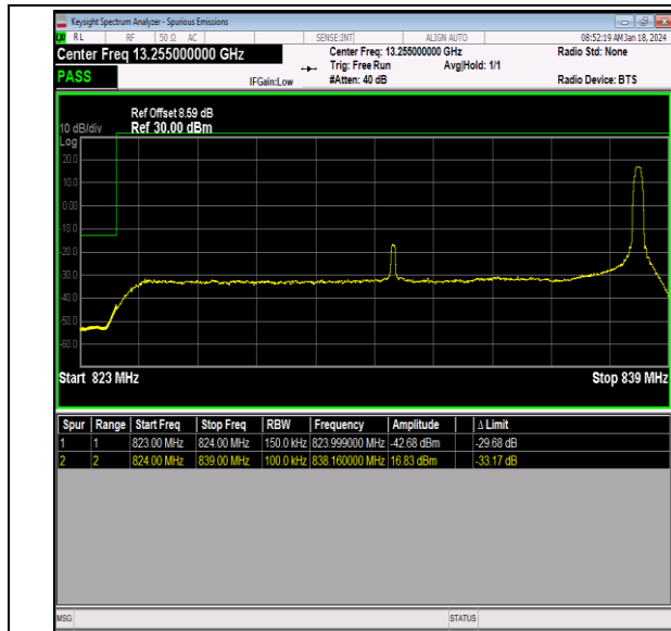
Band26_15MHz_64QAM_26865_1RB#74
