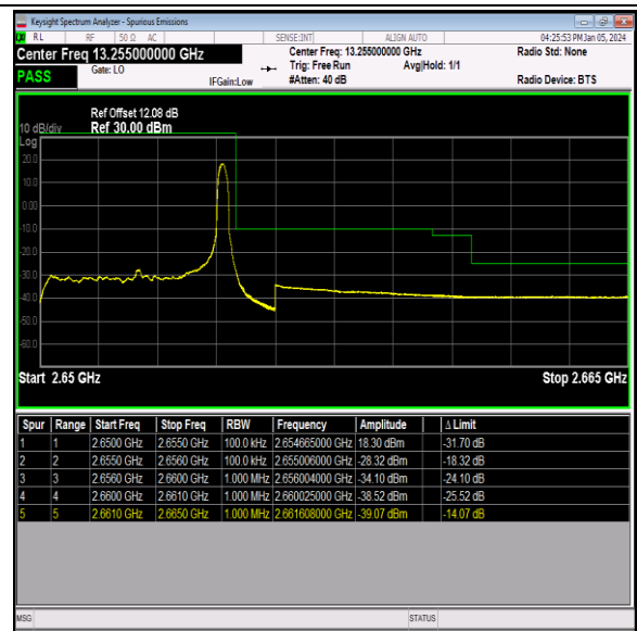
Band41_5MHz_64QAM_41215_1RB#24
