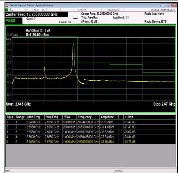
Band41_10MHz_64QAM_41190_1RB#49
