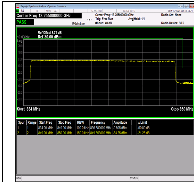
Band26_15MHz_QPSK_26965_75RB#0
