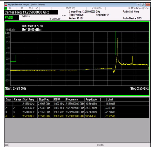
Band41_15MHz_16QAM_40115_1RB#0
