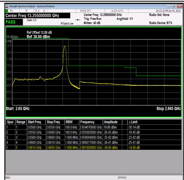
Band41_5MHz_16QAM_41215_1RB#24
