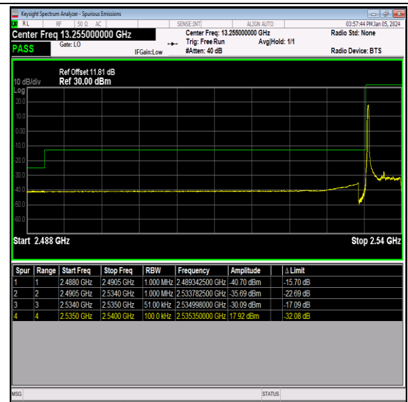
Band41_5MHz_64QAM_40065_1RB#0
