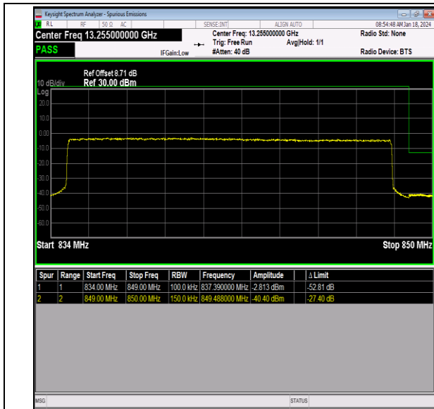
Band26_15MHz_64QAM_26965_75RB#0
