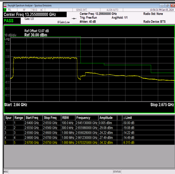
Band41_15MHz_QPSK_41165_75RB#0
