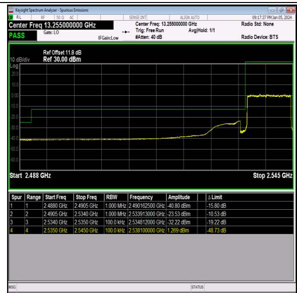
Band41_10MHz_QPSK_40090_50RB#0
