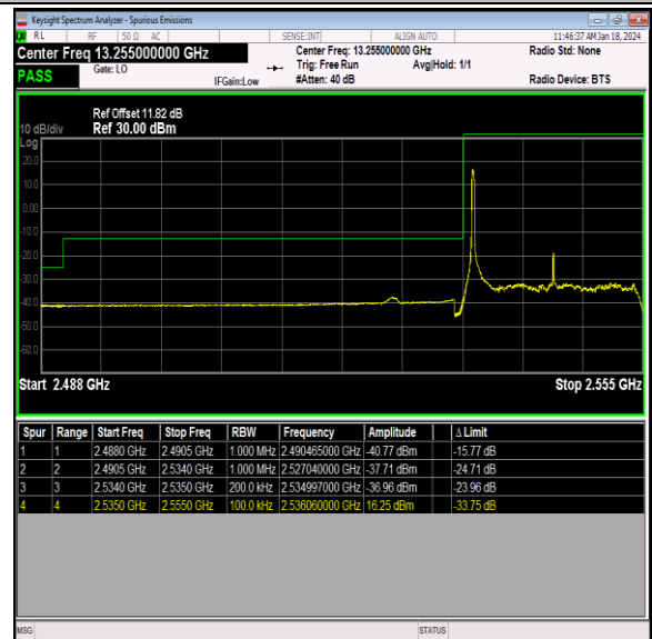
Band41_20MHz_64QAM_40140_1RB#0
