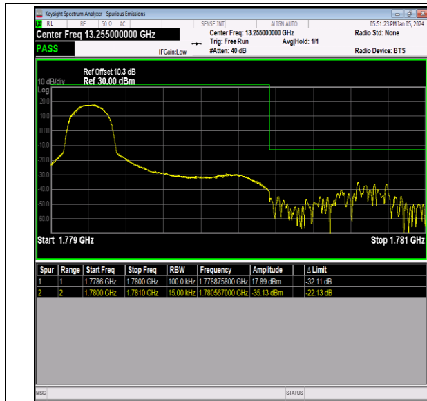
Band66_1.4MHz_64QAM_132665_1RB#0
