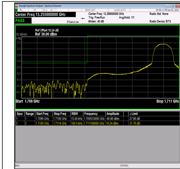
Band66_1.4MHz_16QAM_131979_1RB#5
