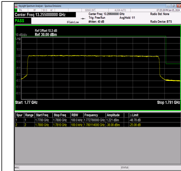
Band66_10MHz_QPSK_132622_50RB#0
