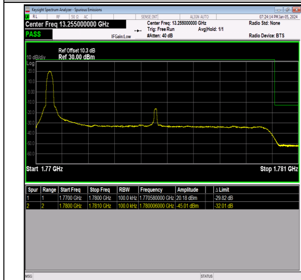
Band66_10MHz_QPSK_132622_1RB#0
