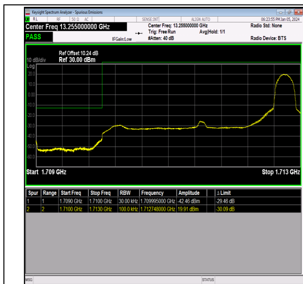
Band66_3MHz_QPSK_131987_1RB#14
