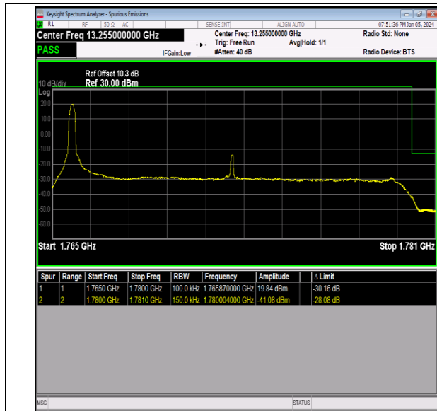
Band66_15MHz_QPSK_132597_1RB#0
