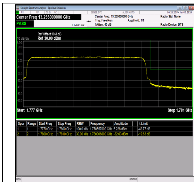
Band66_3MHz_QPSK_132657_15RB#0
