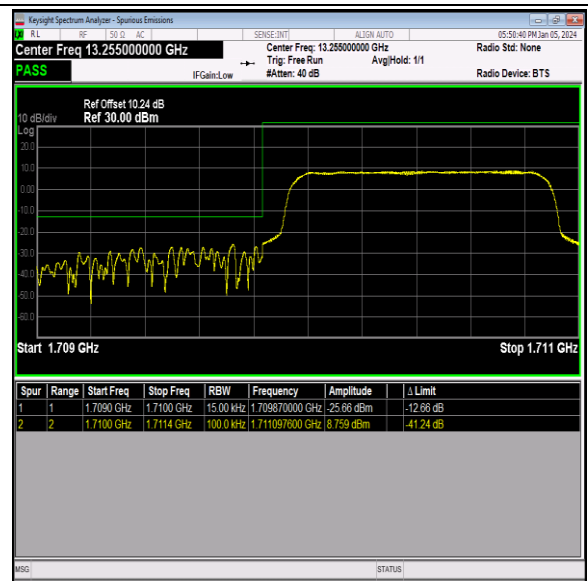
Band66_1.4MHz_16QAM_131979_6RB#0
