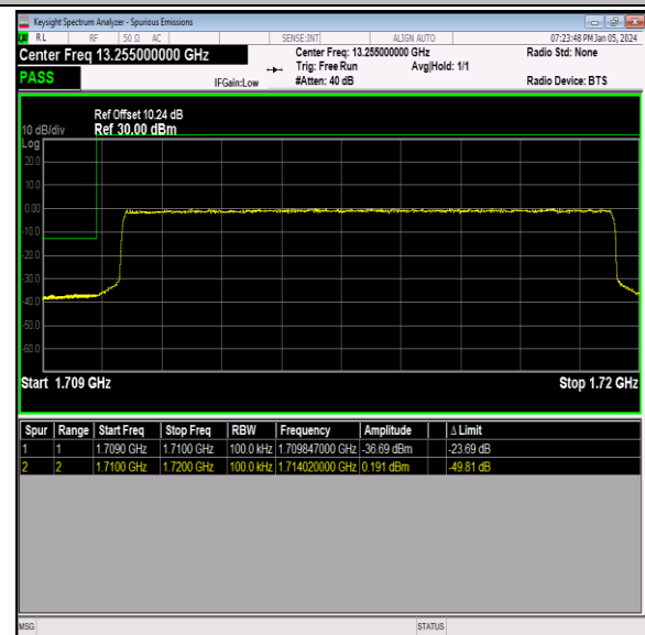
Band66_10MHz_16QAM_132022_50RB#0
