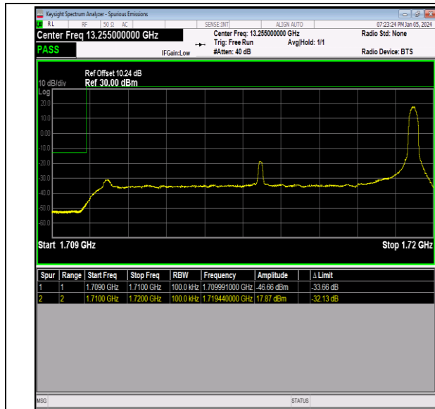
Band66_10MHz_64QAM_132022_1RB#49
