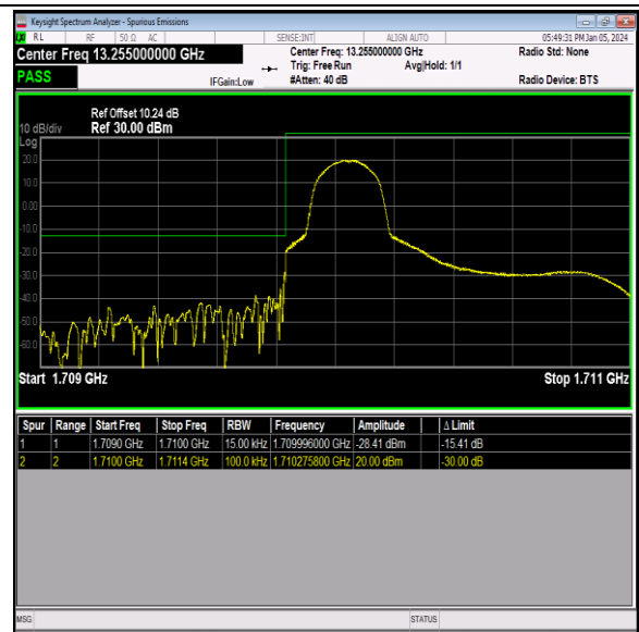
Band66_1.4MHz_QPSK_131979_1RB#0
