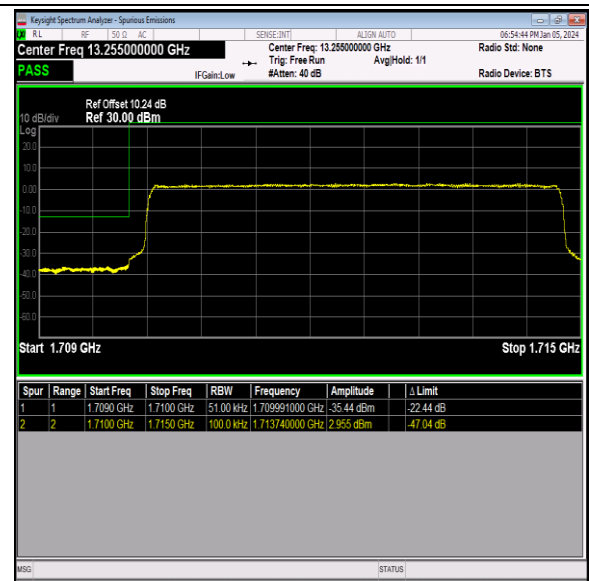
Band66_5MHz_16QAM_131997_25RB#0
