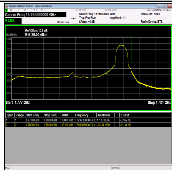
Band66_3MHz_64QAM_132657_1RB#14
