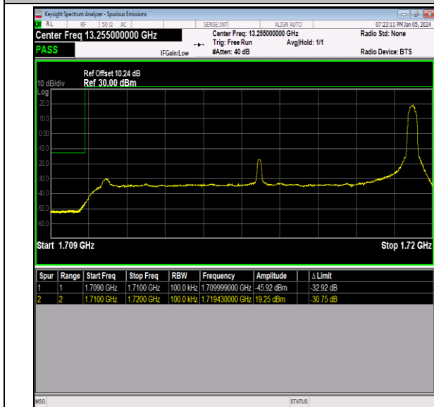
Band66_10MHz_16QAM_132022_1RB#49
