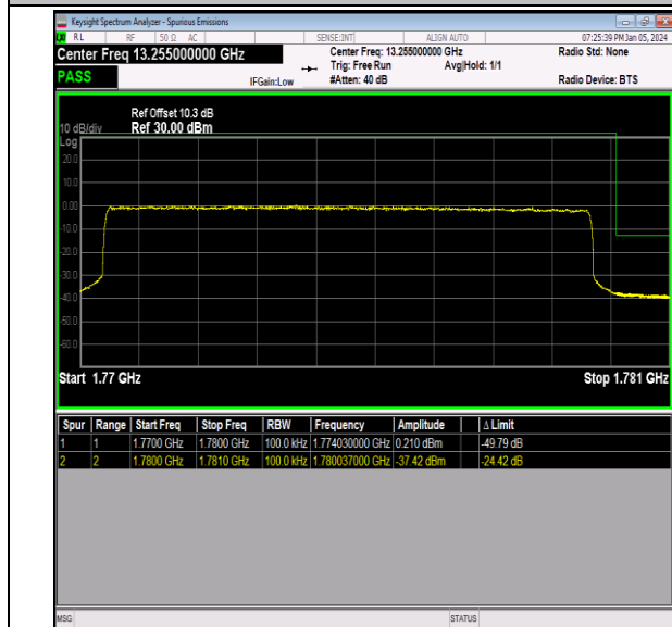
Band66_10MHz_16QAM_132622_50RB#0
