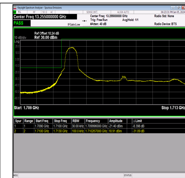
Band66_3MHz_16QAM_131987_1RB#0
