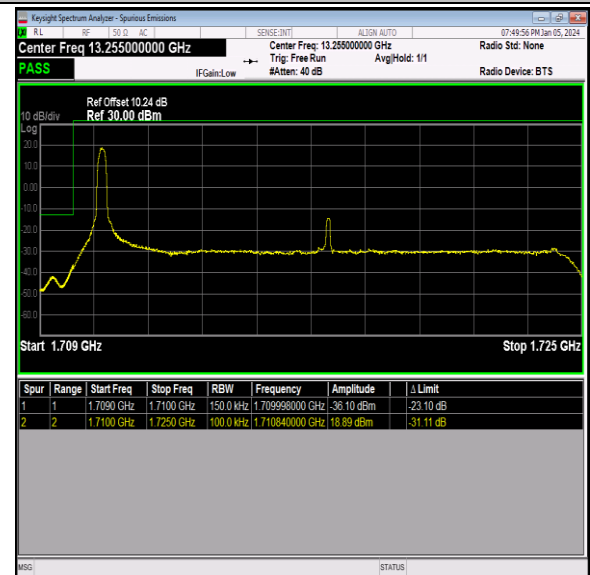
Band66_15MHz_16QAM_132047_1RB#0
