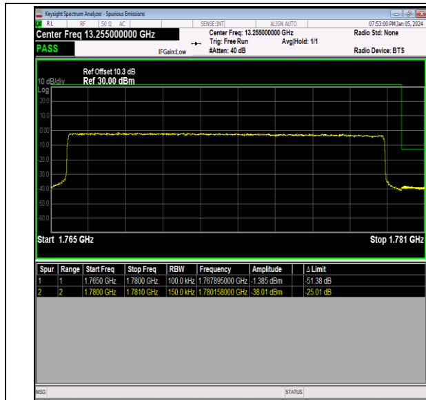
Band66_15MHz_16QAM_132597_75RB#0
