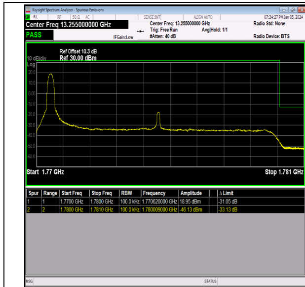
Band66_10MHz_16QAM_132622_1RB#0
