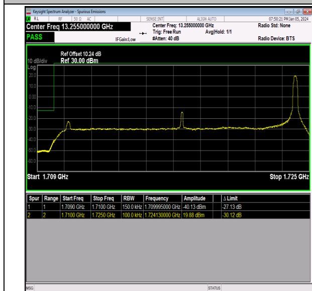
Band66_15MHz_QPSK_132047_1RB#74
