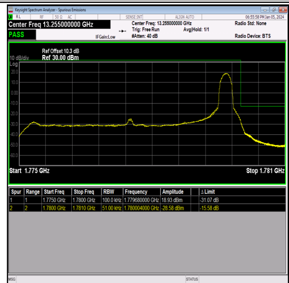
Band66_5MHz_16QAM_132647_1RB#24
