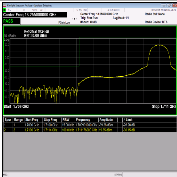
Band66_1.4MHz_QPSK_131979_1RB#5
