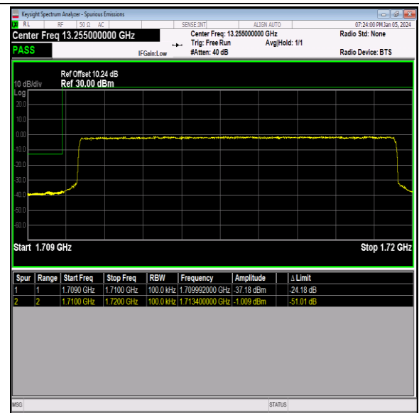
Band66_10MHz_64QAM_132022_50RB#0
