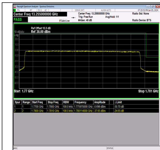
Band66_10MHz_64QAM_132622_50RB#0
