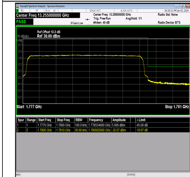
Band66_3MHz_16QAM_132657_15RB#0
