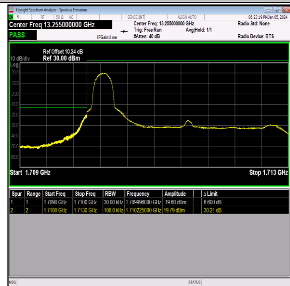
Band66_3MHz_QPSK_131987_1RB#0
