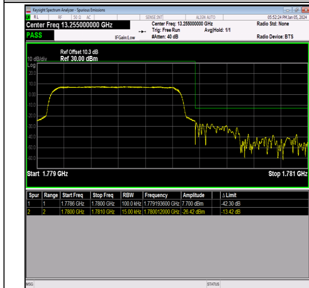
Band66_1.4MHz_64QAM_132665_6RB#0
