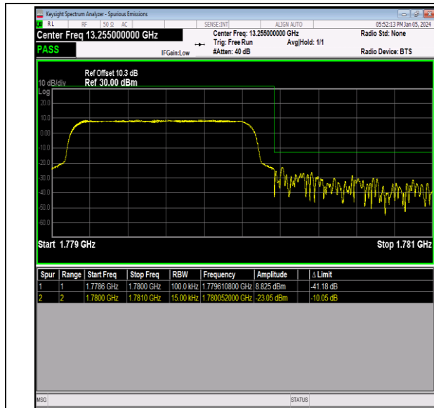
Band66_1.4MHz_16QAM_132665_6RB#0
