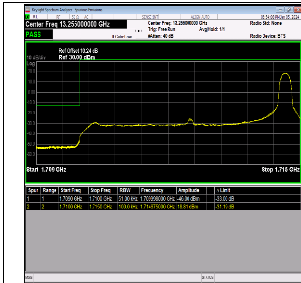
Band66_5MHz_16QAM_131997_1RB#24
