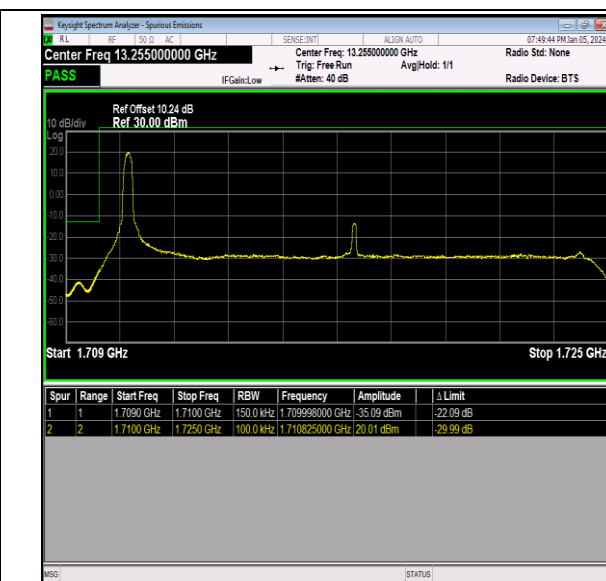
Band66_15MHz_QPSK_132047_1RB#0
