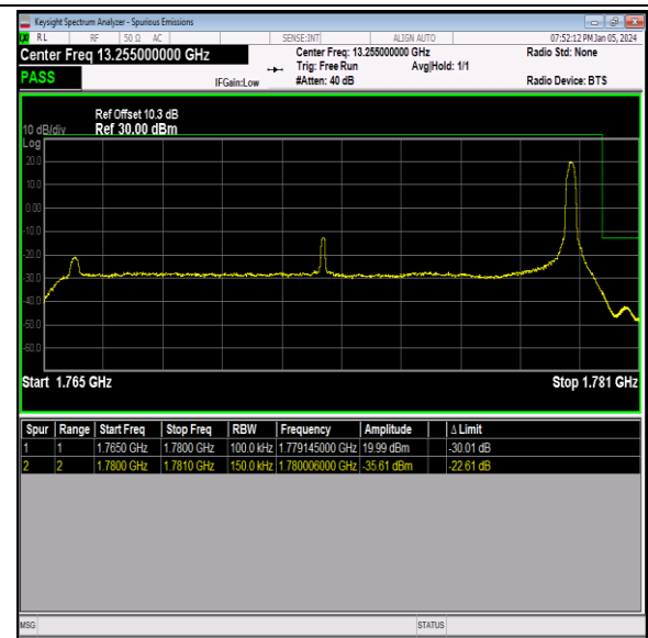
Band66_15MHz_QPSK_132597_1RB#74
