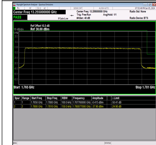
Band66_15MHz_QPSK_132597_75RB#0
