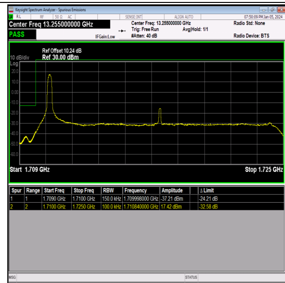
Band66_15MHz_64QAM_132047_1RB#0
