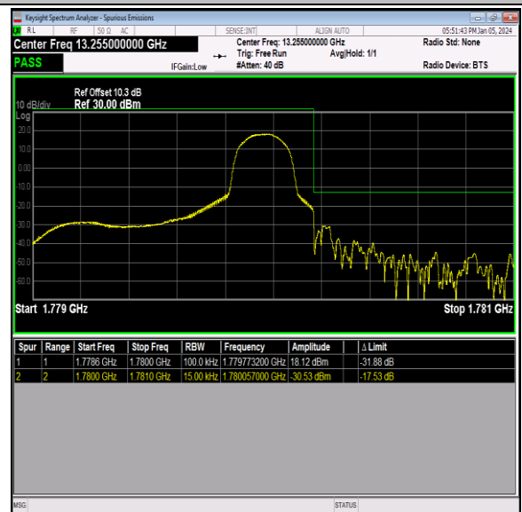
Band66_1.4MHz_16QAM_132665_1RB#5
