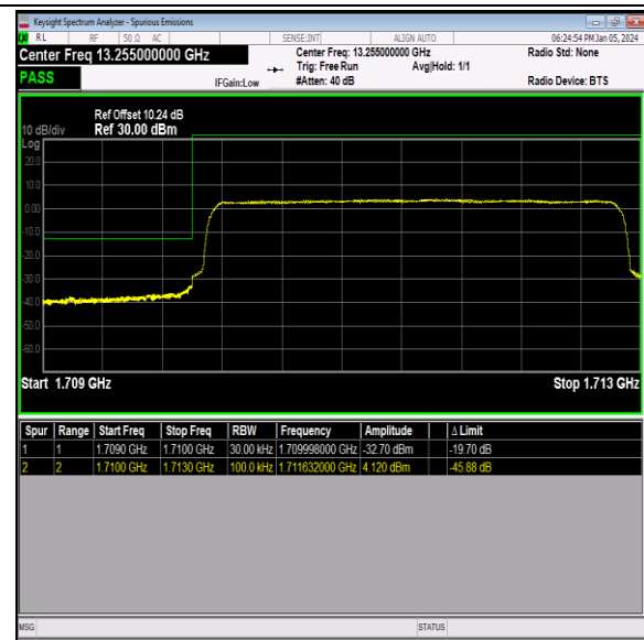
Band66_3MHz_64QAM_131987_15RB#0
