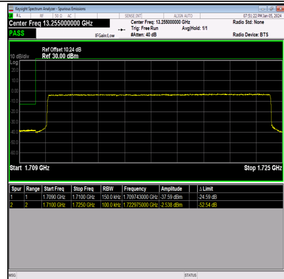
Band66_15MHz_64QAM_132047_75RB#0
