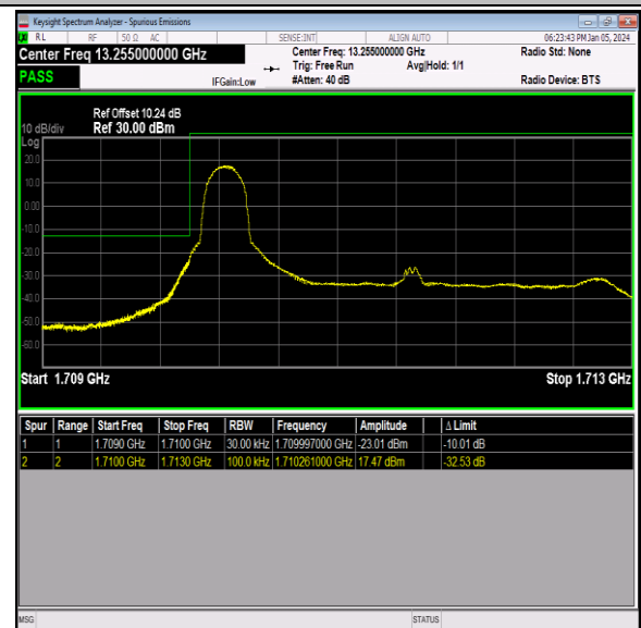
Band66_3MHz_64QAM_131987_1RB#0
