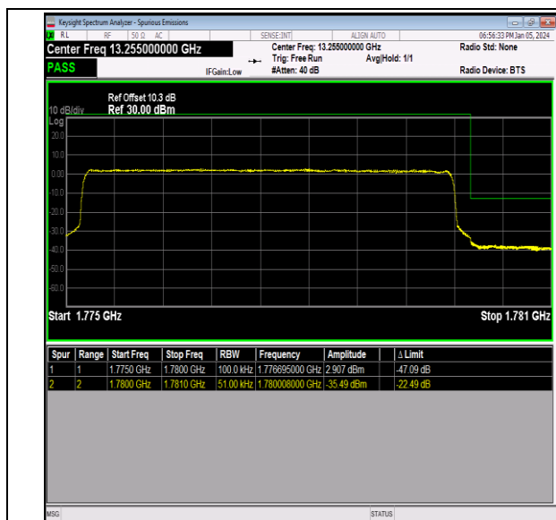
Band66_5MHz_16QAM_132647_25RB#0
