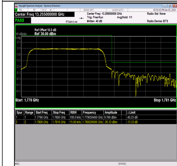
Band66_1.4MHz_QPSK_132665_6RB#0
