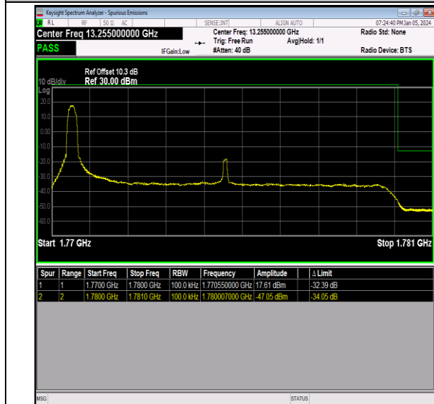
Band66_10MHz_64QAM_132622_1RB#0
