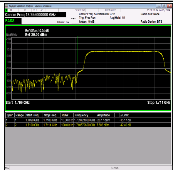
Band66_1.4MHz_64QAM_131979_6RB#0
