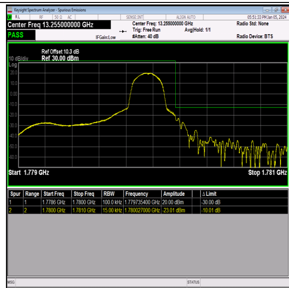
Band66_1.4MHz_QPSK_132665_1RB#5
