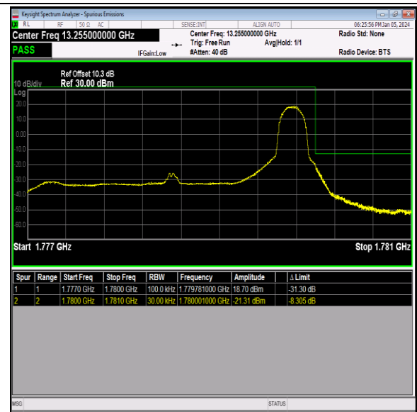
Band66_3MHz_16QAM_132657_1RB#14
