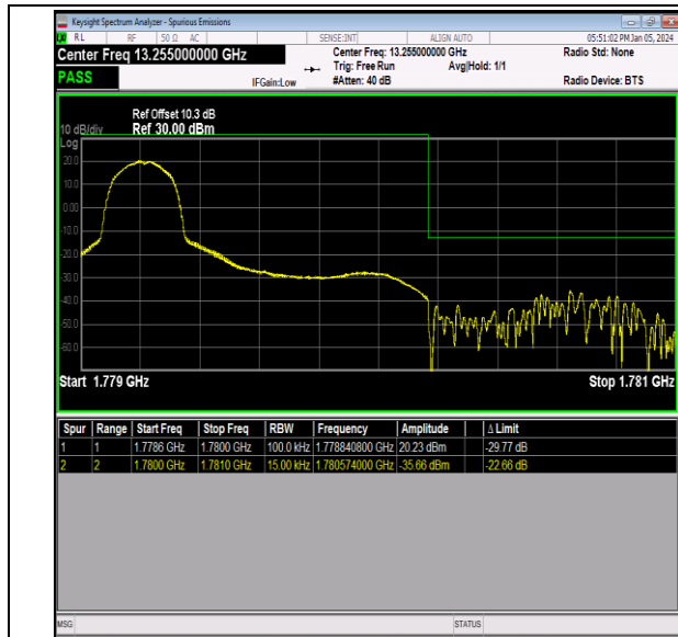
Band66_1.4MHz_QPSK_132665_1RB#0
