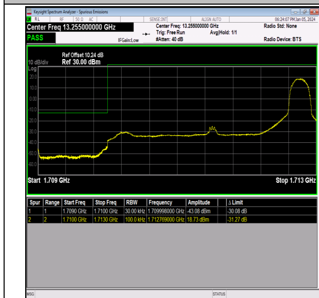
Band66_3MHz_16QAM_131987_1RB#14
