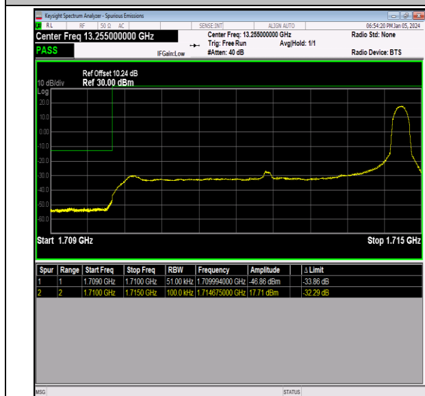
Band66_5MHz_64QAM_131997_1RB#24
