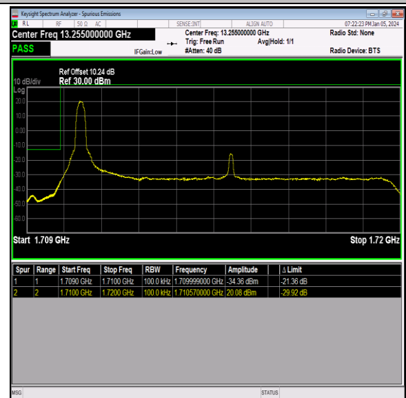
Band66_10MHz_QPSK_132022_1RB#0
