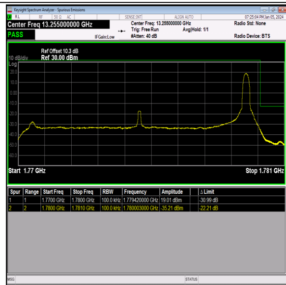
Band66_10MHz_16QAM_132622_1RB#49
