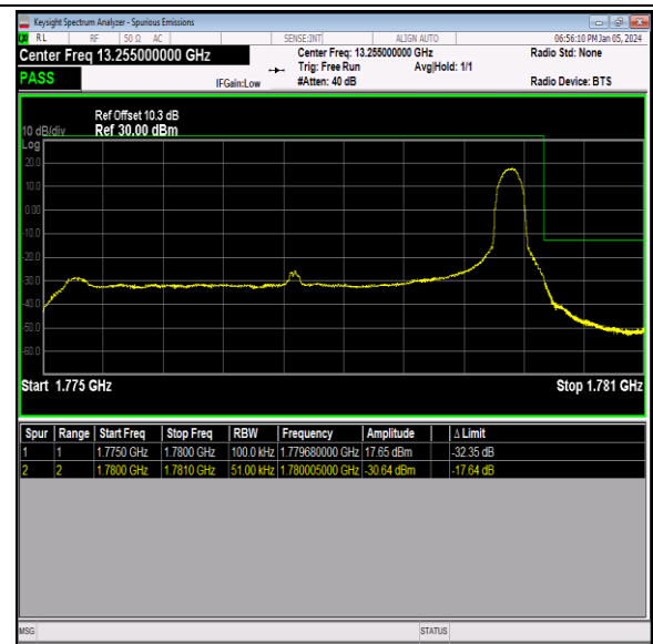
Band66_5MHz_64QAM_132647_1RB#24
