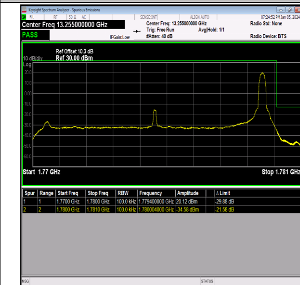
Band66_10MHz_QPSK_132622_1RB#49
