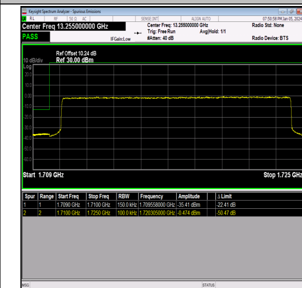
Band66_15MHz_QPSK_132047_75RB#0
