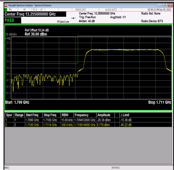
Band66_1.4MHz_QPSK_131979_6RB#0
