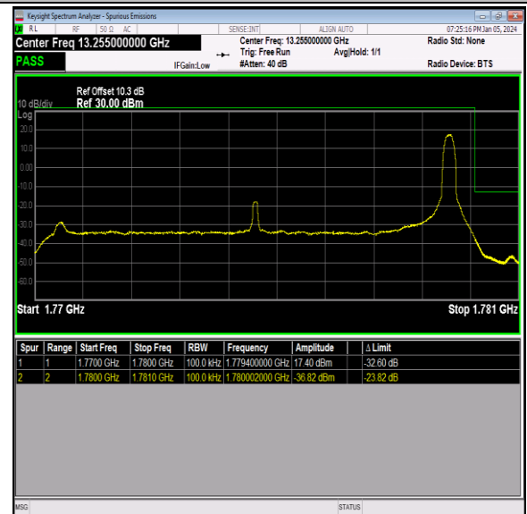
Band66_10MHz_64QAM_132622_1RB#49
