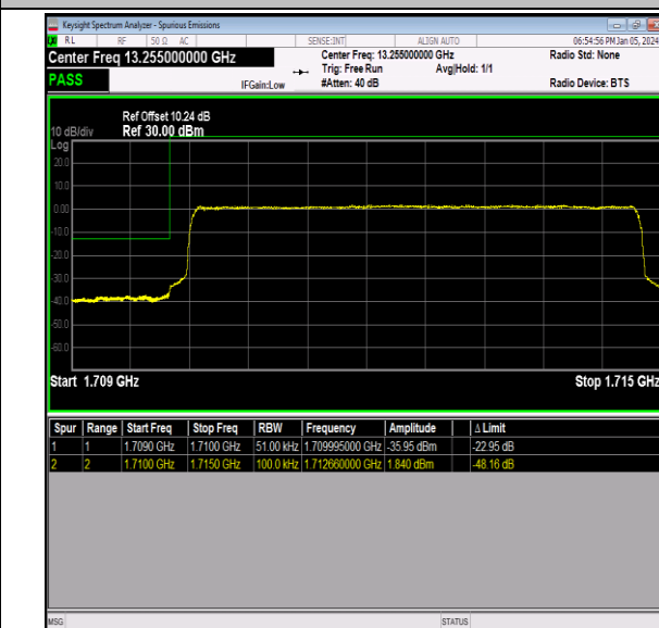
Band66_5MHz_64QAM_131997_25RB#0
