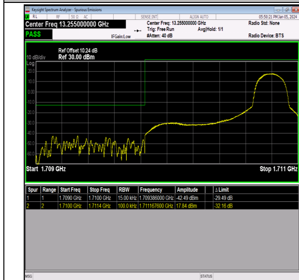
Band66_1.4MHz_64QAM_131979_1RB#5
