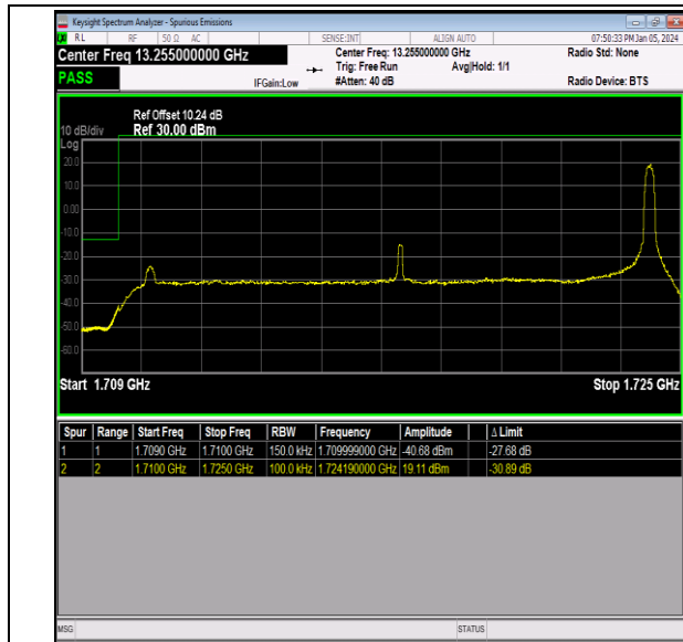
Band66_15MHz_16QAM_132047_1RB#74
