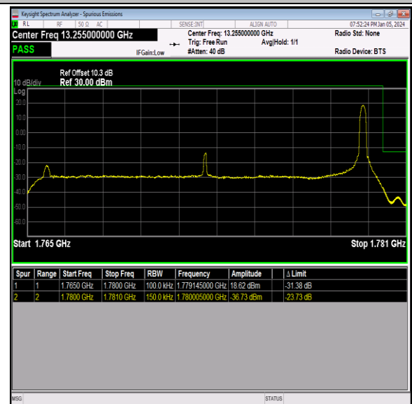
Band66_15MHz_16QAM_132597_1RB#74
