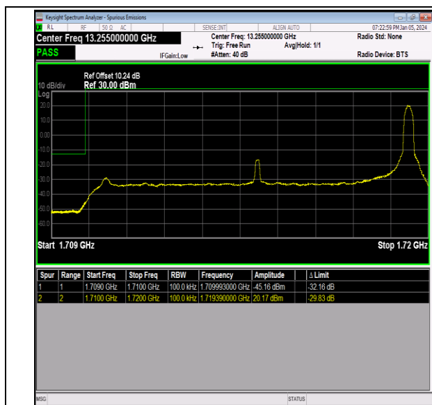
Band66_10MHz_QPSK_132022_1RB#49
