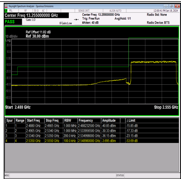
Band41_20MHz_64QAM_40140_100RB#0
