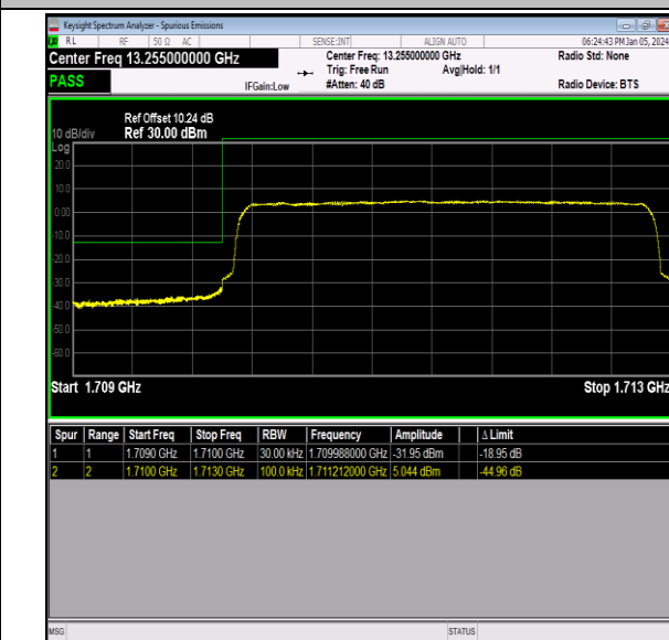
Band66_3MHz_16QAM_131987_15RB#0
