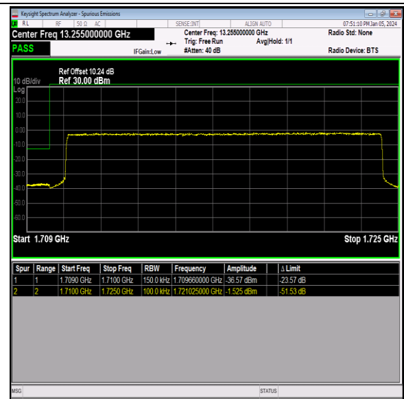
Band66_15MHz_16QAM_132047_75RB#0
