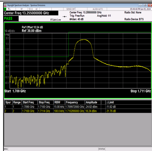
Band66_1.4MHz_16QAM_131979_1RB#0
