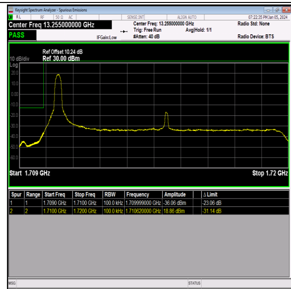
Band66_10MHz_16QAM_132022_1RB#0
