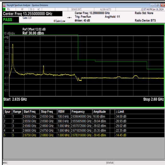
Band41_20MHz_64QAM_41140_1RB#0
