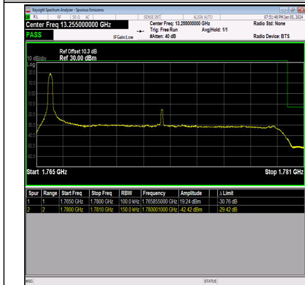
Band66_15MHz_16QAM_132597_1RB#0
