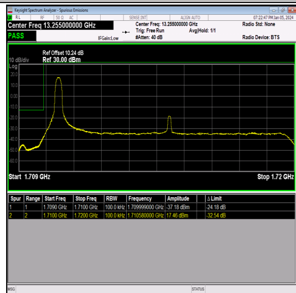
Band66_10MHz_64QAM_132022_1RB#0
