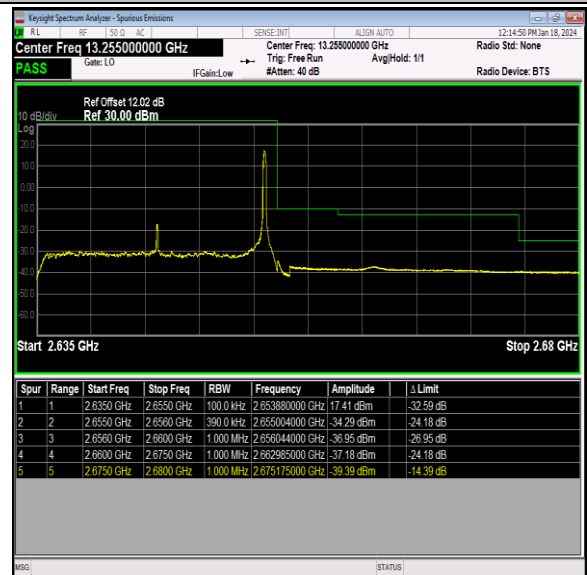
Band41_20MHz_64QAM_41140_1RB#99
