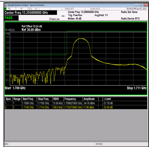
Band66_1.4MHz_64QAM_131979_1RB#0
