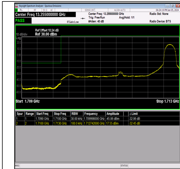
Band66_3MHz_64QAM_131987_1RB#14
