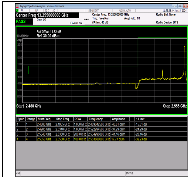
Band41_20MHz_64QAM_40140_1RB#99
