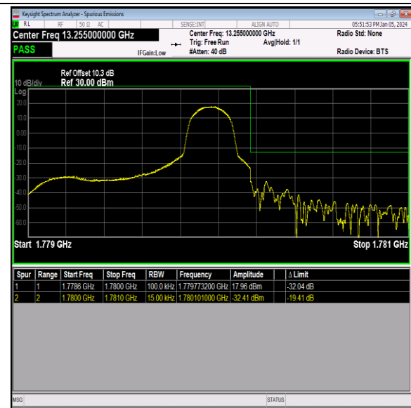
Band66_1.4MHz_64QAM_132665_1RB#5
