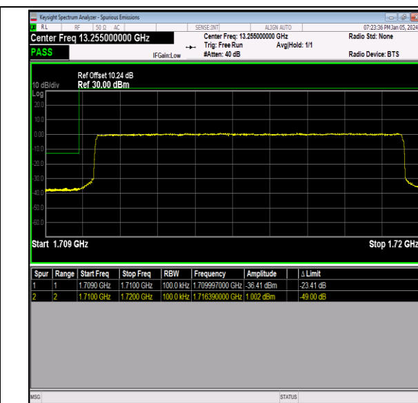
Band66_10MHz_QPSK_132022_50RB#0
