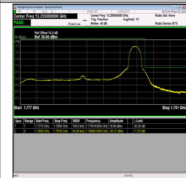
Band66_3MHz_QPSK_132657_1RB#14
