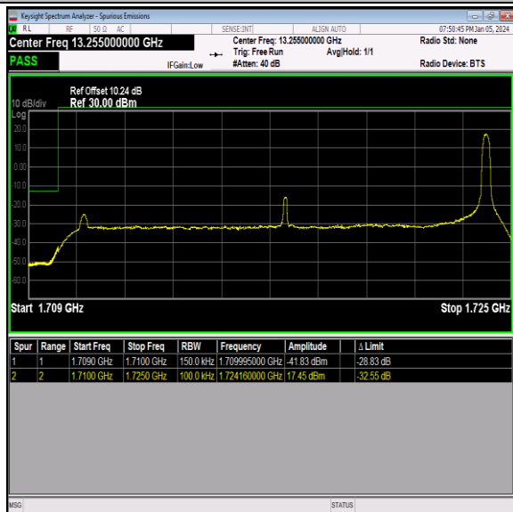
Band66_15MHz_64QAM_132047_1RB#74
