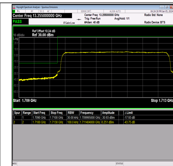
Band66_3MHz_QPSK_131987_15RB#0
