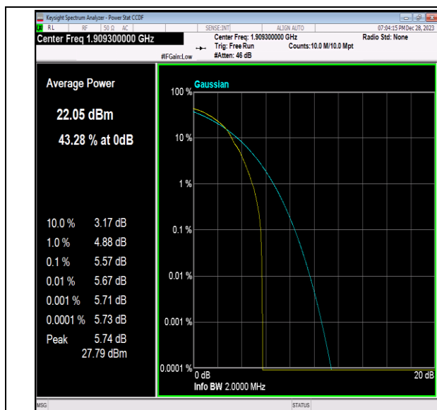
Band2-1.4MHz-64QAM-19193-1RB#0-PASS
