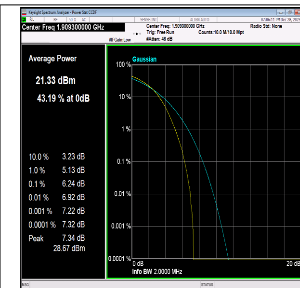
Band2-1.4MHz-64QAM-19193-6RB#0-PASS
