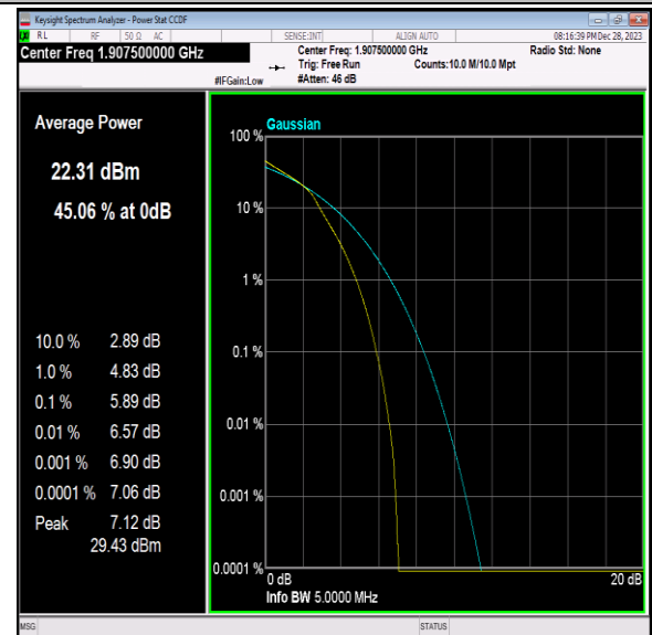
Band2-5MHz-16QAM-19175-25RB#0-PASS
