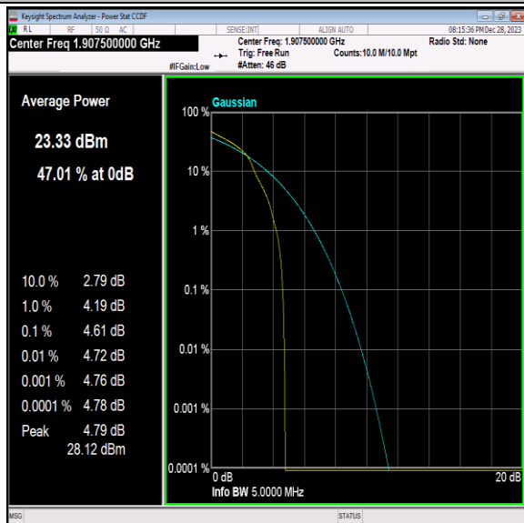
Band2-5MHz-16QAM-19175-1RB#0-PASS
