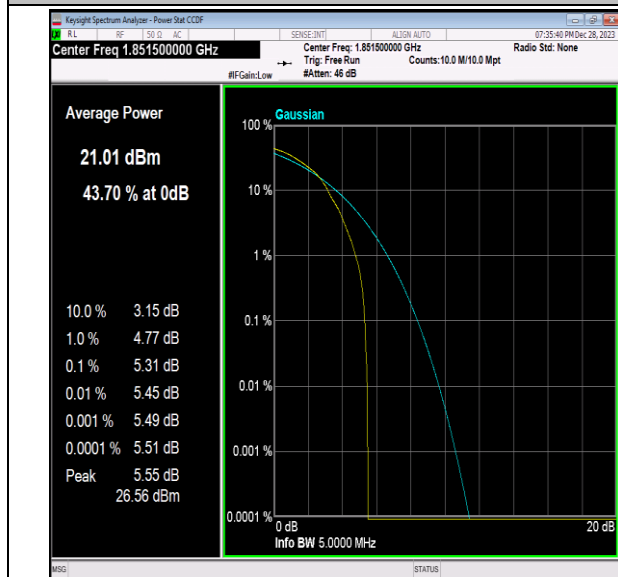
Band2-3MHz-64QAM-18615-1RB#0-PASS
