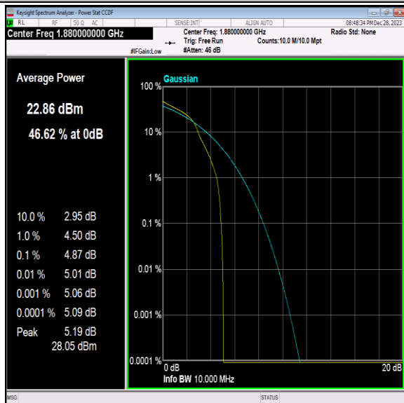
Band2-10MHz-16QAM-18900-1RB#0-PASS
