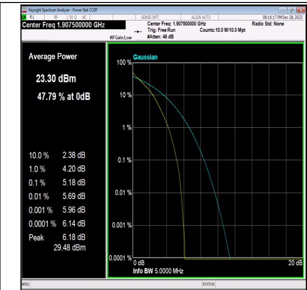
Band2-5MHz-QPSK-19175-25RB#0-PASS
