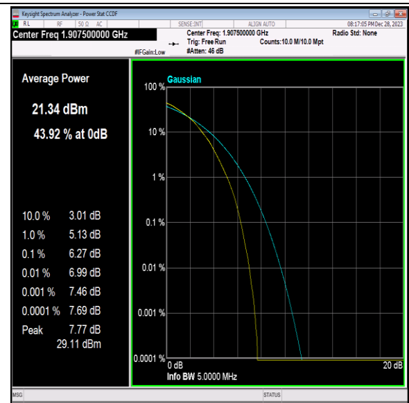
Band2-5MHz-64QAM-19175-25RB#0-PASS
