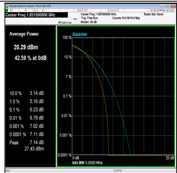
Band2-3MHz-64QAM-18615-15RB#0-PASS
