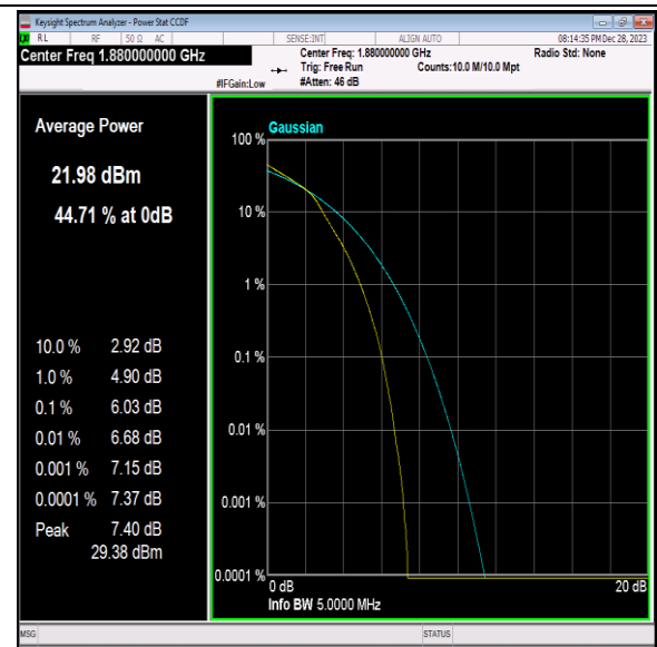
Band2-5MHz-16QAM-18900-25RB#0-PASS
