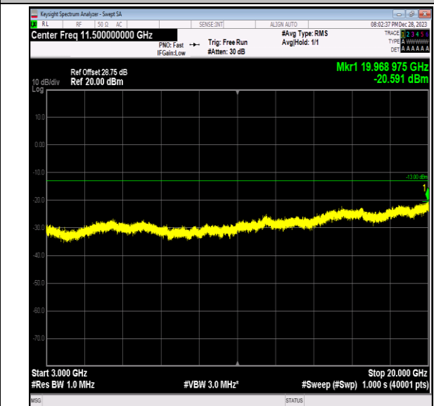
Band2_5MHz_16QAM_19175_1RB#0_3000~20000_3000~20000
