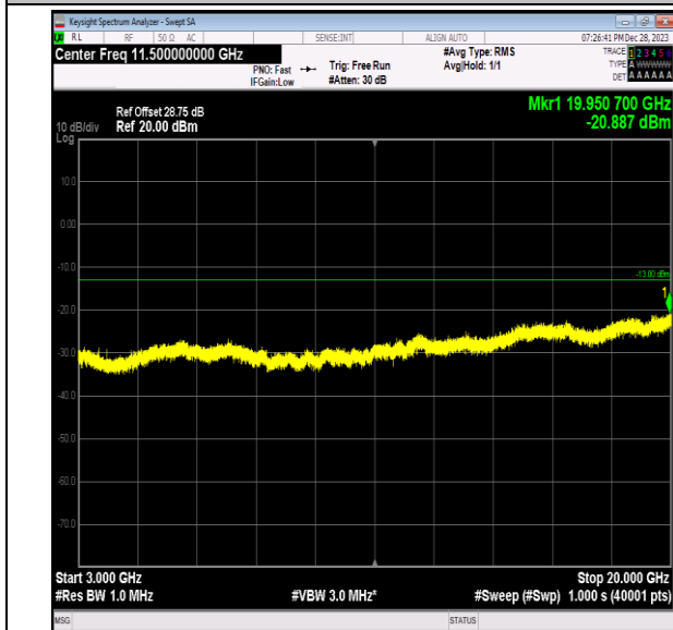
Band2_3MHz_16QAM_19185_1RB#0_3000~20000_3000~20000
