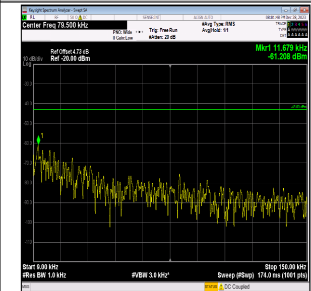
Band2_5MHz_16QAM_19175_1RB#0_0.009~0.15_0.009~0.15
