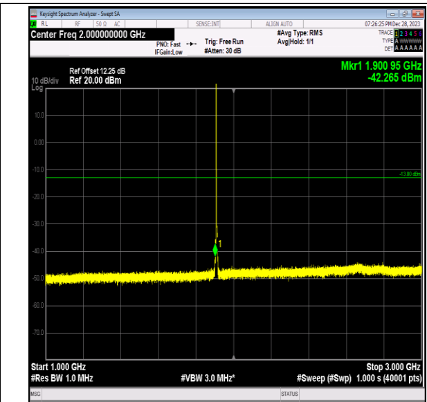
Band2_3MHz_16QAM_19185_1RB#0_1000~3000_1000~3000
