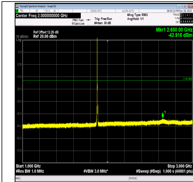
Band2_5MHz_64QAM_18900_1RB#0_1000~3000_1000~3000
