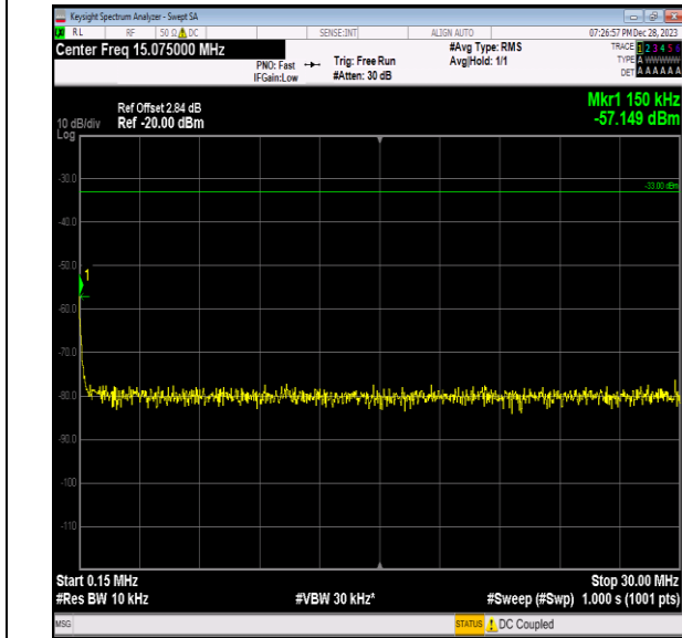
Band2_3MHz_64QAM_19185_1RB#0_0.15~30_0.15~30
