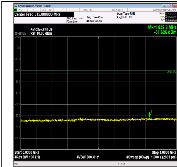
Band2_5MHz_16QAM_18900_1RB#0_30~1000_30~1000
