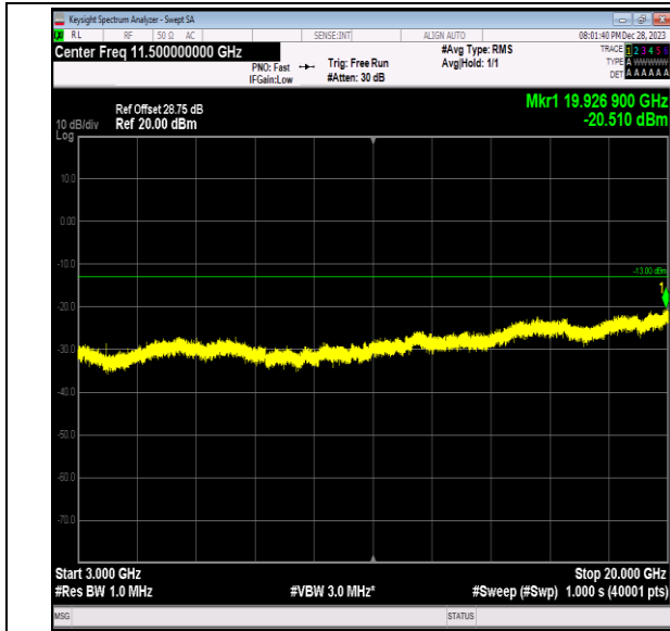
Band2_5MHz_QPSK_19175_1RB#0_3000~20000_3000~20000
