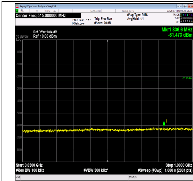
Band2_3MHz_16QAM_19185_1RB#0_30~1000_30~1000
