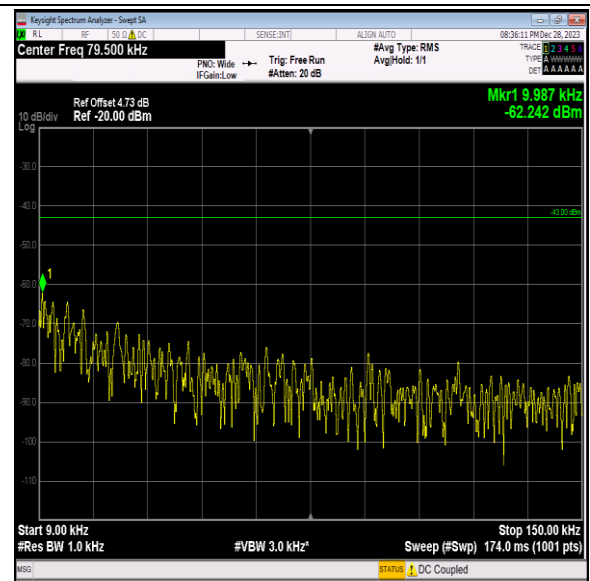
Band2_10MHz_QPSK_19150_1RB#0_0.009~0.15_0.009~ 0.15
