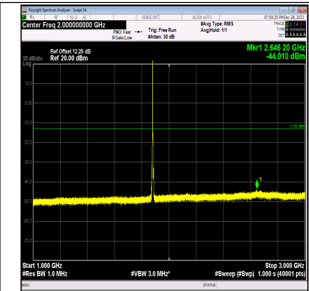
Band2_5MHz_16QAM_18900_1RB#0_1000~3000_1000~3000
