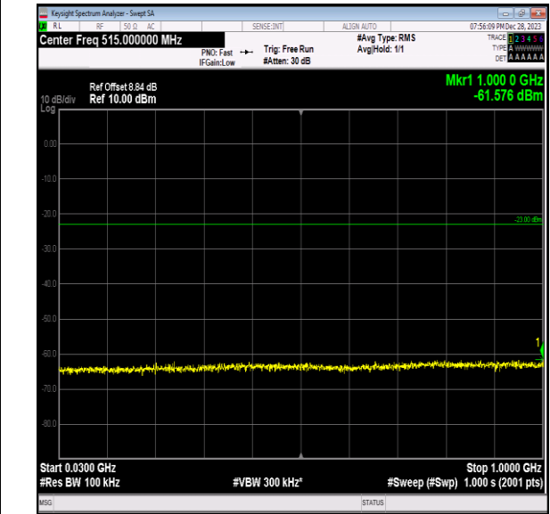
Band2_5MHz_16QAM_18625_1RB#0_30~1000_30~1000
