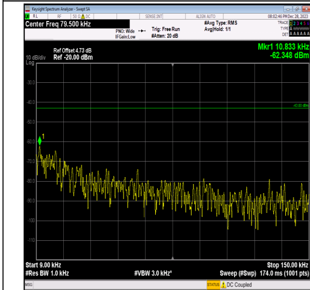
Band2_5MHz_64QAM_19175_1RB#0_0.009~0.15_0.009~0.15
