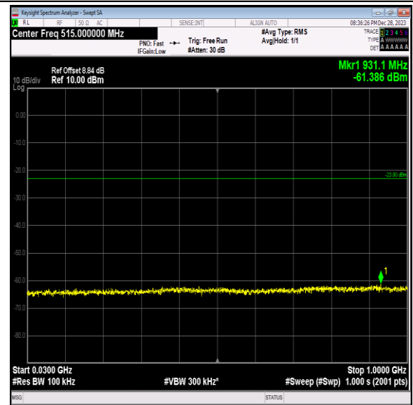
Band2_10MHz_QPSK_19150_1RB#0_30~1000_30~1000
