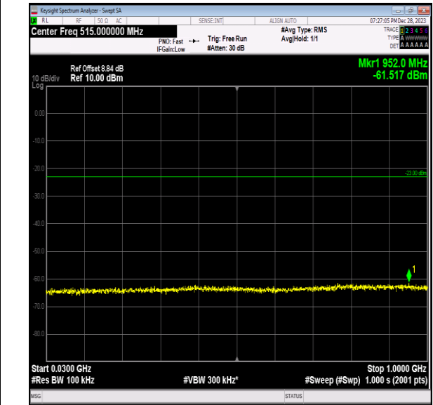
Band2_3MHz_64QAM_19185_1RB#0_30~1000_30~1000
