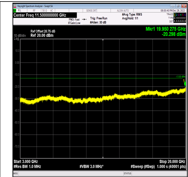
Band2_5MHz_64QAM_18900_1RB#0_3000~20000_3000~20000
