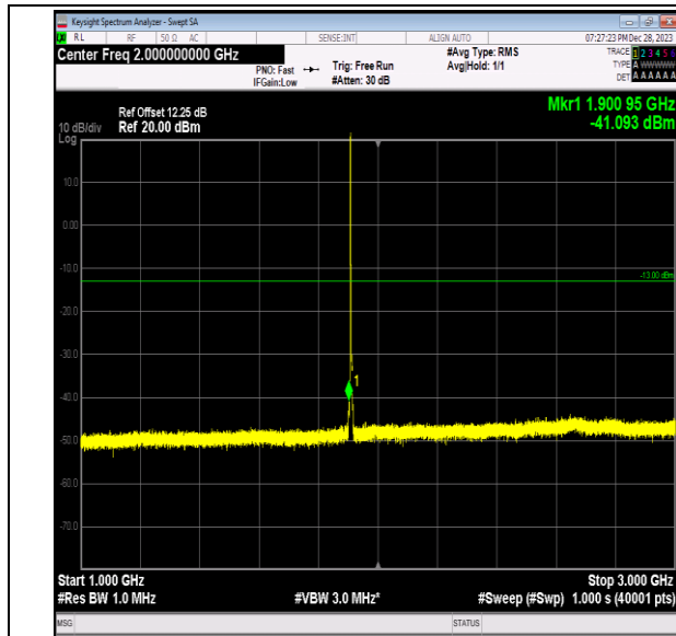
Band2_3MHz_64QAM_19185_1RB#0_1000~3000_1000~3000
