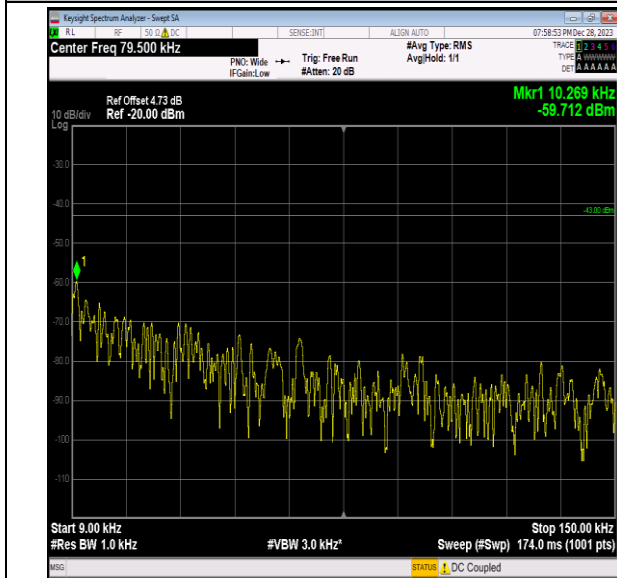
Band2_5MHz_16QAM_18900_1RB#0_0.009~0.15_0.009~0.15
