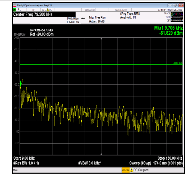
Band2_5MHz_16QAM_18625_1RB#0_0.009~0.15_0.009~0.15
