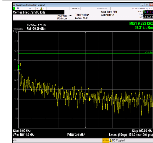
Band2_5MHz_QPSK_18625_1RB#0_0.009~0.15_0.009~0.15
