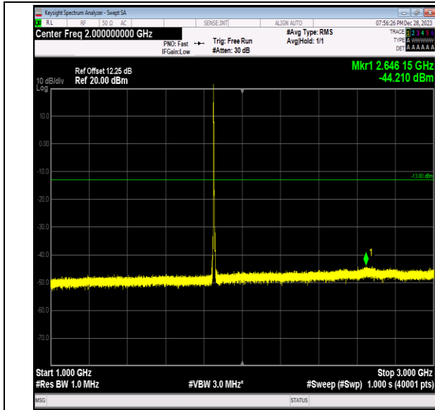
Band2_5MHz_16QAM_18625_1RB#0_1000~3000_1000~3000
