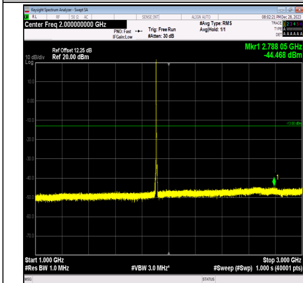
Band2_5MHz_16QAM_19175_1RB#0_1000~3000_1000~3000
