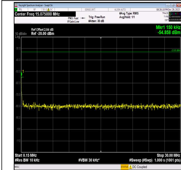
Band2_10MHz_QPSK_19150_1RB#0_0.15~30_0.15~30
