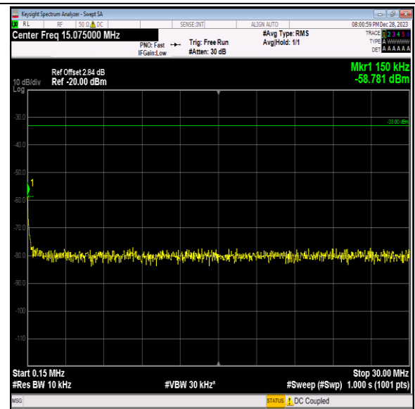
Band2_5MHz_QPSK_19175_1RB#0_0.15~30_0.15~30
