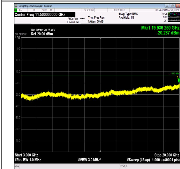
Band2_5MHz_16QAM_18900_1RB#0_3000~20000_3000~20000
