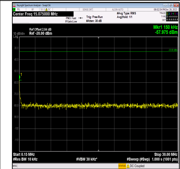
Band2_5MHz_64QAM_19175_1RB#0_0.15~30_0.15~30
