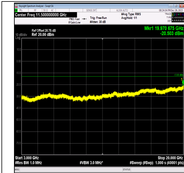
Band2_10MHz_QPSK_18900_1RB#0_3000~20000_3000 ~20000
