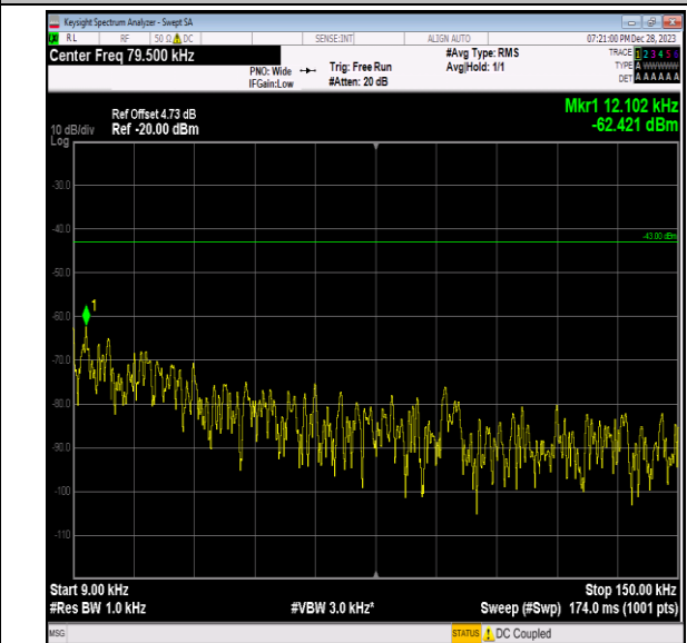
Band2_3MHz_64QAM_18615_1RB#0_0.009~0.15_0.009~0.15
