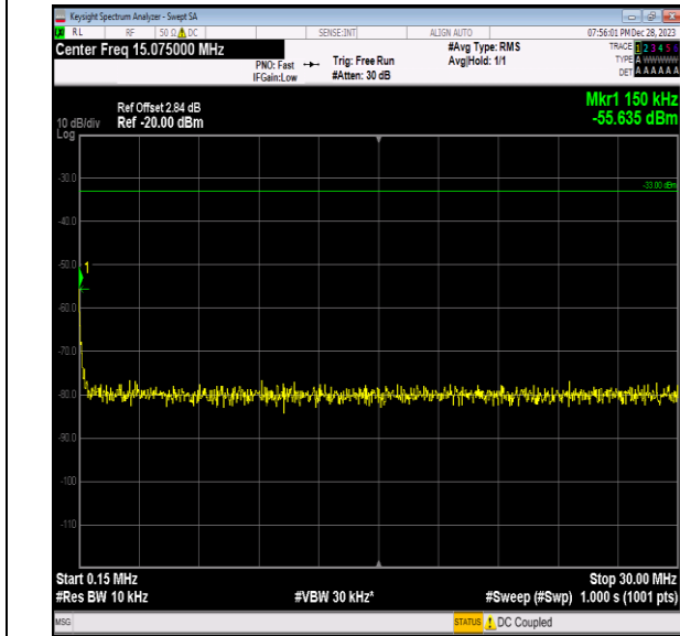
Band2_5MHz_16QAM_18625_1RB#0_0.15~30_0.15~30
