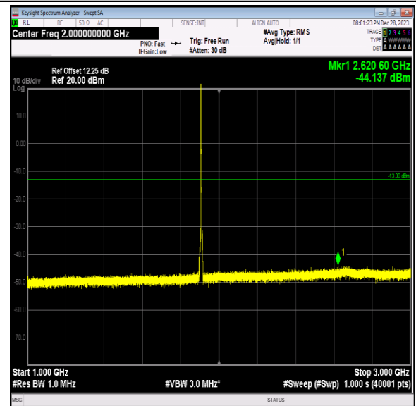
Band2_5MHz_QPSK_19175_1RB#0_1000~3000_1000~3000
