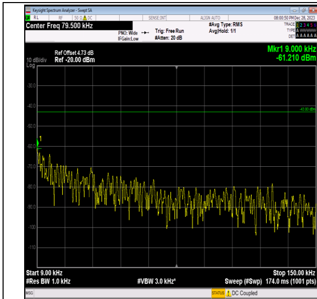
Band2_5MHz_QPSK_19175_1RB#0_0.009~0.15_0.009~0.15
