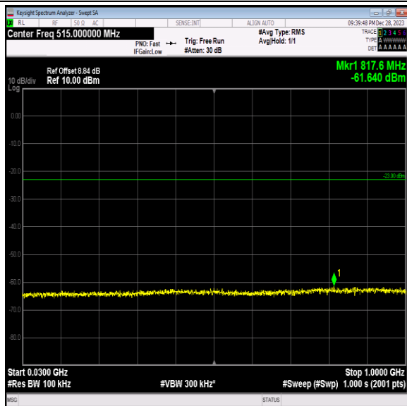
Band2_20MHz_16QAM_18700_1RB#0_30~1000_30~100 0
