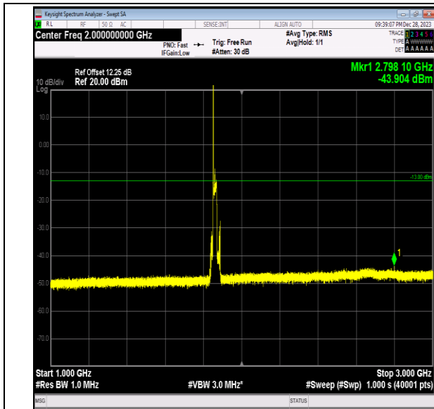
Band2_20MHz_QPSK_18700_1RB#0_1000~3000_1000~3000
