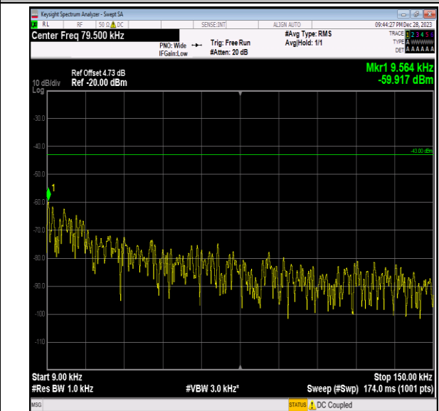
Band2_20MHz_QPSK_19100_1RB#0_0.009~0.15_0.009~0.15
