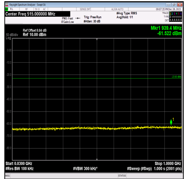
Band2_15MHz_QPSK_18900_1RB#0_30~1000_30~1000
