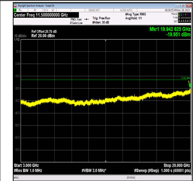
Band2_10MHz_64QAM_19150_1RB#0_3000~20000_3000 0~20000
