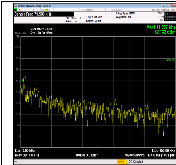
Band2_10MHz_16QAM_19150_1RB#0_0.009~0.15_0.009 ~0.15
