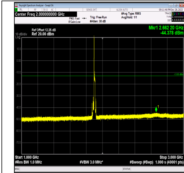
Band2_15MHz_16QAM_19125_1RB#0_1000~3000_1000 ~3000
