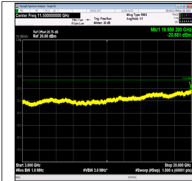
Band2_20MHz_16QAM_18700_1RB#0_3000~20000_300 0~20000
