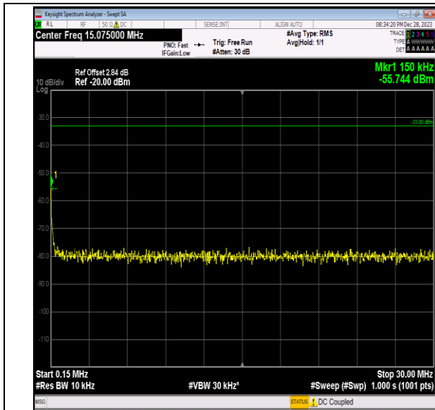
Band2_10MHz_16QAM_18900_1RB#0_0.15~30_0.15~30
