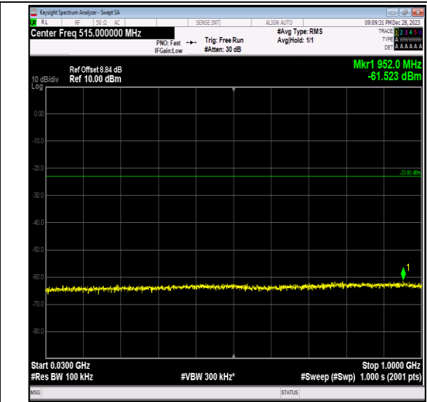
Band2_15MHz_64QAM_18900_1RB#0_30~1000_30~1000
