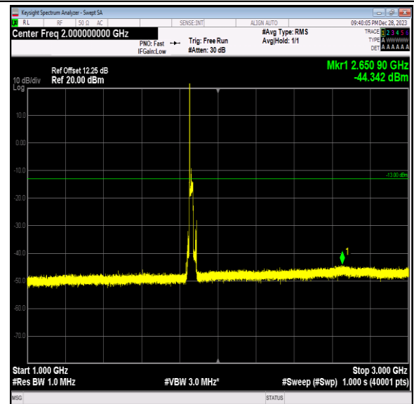
Band2_20MHz_16QAM_18700_1RB#0_1000~3000_1000 ~3000
