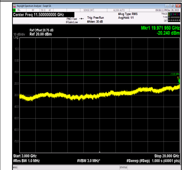
Band2_15MHz_16QAM_18675_1RB#0_3000~20000_3000 0~20000
