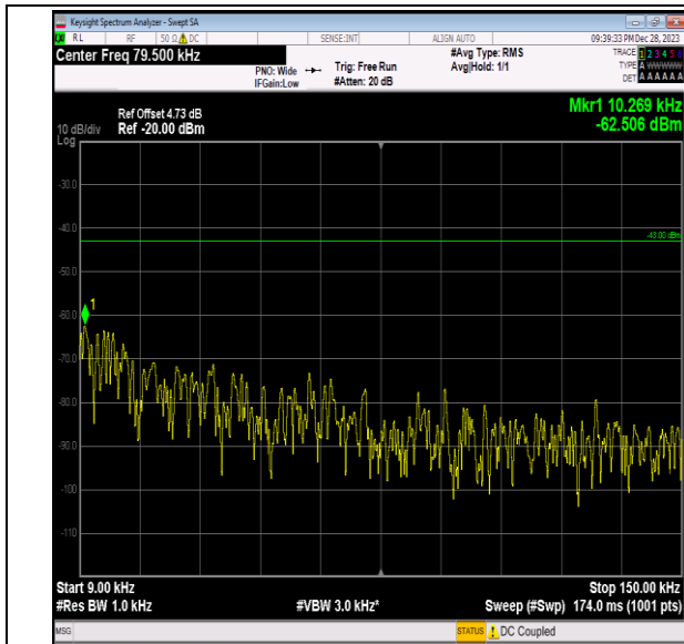
Band2_20MHz_16QAM_18700_1RB#0_0.009~0.15_0.009 ~0.15
