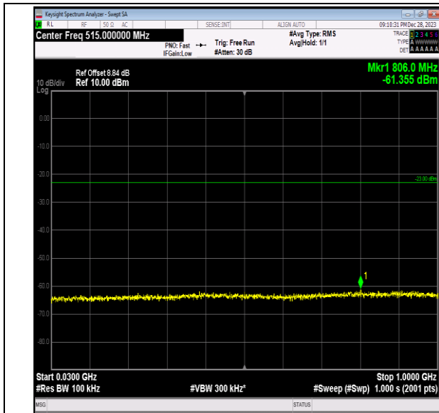
Band2_15MHz_QPSK_19125_1RB#0_30~1000_30~1000
