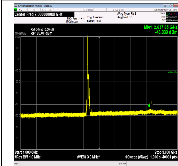
Band2_15MHz_16QAM_18675_1RB#0_1000~3000_1000 ~3000
