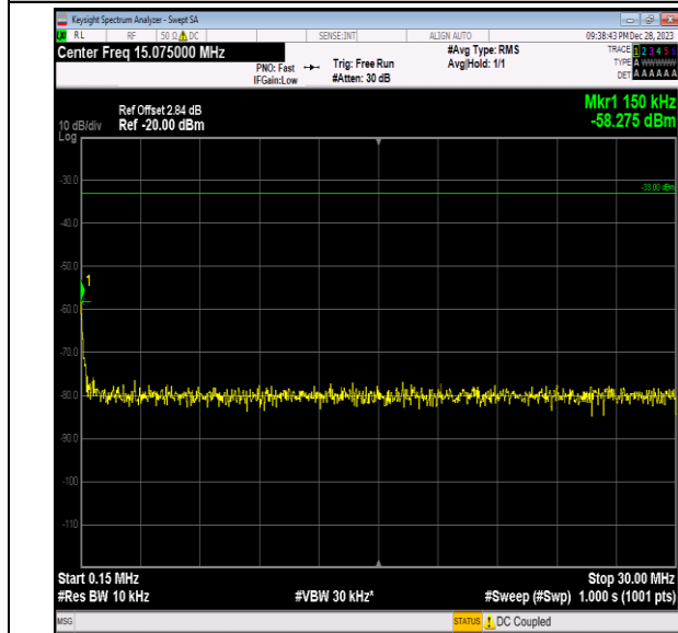
Band2_20MHz_QPSK_18700_1RB#0_0.15~30_0.15~30
