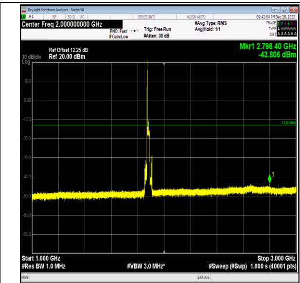
Band2_20MHz_QPSK_18900_1RB#0_1000~3000_1000~3000
