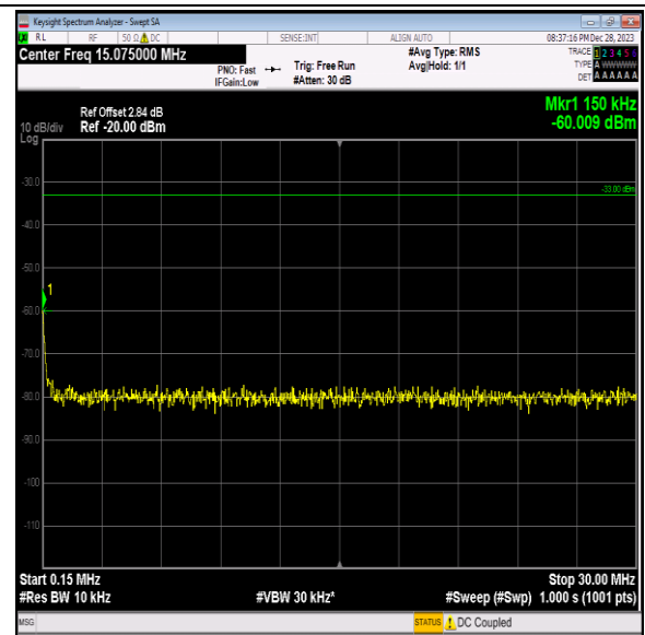
Band2_10MHz_16QAM_19150_1RB#0_0.15~30_0.15~30
