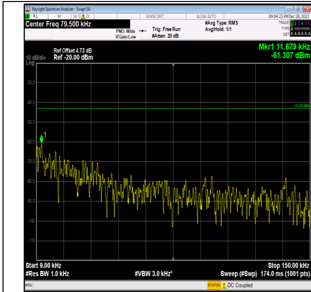
Band2_15MHz_QPSK_18675_1RB#0_0.009~0.15_0.009~0.15
