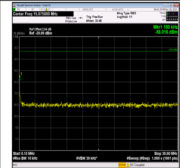
Band2_20MHz_QPSK_18900_1RB#0_0.15~30_0.15~30
