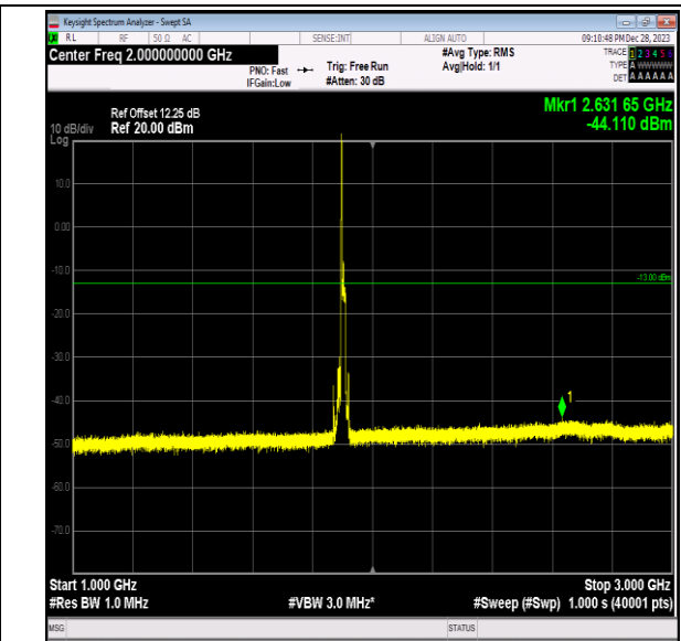
Band2_15MHz_QPSK_19125_1RB#0_1000~3000_1000~3000
