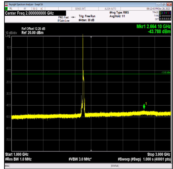
Band2_15MHz_64QAM_19125_1RB#0_1000~3000_1000 ~3000
