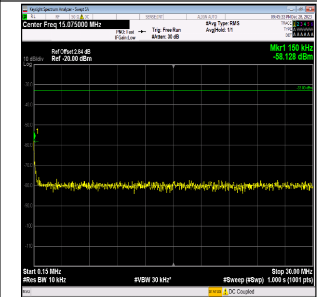
Band2_20MHz_16QAM_19100_1RB#0_0.15~30_0.15~30
