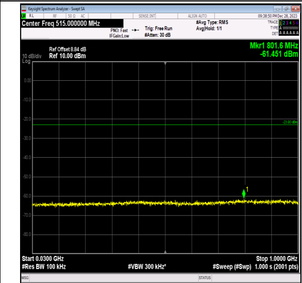
Band2_20MHz_QPSK_18700_1RB#0_30~1000_30~1000
