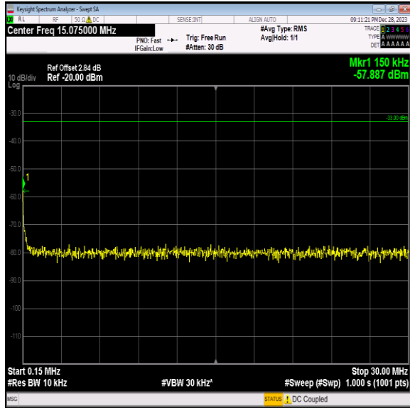
Band2_15MHz_16QAM_19125_1RB#0_0.15~30_0.15~30
