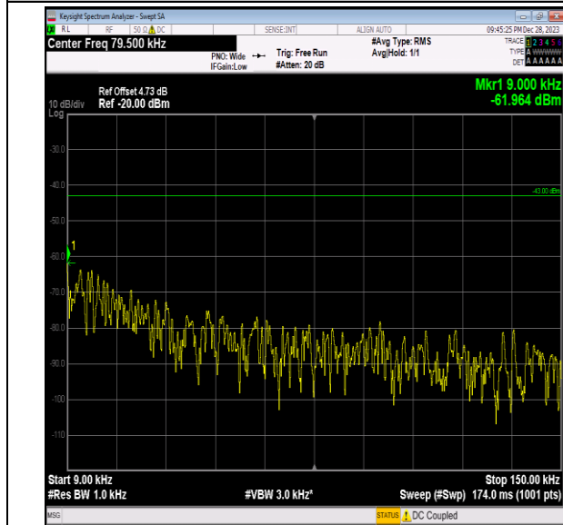
Band2_20MHz_16QAM_19100_1RB#0_0.009~0.15_0.009 ~0.15
