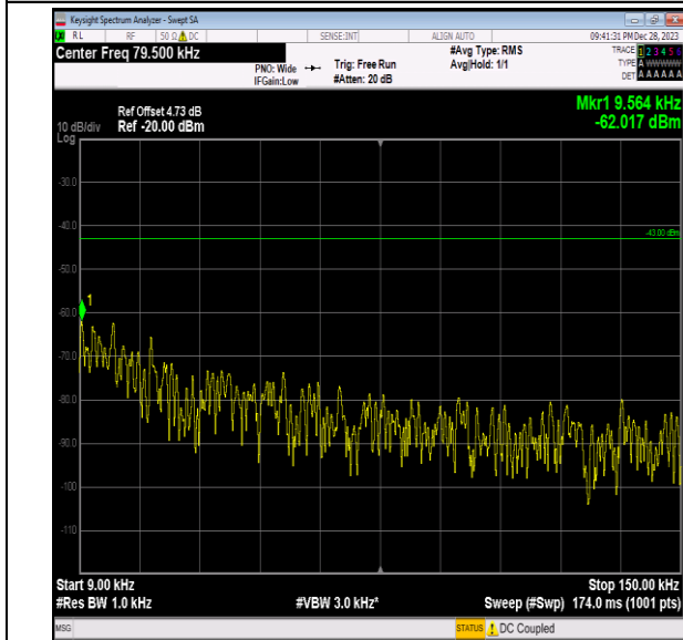
Band2_20MHz_QPSK_18900_1RB#0_0.009~0.15_0.009~0.15
