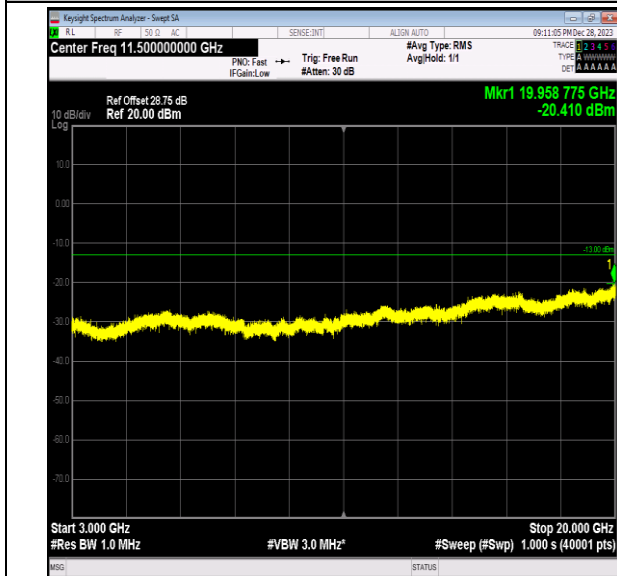
Band2_15MHz_QPSK_19125_1RB#0_3000~20000_3000~20000
