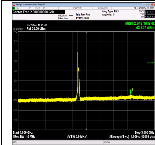
Band2_15MHz_64QAM_18900_1RB#0_1000~3000_1000~3000
