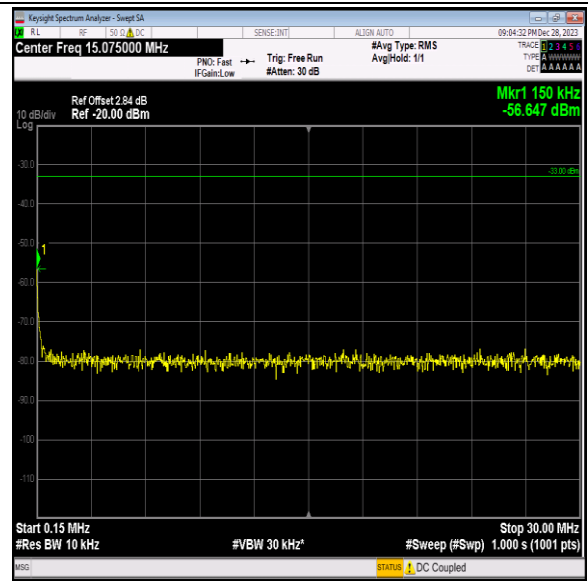
Band2_15MHz_QPSK_18675_1RB#0_0.15~30_0.15~30
