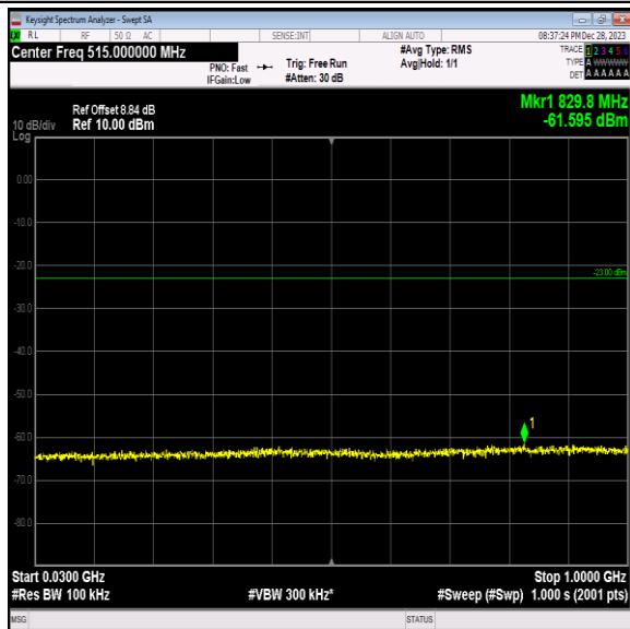
Band2_10MHz_16QAM_19150_1RB#0_30~1000_30~100 0
