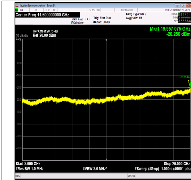
Band2_15MHz_QPSK_18675_1RB#0_3000~20000_3000 ~20000
