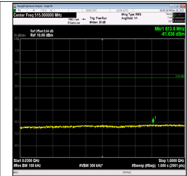
Band2_15MHz_16QAM_18675_1RB#0_30~1000_30~1000 0
