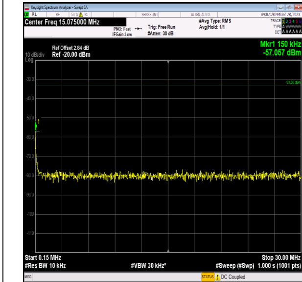
Band2_15MHz_QPSK_18900_1RB#0_0.15~30_0.15~30
