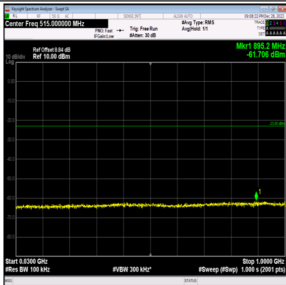
Band2_15MHz_16QAM_18900_1RB#0_30~1000_30~100 0
