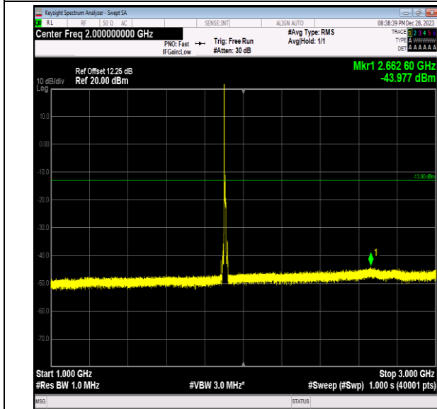
Band2_10MHz_64QAM_19150_1RB#0_1000~3000_1000 ~3000
