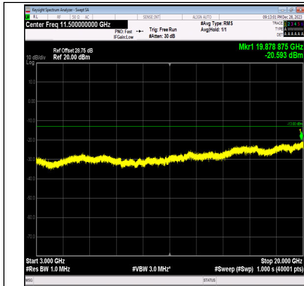
Band2_15MHz_64QAM_19125_1RB#0_3000~20000_300 0~20000
