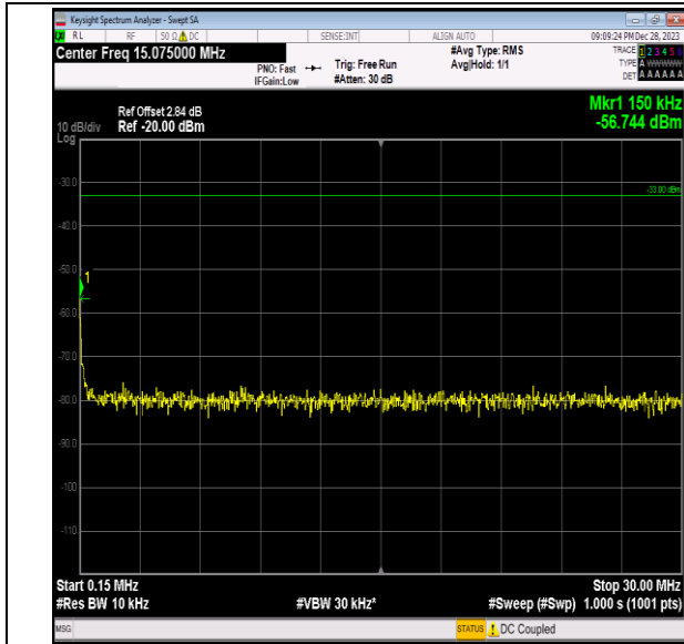
Band2_15MHz_64QAM_18900_1RB#0_0.15~30_0.15~30
