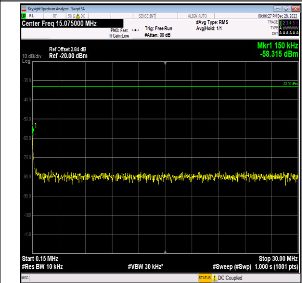
Band2_15MHz_64QAM_18675_1RB#0_0.15~30_0.15~30
