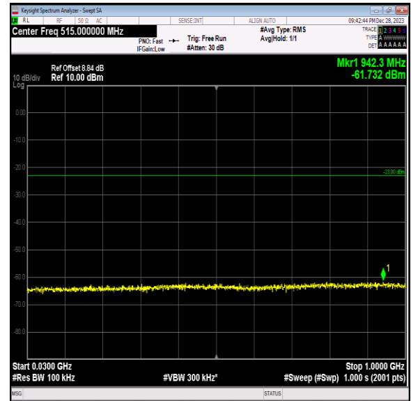
Band2_20MHz_16QAM_18900_1RB#0_30~1000_30~100 0
