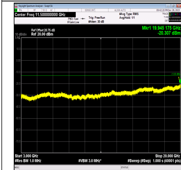
Band2_20MHz_QPSK_18900_1RB#0_3000~20000_3000~20000
