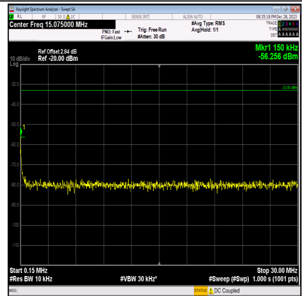
Band2_10MHz_64QAM_18900_1RB#0_0.15~30_0.15~30
