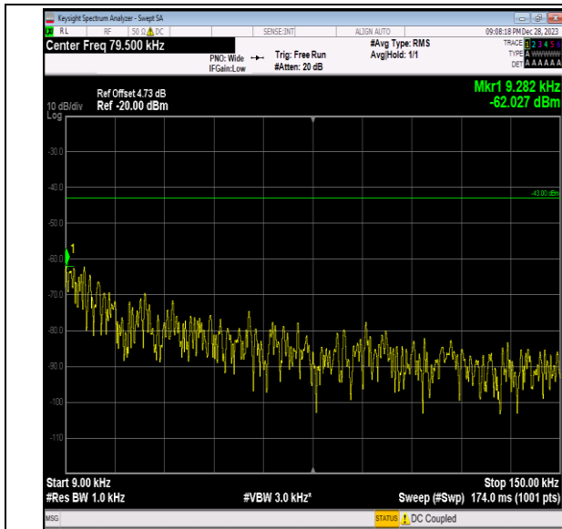
Band2_15MHz_16QAM_18900_1RB#0_0.009~0.15_0.009 ~0.15
