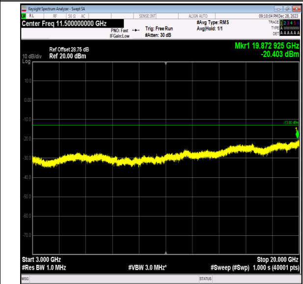
Band2_15MHz_64QAM_18900_1RB#0_3000~20000_3000~20000
