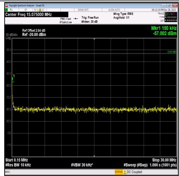
Band2_15MHz_64QAM_19125_1RB#0_0.15~30_0.15~30
