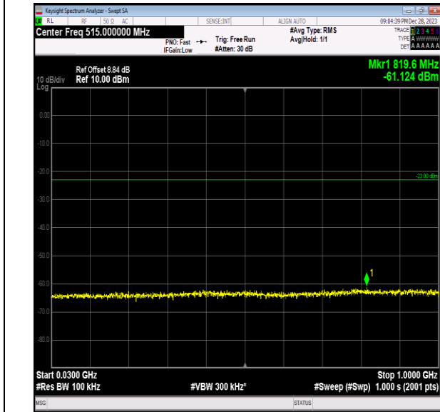
Band2_15MHz_QPSK_18675_1RB#0_30~1000_30~1000
