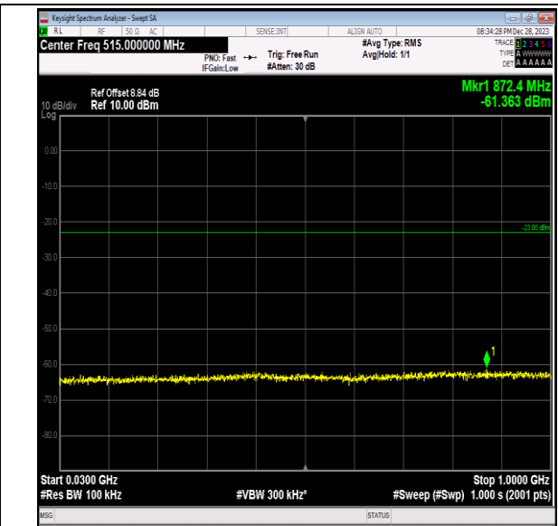
Band2_10MHz_16QAM_18900_1RB#0_30~1000_30~1000
