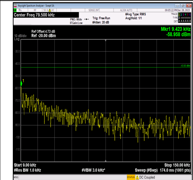
Band2_15MHz_16QAM_18675_1RB#0_0.009~0.15_0.009~0.15
