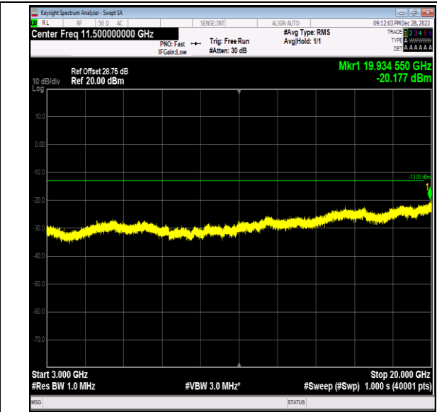
Band2_15MHz_16QAM_19125_1RB#0_3000~20000_300 0~20000
