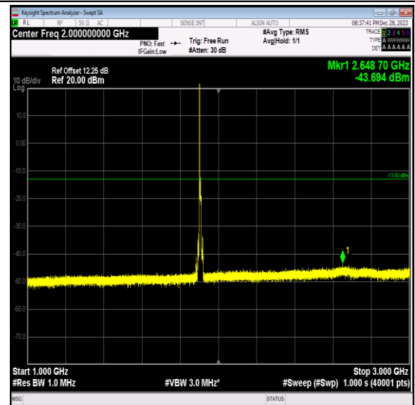
Band2_10MHz_16QAM_19150_1RB#0_1000~3000_1000 ~3000
