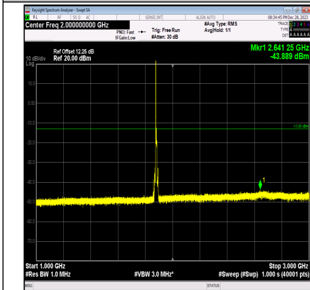
Band2_10MHz_16QAM_18900_1RB#0_1000~3000_1000~3000
