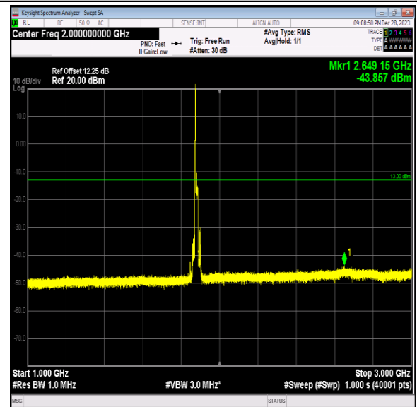
Band2_15MHz_16QAM_18900_1RB#0_1000~3000_1000 ~3000
