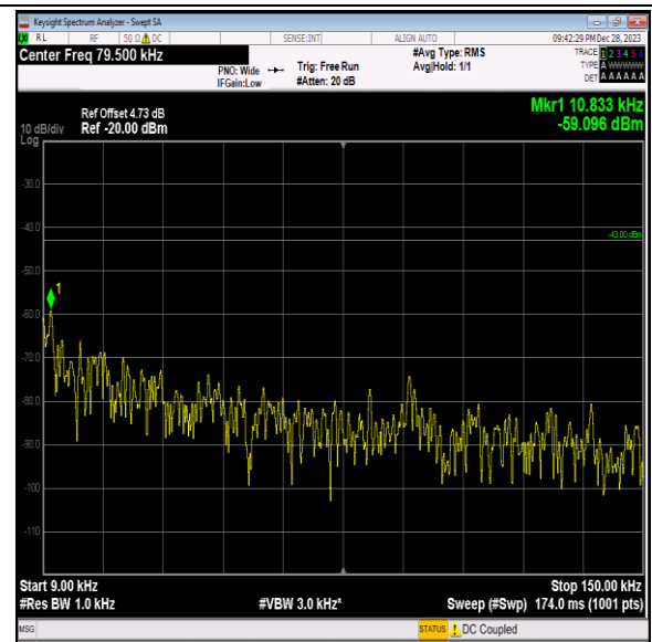
Band2_20MHz_16QAM_18900_1RB#0_0.009~0.15_0.009 ~0.15
