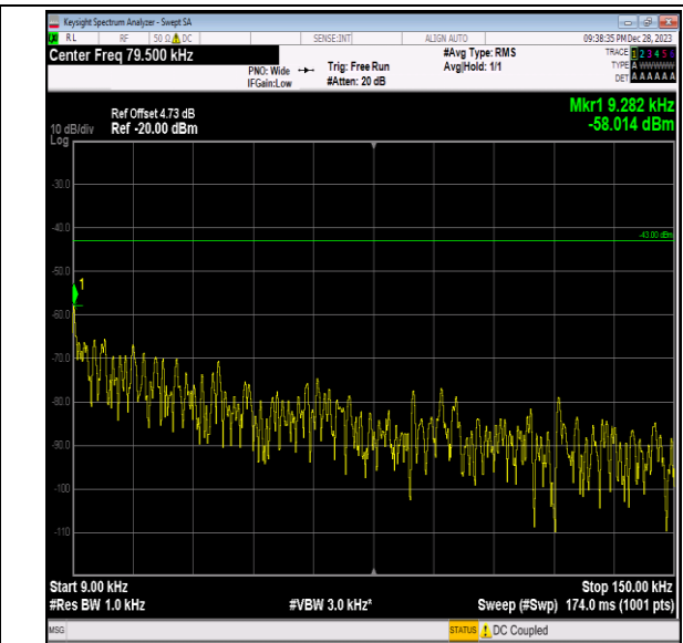
Band2_20MHz_QPSK_18700_1RB#0_0.009~0.15_0.009~ 0.15
