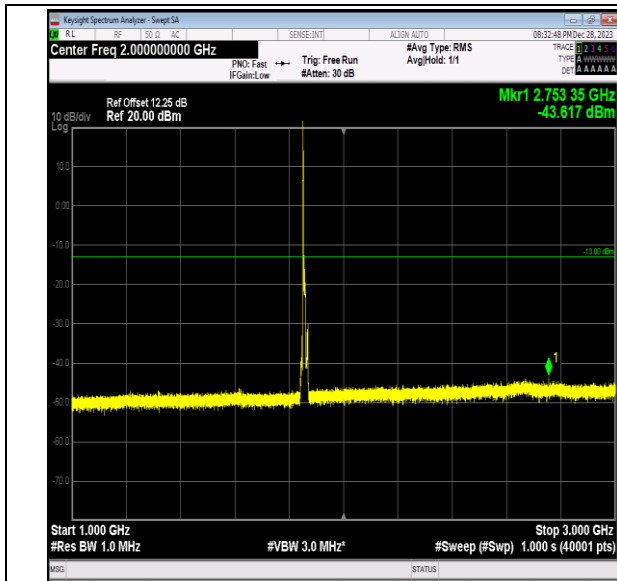
Band2_10MHz_64QAM_18650_1RB#0_1000~3000_1000 ~3000
