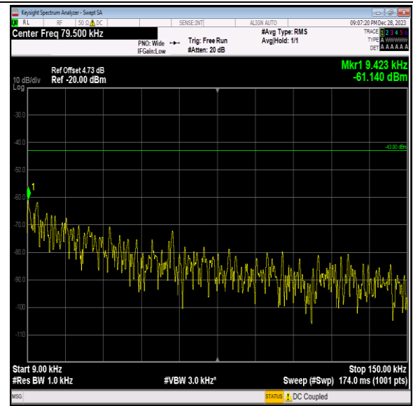
Band2_15MHz_QPSK_18900_1RB#0_0.009~0.15_0.009~ 0.15
