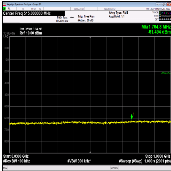
Band2_15MHz_64QAM_19125_1RB#0_30~1000_30~100 0
