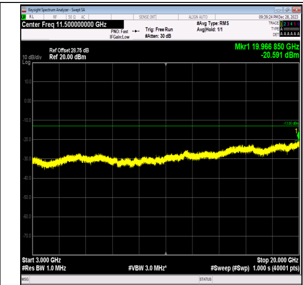
Band2_20MHz_QPSK_18700_1RB#0_3000~20000_3000~20000
