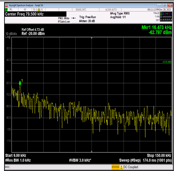
Band2_15MHz_16QAM_19125_1RB#0_0.009~0.15_0.009 ~0.15
