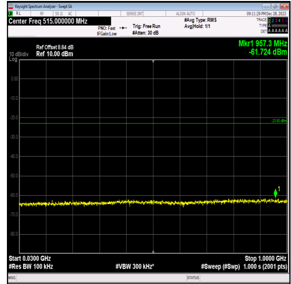
Band2_15MHz_16QAM_19125_1RB#0_30~1000_30~100 0
