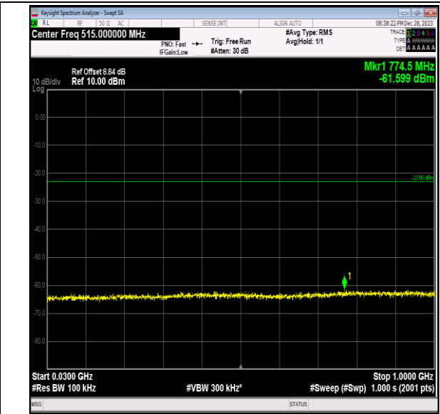
Band2_10MHz_64QAM_19150_1RB#0_30~1000_30~1000 0
