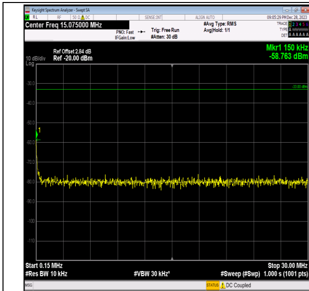
Band2_15MHz_16QAM_18675_1RB#0_0.15~30_0.15~30
