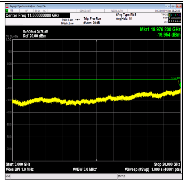
Band2_10MHz_64QAM_18650_1RB#0_3000~20000_300 0~20000
