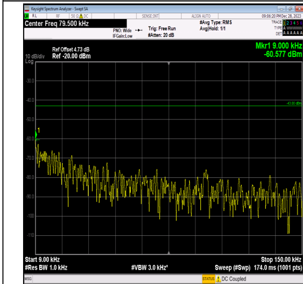
Band2_15MHz_64QAM_18675_1RB#0_0.009~0.15_0.009 ~0.15
