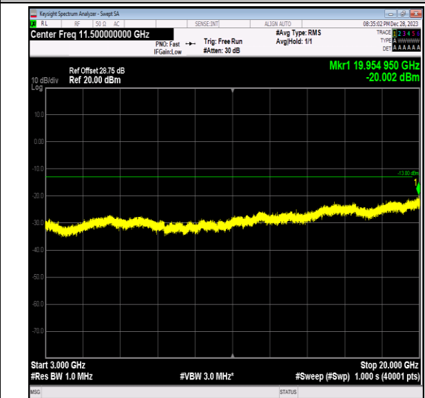
Band2_10MHz_16QAM_18900_1RB#0_3000~20000_3000~20000
