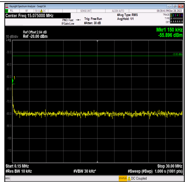
Band2_20MHz_16QAM_18700_1RB#0_0.15~30_0.15~30
