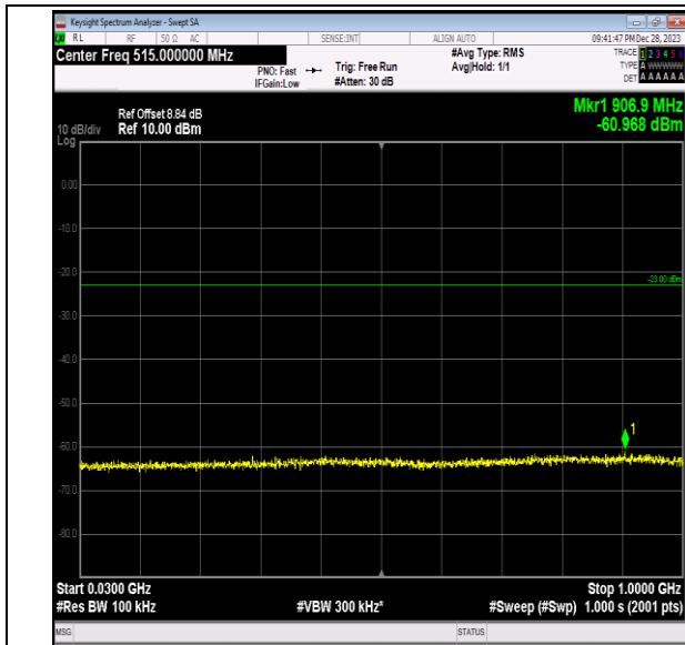
Band2_20MHz_QPSK_18900_1RB#0_30~1000_30~1000
