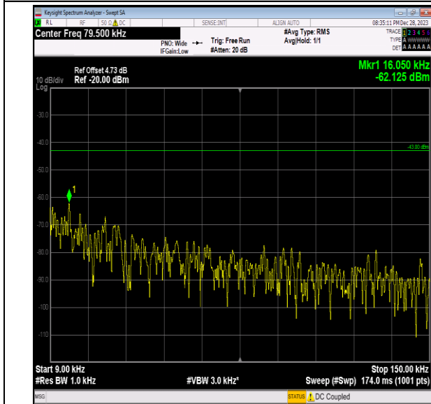
Band2_10MHz_64QAM_18900_1RB#0_0.009~0.15_0.009 ~0.15
