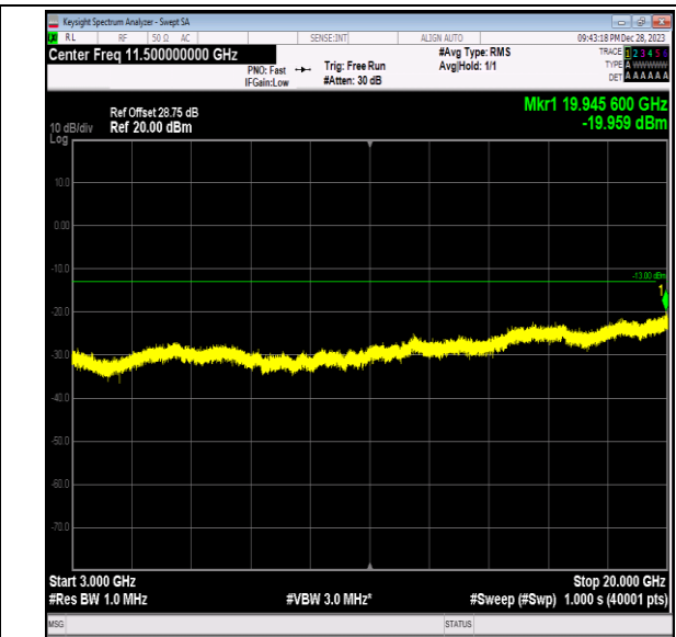
Band2_20MHz_16QAM_18900_1RB#0_3000~20000_300 0~20000
