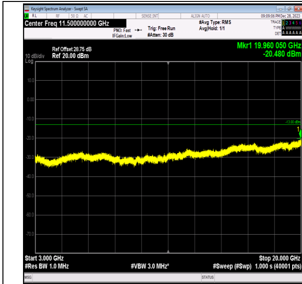
Band2_15MHz_16QAM_18900_1RB#0_3000~20000_300 0~20000
