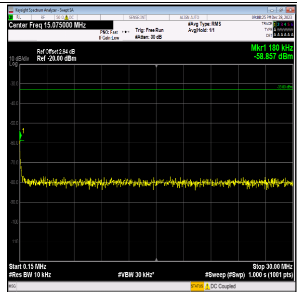
Band2_15MHz_16QAM_18900_1RB#0_0.15~30_0.15~30
