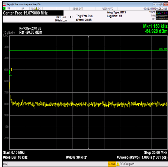
Band2_20MHz_16QAM_18900_1RB#0_0.15~30_0.15~30
