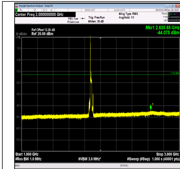
Band2_20MHz_16QAM_18900_1RB#0_1000~3000_1000 ~3000
