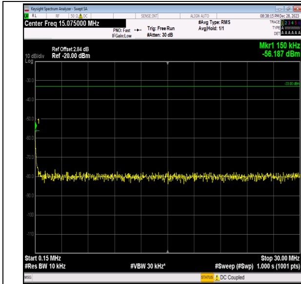
Band2_10MHz_64QAM_19150_1RB#0_0.15~30_0.15~30
