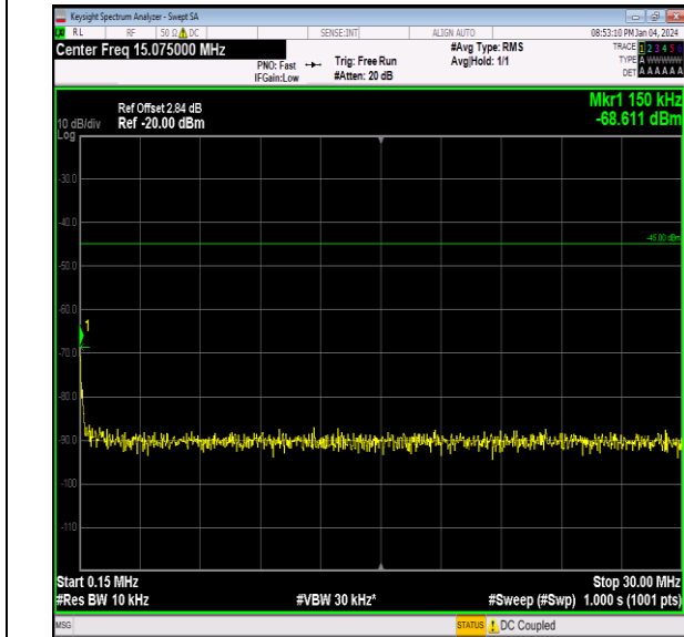
Band7_20MHz_QPSK_20850_1RB#0_0.15~30_0.15~30
