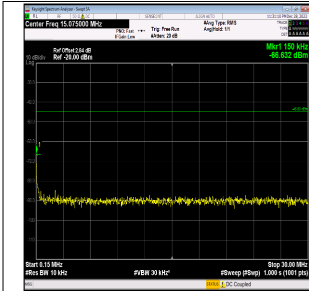
Band7_15MHz_64QAM_21100_1RB#0_0.15~30_0.15~30
