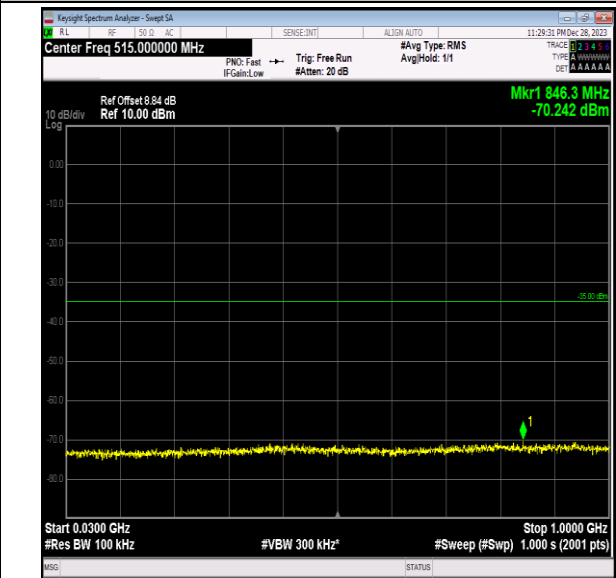
Band7_15MHz_QPSK_21100_1RB#0_30~1000_30~1000
