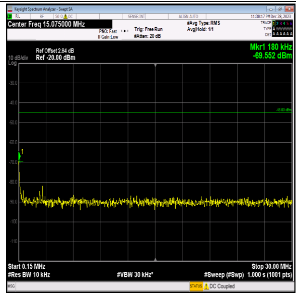
Band7_15MHz_16QAM_21100_1RB#0_0.15~30_0.15~30
