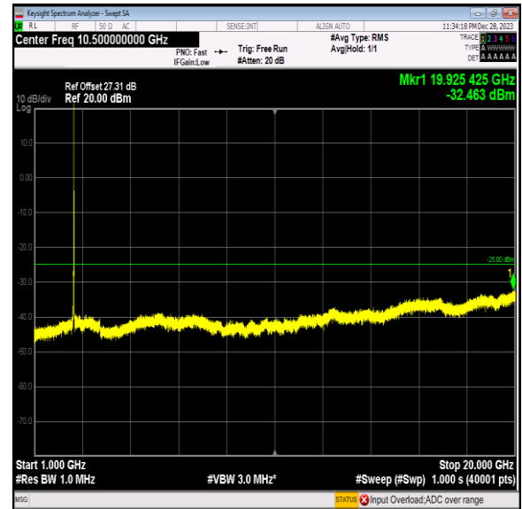
Band7_15MHz_64QAM_21375_1RB#0_1000~20000_100 0~20000
