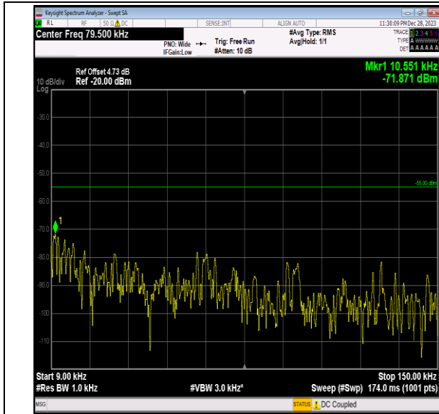
Band7_15MHz_16QAM_21100_1RB#0_0.009~0.15_0.009 ~0.15
