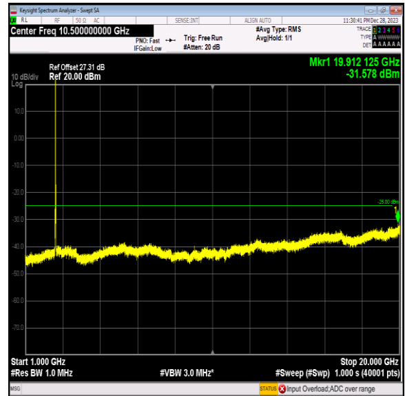
Band7_15MHz_16QAM_21100_1RB#0_1000~20000_100 0~20000
