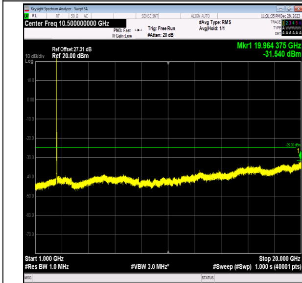
Band7_15MHz_64QAM_21100_1RB#0_1000~20000_100 0~20000
