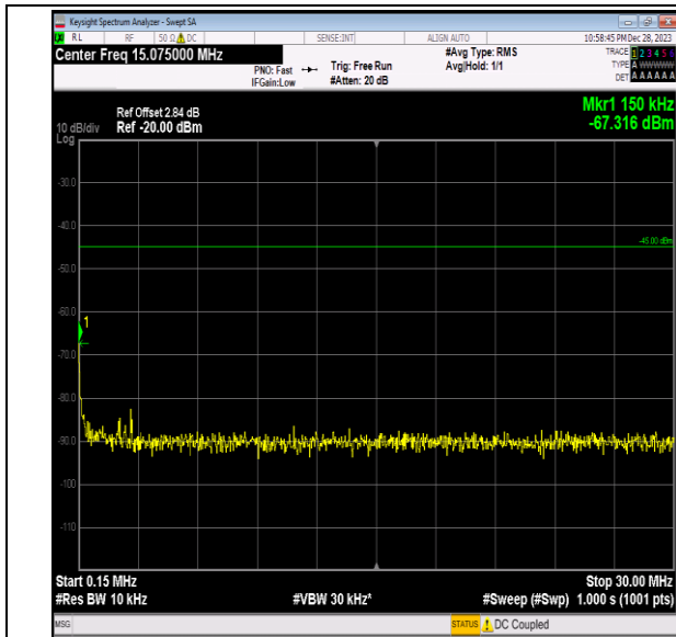
Band7_10MHz_64QAM_21400_1RB#0_0.15~30_0.15~30
