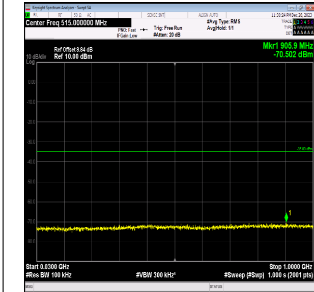
Band7_15MHz_16QAM_21100_1RB#0_30~1000_30~100 0
