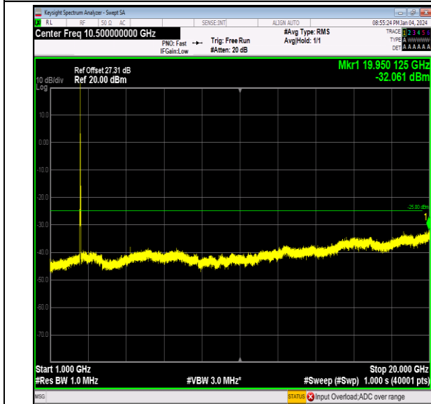
Band7_20MHz_64QAM_20850_1RB#0_1000~20000_100 0~20000
