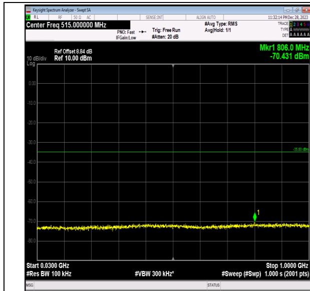
Band7_15MHz_QPSK_21375_1RB#0_30~1000_30~1000
