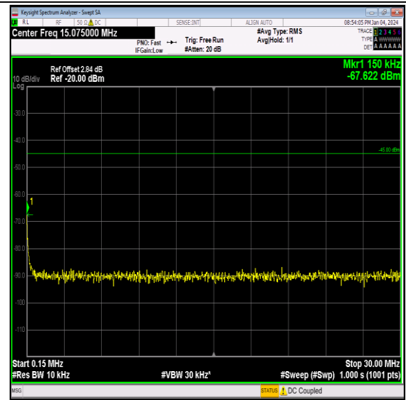
Band7_20MHz_16QAM_20850_1RB#0_0.15~30_0.15~30
