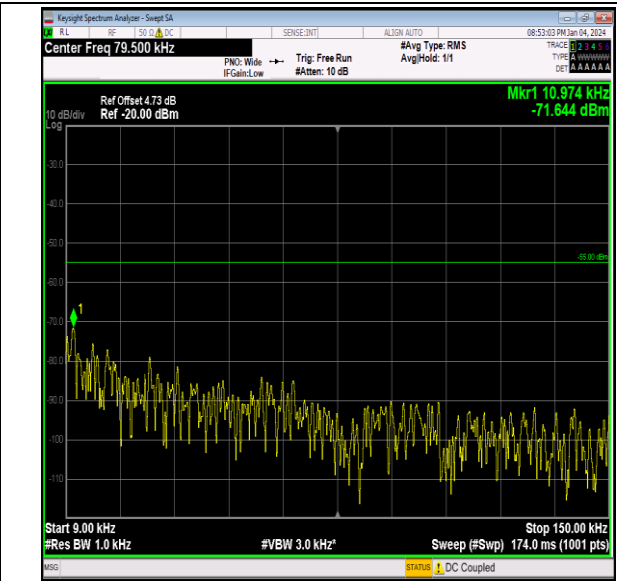
Band7_20MHz_QPSK_20850_1RB#0_0.009~0.15_0.009~0.15
