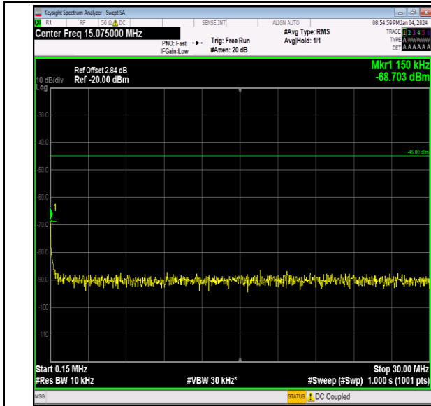
Band7_20MHz_64QAM_20850_1RB#0_0.15~30_0.15~30
