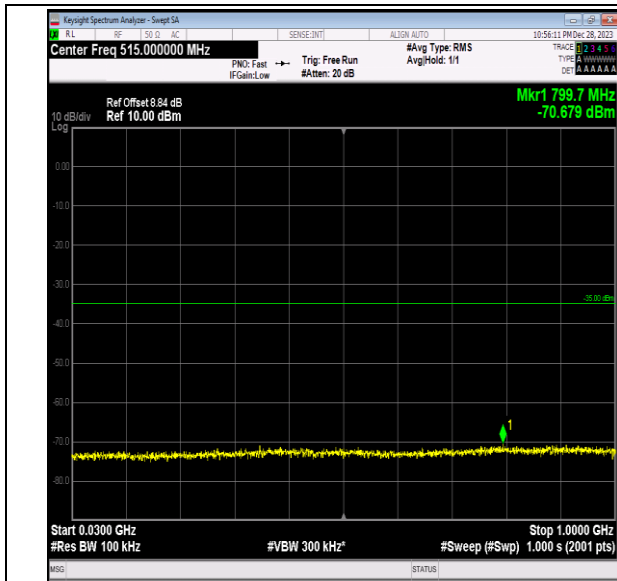
Band7_10MHz_64QAM_21100_1RB#0_30~1000_30~100 0
