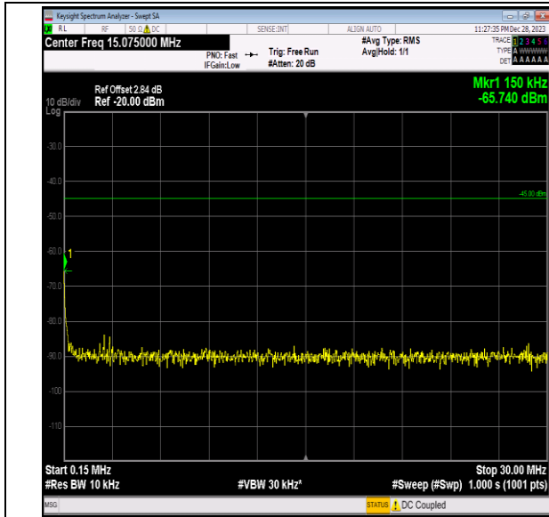
Band7_15MHz_16QAM_20825_1RB#0_0.15~30_0.15~30
