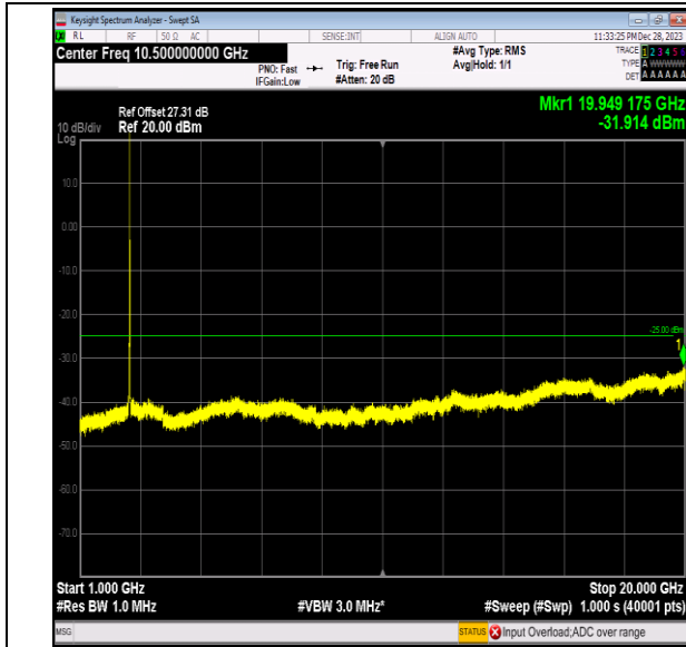
Band7_15MHz_16QAM_21375_1RB#0_1000~20000_100 0~20000
