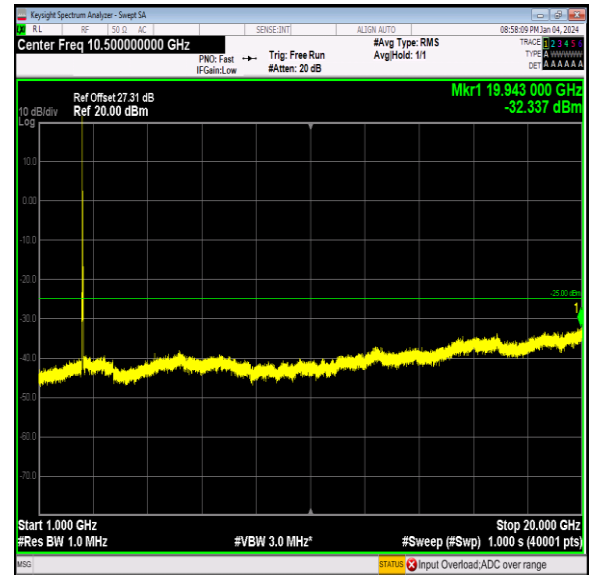
Band7_20MHz_64QAM_21100_1RB#0_1000~20000_100 0~20000
