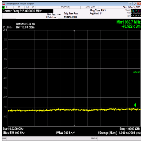
Band7_15MHz_64QAM_21375_1RB#0_30~1000_30~100 0
