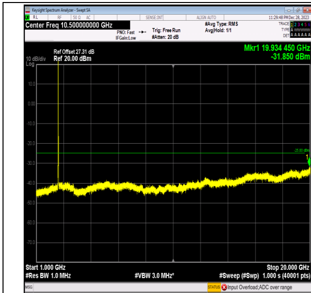
Band7_15MHz_QPSK_21100_1RB#0_1000~20000_1000 ~20000
