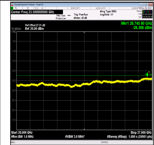
Band7_15MHz_64QAM_21100_1RB#0_20000~27000_20 000~27000
