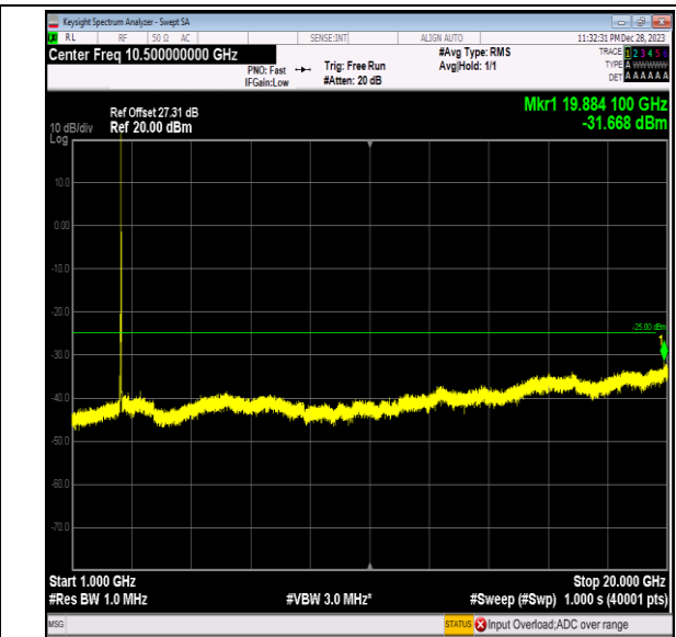
Band7_15MHz_QPSK_21375_1RB#0_1000~20000_1000~20000
