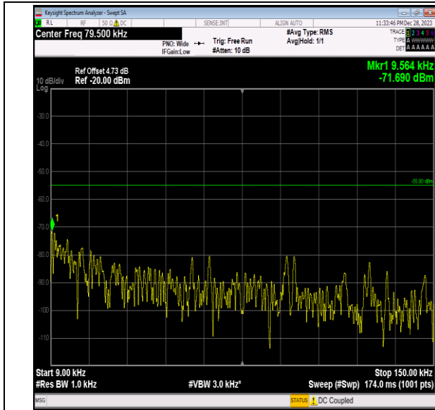
Band7_15MHz_64QAM_21375_1RB#0_0.009~0.15_0.009 ~0.15
