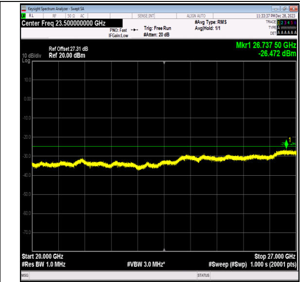
Band7_15MHz_16QAM_21375_1RB#0_20000~27000_20 000~27000
