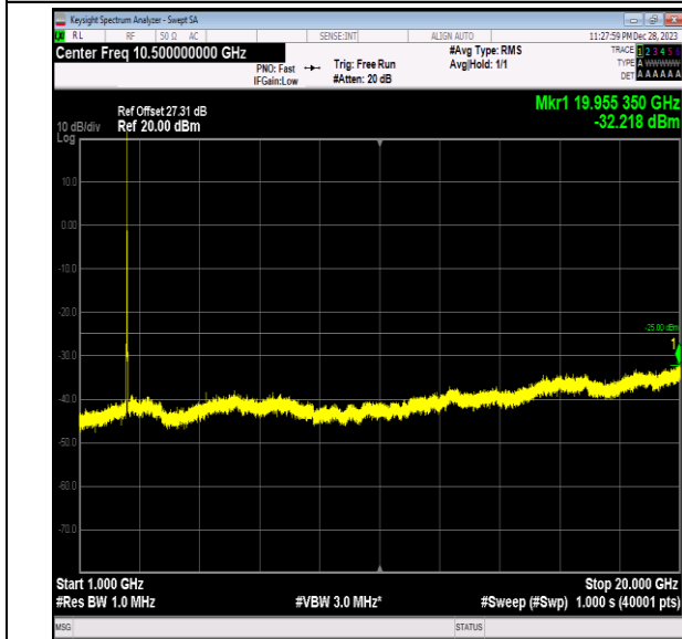
Band7_15MHz_16QAM_20825_1RB#0_1000~20000_1000~20000
