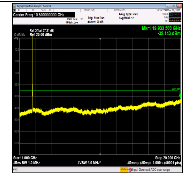
Band7_10MHz_64QAM_21100_1RB#0_1000~20000_100 0~20000
