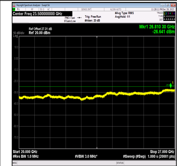
Band7_15MHz_16QAM_20825_1RB#0_20000~27000_20000~27000
