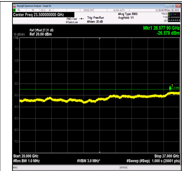
Band7_15MHz_QPSK_21100_1RB#0_20000~27000_200 00~27000
