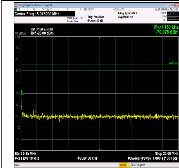
Band7_15MHz_QPSK_21100_1RB#0_0.15~30_0.15~30
