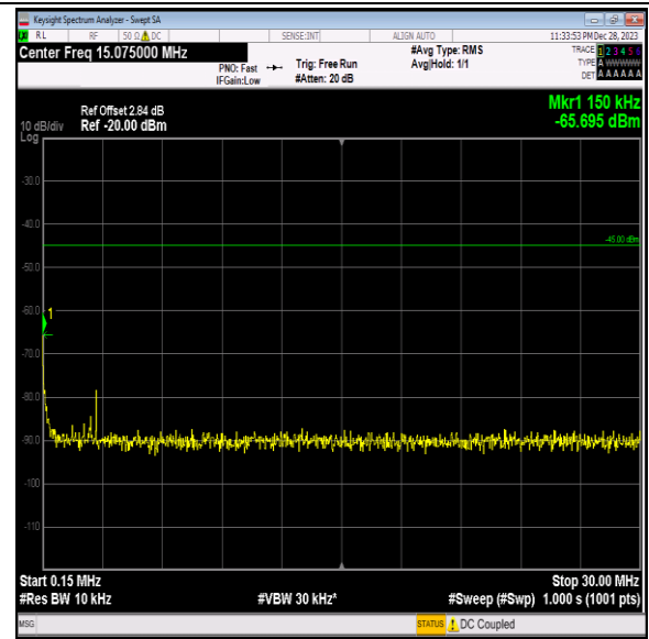
Band7_15MHz_64QAM_21375_1RB#0_0.15~30_0.15~30
