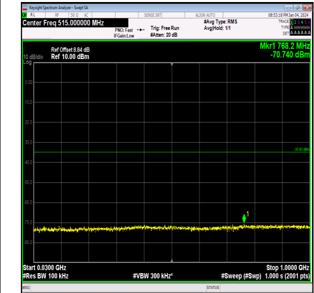
Band7_20MHz_QPSK_20850_1RB#0_30~1000_30~1000
