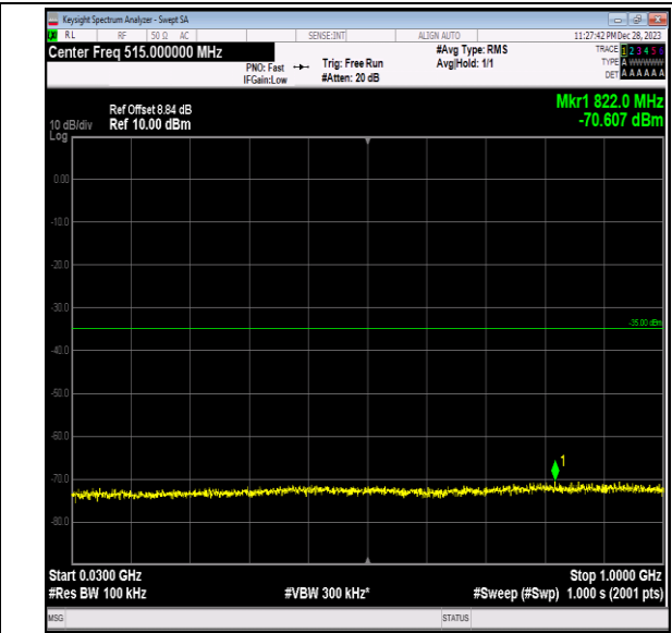
Band7_15MHz_16QAM_20825_1RB#0_30~1000_30~1000
