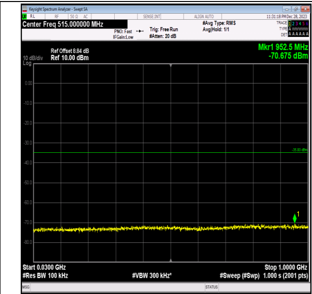
Band7_15MHz_64QAM_21100_1RB#0_30~1000_30~100 0
