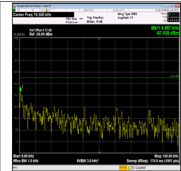
Band7_15MHz_QPSK_21100_1RB#0_0.009~0.15_0.009~0.15
