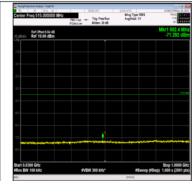
Band7_10MHz_64QAM_21400_1RB#0_30~1000_30~1000
