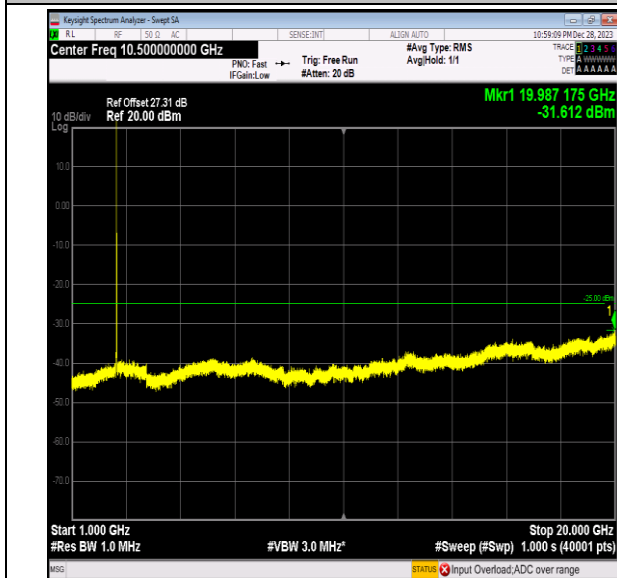
Band7_10MHz_64QAM_21400_1RB#0_1000~20000_1000~20000
