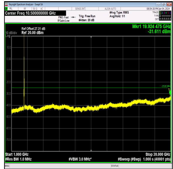
Band7_20MHz_16QAM_20850_1RB#0_1000~20000_100 0~20000
