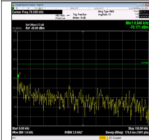
Band7_15MHz_QPSK_21375_1RB#0_0.009~0.15_0.009~ 0.15
