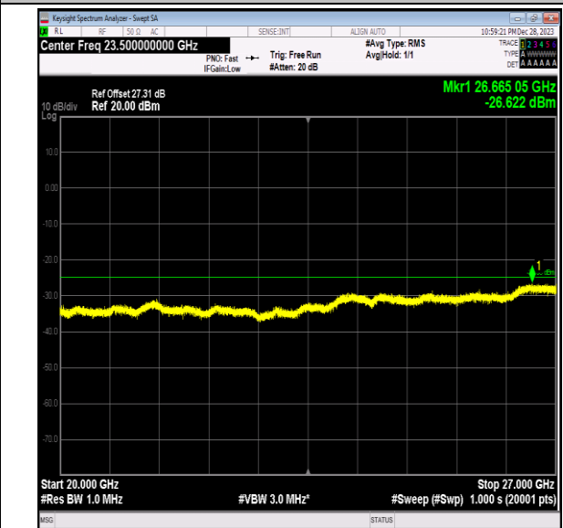
Band7_10MHz_64QAM_21400_1RB#0_20000~27000_20000~27000
