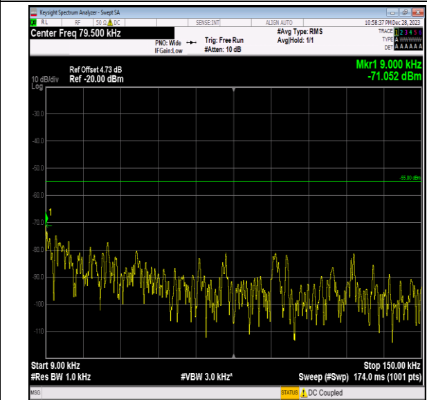
Band7_10MHz_64QAM_21400_1RB#0_0.009~0.15_0.009 ~0.15
