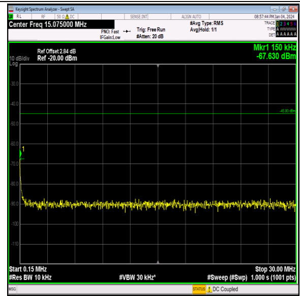
Band7_20MHz_64QAM_21100_1RB#0_0.15~30_0.15~30
