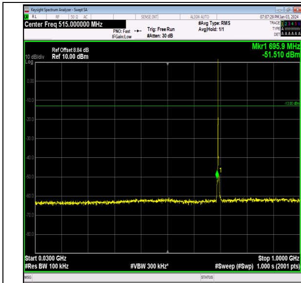
Band12_1.4MHz_QPSK_23017_1RB#0_30~1000_30~100 0
