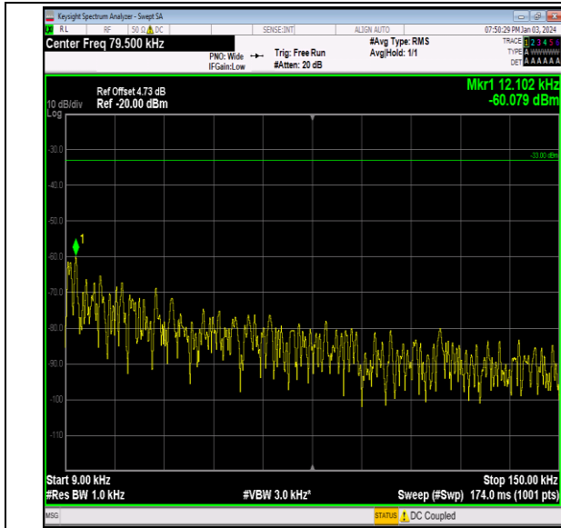
Band12_3MHz_QPSK_23095_1RB#0_0.009~0.15_0.009~0.15
