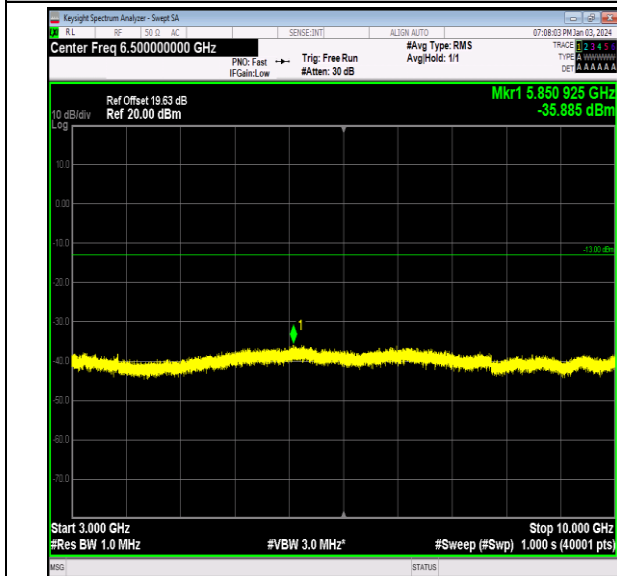
Band12_1.4MHz_QPSK_23017_1RB#0_3000~10000_300 0~10000
