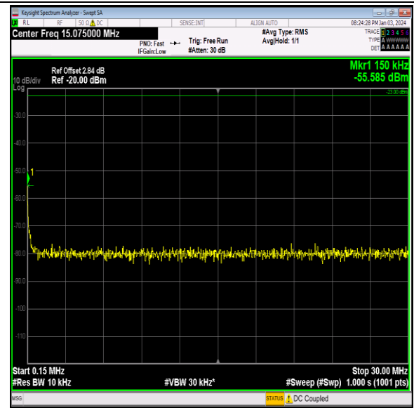
Band12_5MHz_QPSK_23035_1RB#0_0.15~30_0.15~30
