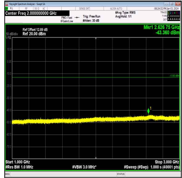
Band12_5MHz_QPSK_23035_1RB#0_1000~3000_1000~3000
