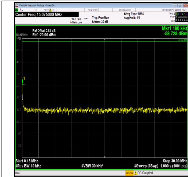
Band12_3MHz_QPSK_23025_1RB#0_0.15~30_0.15~30
