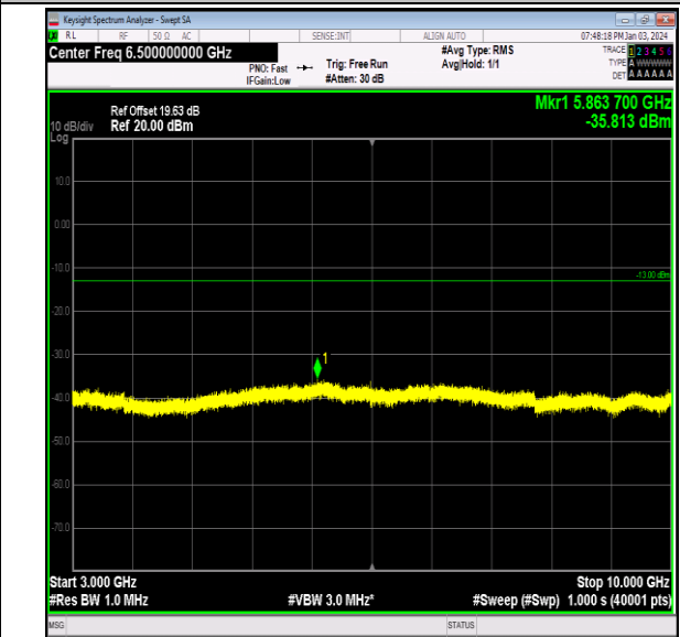
Band12_3MHz_QPSK_23025_1RB#0_3000~10000_3000~10000
