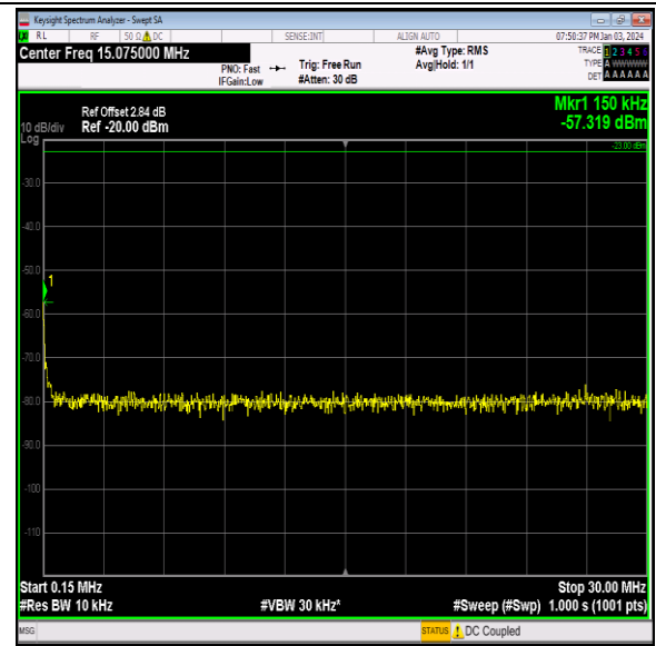
Band12_3MHz_QPSK_23095_1RB#0_0.15~30_0.15~30
