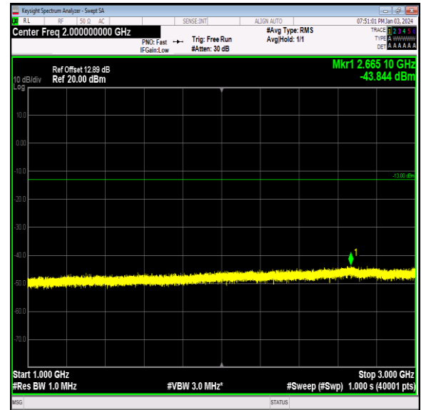
Band12_3MHz_QPSK_23095_1RB#0_1000~3000_1000~3000
