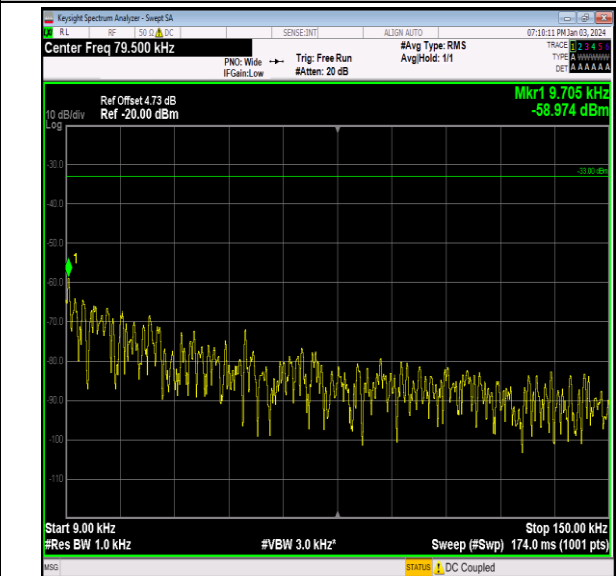
Band12_1.4MHz_QPSK_23095_1RB#0_0.009~0.15_0.00 9~0.15
