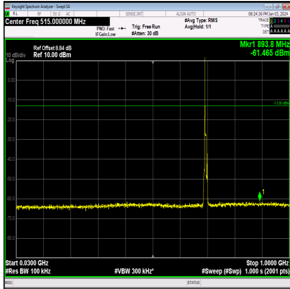
Band12_5MHz_QPSK_23035_1RB#0_30~1000_30~1000
