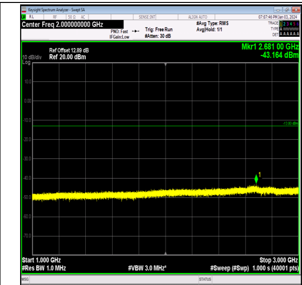
Band12_1.4MHz_QPSK_23017_1RB#0_1000~3000_1000 ~3000
