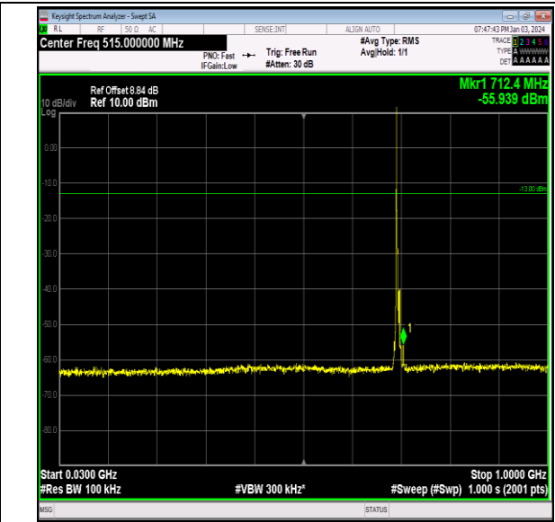
Band12_3MHz_QPSK_23025_1RB#0_30~1000_30~1000
