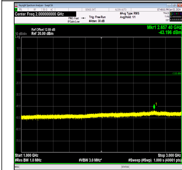
Band12_3MHz_QPSK_23025_1RB#0_1000~3000_1000~3000
