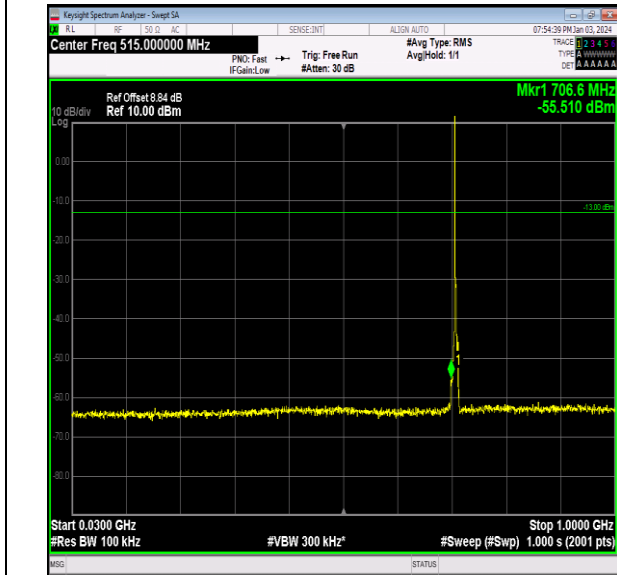
Band12_3MHz_16QAM_23165_1RB#0_30~1000_30~100 0
